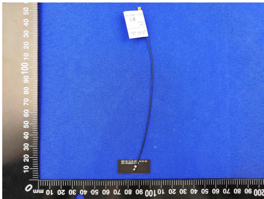
Antenna-iM50/iM60/iM70/iM80/X10/X12
