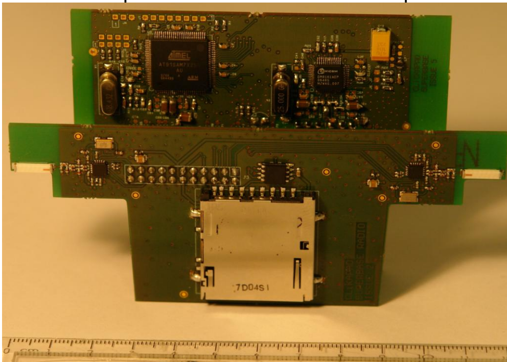
CLiKAPAD SuperBase Internal Front close-up
