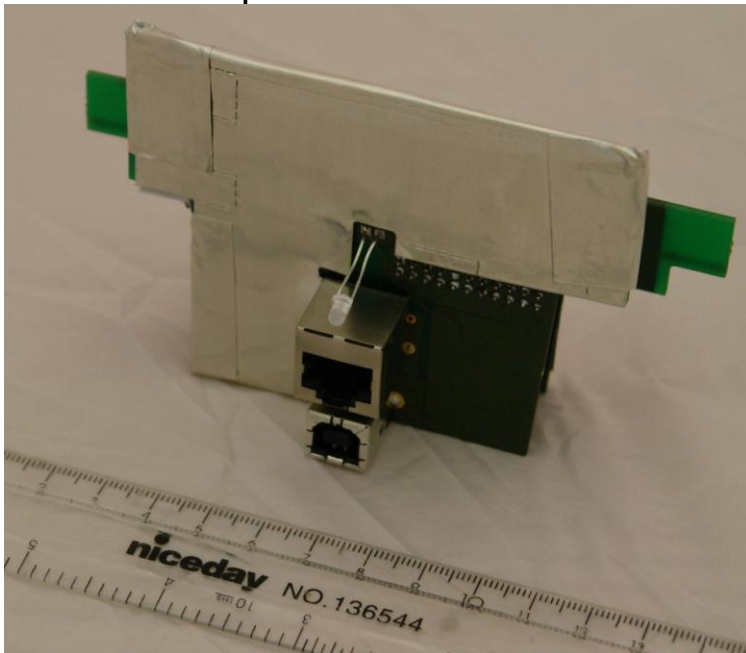
CLiKAPAD SuperBase Internal Back with SHIELD fitted
