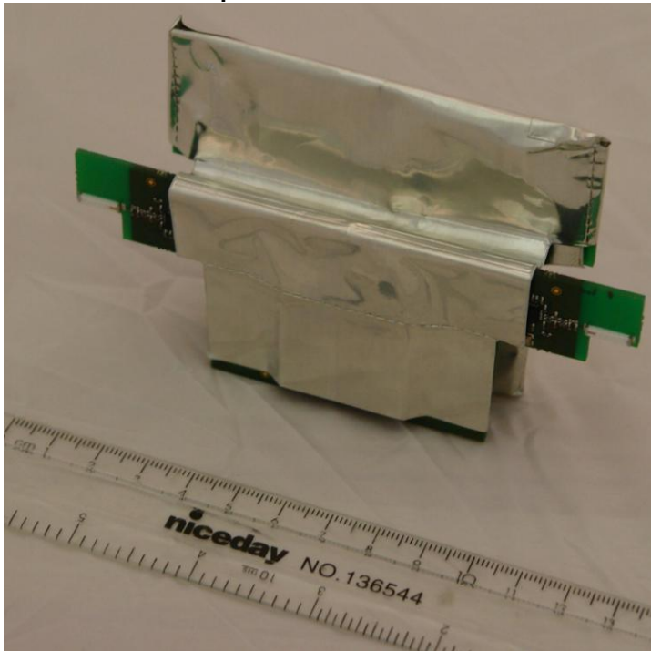
CLiKAPAD SuperBase Internal Front with SHIELD fitted
