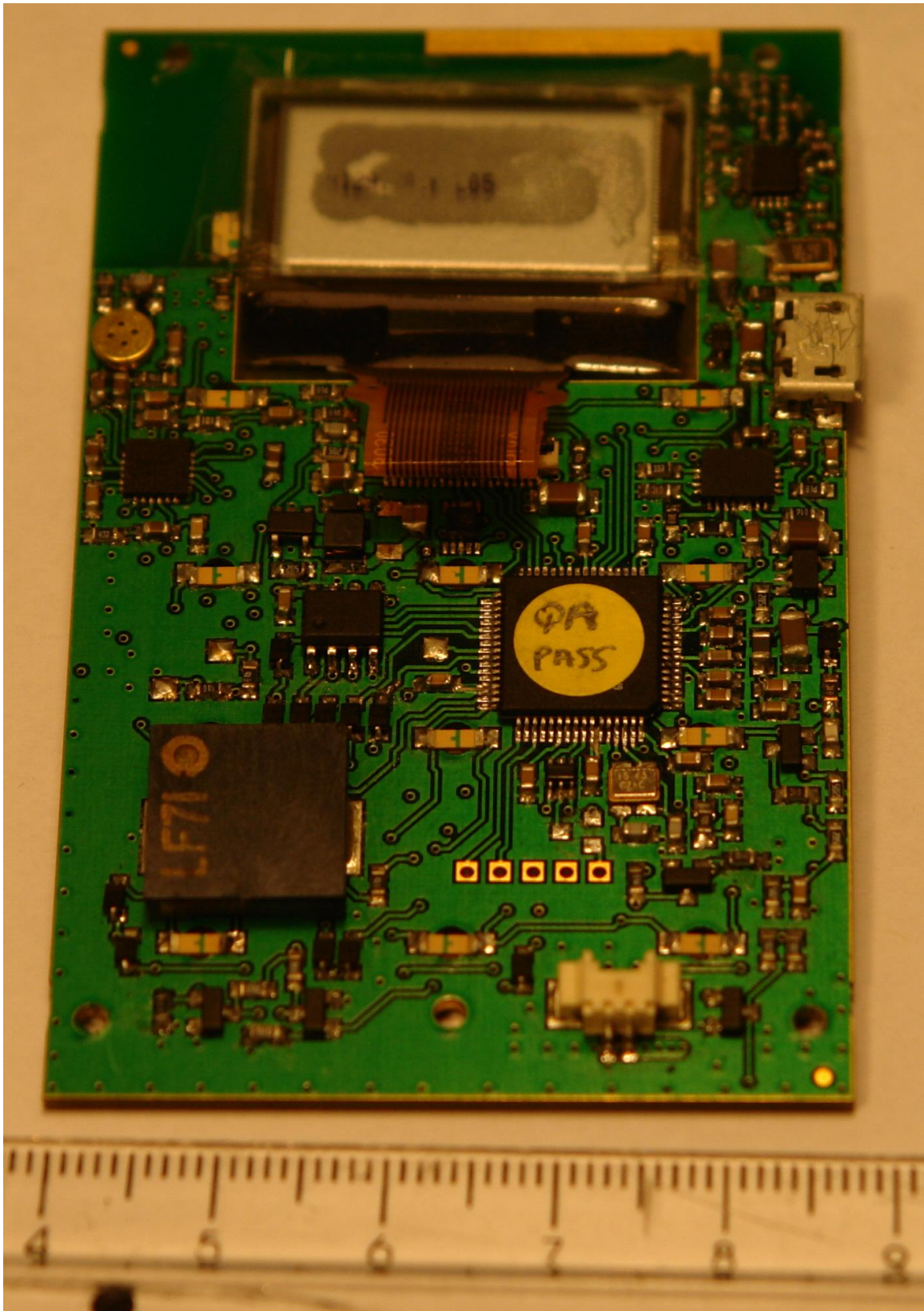
CLiKAPADprioritizer internal - COMPONENT side
