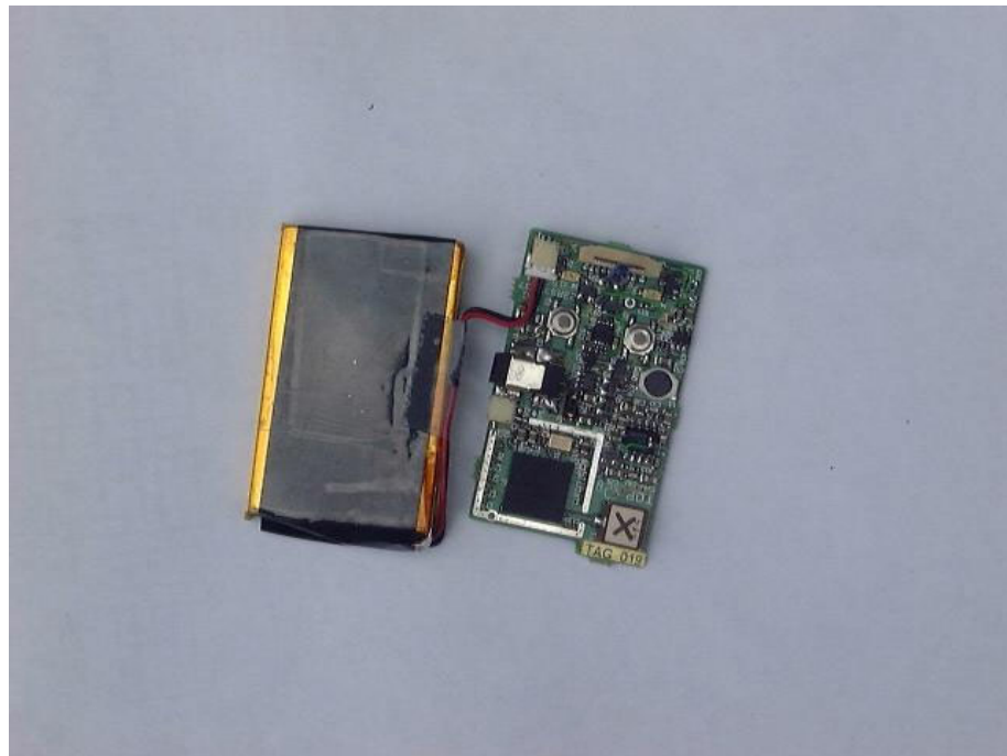
Figure 3 PCB and Battery Side 1
