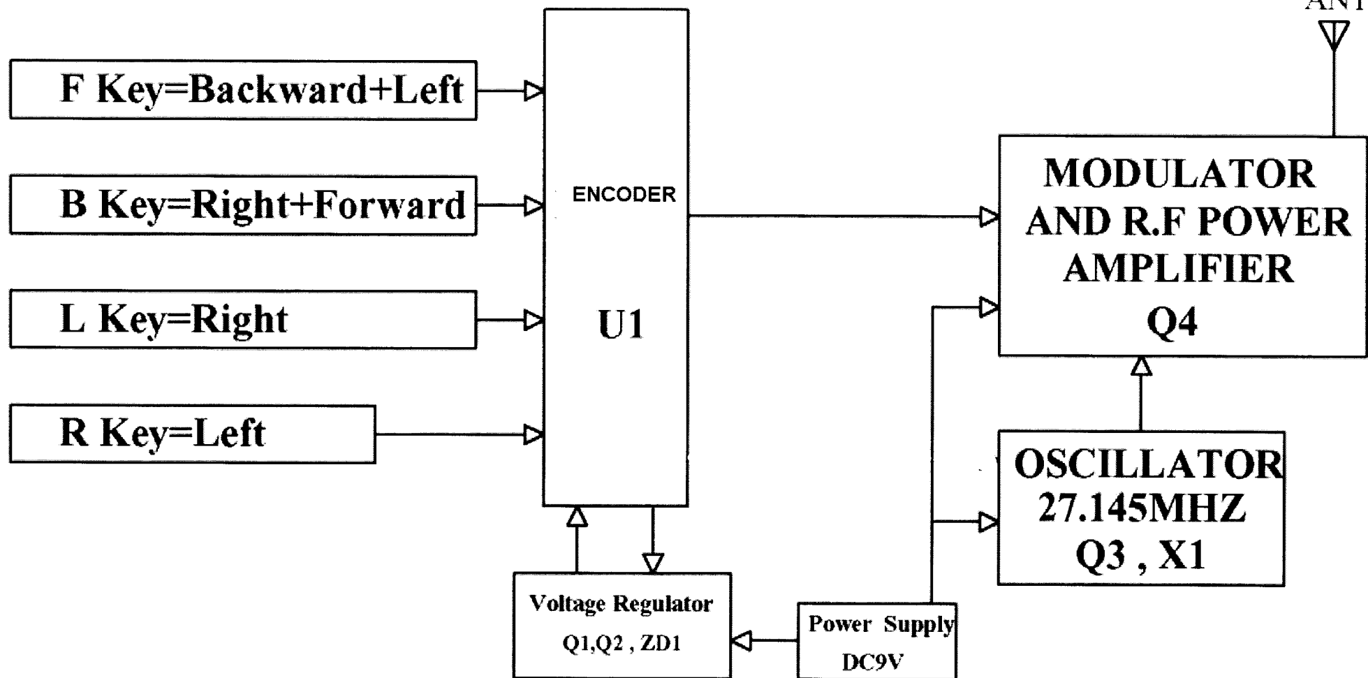
TX 27.145MHz -FUNCTION BLOCK DIAGRAM
