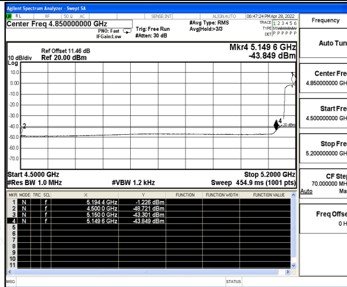
11AC40SISO_Ant_Low_5190_Peak
