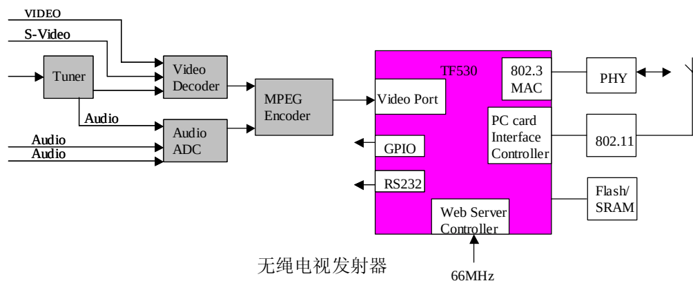
Wireless TV Transmitter
