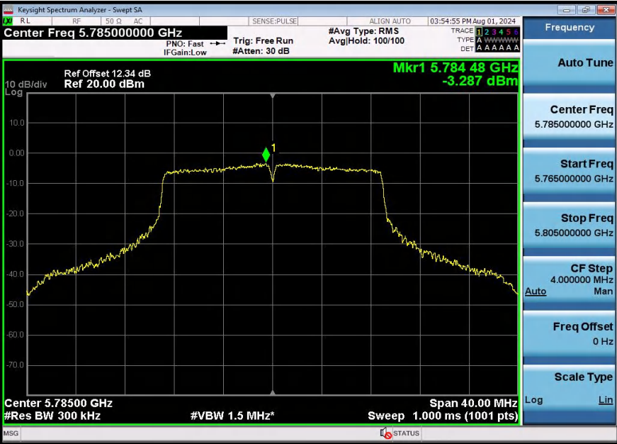
11AC20SISO-Ant1-5785-PASS
