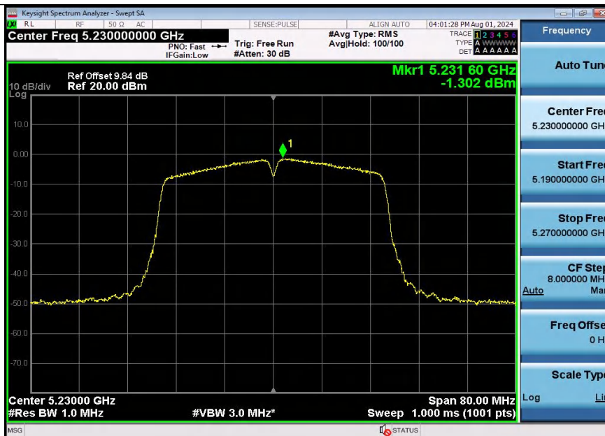
11AC40SISO-Ant1-5230-PASS
