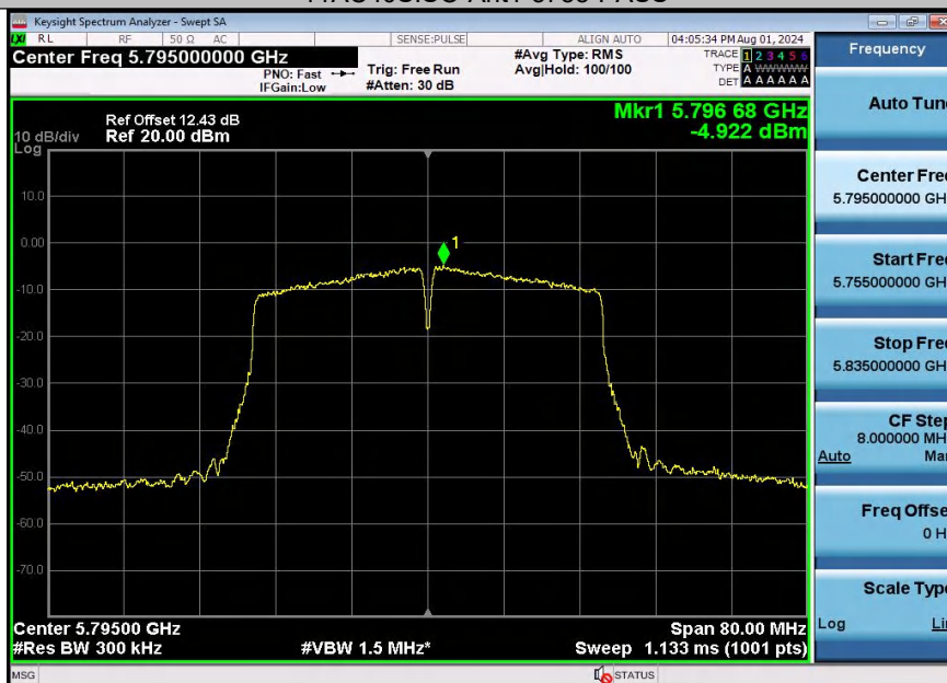
11AC40SISO-Ant1-5795-PASS
