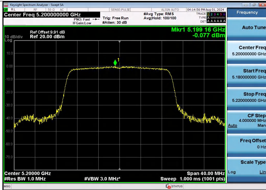
11AX20SISO-Ant1-5200-PASS
