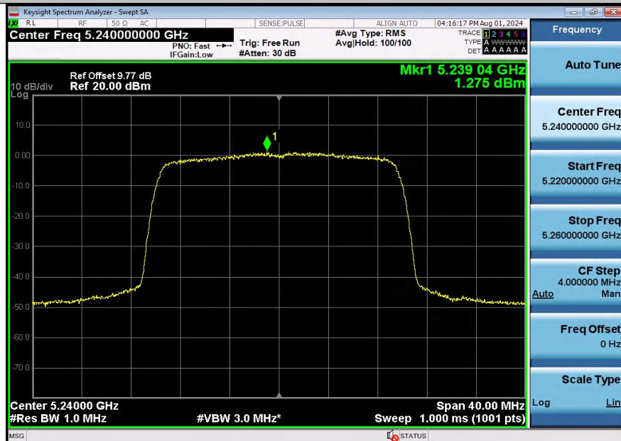
11AX20SISO-Ant1-5240-PASS
