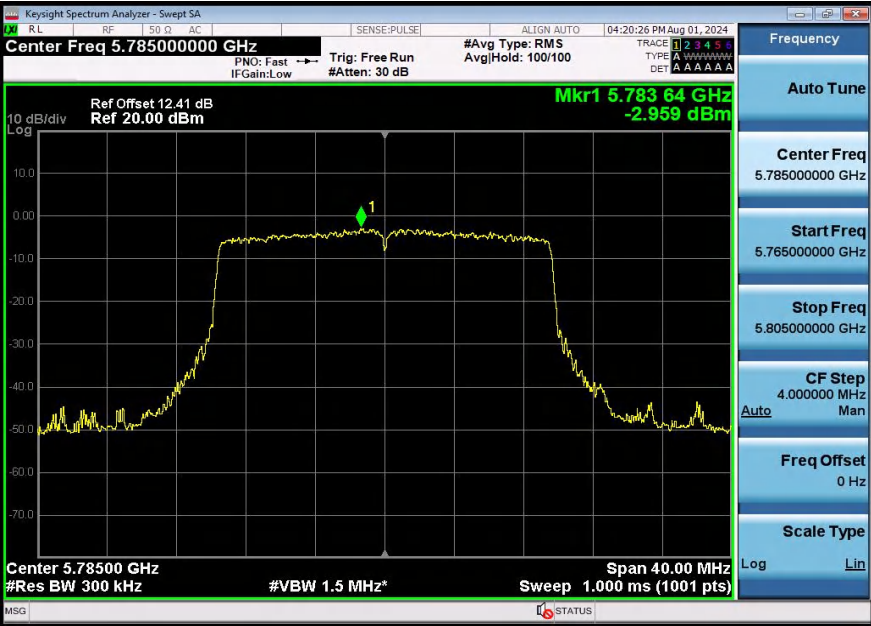
11AX20SISO-Ant1-5785-PASS
