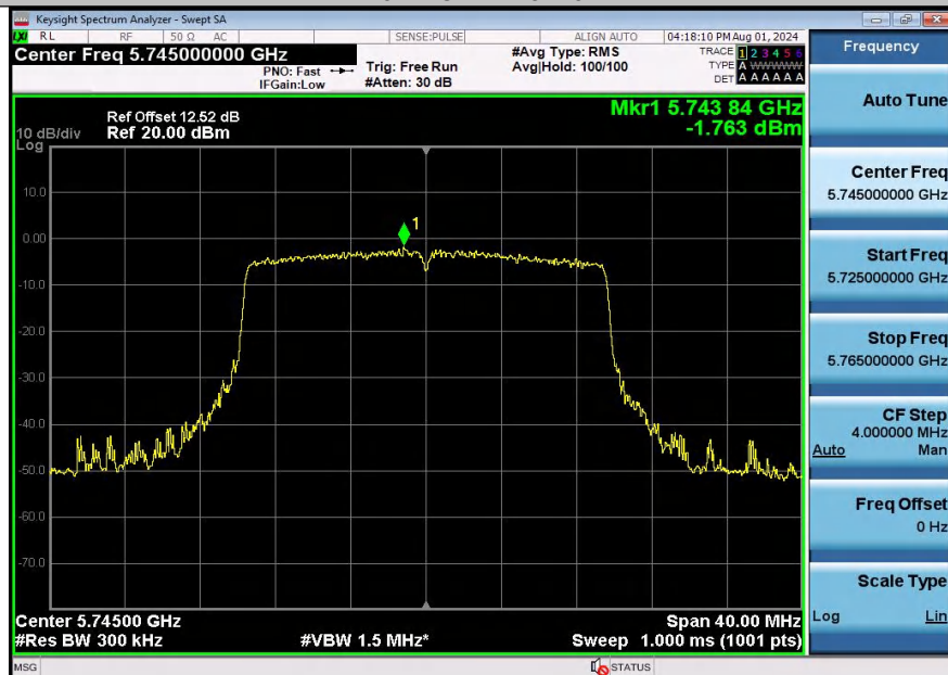
11AX20SISO-Ant1-5745-PASS
