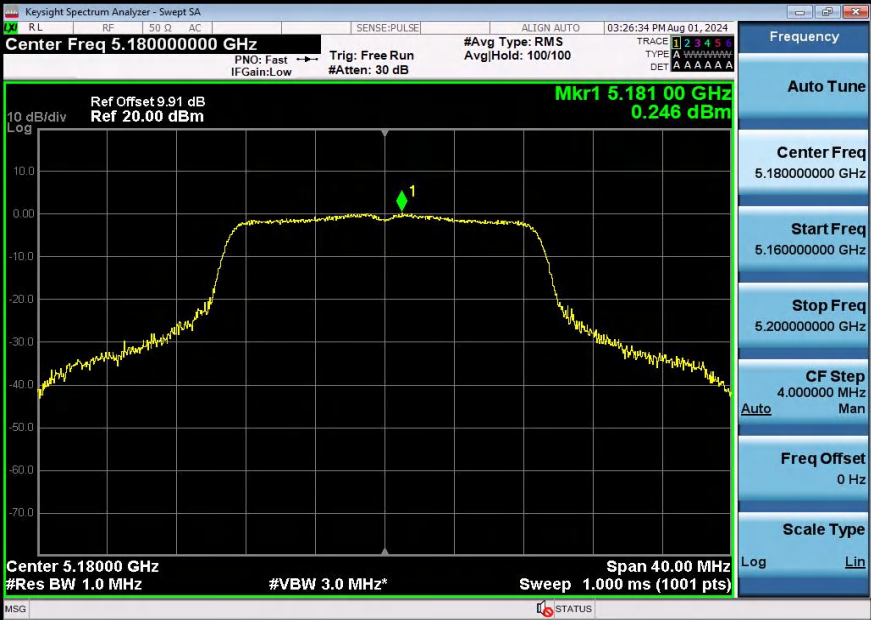
11N20SISO-Ant1-5180-PASS
