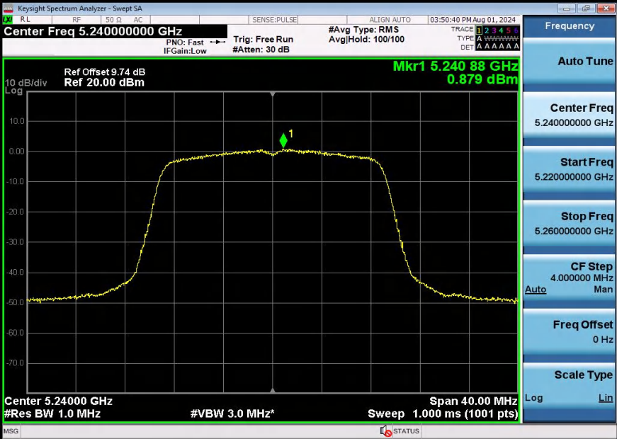
11AC20SISO-Ant1-5240-PASS
