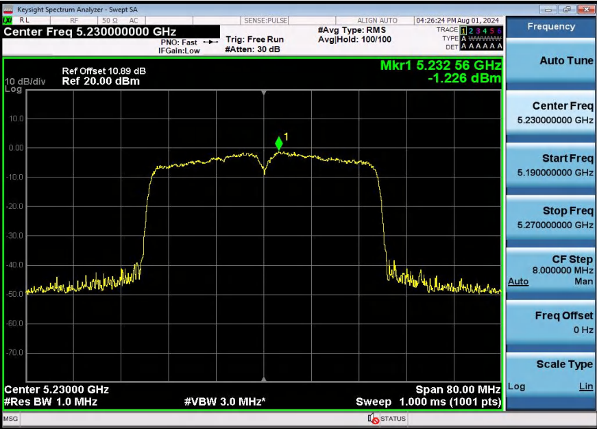
11AX40SISO-Ant1-5230-PASS
