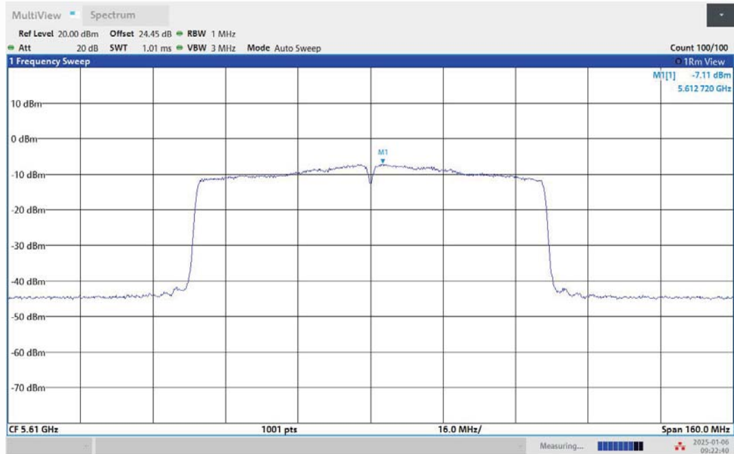
11AC80MIMO-Ant2-5610-PASS
