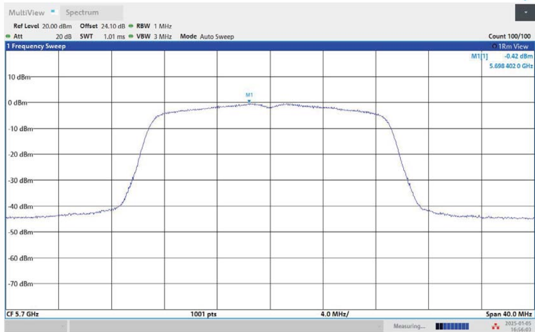
11AC20MIMO-Ant2-5700-PASS
