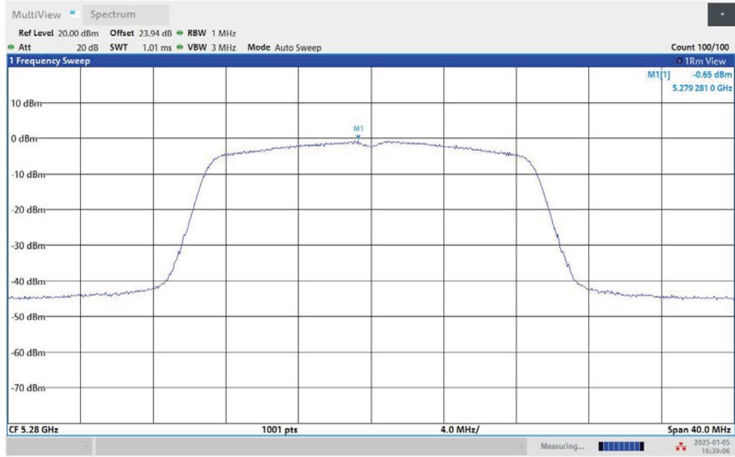
11AC20MIMO-Ant1-5280-PASS
