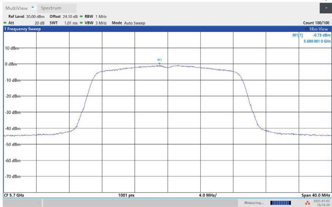
11AC20MIMO-Ant1-5700-PASS
