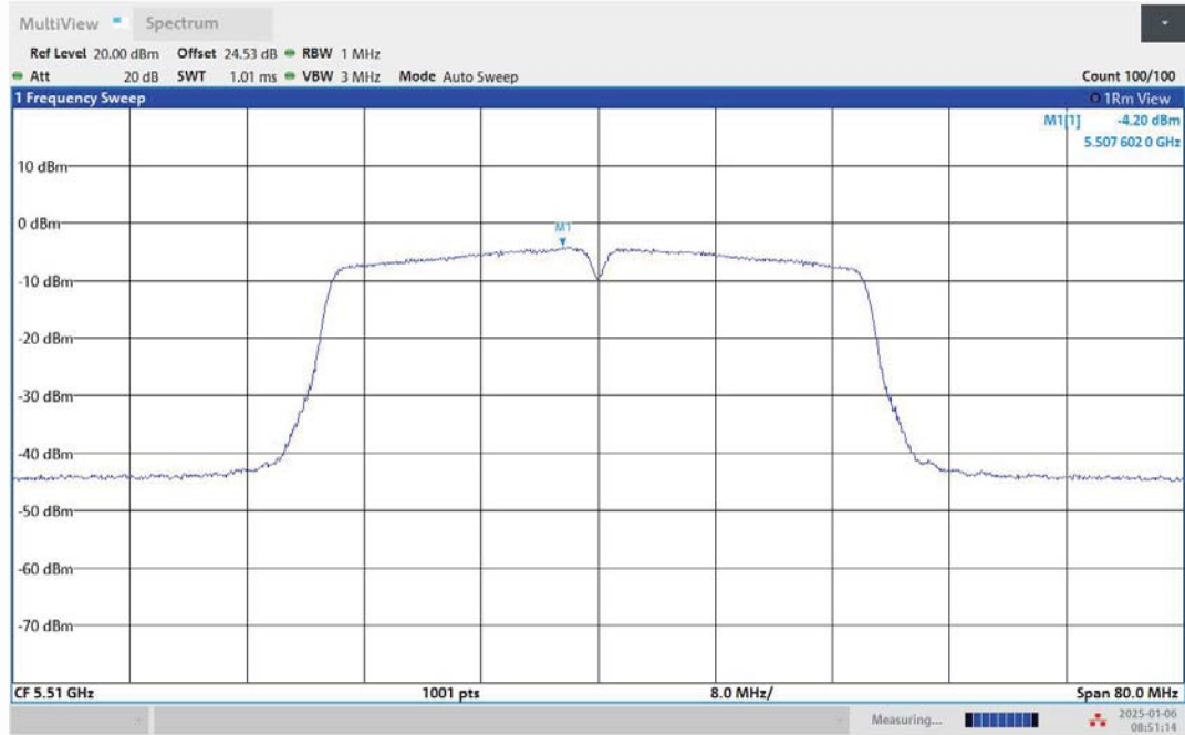
11AC40MIMO-Ant1-5510-PASS
