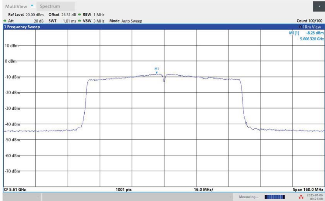
11AC80MIMO-Ant1-5610-PASS
