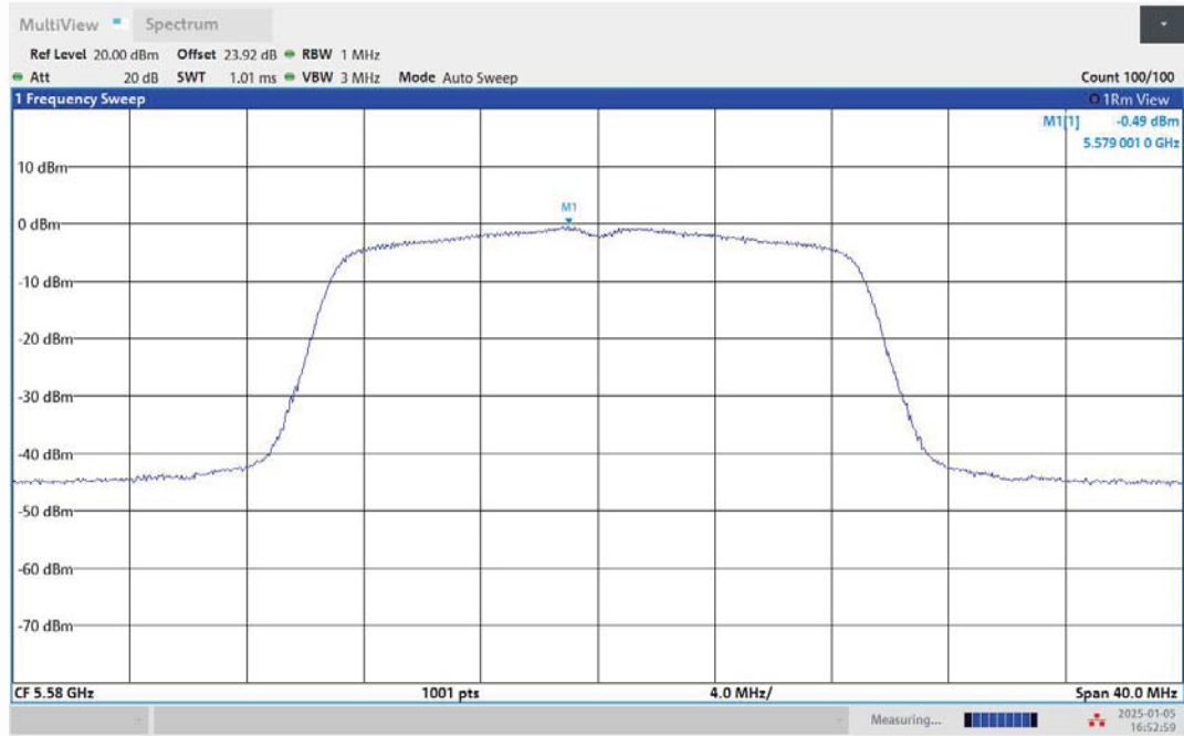
11AC20MIMO-Ant2-5580-PASS
