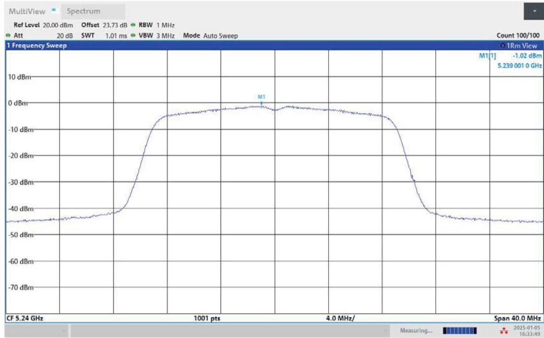
11AC20MIMO-Ant2-5240-PASS
