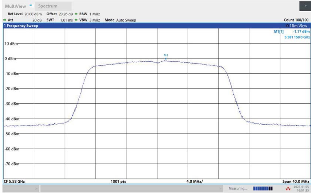
11AC20MIMO-Ant1-5580-PASS
