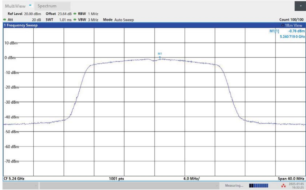
11AC20MIMO-Ant1-5240-PASS
