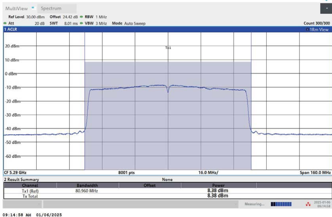
11AC80MIMO-Ant2-5290-PASS
