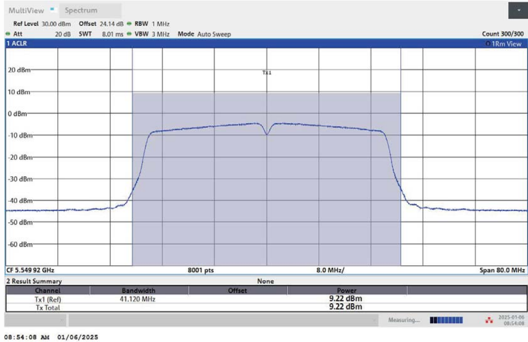
11AC40MIMO-Ant1-5550-PASS
