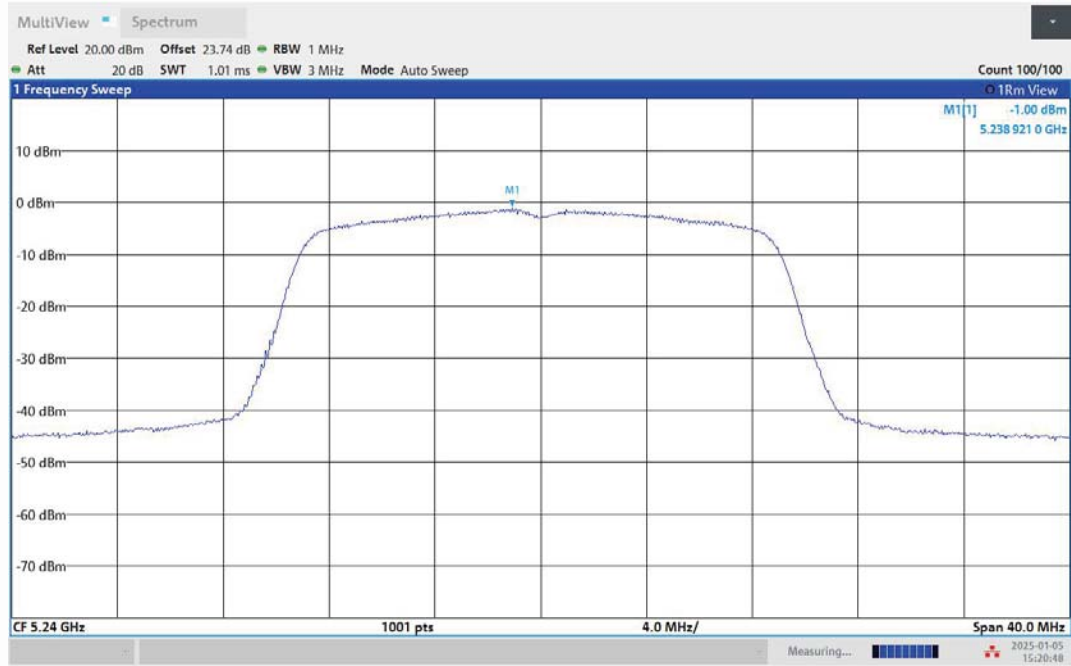
11N20MIMO-Ant2-5240-PASS
