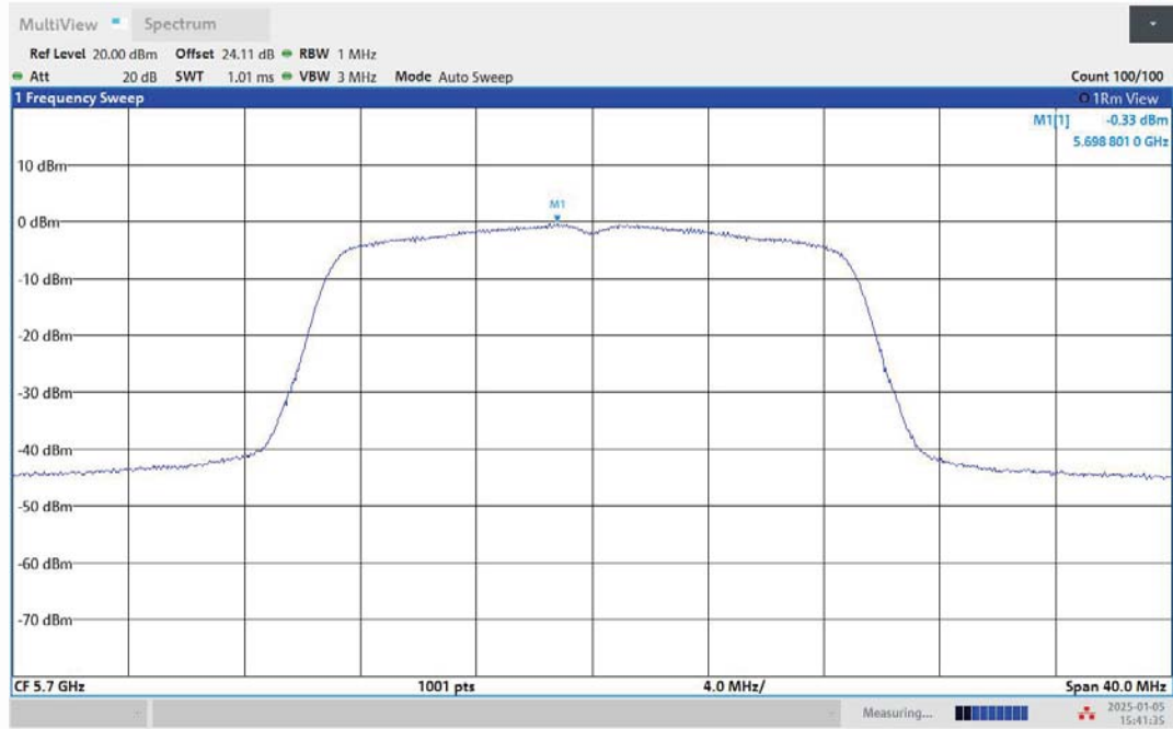
11N20MIMO-Ant2-5700-PASS
