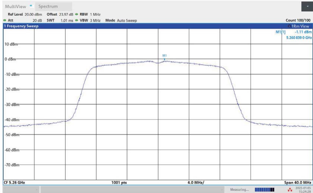
11N20MIMO-Ant2-5260-PASS
