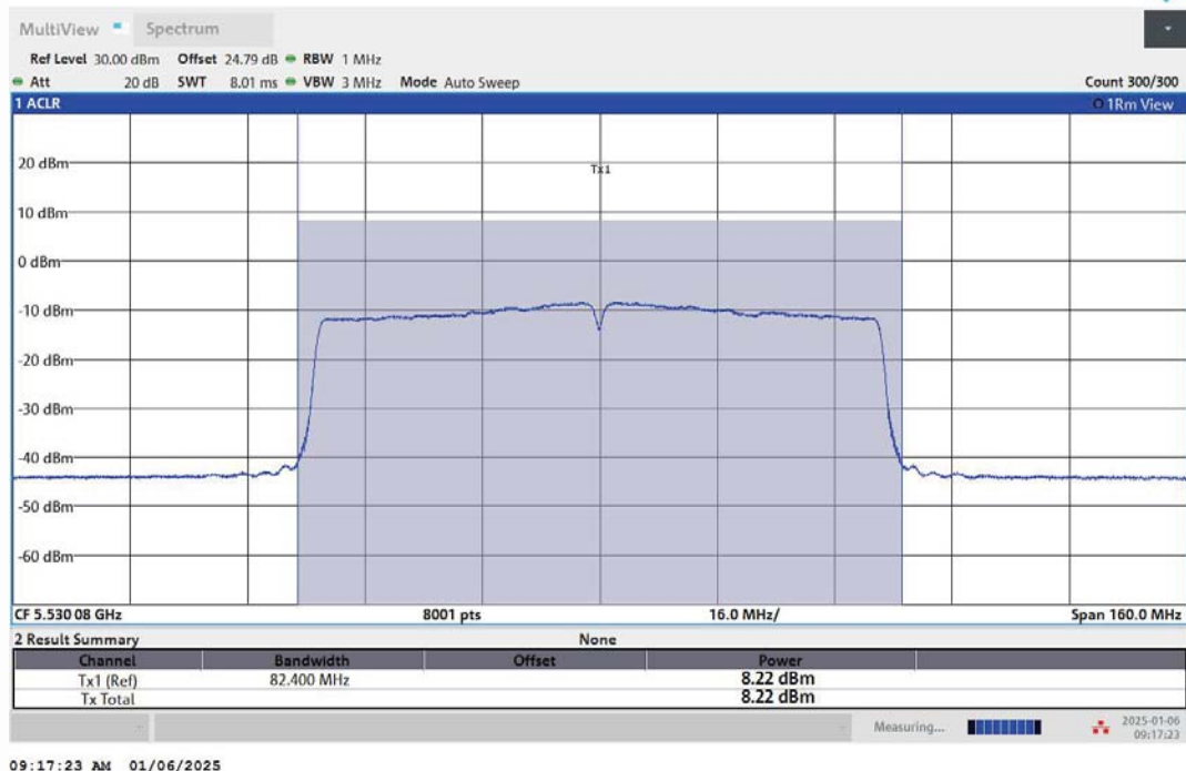
11AC80MIMO-Ant1-5530-PASS
