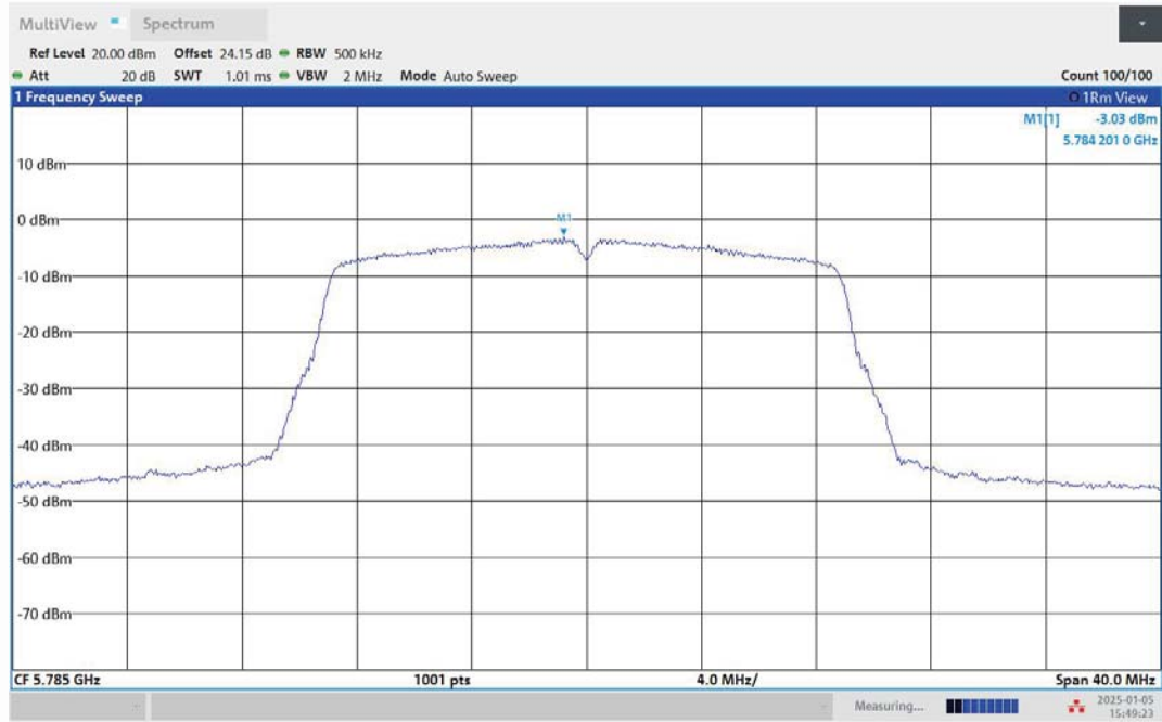
11N20MIMO-Ant2-5785-PASS
