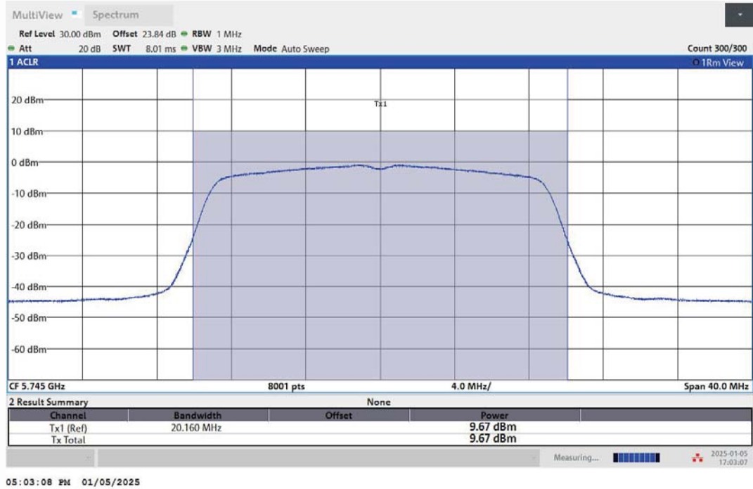
11AC20MIMO-Ant1-5745-PASS
