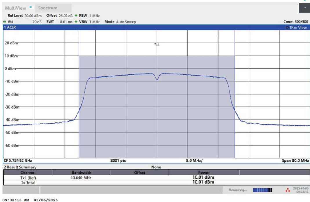
11AC40MIMO-Ant2-5755-PASS
