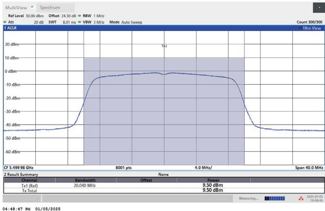
11AC20MIMO-Ant2-5500-PASS
