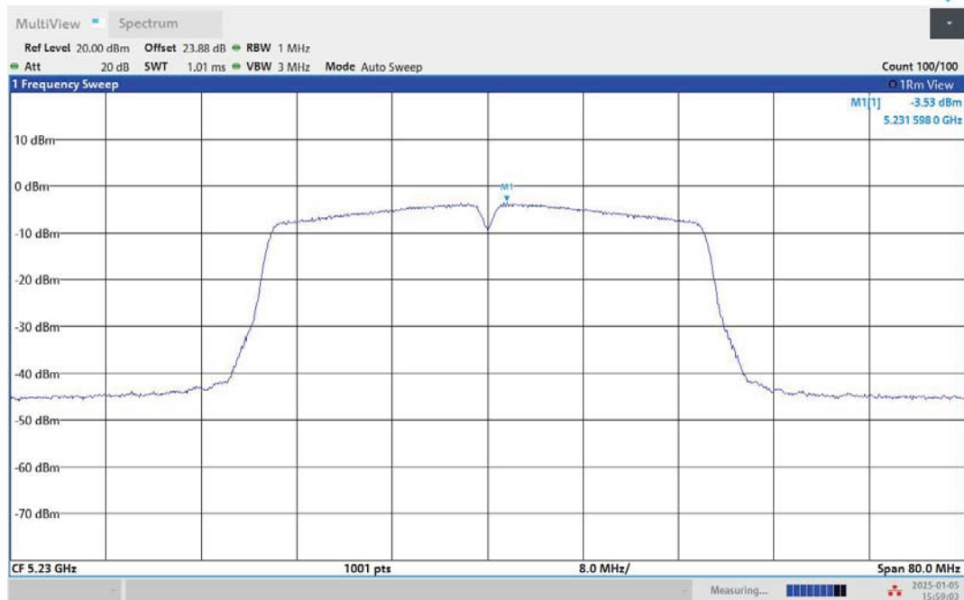
11N40MIMO-Ant1-5230-PASS
