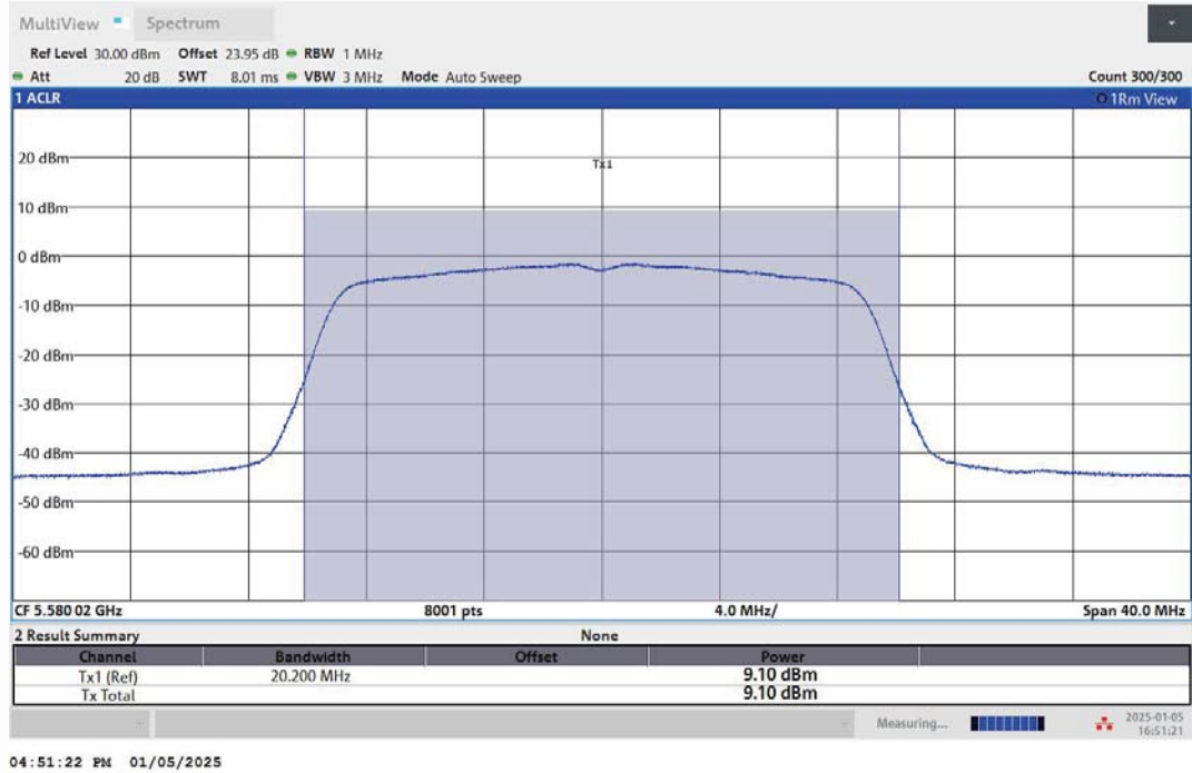
11AC20MIMO-Ant1-5580-PASS
