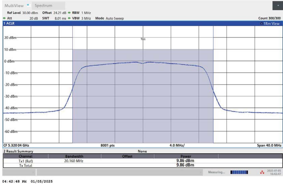
11AC20MIMO-Ant1-5320-PASS
