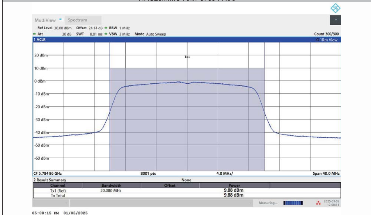
11AC20MIMO-Ant2-5785-PASS
