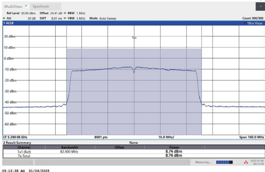
11AC80MIMO-Ant1-5290-PASS
