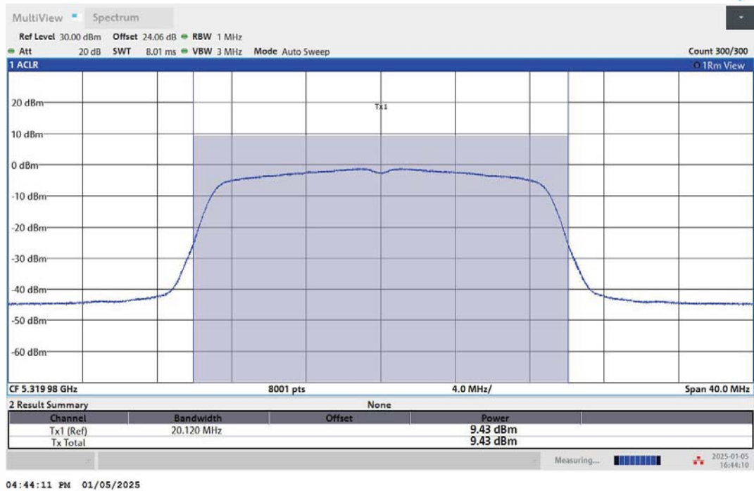
11AC20MIMO-Ant2-5320-PASS
