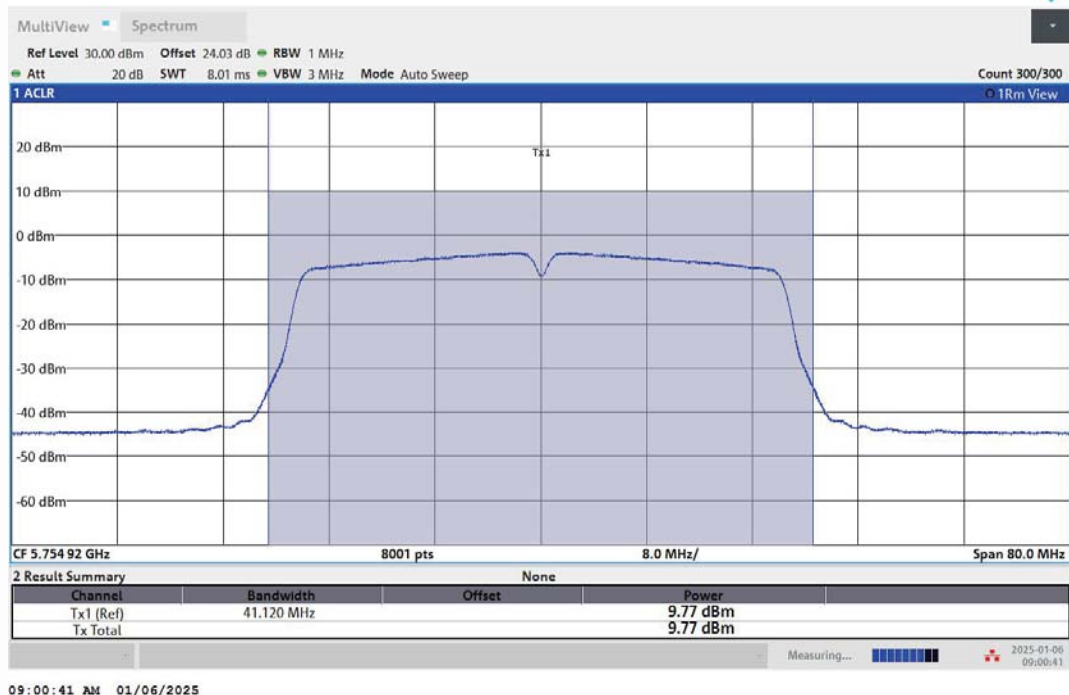
11AC40MIMO-Ant1-5755-PASS
