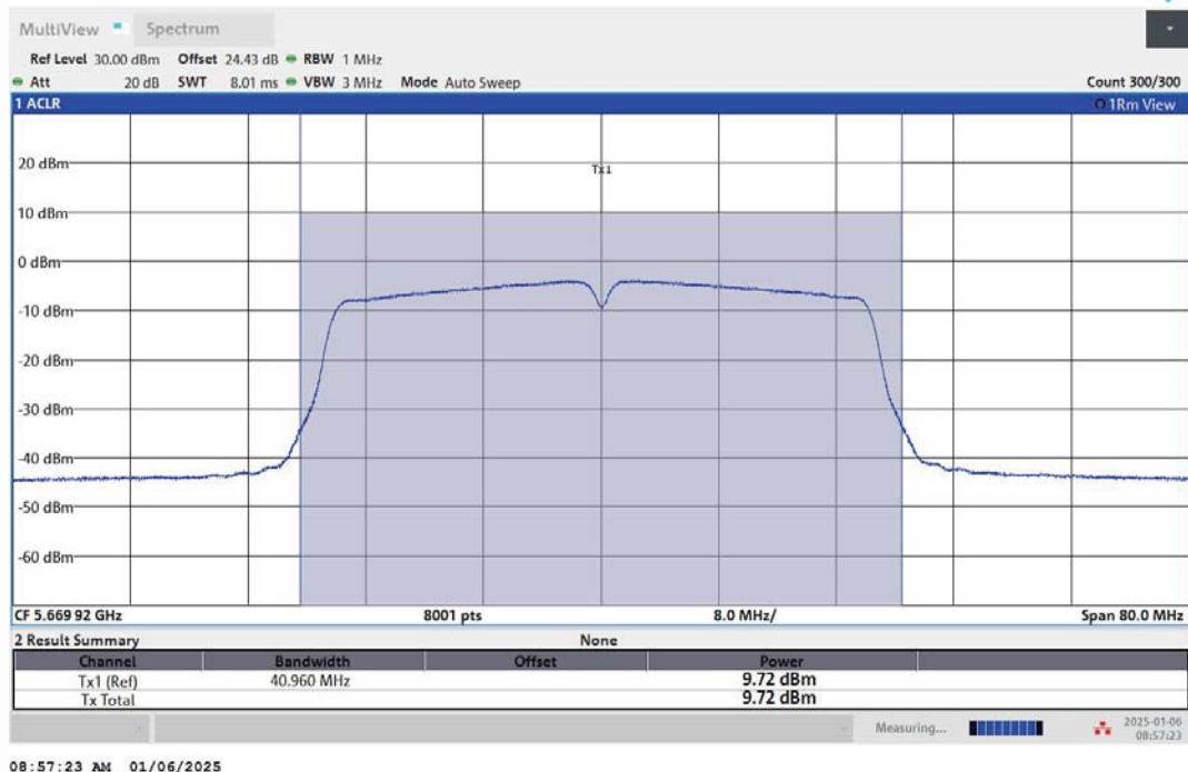
11AC40MIMO-Ant1-5670-PASS
