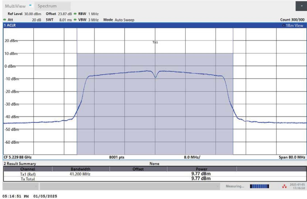
11AC40MIMO-Ant1-5230-PASS
