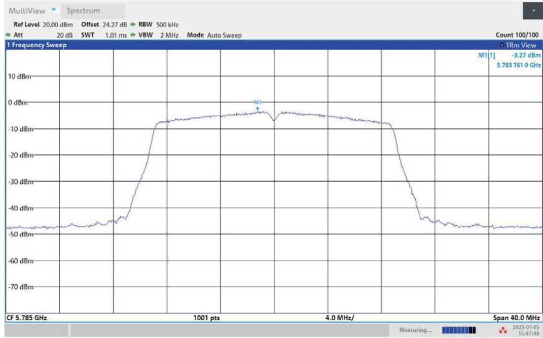
11N20MIMO-Ant1-5785-PASS
