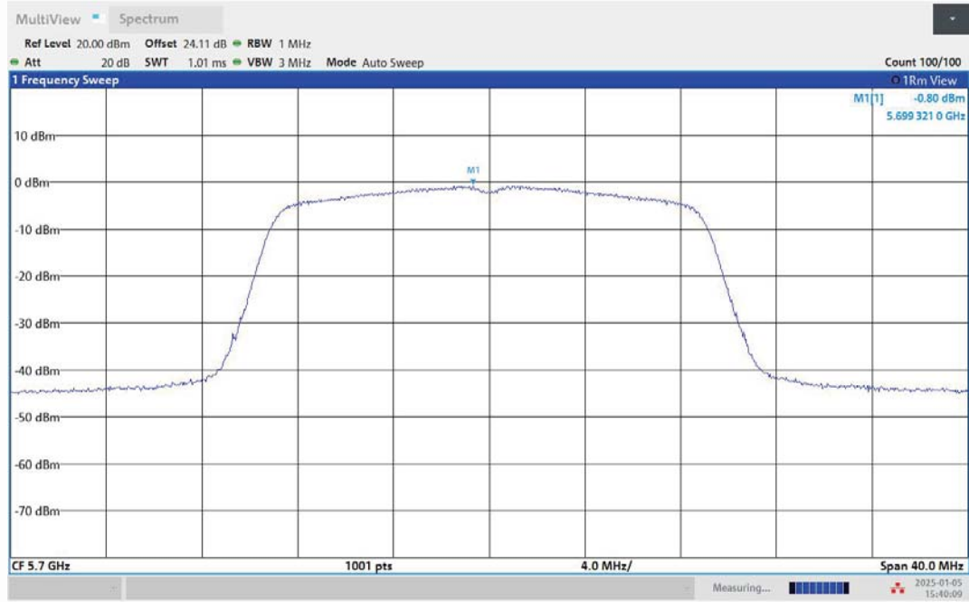
11N20MIMO-Ant1-5700-PASS
