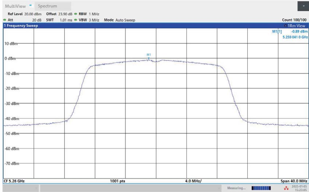
11N20MIMO-Ant1-5260-PASS
