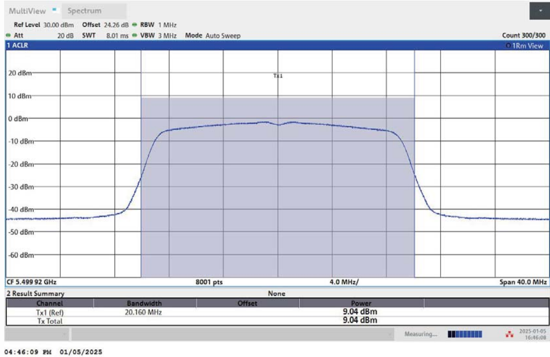
11AC20MIMO-Ant1-5500-PASS
