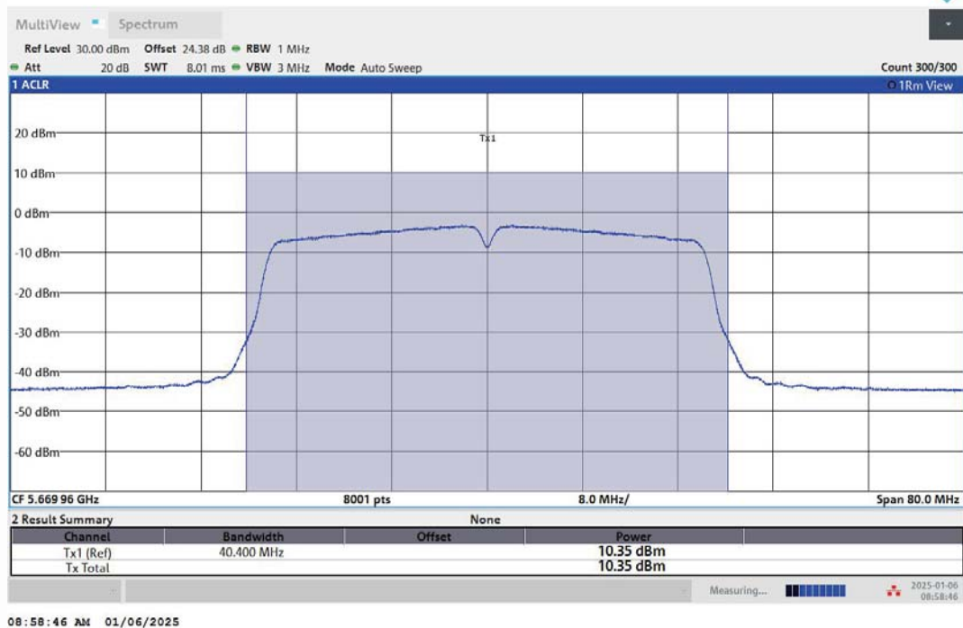
11AC40MIMO-Ant2-5670-PASS
