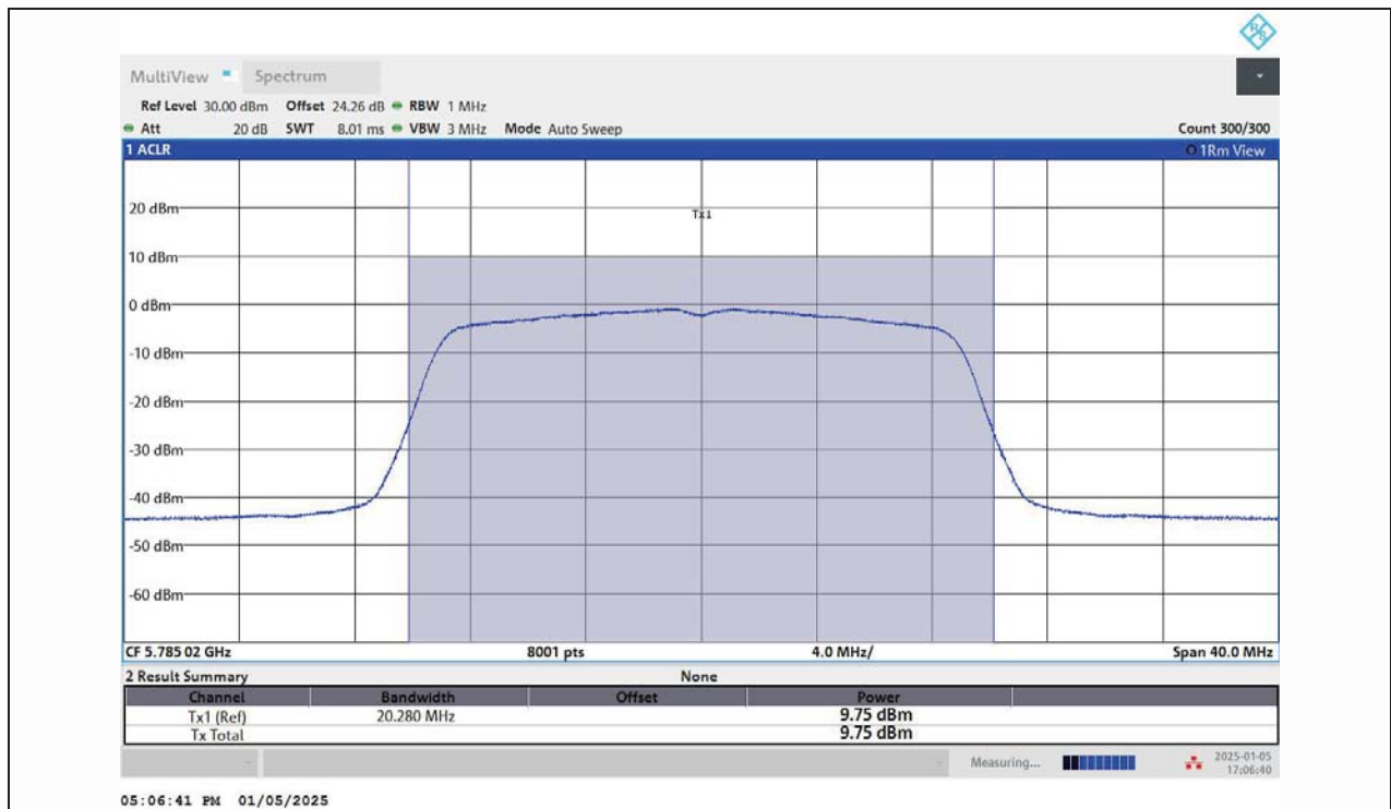
11AC20MIMO-Ant1-5785-PASS
