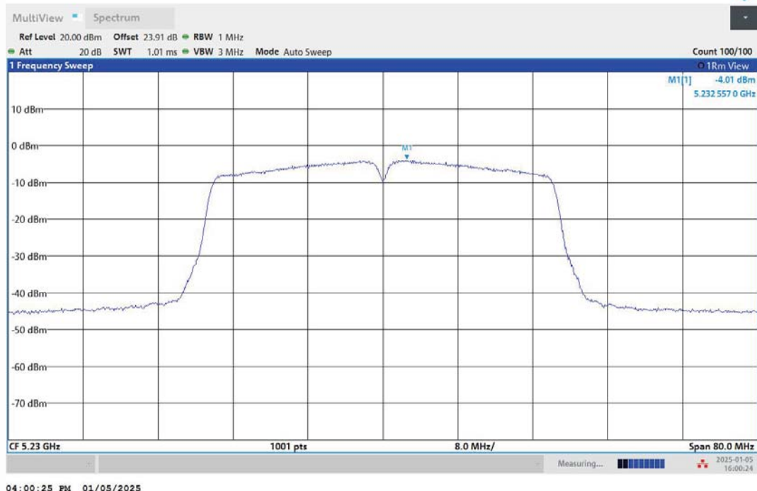
11N40MIMO-Ant2-5230-PASS
