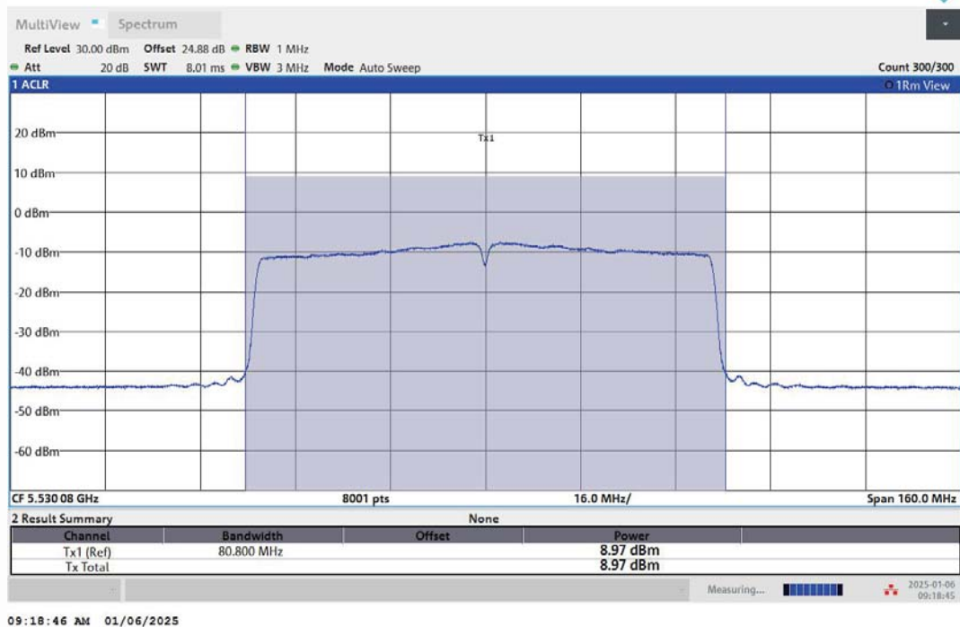
11AC80MIMO-Ant2-5530-PASS
