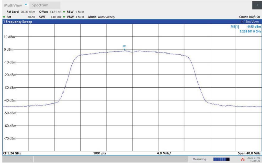
11N20MIMO-Ant1-5240-PASS
