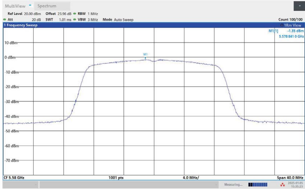
11N20MIMO-Ant1-5580-PASS
