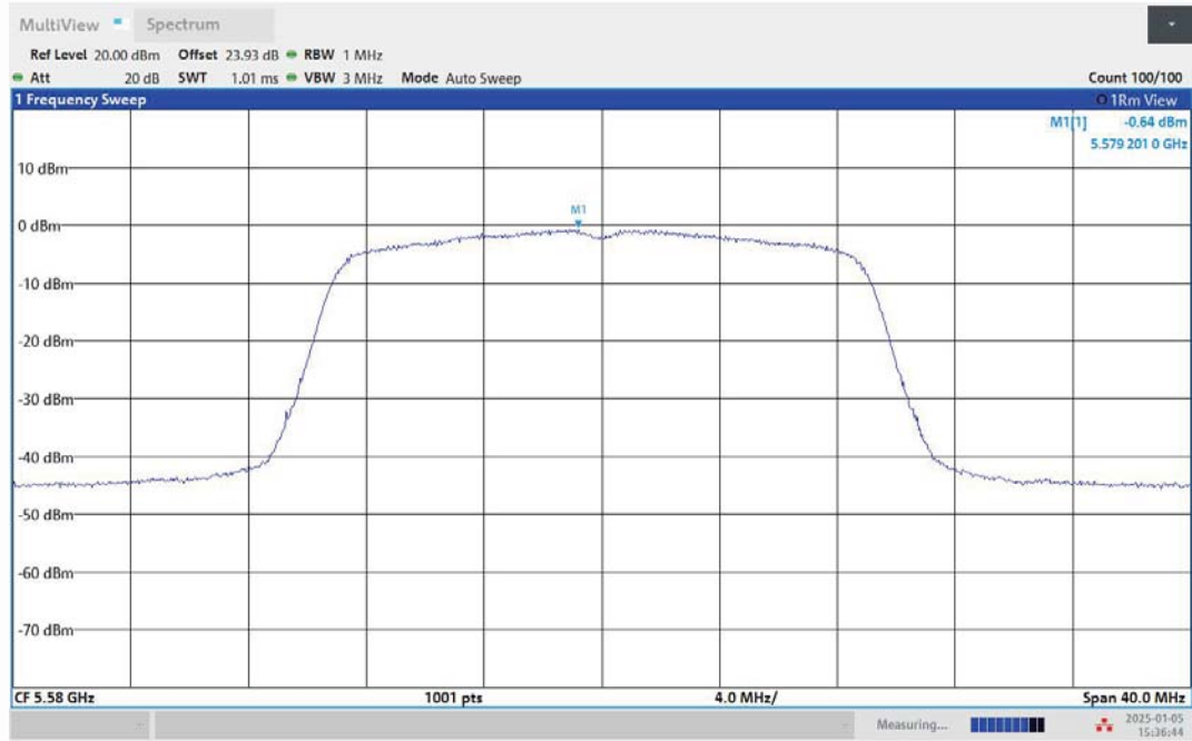
11N20MIMO-Ant2-5580-PASS
