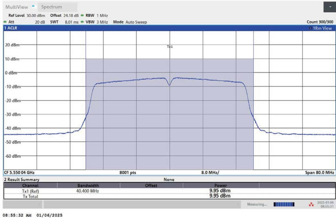
11AC40MIMO-Ant2-5550-PASS
