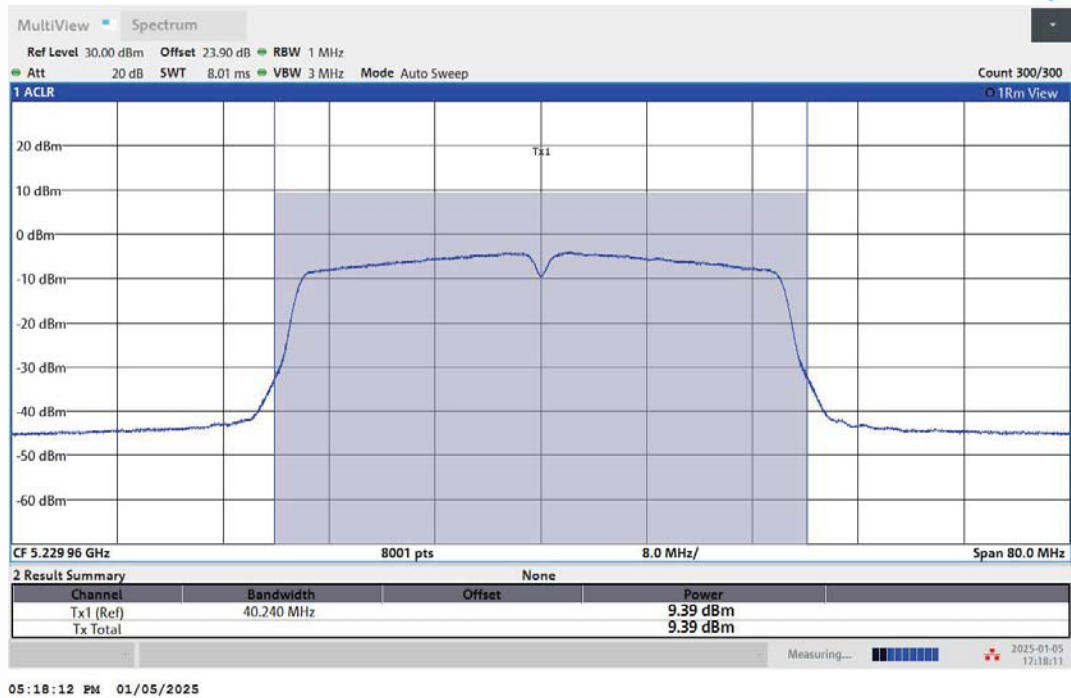
11AC40MIMO-Ant2-5230-PASS
