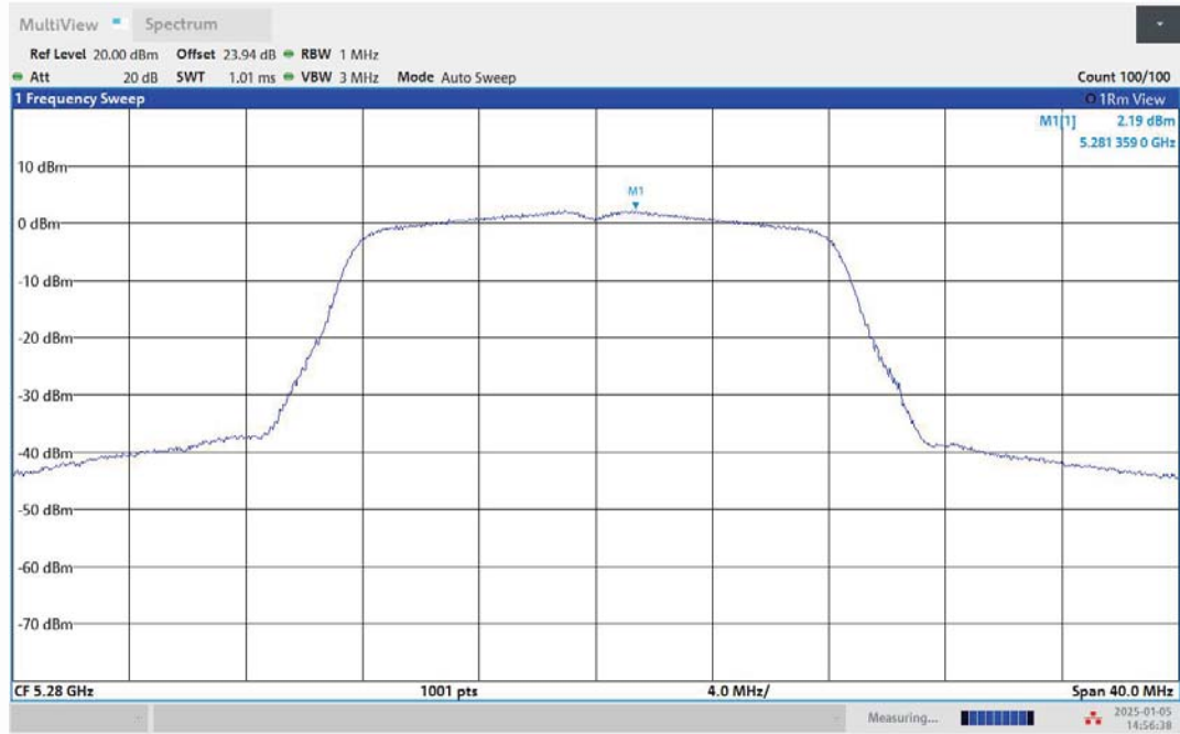
11A-Ant2-5280-PASS
