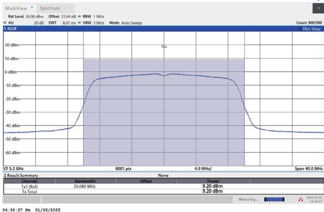
11AC20MIMO-Ant2-5200-PASS
