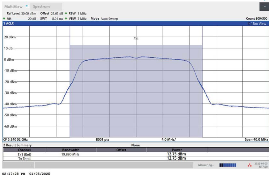
11A-Ant1-5240-PASS
