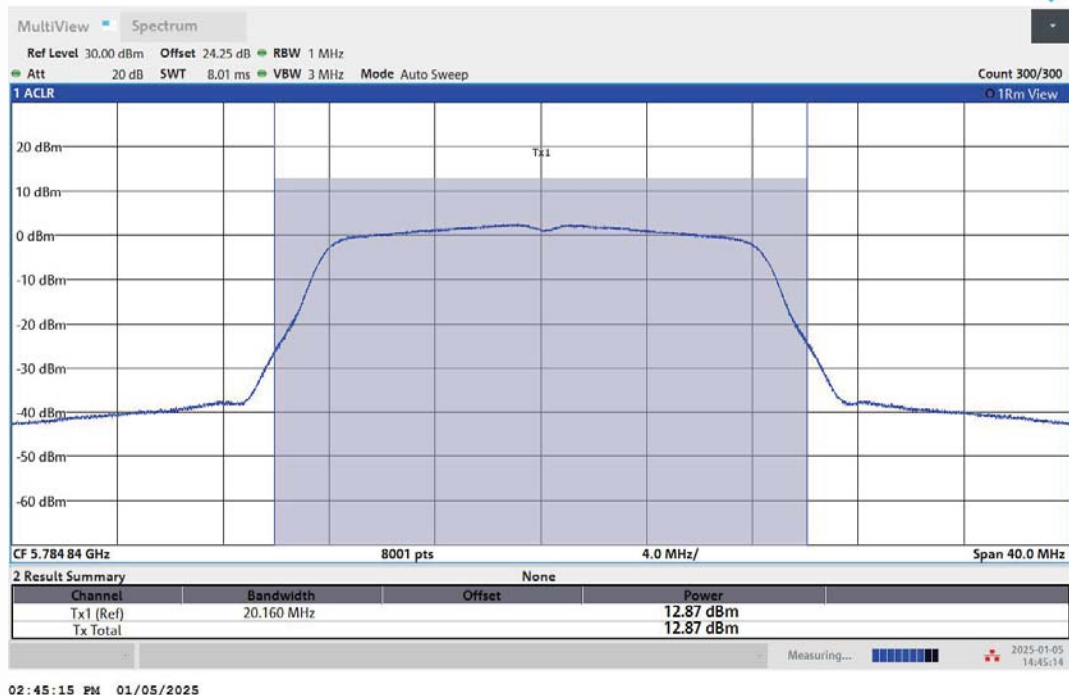
11A-Ant1-5785-PASS
