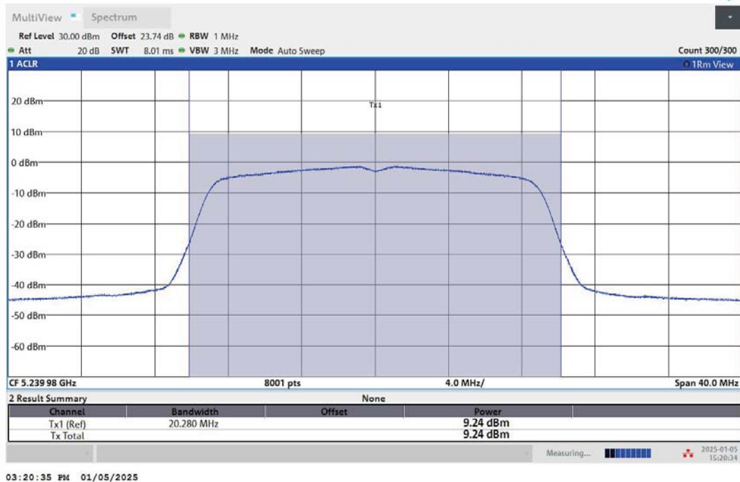
11N20MIMO-Ant2-5240-PASS
