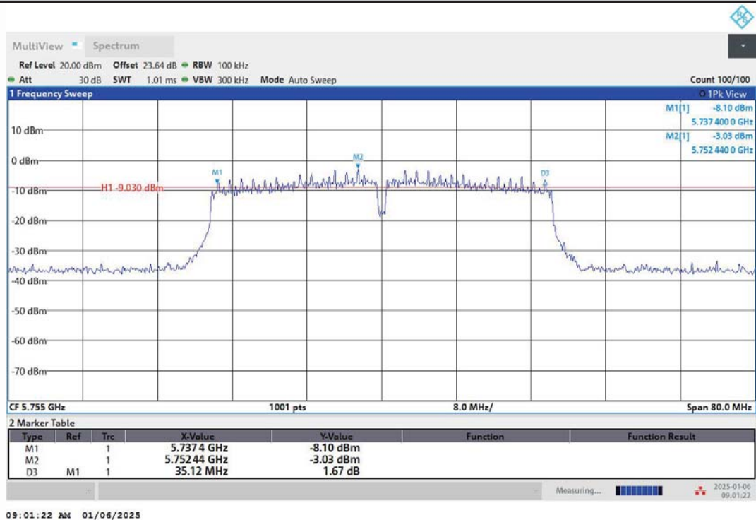
11AC40MIMO-Ant2-5755-PASS
