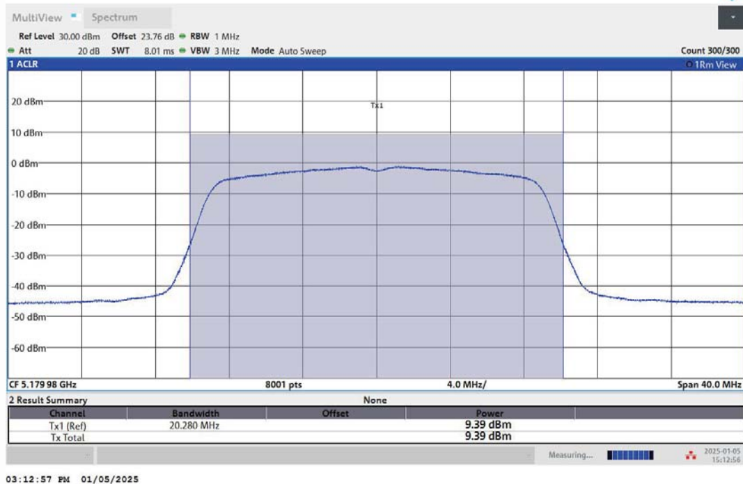
11N20MIMO-Ant2-5180-PASS
