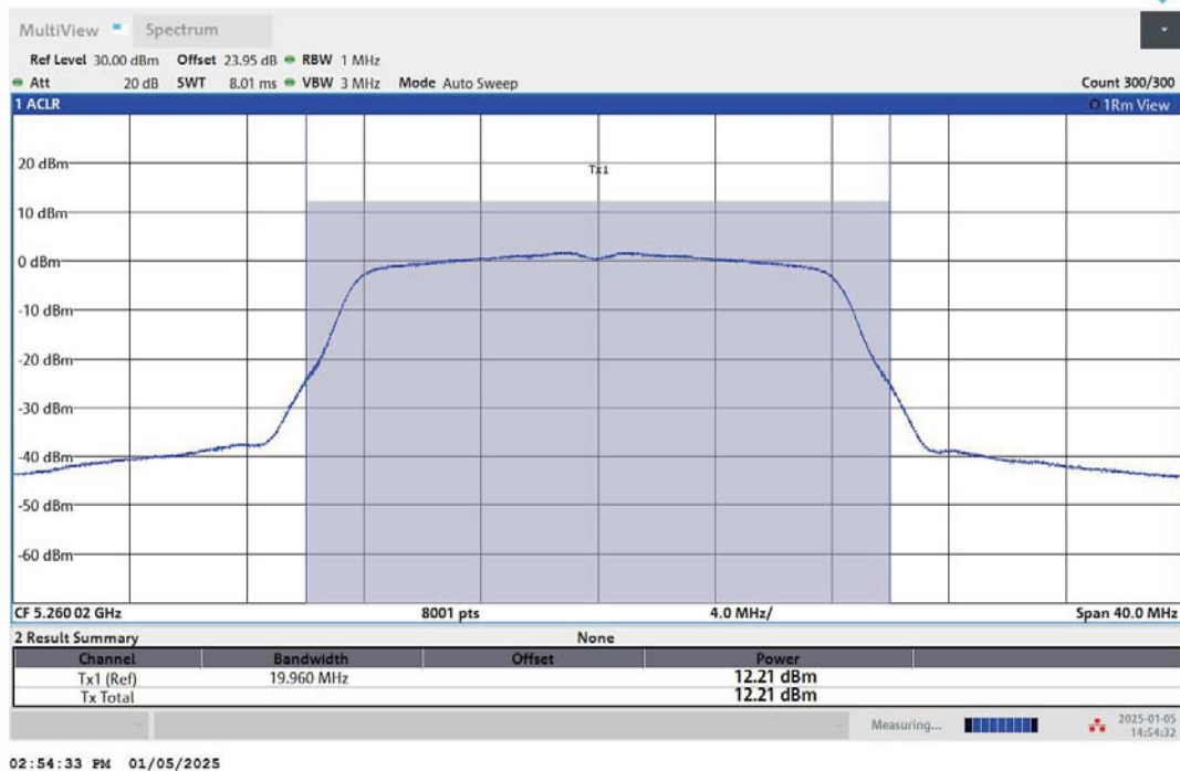
11A-Ant2-5260-PASS
