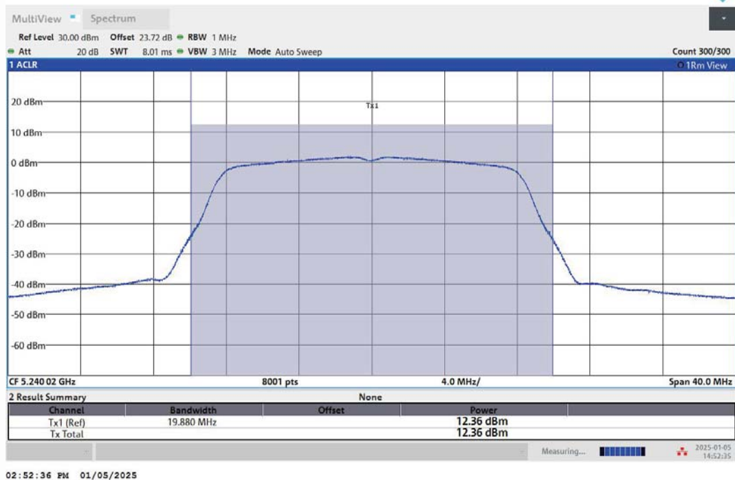
11A-Ant2-5240-PASS
