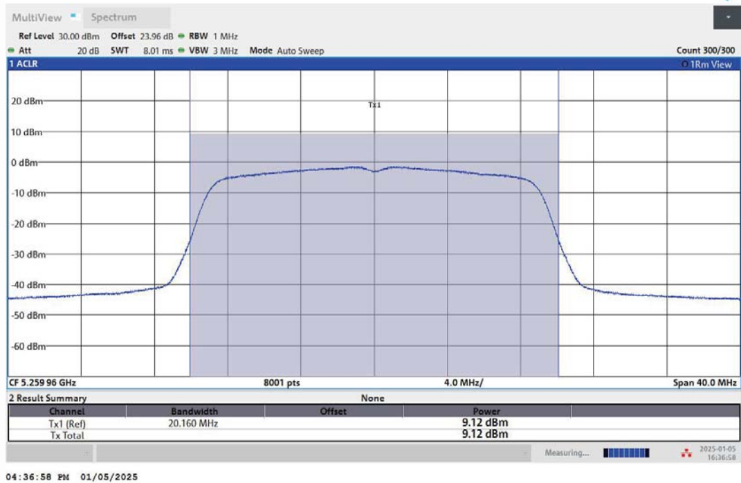
11AC20MIMO-Ant2-5260-PASS
