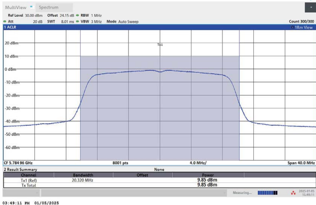
11N20MIMO-Ant2-5785-PASS
