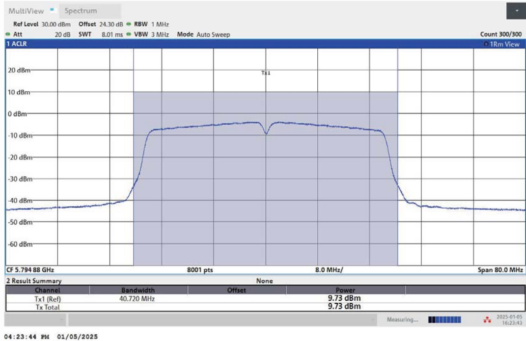
11N40MIMO-Ant2-5795-PASS
