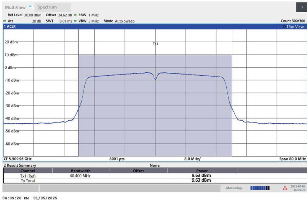
11N40MIMO-Ant2-5510-PASS
