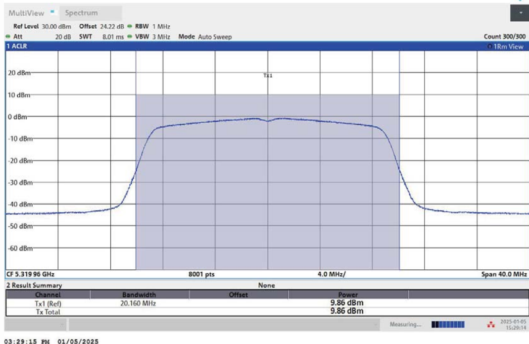
11N20MIMO-Ant1-5320-PASS
