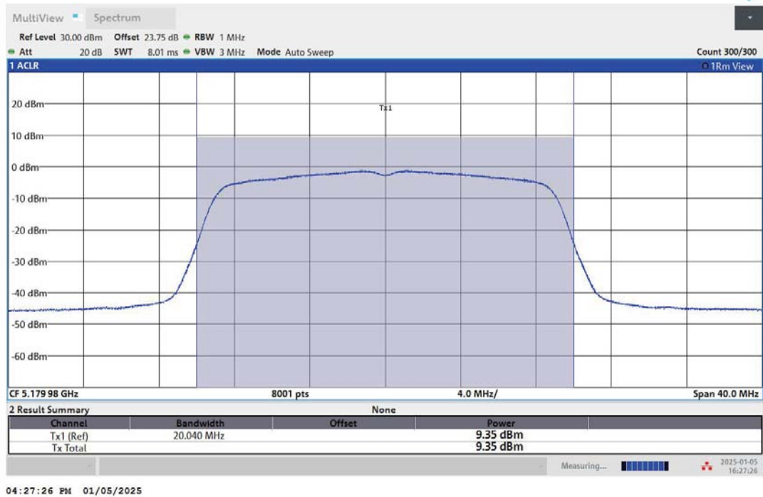
11AC20MIMO-Ant2-5180-PASS
