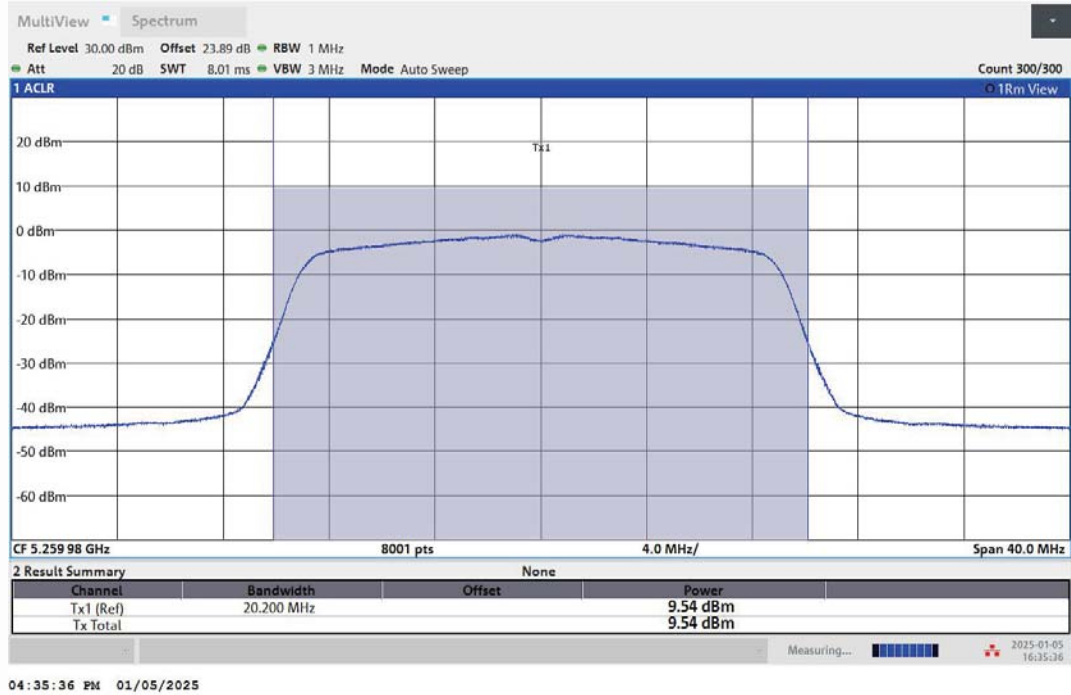
11AC20MIMO-Ant1-5260-PASS
