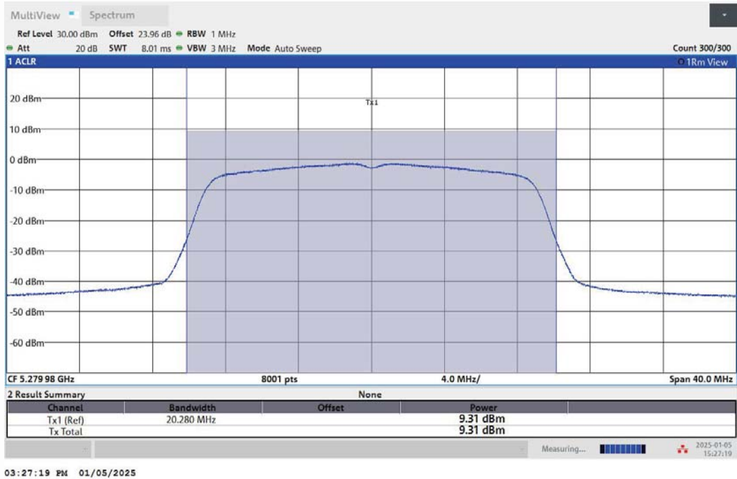
11N20MIMO-Ant2-5280-PASS
