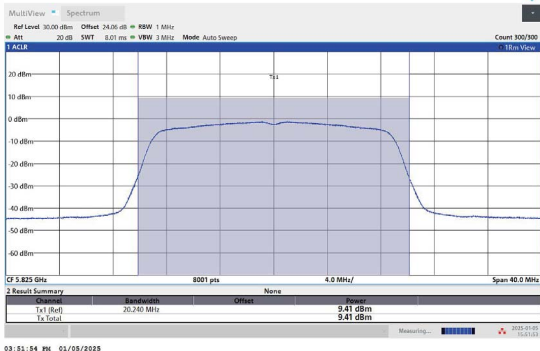
11N20MIMO-Ant1-5825-PASS
