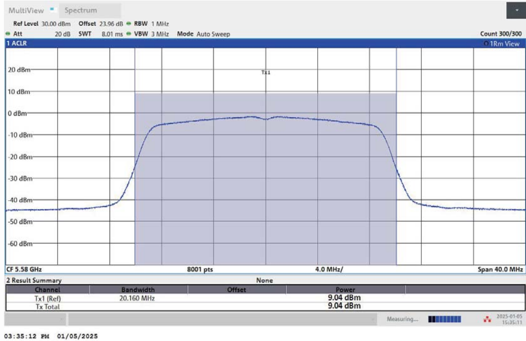
11N20MIMO-Ant1-5580-PASS
