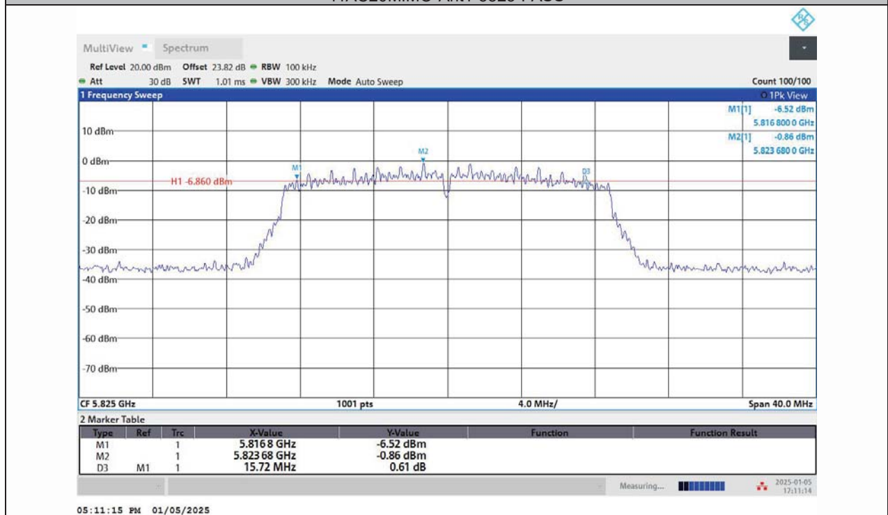
11AC20MIMO-Ant2-5825-PASS
