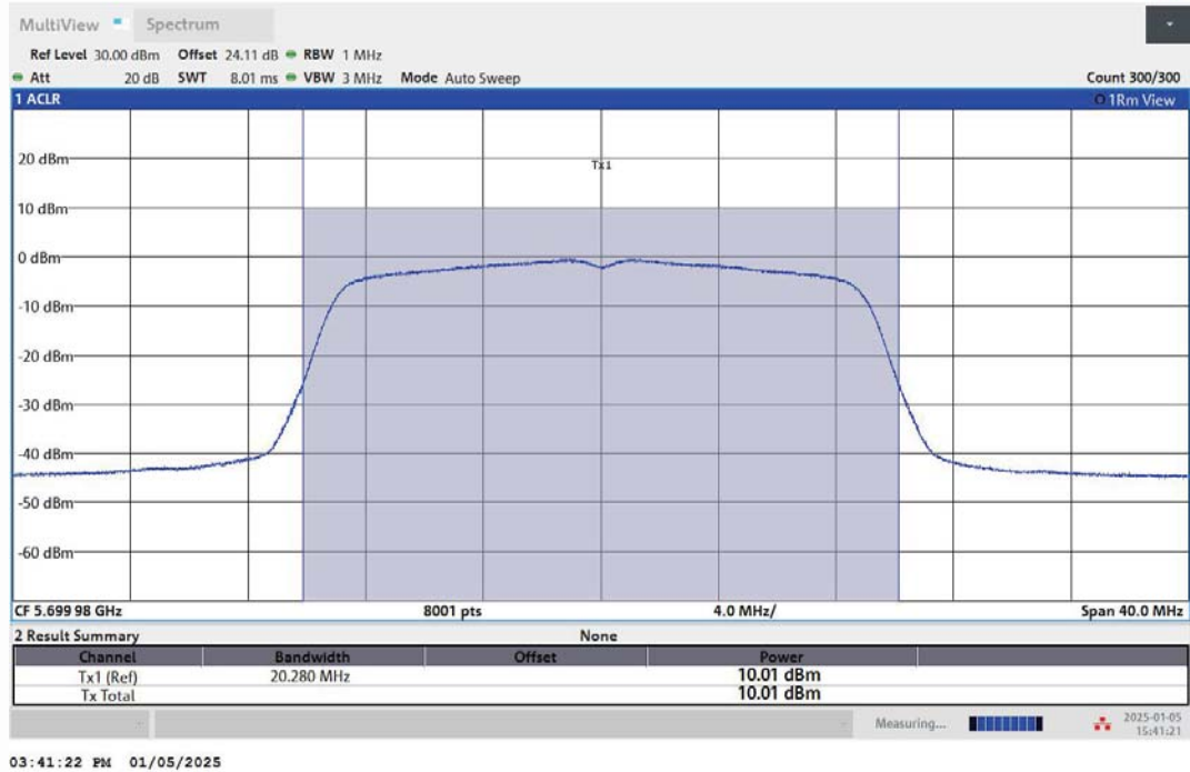
11N20MIMO-Ant2-5700-PASS
