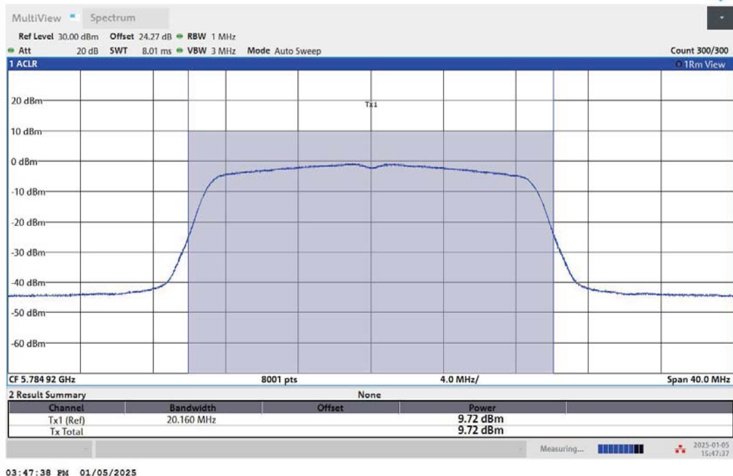
11N20MIMO-Ant1-5785-PASS
