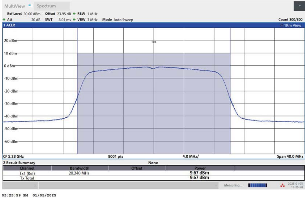
11N20MIMO-Ant1-5280-PASS
