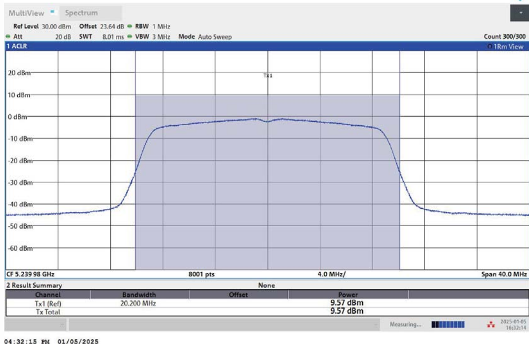
11AC20MIMO-Ant1-5240-PASS
