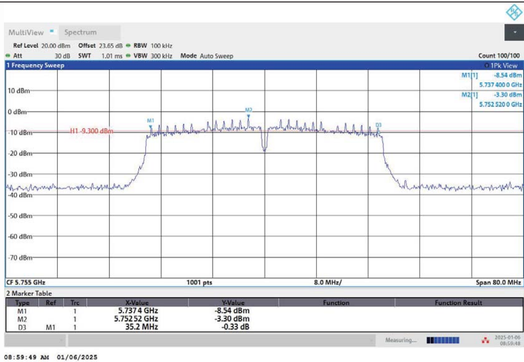
11AC40MIMO-Ant1-5755-PASS
