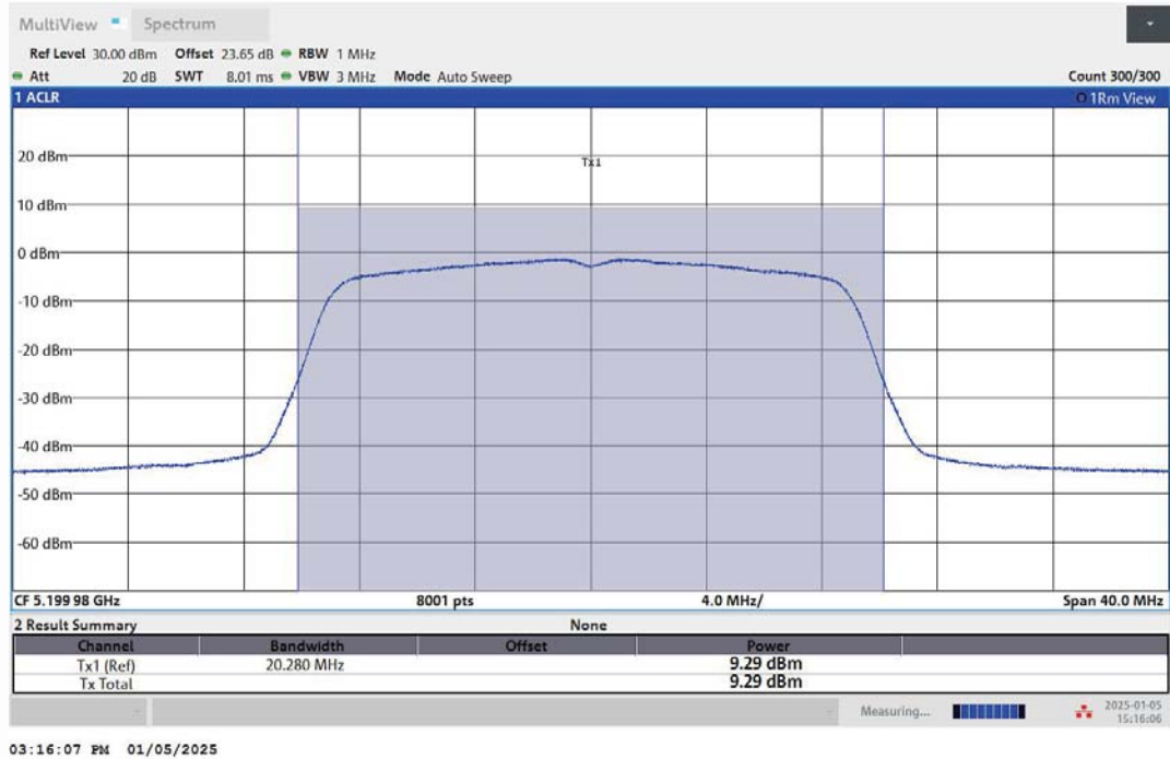
11N20MIMO-Ant2-5200-PASS
