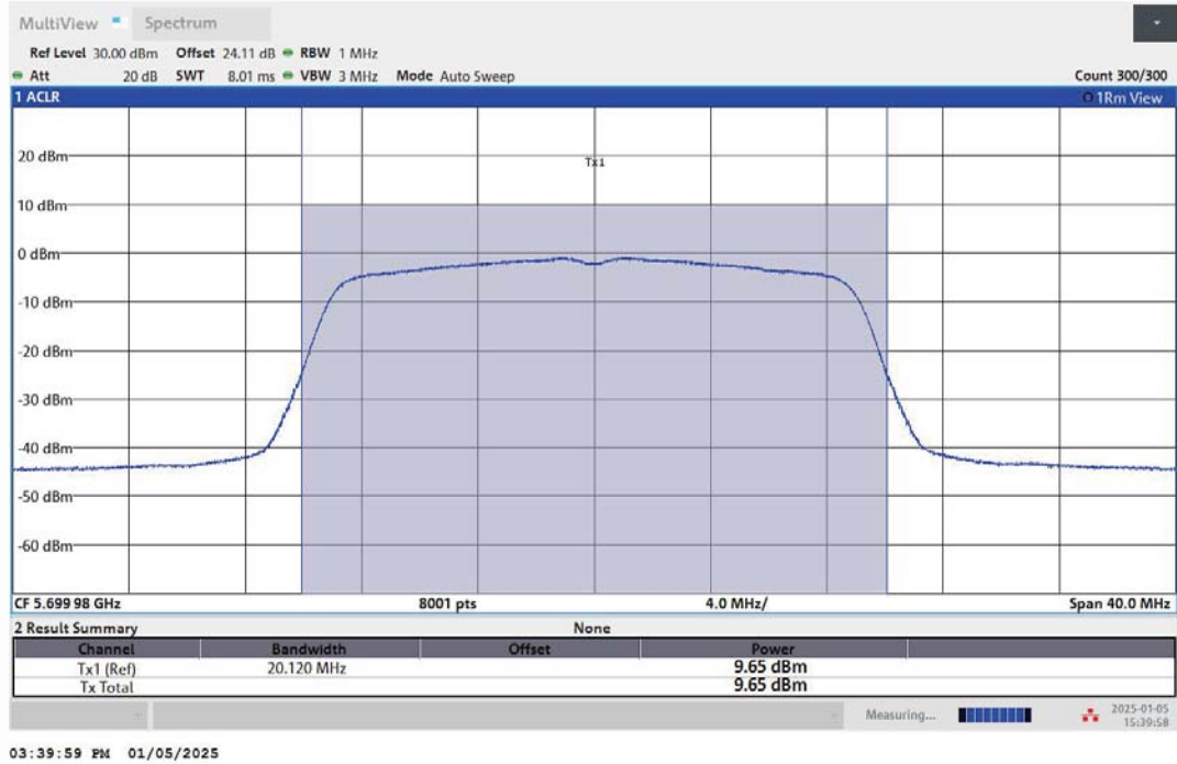
11N20MIMO-Ant1-5700-PASS
