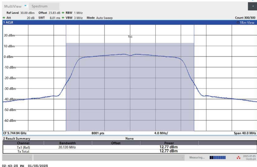
11A-Ant1-5745-PASS
