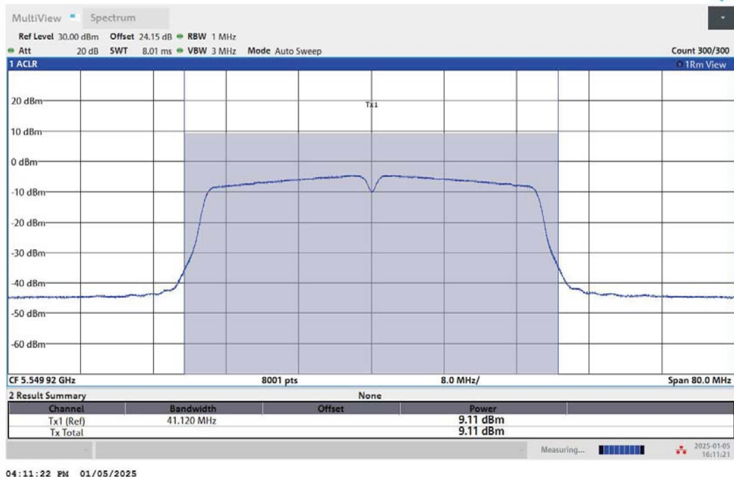
11N40MIMO-Ant1-5550-PASS
