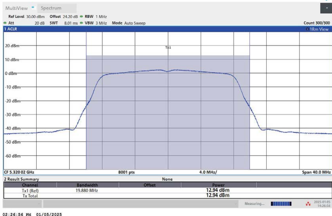
11A-Ant1-5320-PASS
