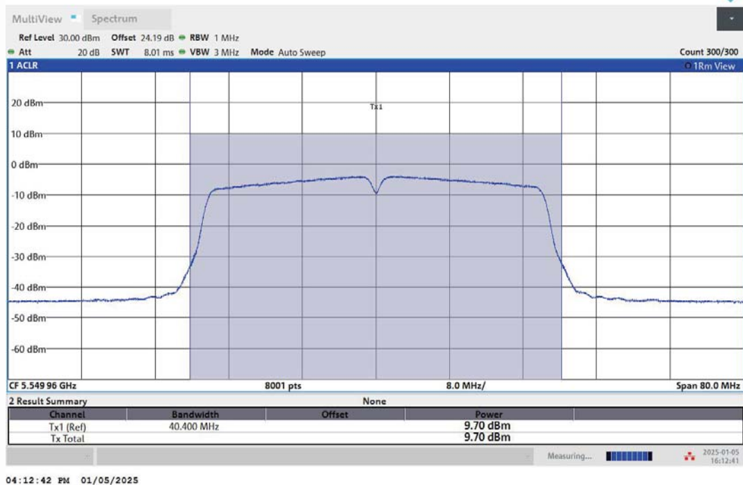
11N40MIMO-Ant2-5550-PASS
