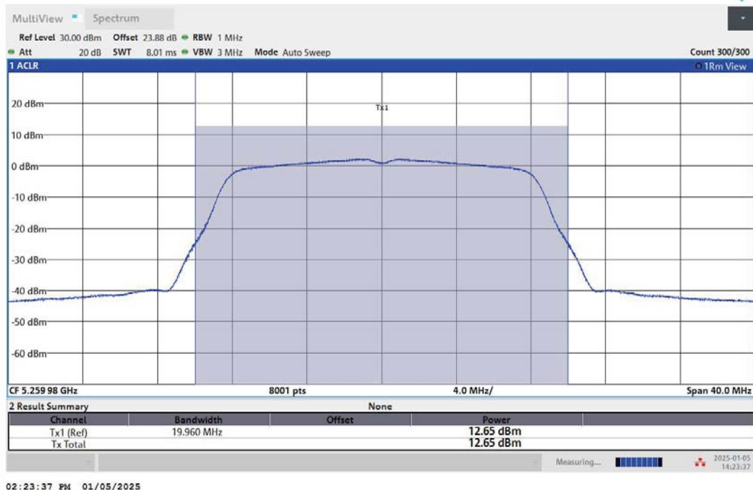
11A-Ant1-5260-PASS
