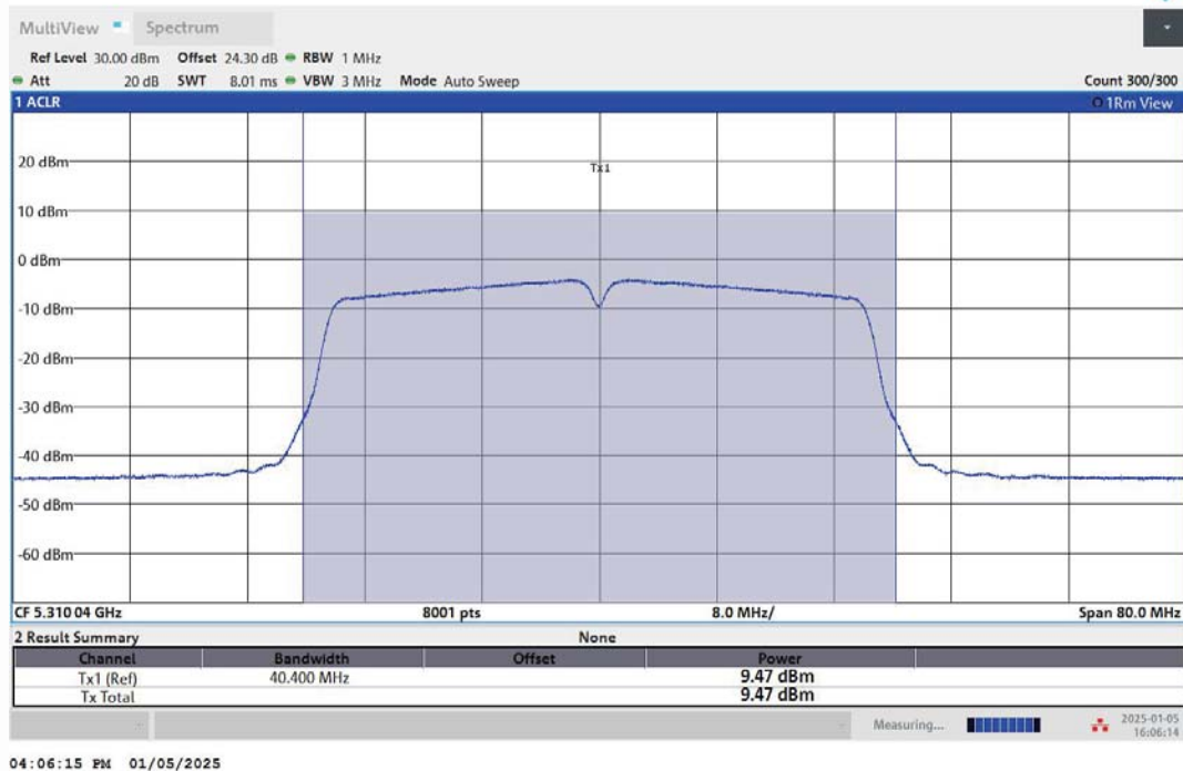
11N40MIMO-Ant2-5310-PASS
