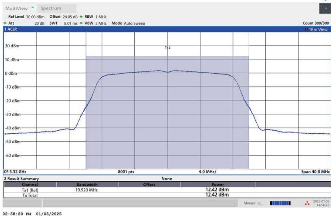
11A-Ant2-5320-PASS
