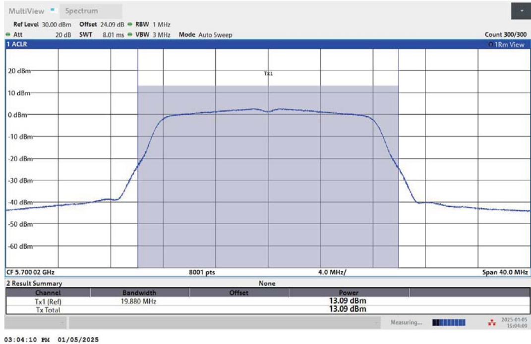
11A-Ant2-5700-PASS
