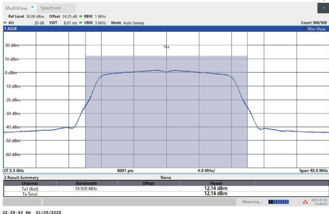
11A-Ant1-5500-PASS
