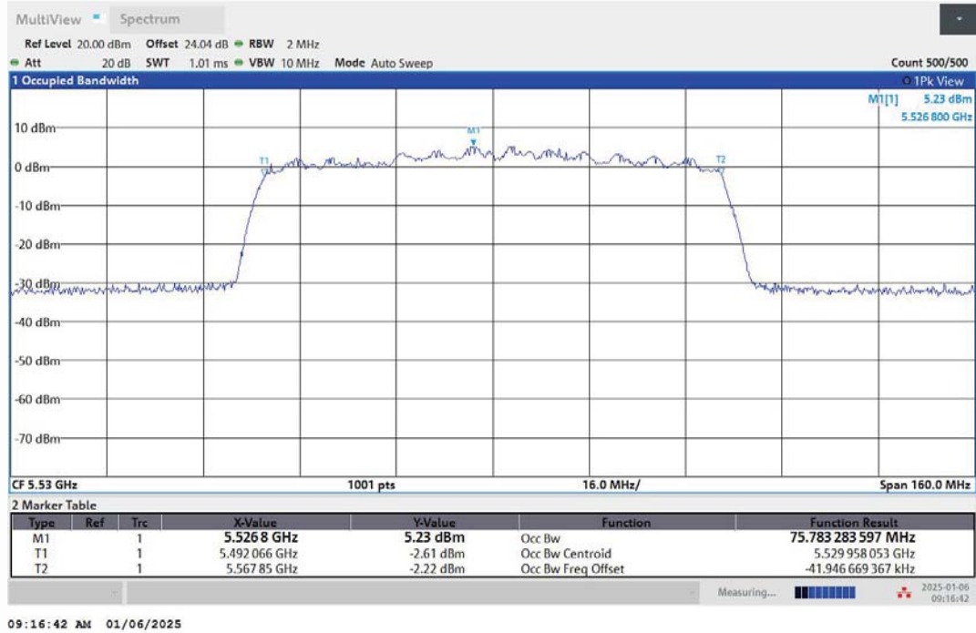
11AC80MIMO-Ant1-5530
