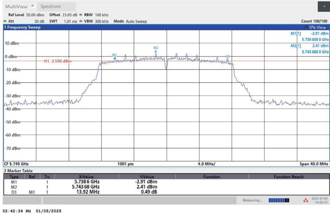
11A-Ant1-5745-PASS
