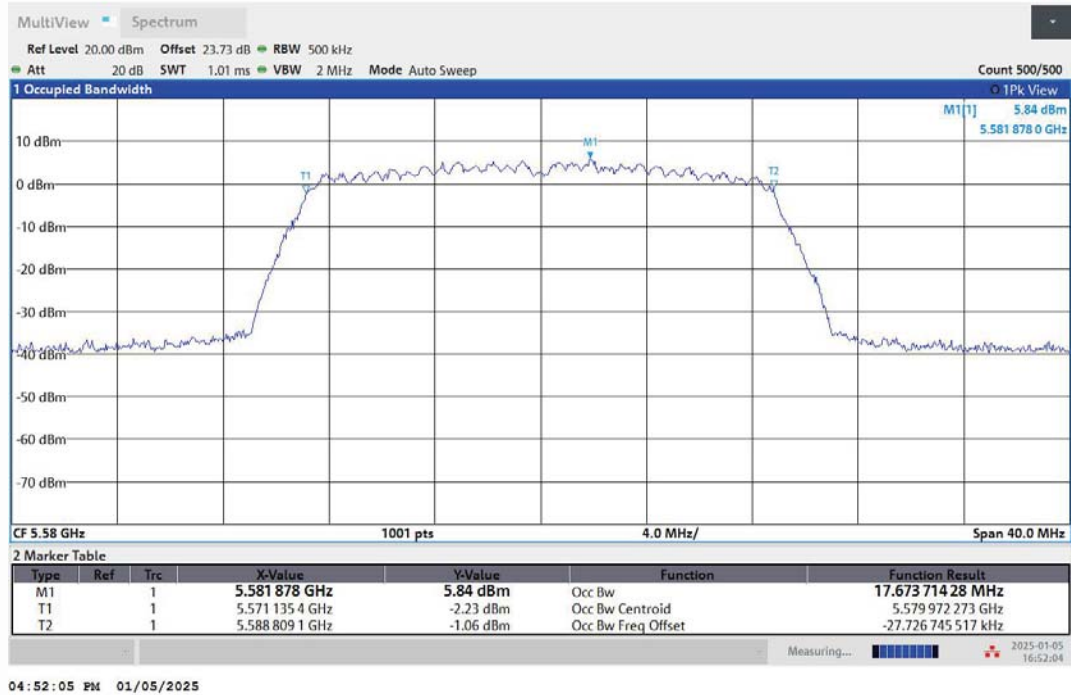
11AC20MIMO-Ant2-5580
