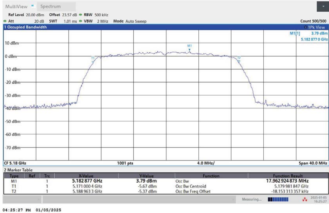
11AC20MIMO-Ant1-5180
