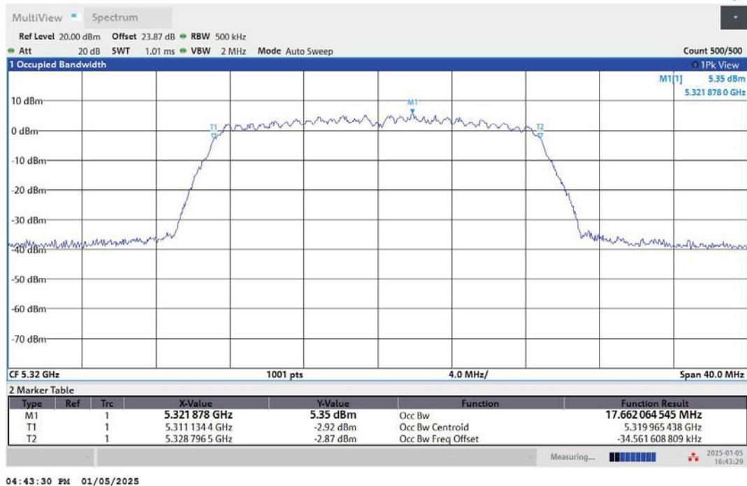
11AC20MIMO-Ant2-5320
