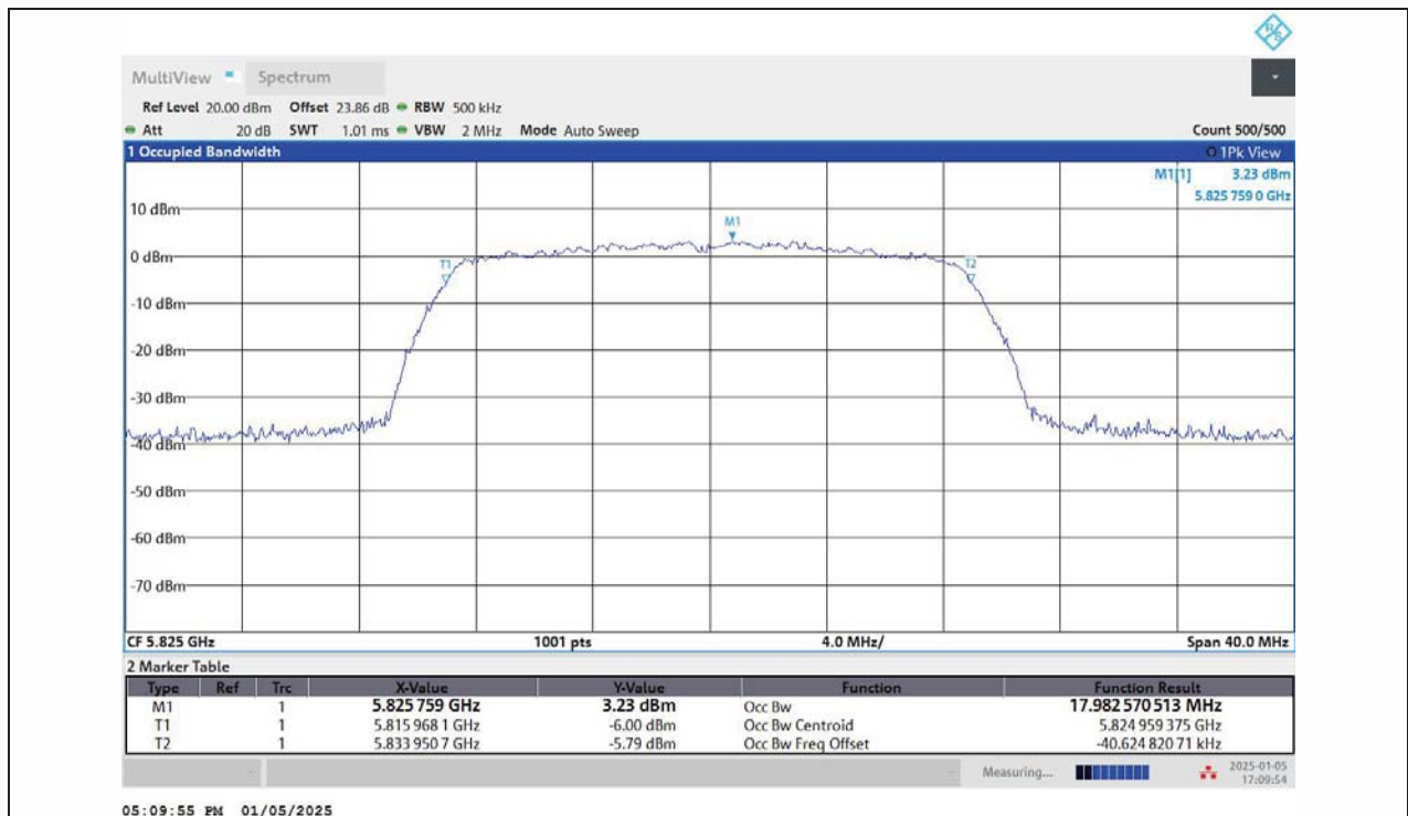
11AC20MIMO-Ant1-5825
