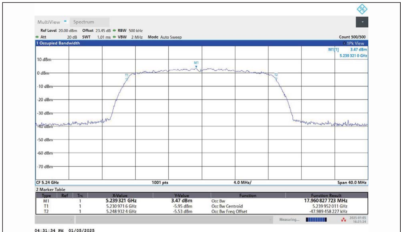
11AC20MIMO-Ant1-5240
