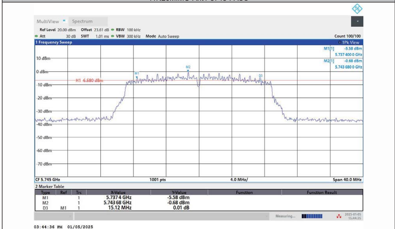
11N20MIMO-Ant2-5745-PASS
