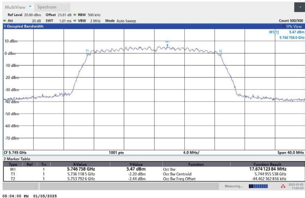
11AC20MIMO-Ant2-5745
