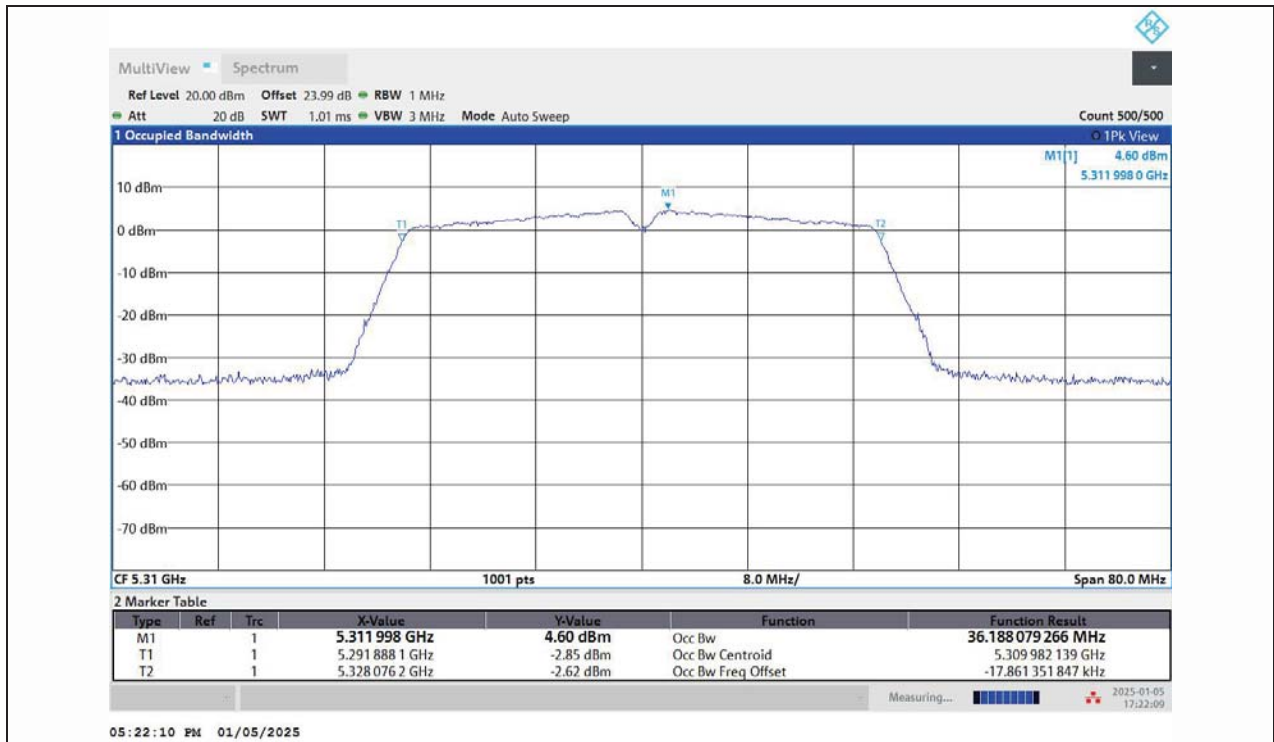
11AC40MIMO-Ant1-5310
