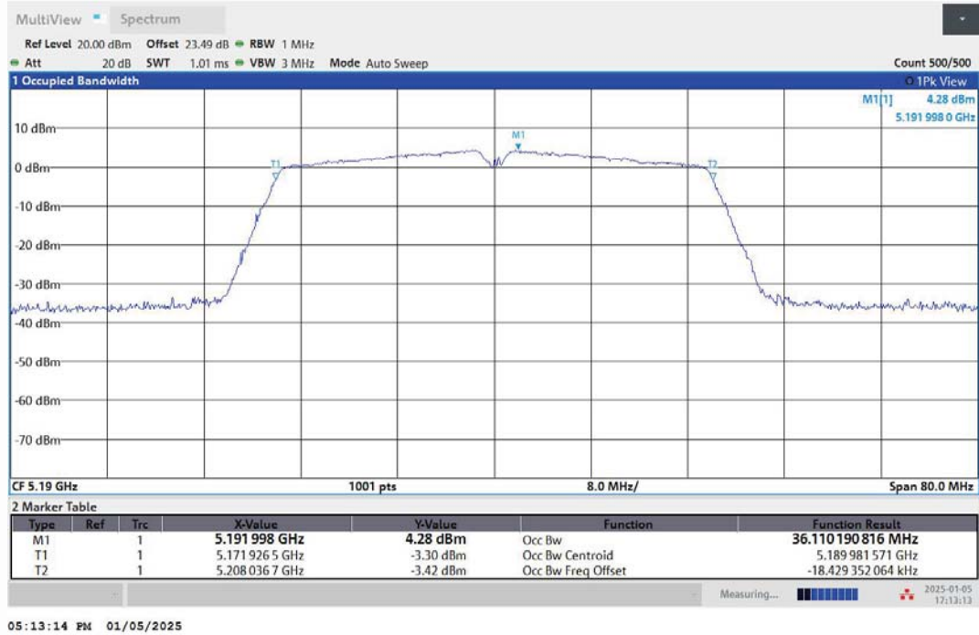
11AC40MIMO-Ant1-5190
