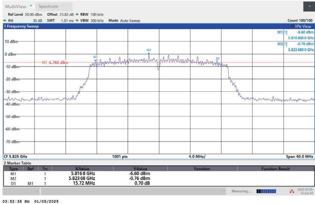
11N20MIMO-Ant2-5825-PASS
