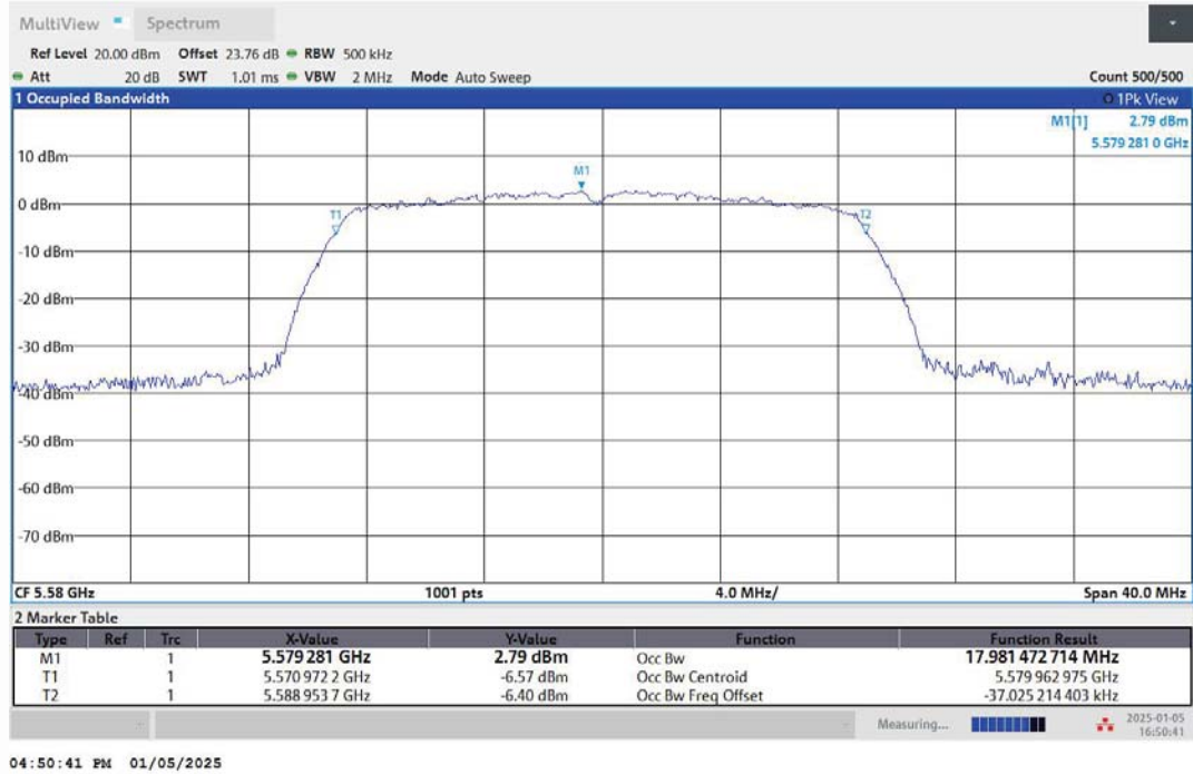
11AC20MIMO-Ant1-5580
