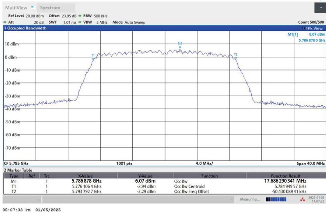
11AC20MIMO-Ant2-5785
