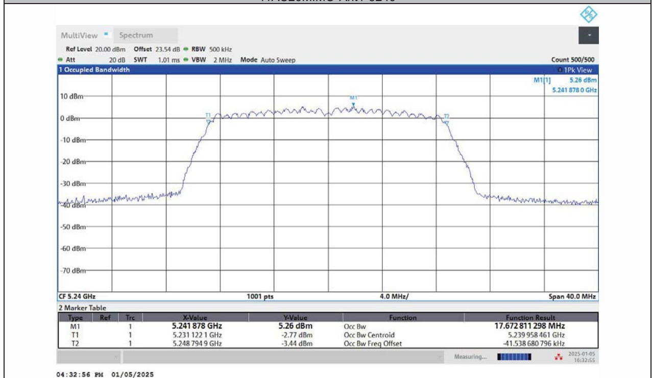
11AC20MIMO-Ant2-5240
