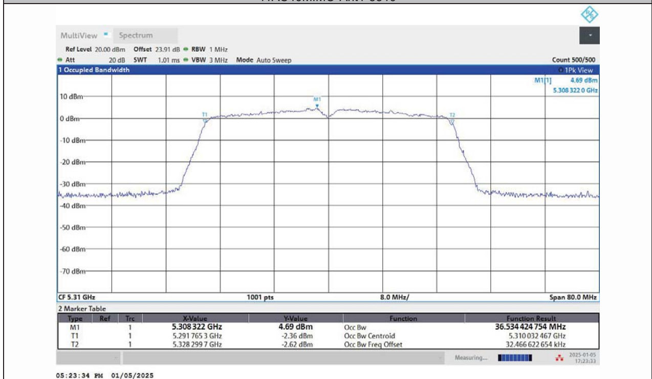
11AC40MIMO-Ant2-5310
