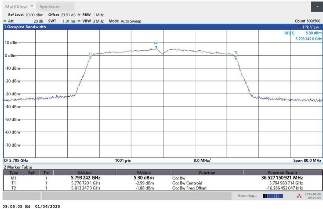
11AC40MIMO-Ant2-5795
