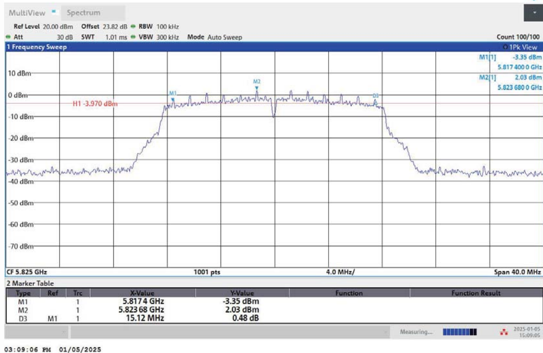
11A-Ant2-5825-PASS
