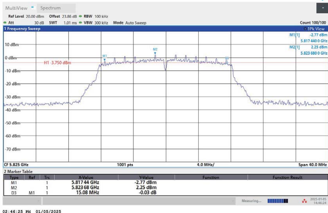
11A-Ant1-5825-PASS
