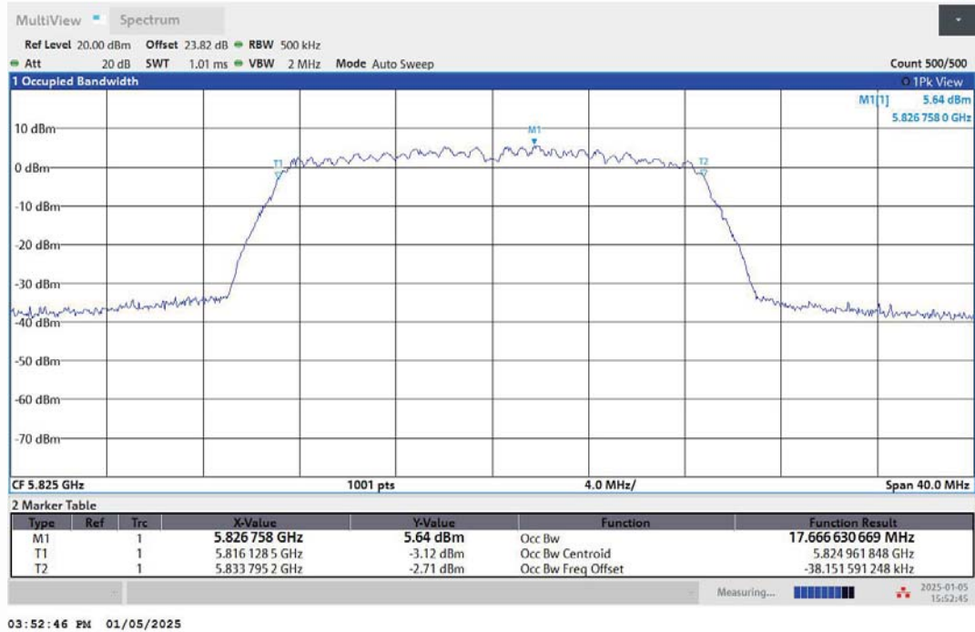
11N20MIMO-Ant2-5825
