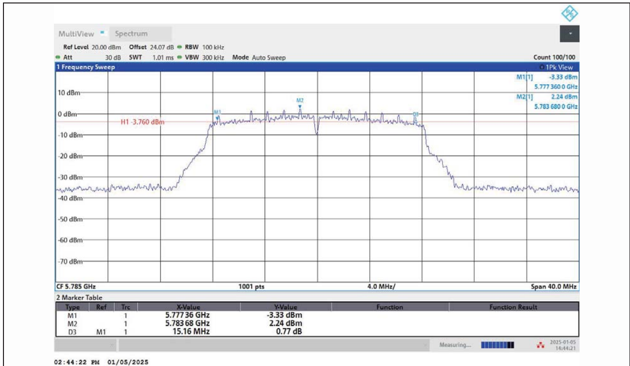
11A-Ant1-5785-PASS
