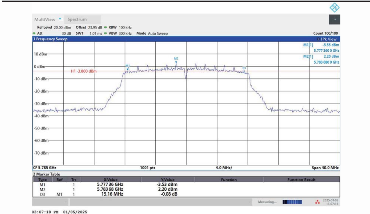
11A-Ant2-5785-PASS
