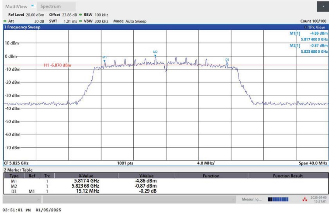
11N20MIMO-Ant1-5825-PASS
