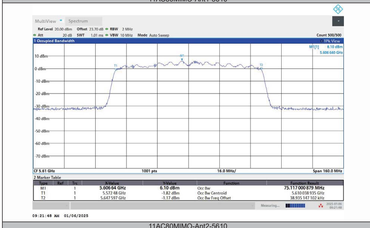
11AC80MIMO-Ant2-5610
