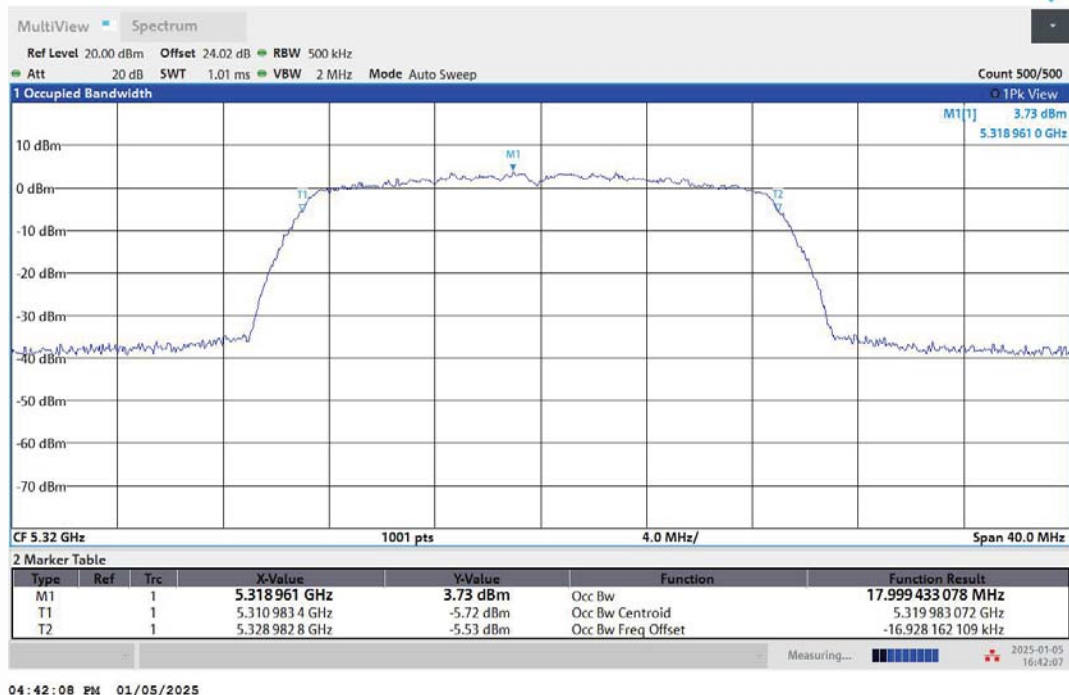
11AC20MIMO-Ant1-5320
