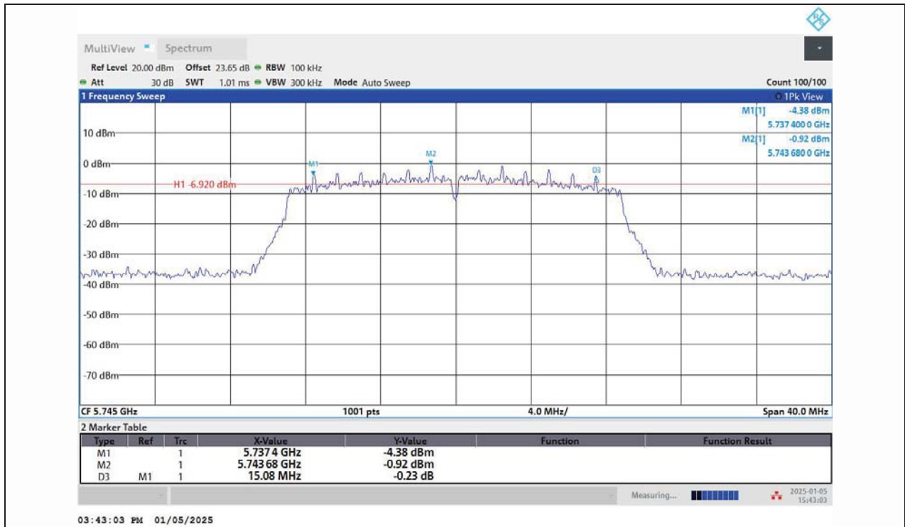
11N20MIMO-Ant1-5745-PASS
