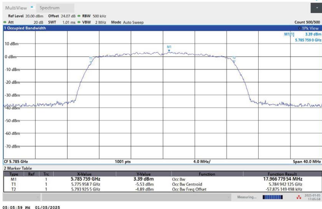
11AC20MIMO-Ant1-5785
