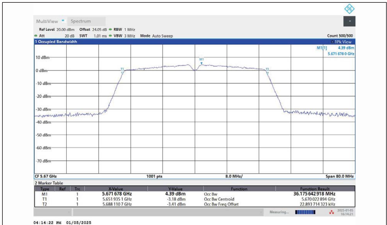
11N40MIMO-Ant1-5670
