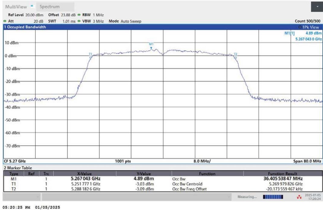
11AC40MIMO-Ant2-5270
