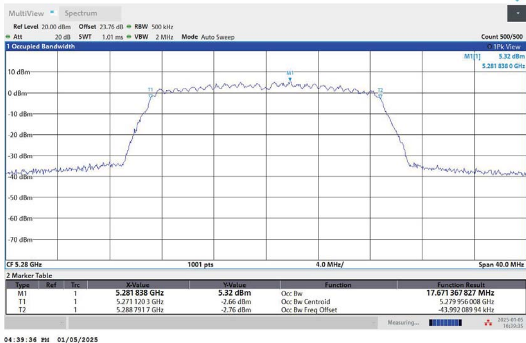
11AC20MIMO-Ant2-5280
