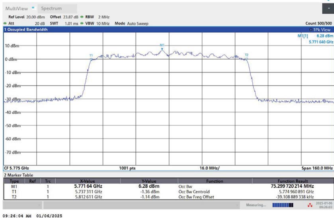
11AC80MIMO-Ant2-5775
