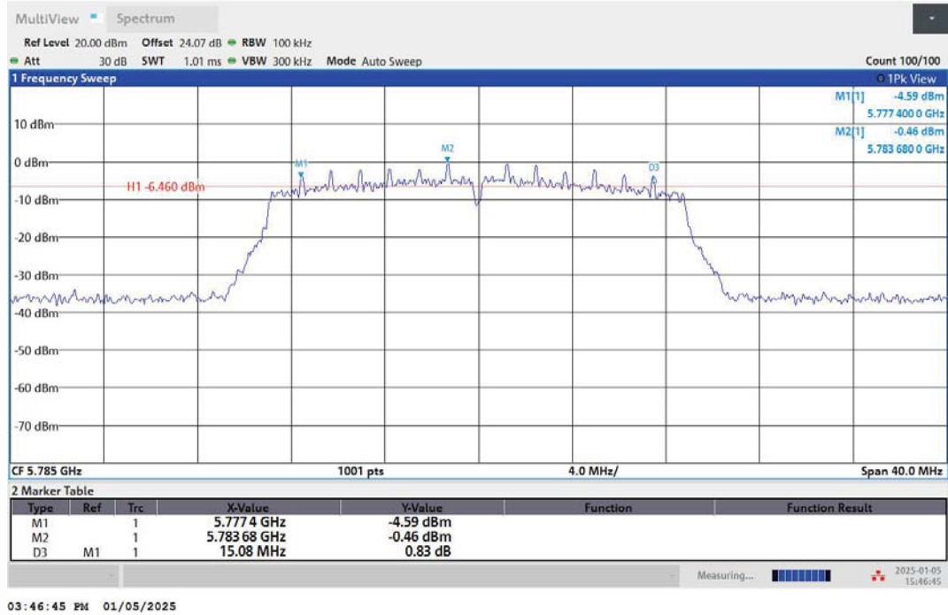
11N20MIMO-Ant1-5785-PASS
