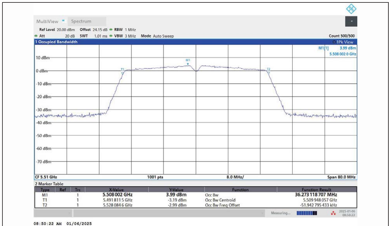
11AC40MIMO-Ant1-5510
