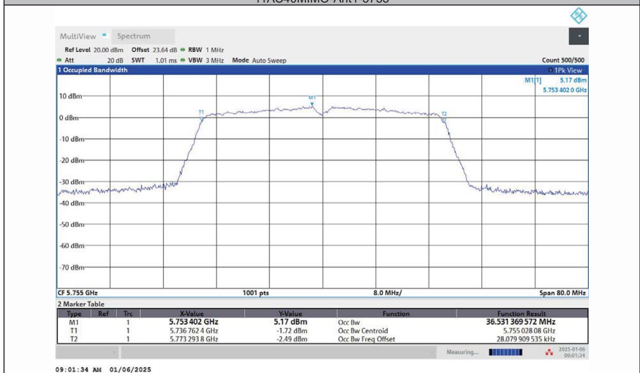
11AC40MIMO-Ant2-5755
