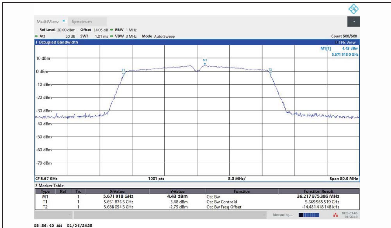
11AC40MIMO-Ant1-5670
