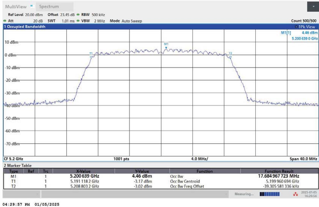
11AC20MIMO-Ant2-5200
