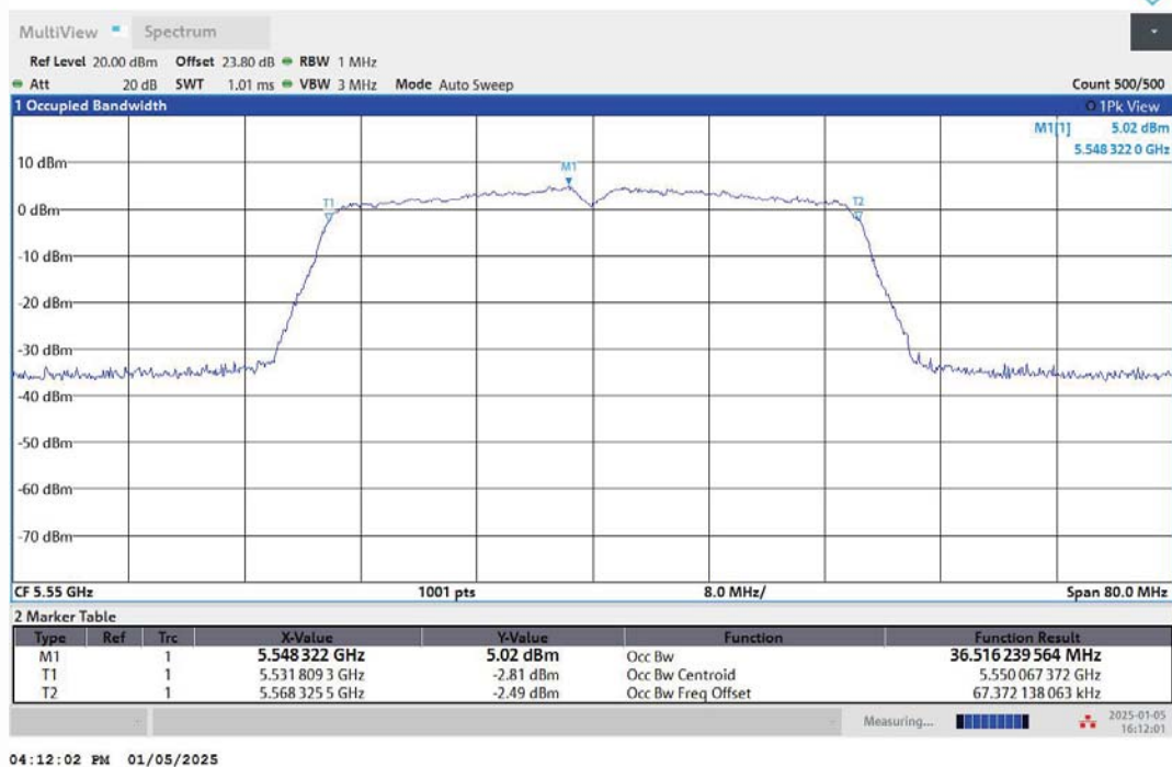
11N40MIMO-Ant2-5550
