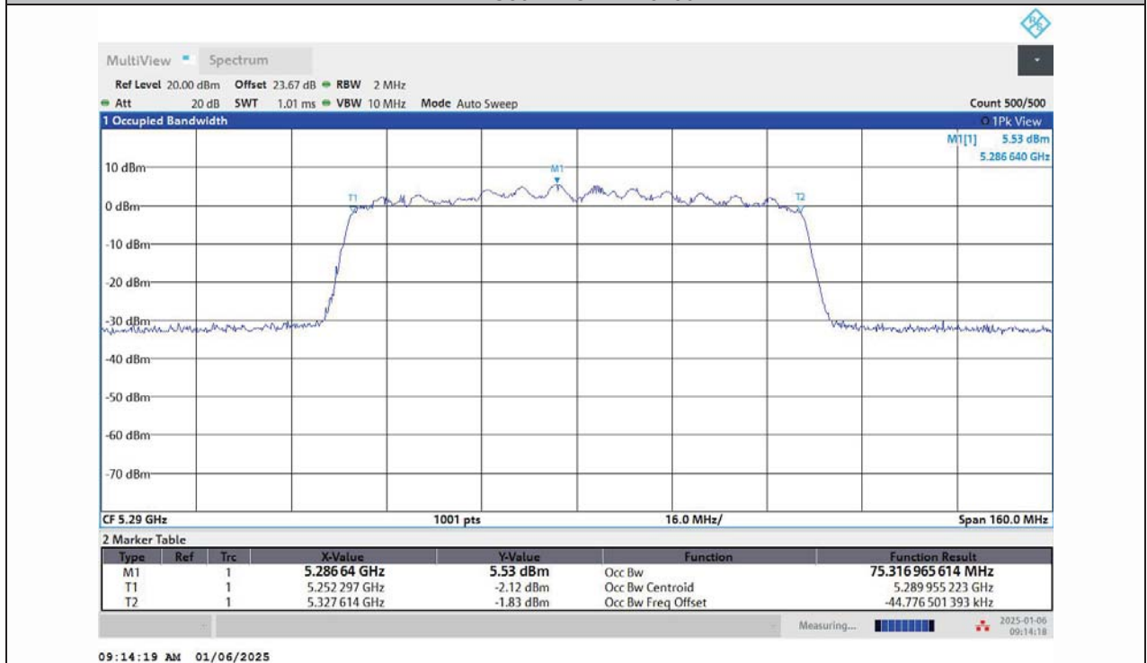
11AC80MIMO-Ant2-5290
