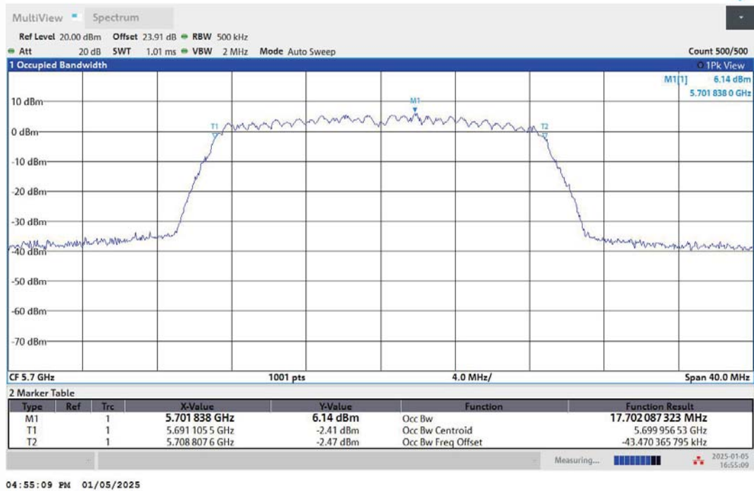
11AC20MIMO-Ant2-5700
