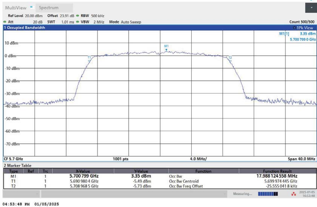
11AC20MIMO-Ant1-5700
