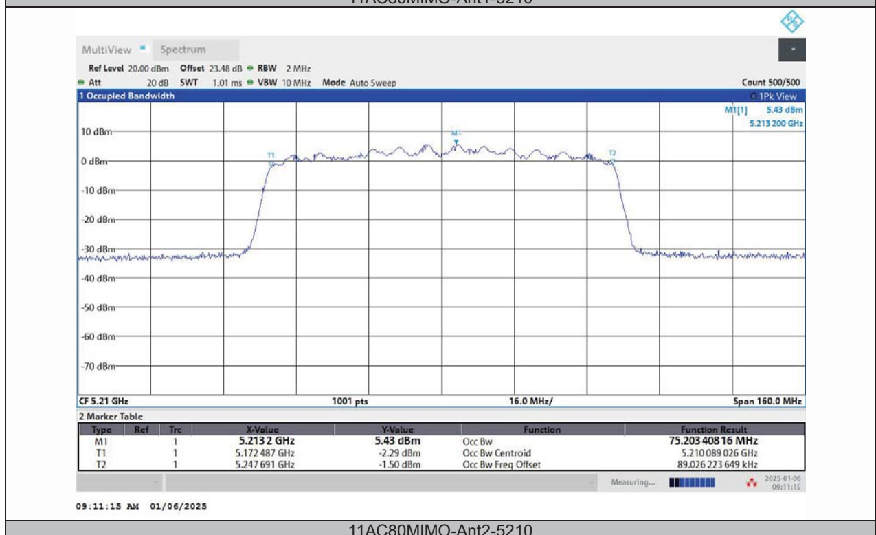
11AC80MIMO-Ant2-5210
