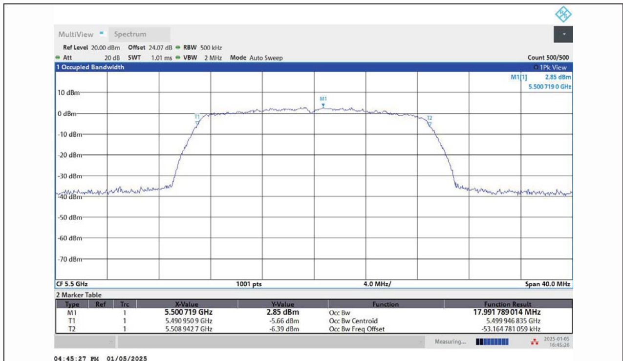
11AC20MIMO-Ant1-5500
