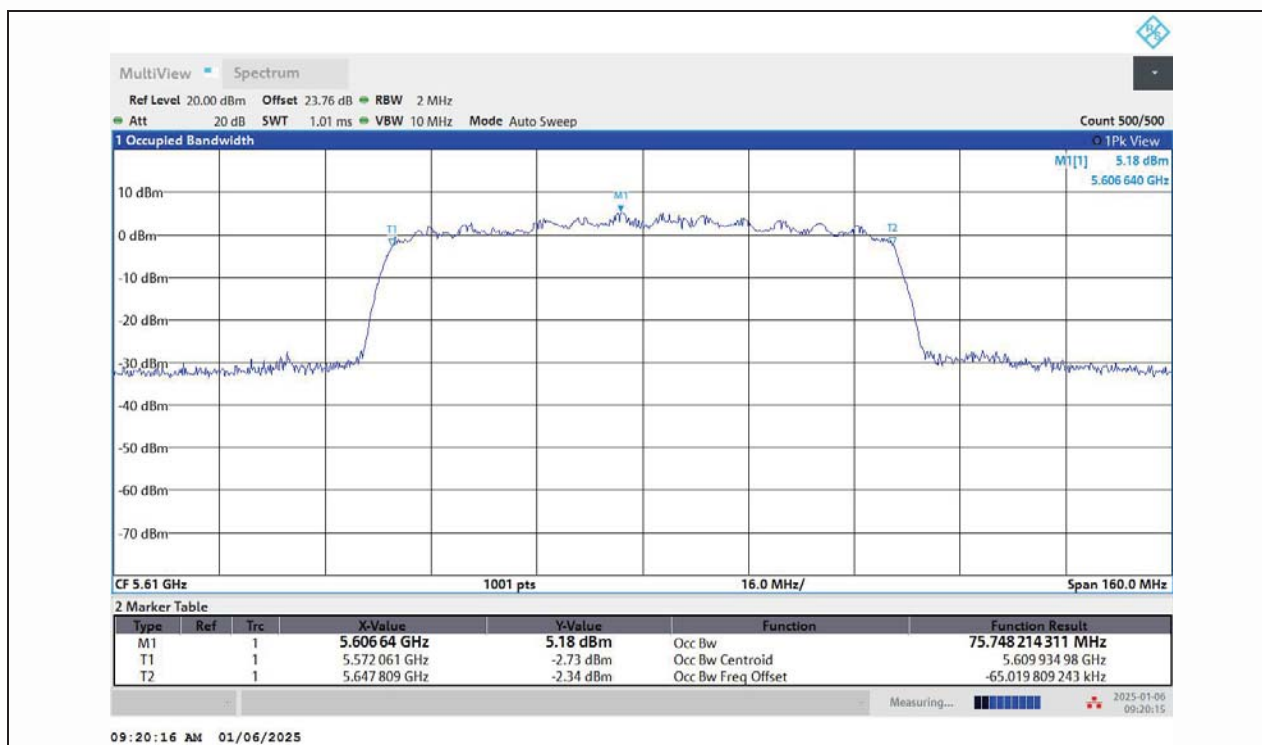
11AC80MIMO-Ant1-5610
