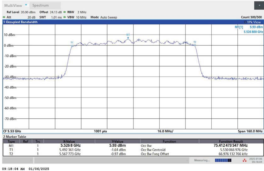
11AC80MIMO-Ant2-5530
