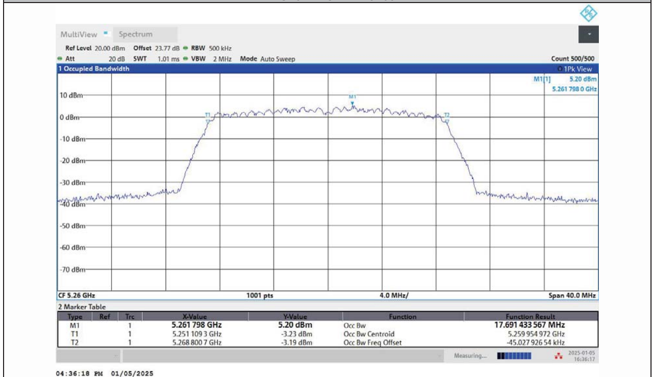
11AC20MIMO-Ant2-5260
