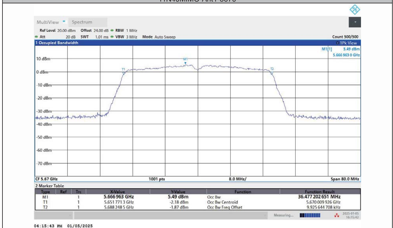
11N40MIMO-Ant2-5670
