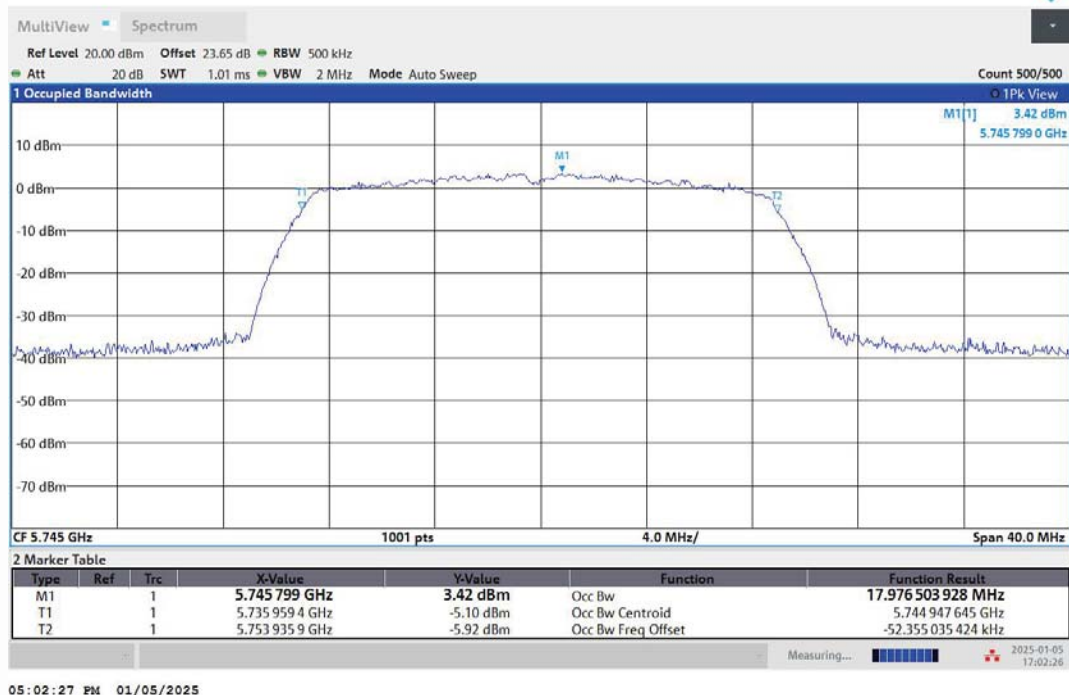
11AC20MIMO-Ant1-5745
