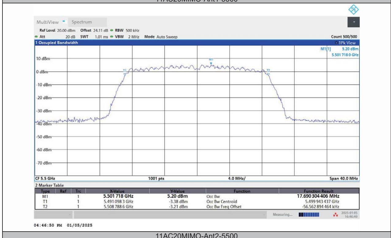
11AC20MIMO-Ant2-5500
