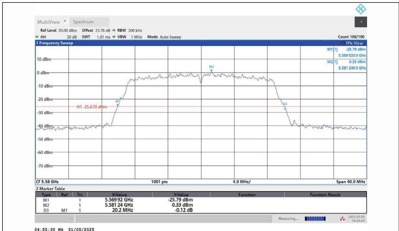
11AC20MIMO-Ant1-5580
