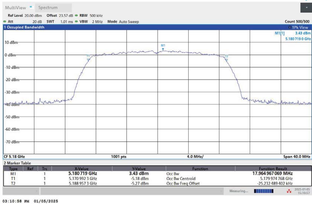
11N20MIMO-Ant1-5180
