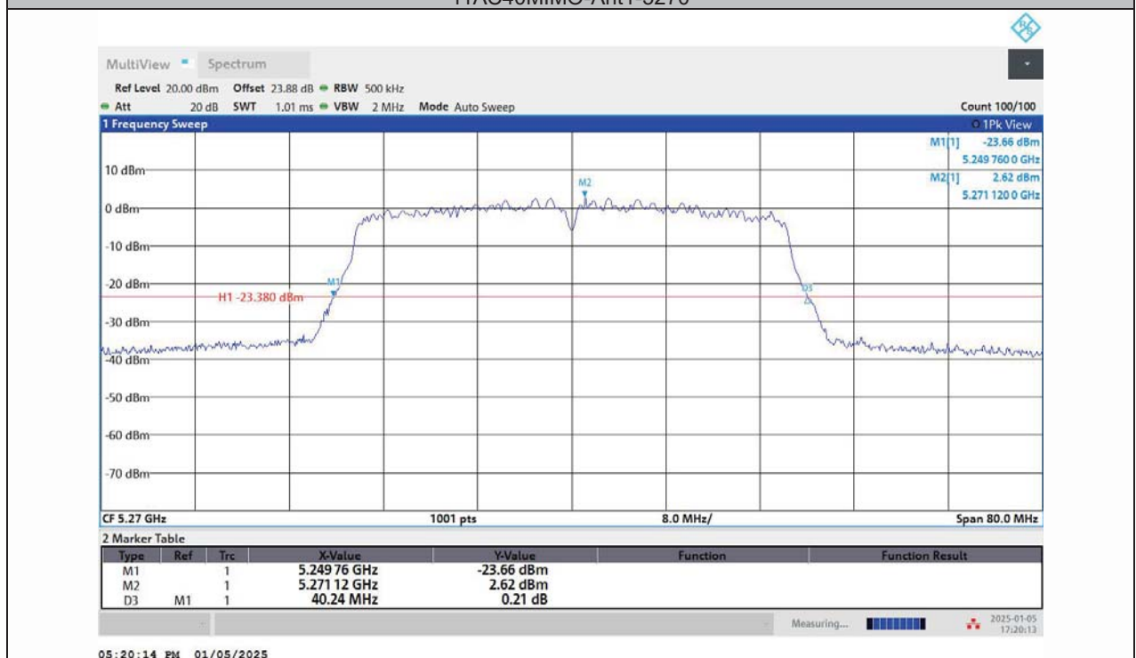
11AC40MIMO-Ant2-5270
