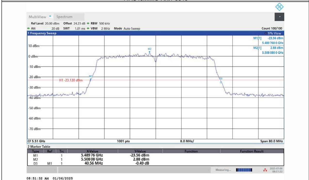
11AC40MIMO-Ant2-5510
