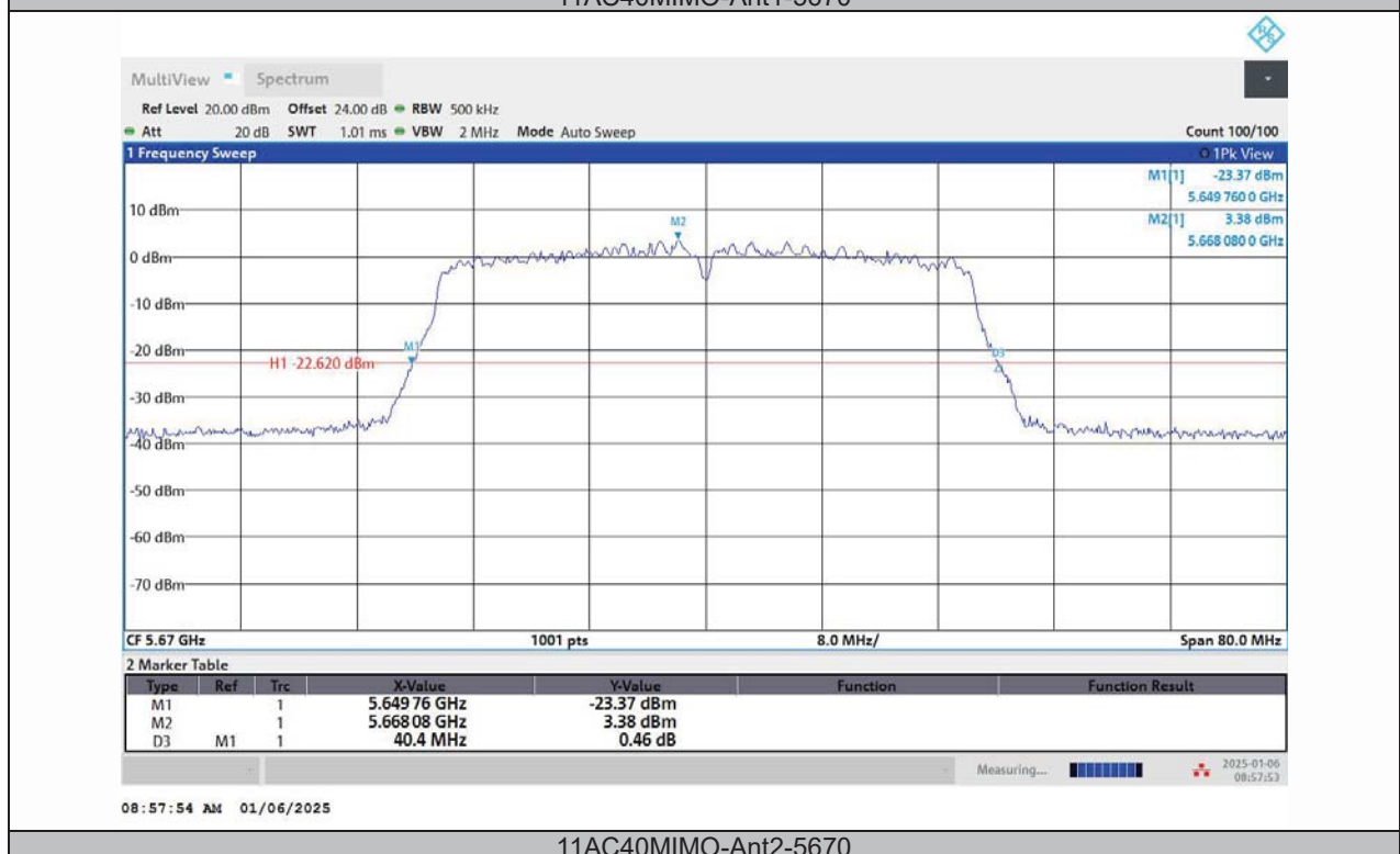
11AC40MIMO-Ant2-5670
