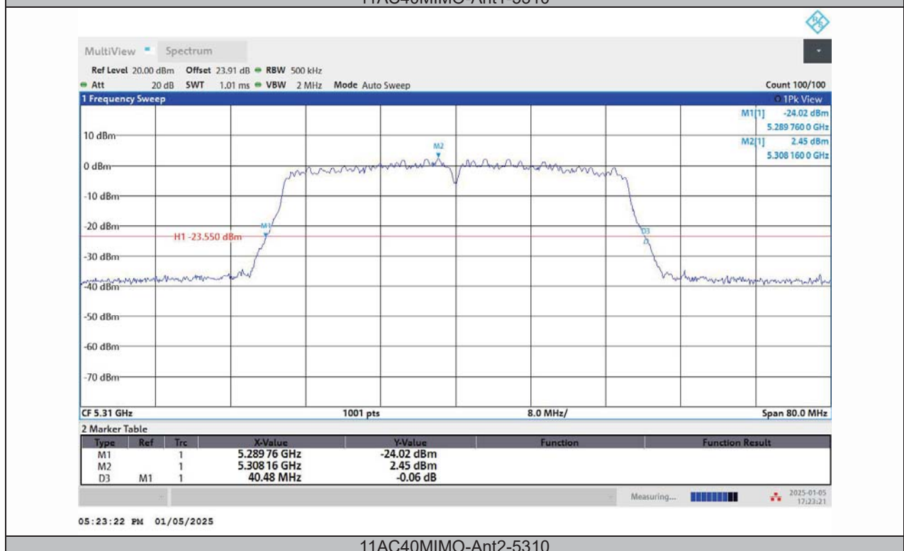
11AC40MIMO-Ant2-5310
