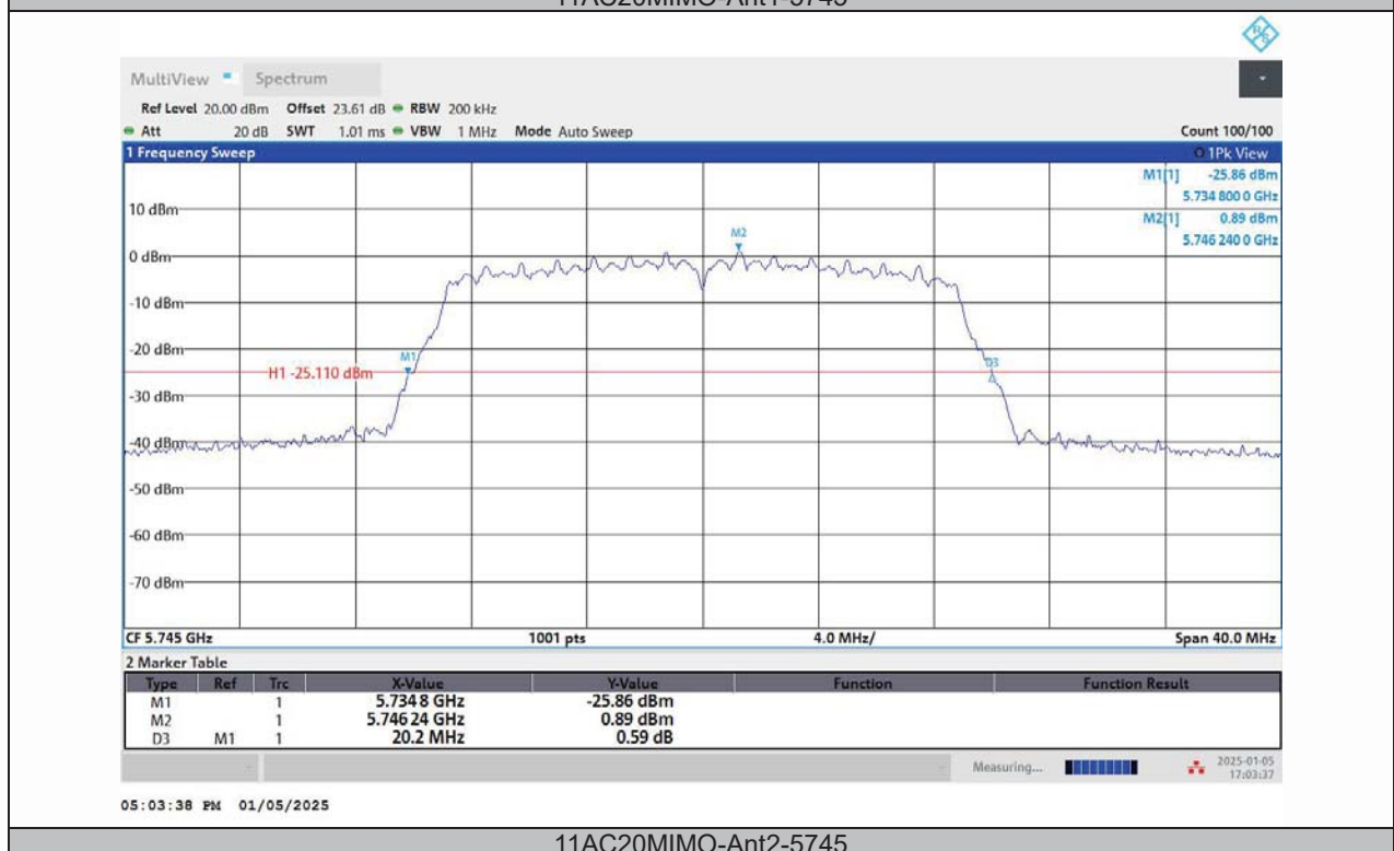
11AC20MIMO-Ant2-5745
