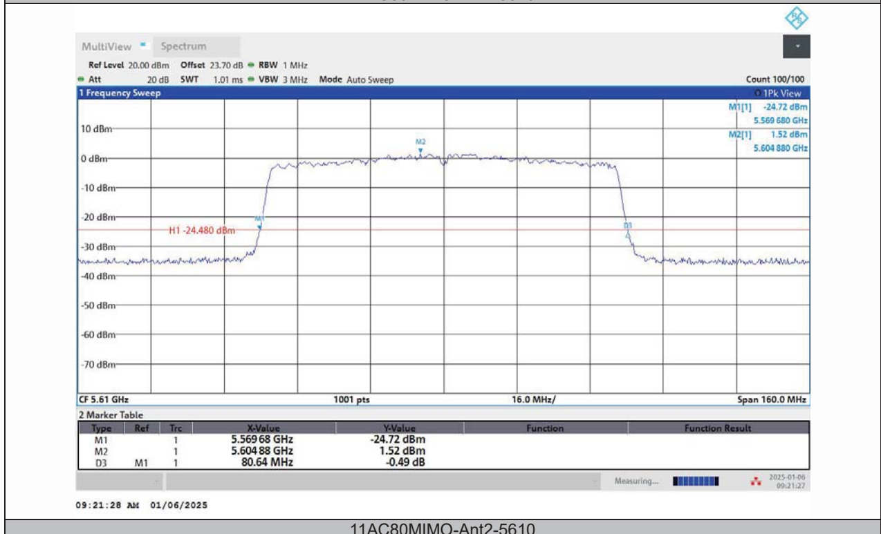
11AC80MIMO-Ant2-5610
