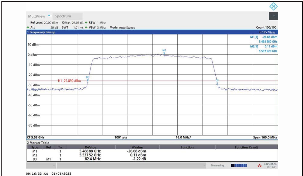
11AC80MIMO-Ant1-5530
