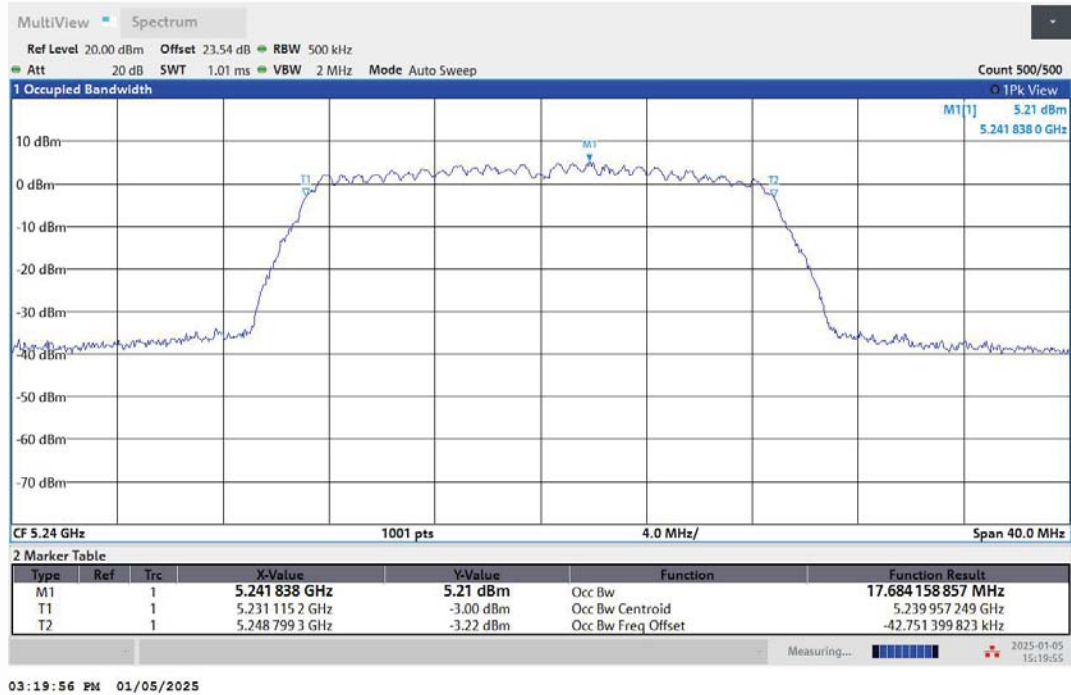
11N20MIMO-Ant2-5240
