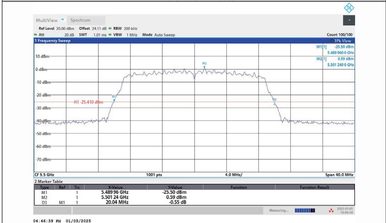
11AC20MIMO-Ant2-5500
