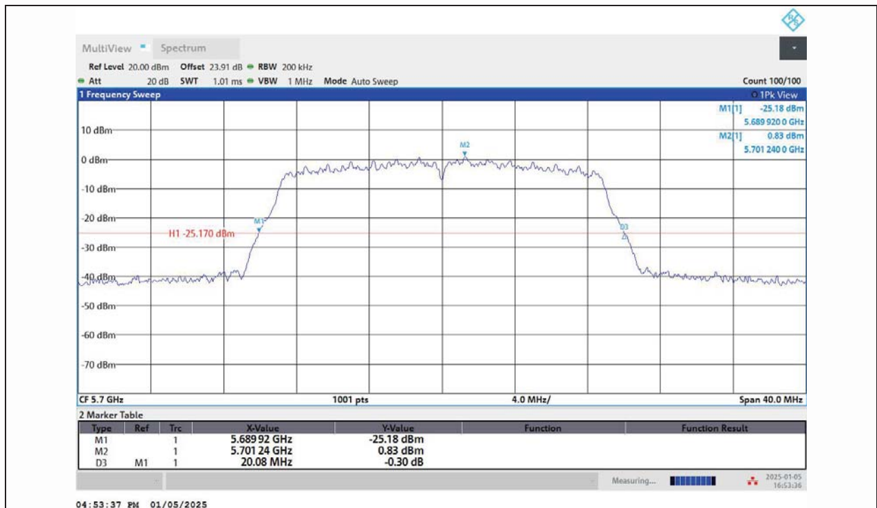
11AC20MIMO-Ant1-5700
