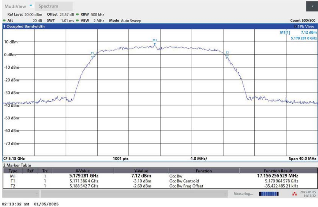
11A-Ant1-5180
