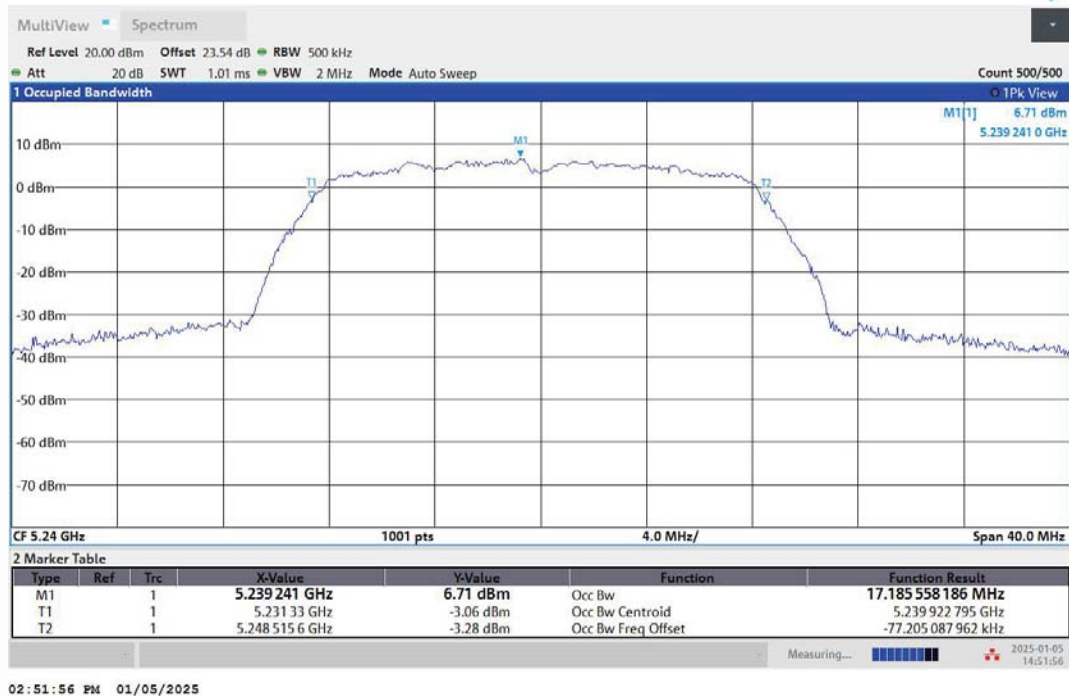
11A-Ant2-5240
