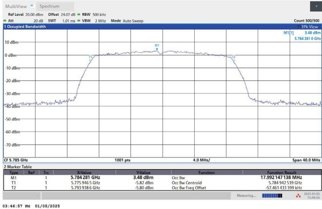
11N20MIMO-Ant1-5785
