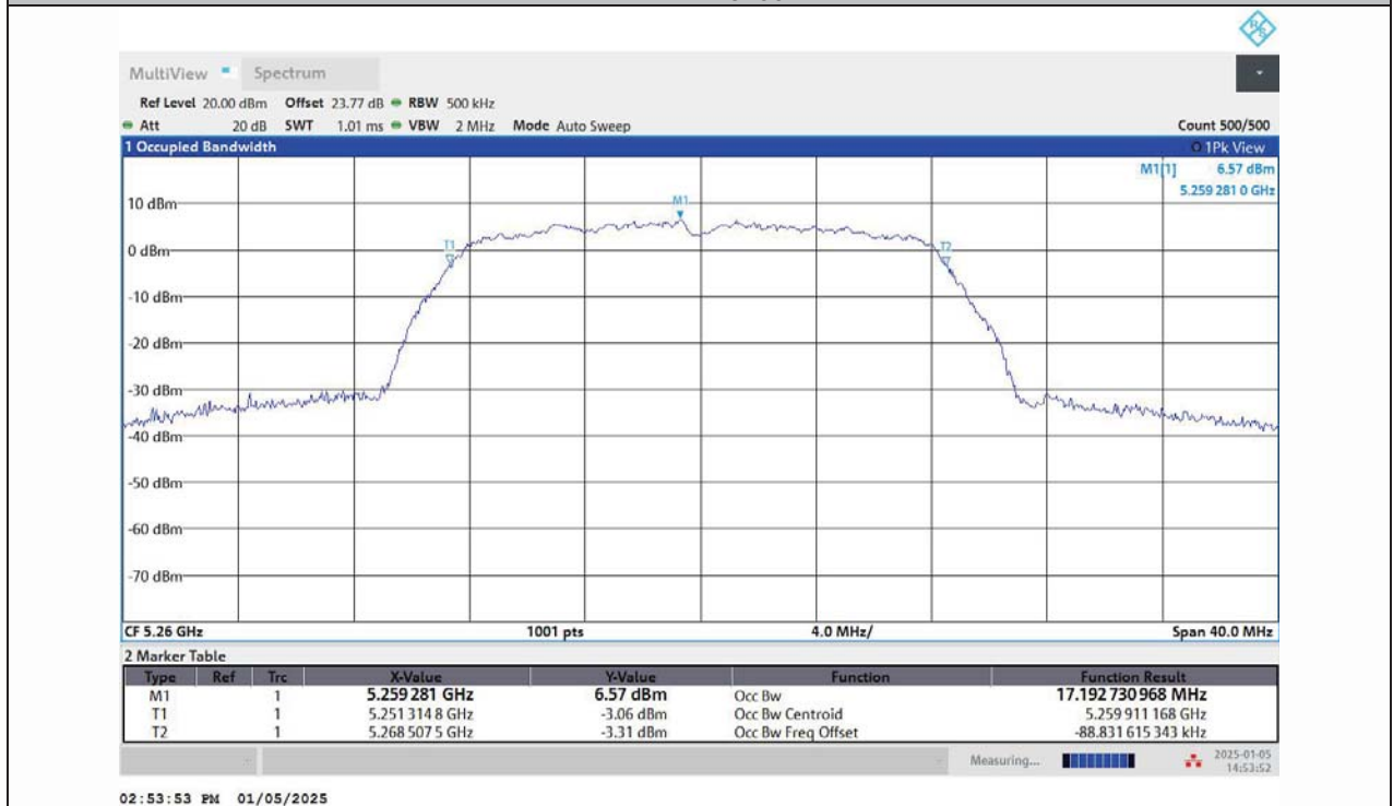
11A-Ant2-5260
