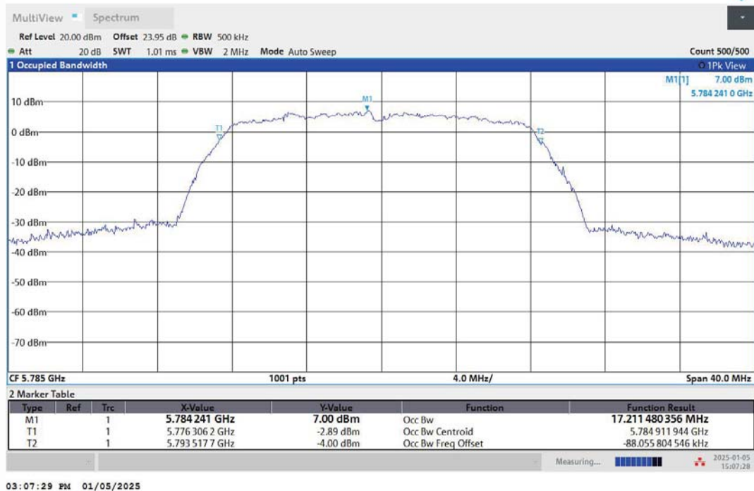
11A-Ant2-5785
