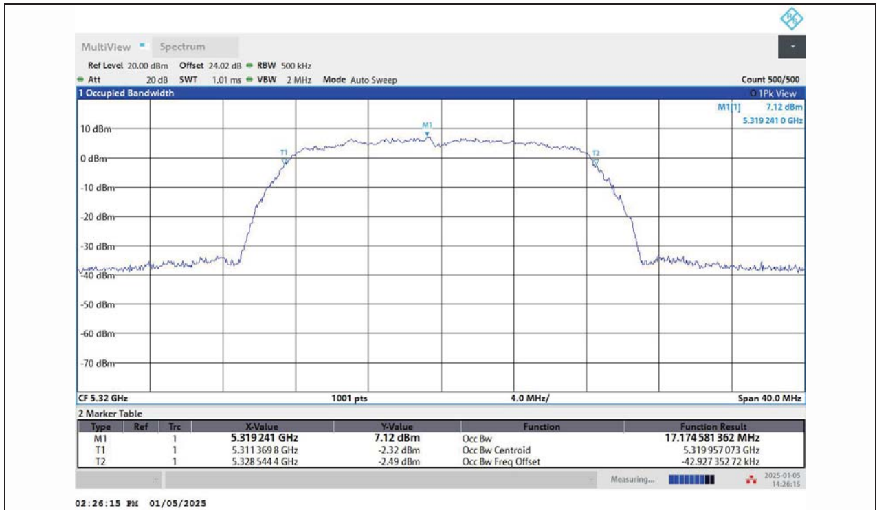
11A-Ant1-5320
