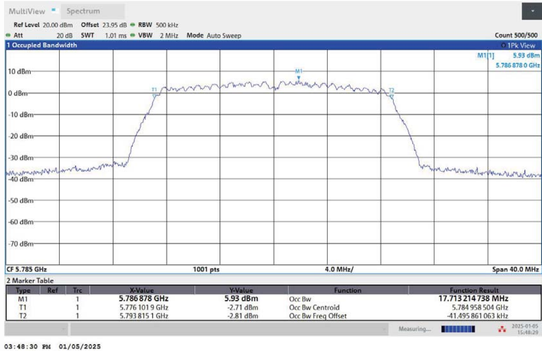
11N20MIMO-Ant2-5785
