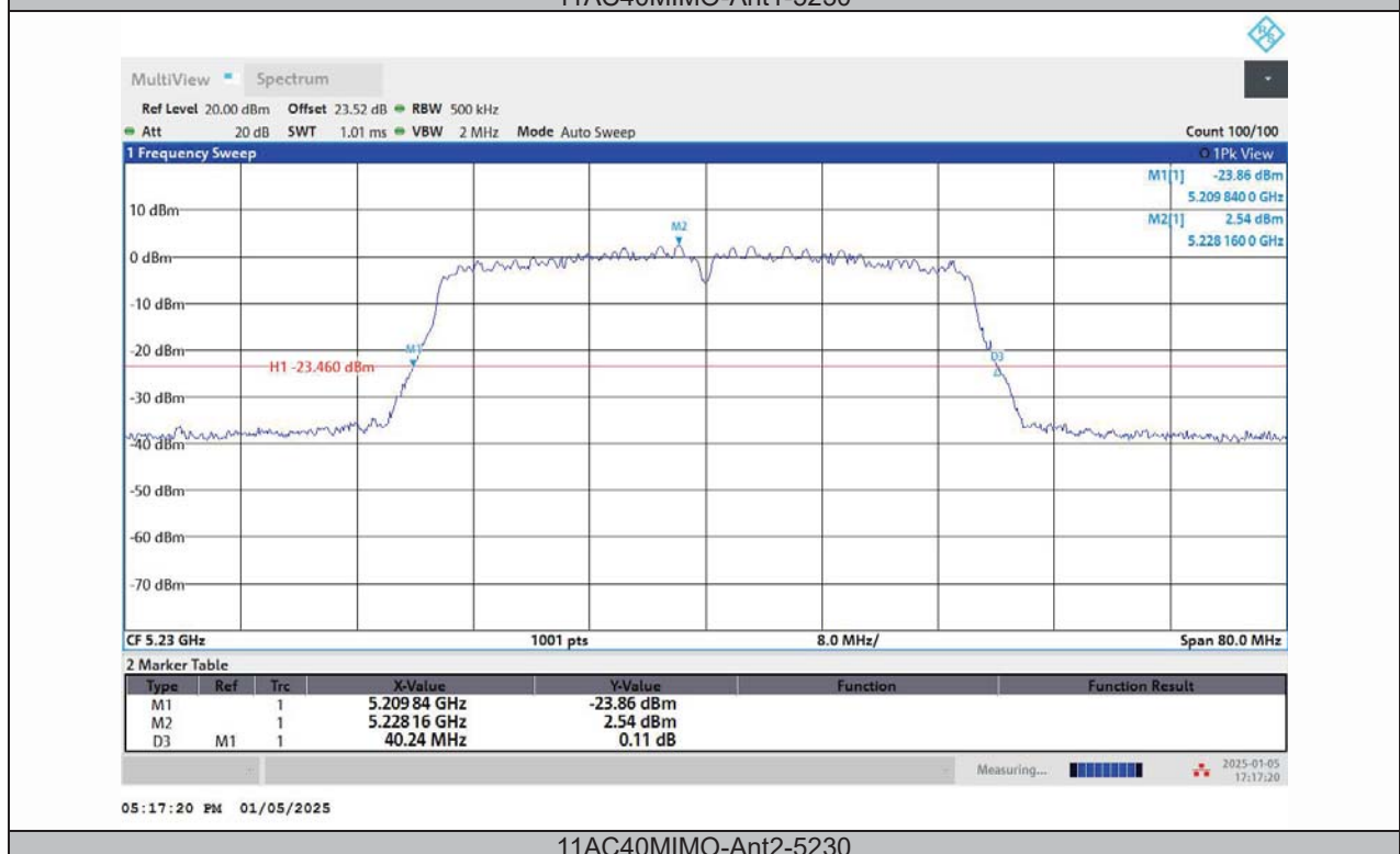
11AC40MIMO-Ant2-5230
