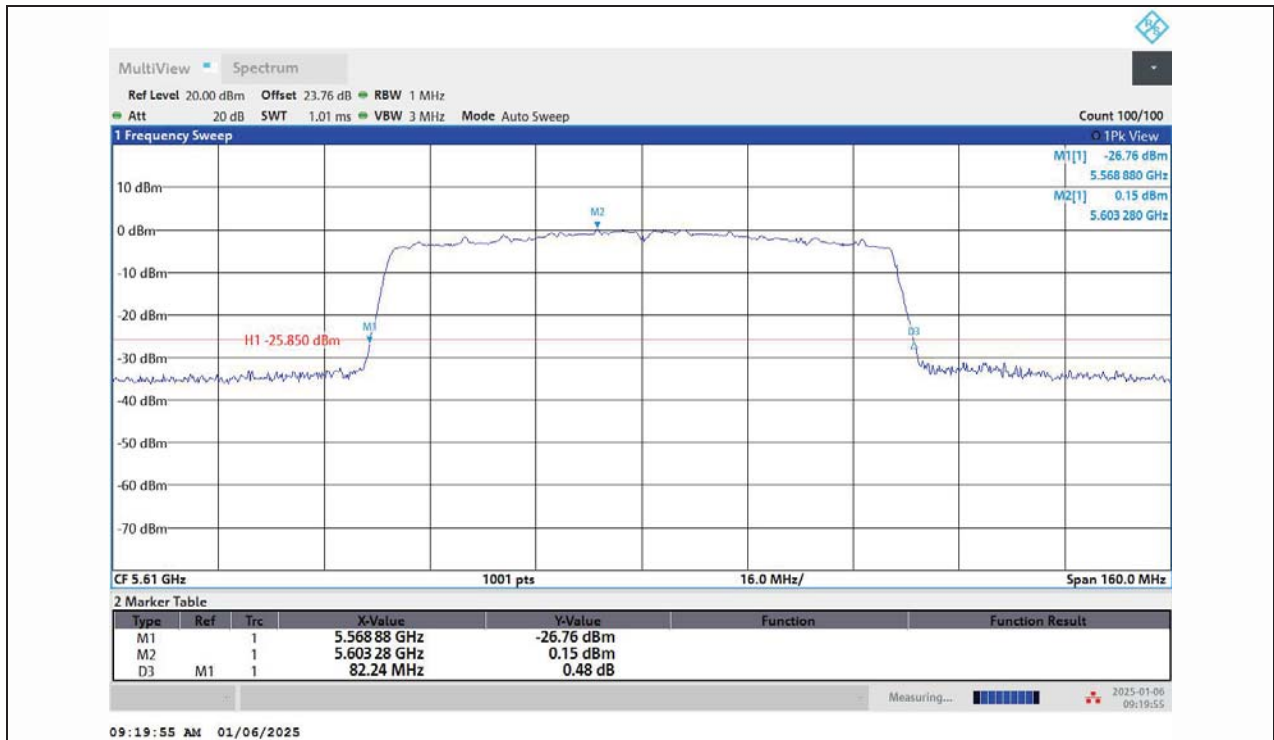
11AC80MIMO-Ant1-5610
