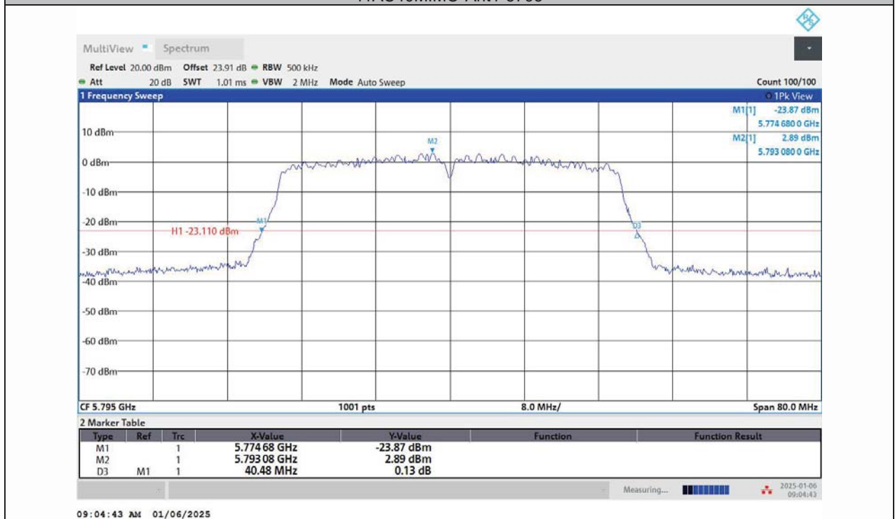
11AC40MIMO-Ant2-5795
