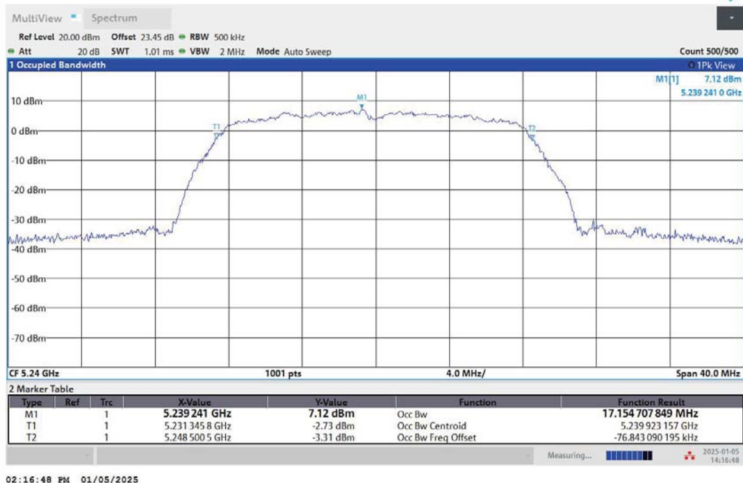
11A-Ant1-5240
