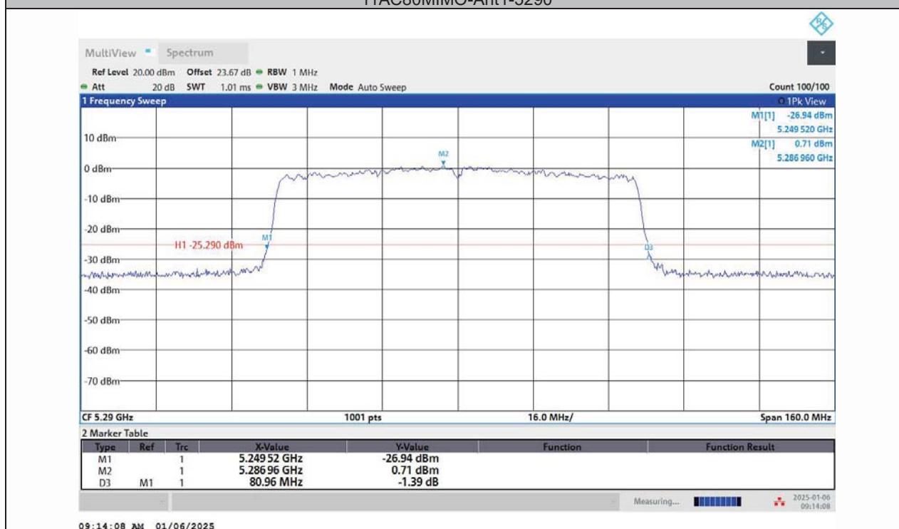
11AC80MIMO-Ant2-5290
