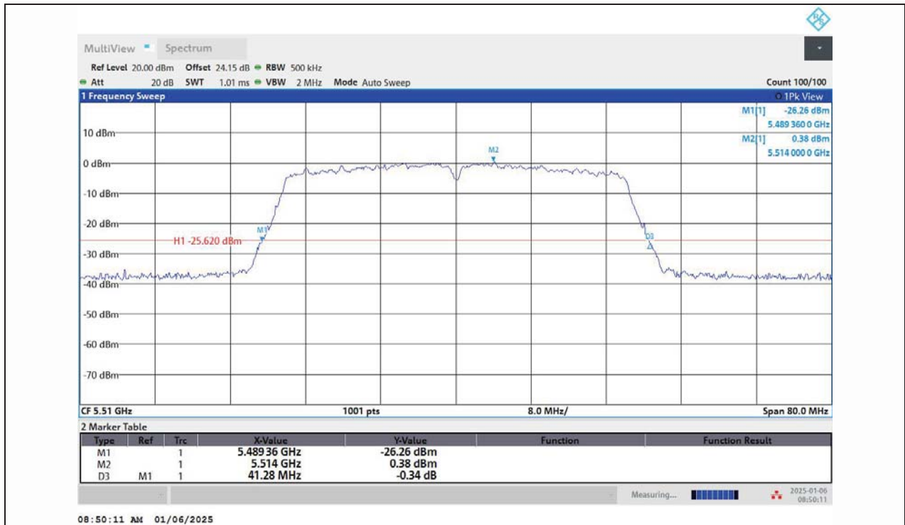
11AC40MIMO-Ant1-5510
