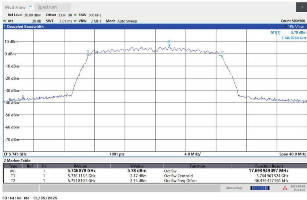
11N20MIMO-Ant2-5745
