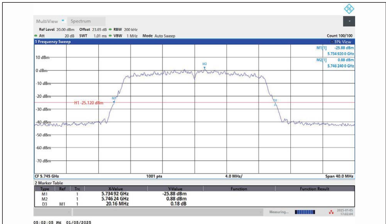
11AC20MIMO-Ant1-5745
