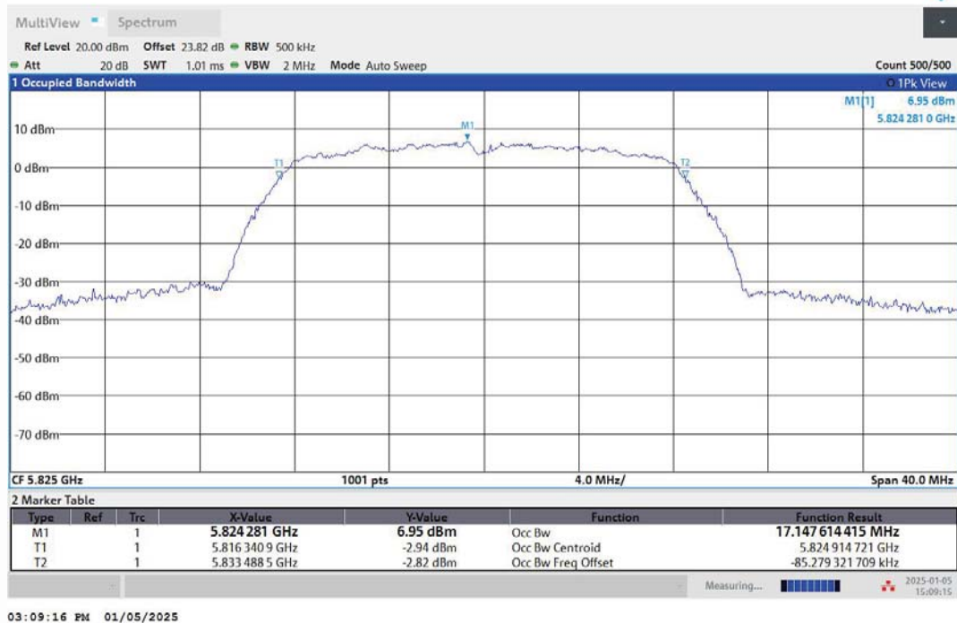
11A-Ant2-5825
