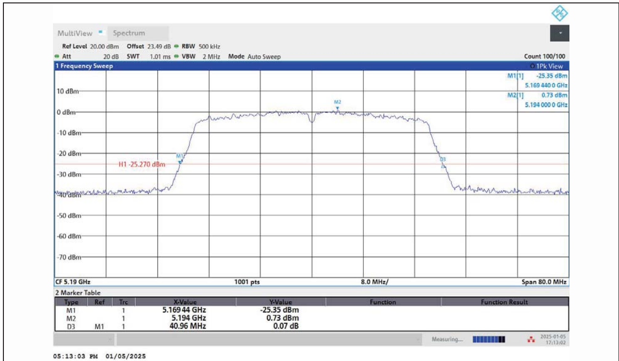
11AC40MIMO-Ant1-5190
