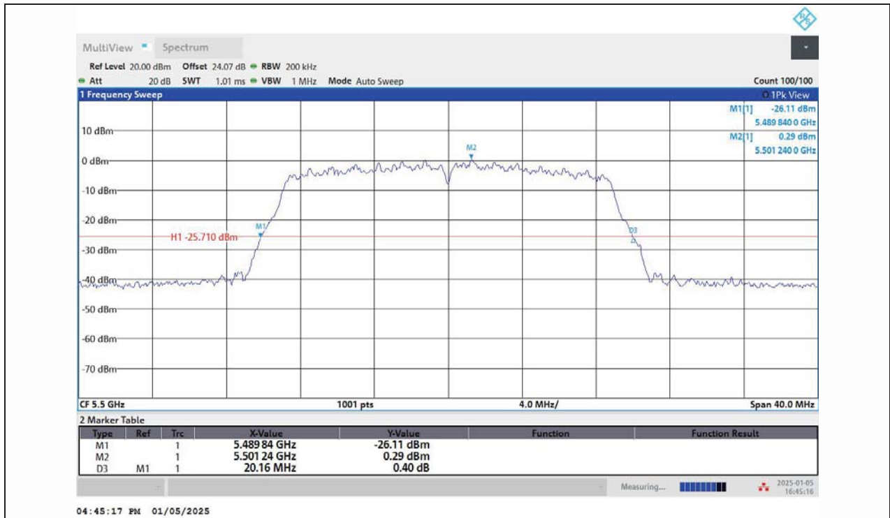
11AC20MIMO-Ant1-5500
