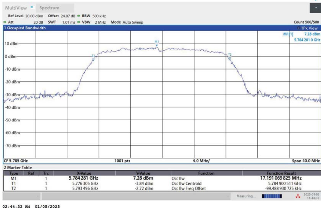
11A-Ant1-5785
