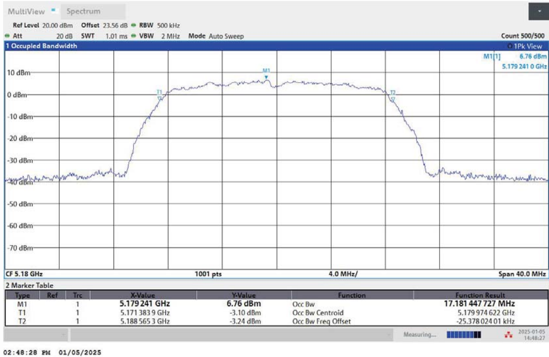
11A-Ant2-5180
