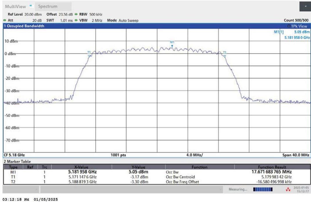
11N20MIMO-Ant2-5180
