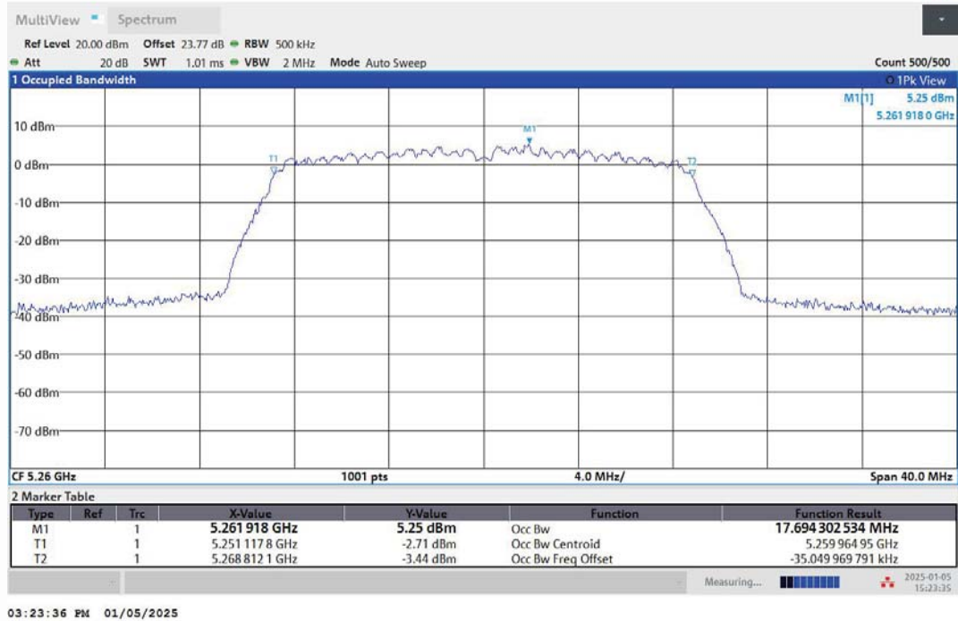
11N20MIMO-Ant2-5260
