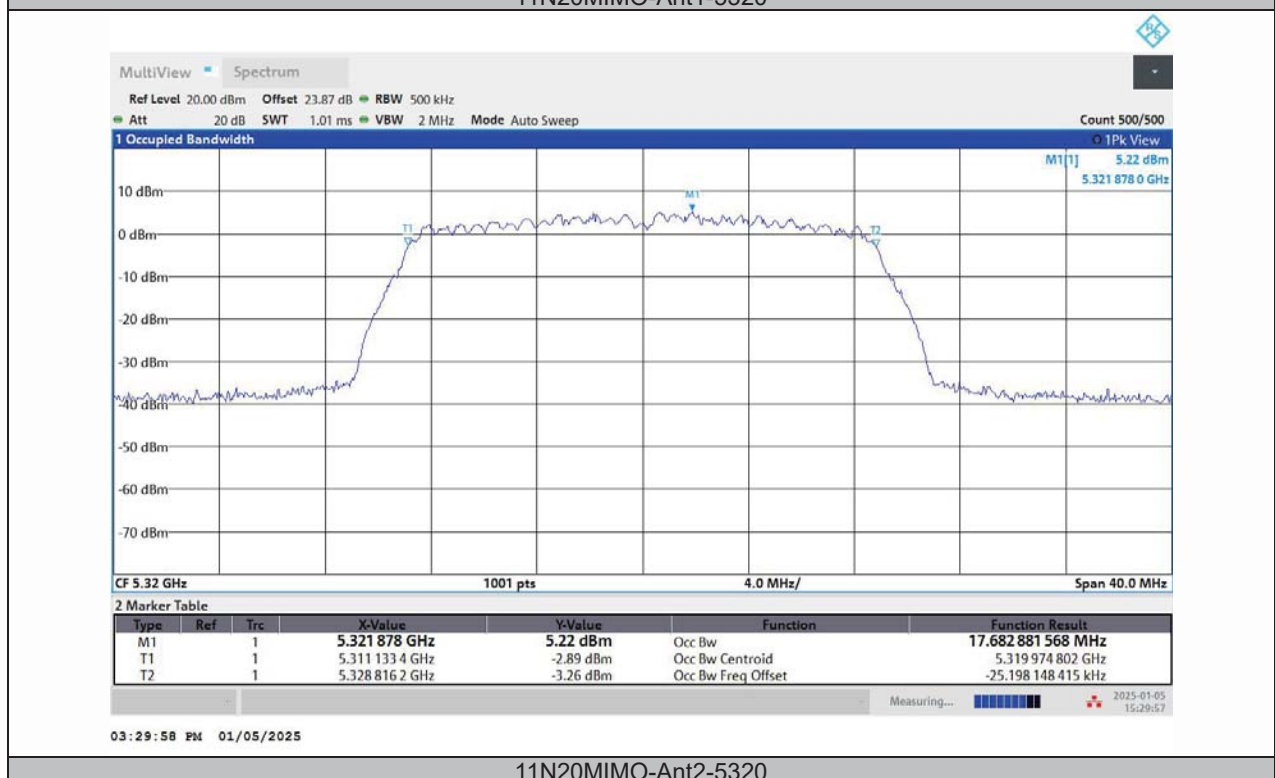
11N20MIMO-Ant2-5320
