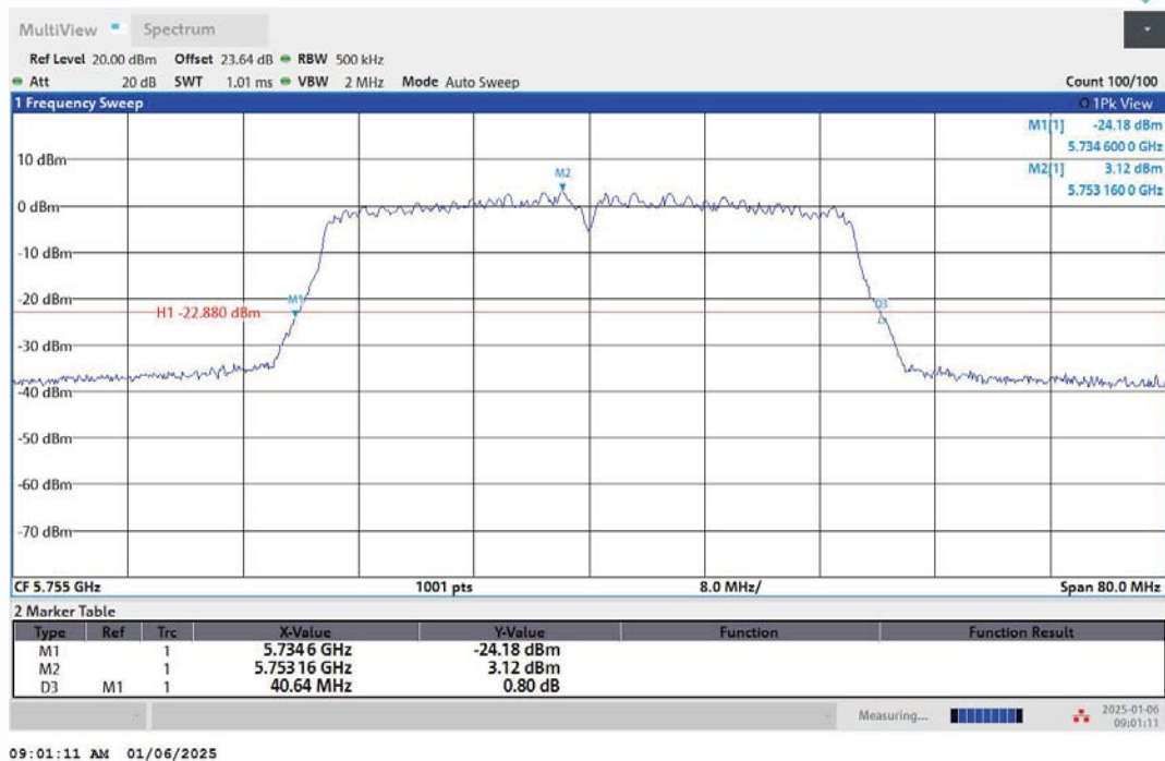
11AC40MIMO-Ant2-5755
