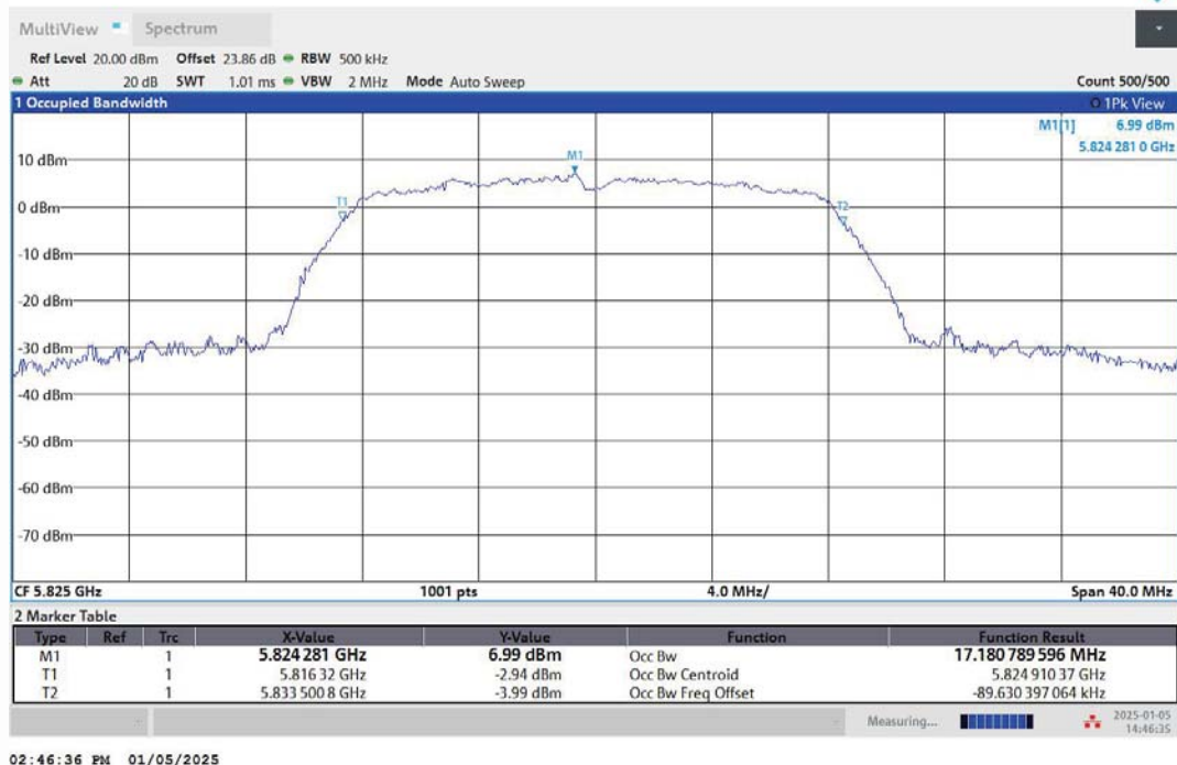
11A-Ant1-5825
