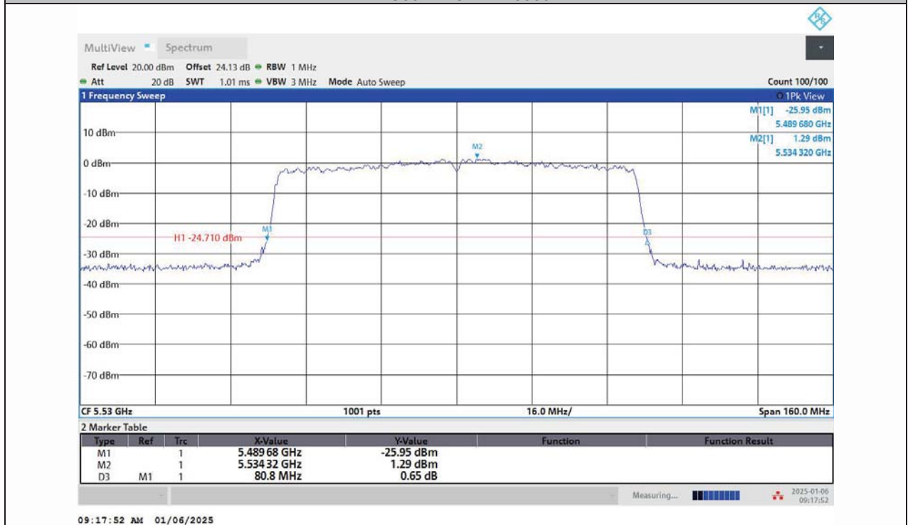
11AC80MIMO-Ant2-5530
