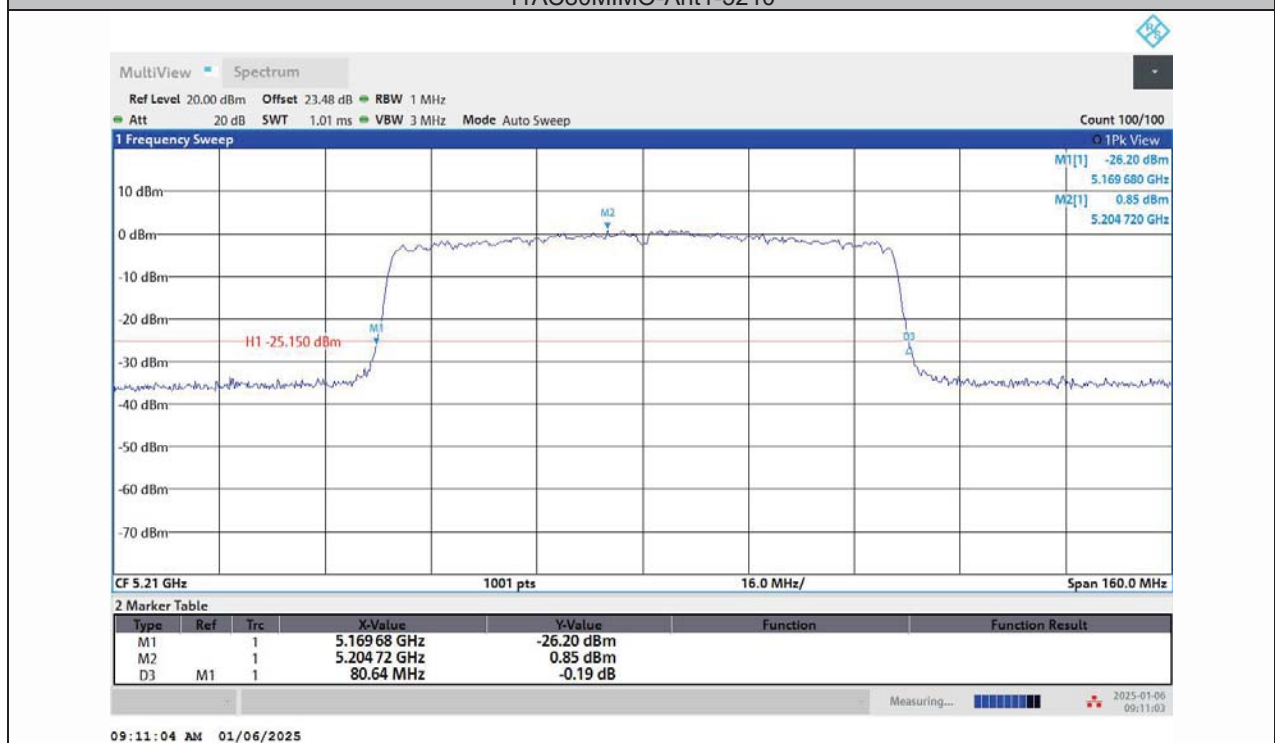
11AC80MIMO-Ant2-5210
