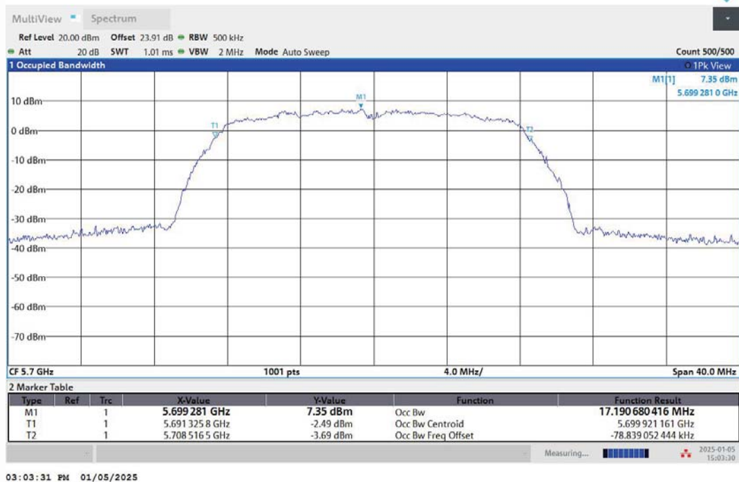
11A-Ant2-5700
