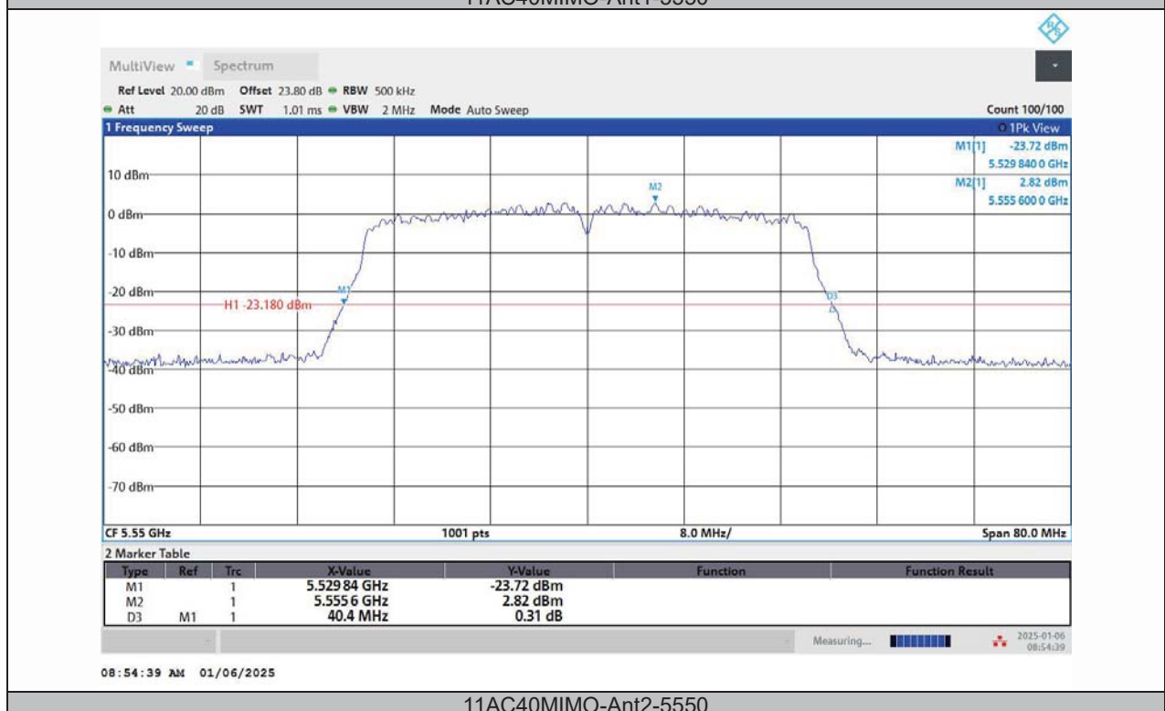
11AC40MIMO-Ant2-5550
