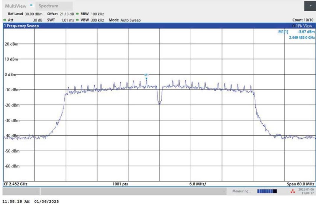
11N40MIMO-Ant1-2452-0~Reference-PASS
