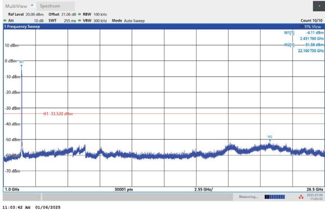
11N40MIMO-Ant1-2437-1000~26500-PASS
