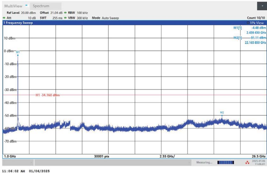
11N40MIMO-Ant2-2437-1000~26500-PASS
