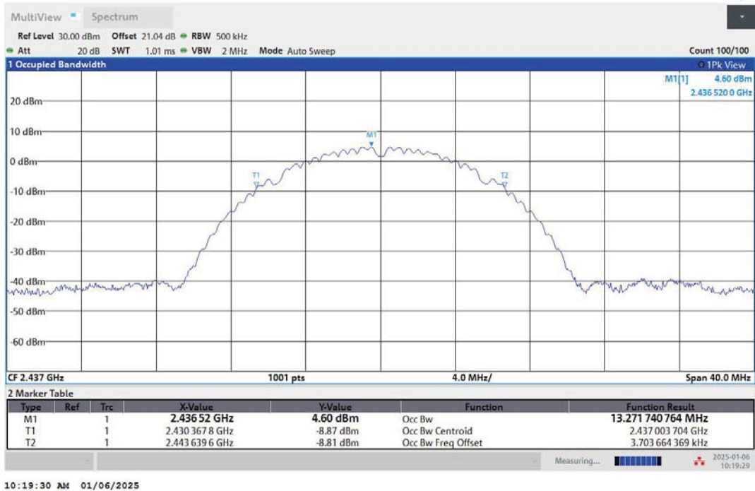
11B-Ant2-2437
