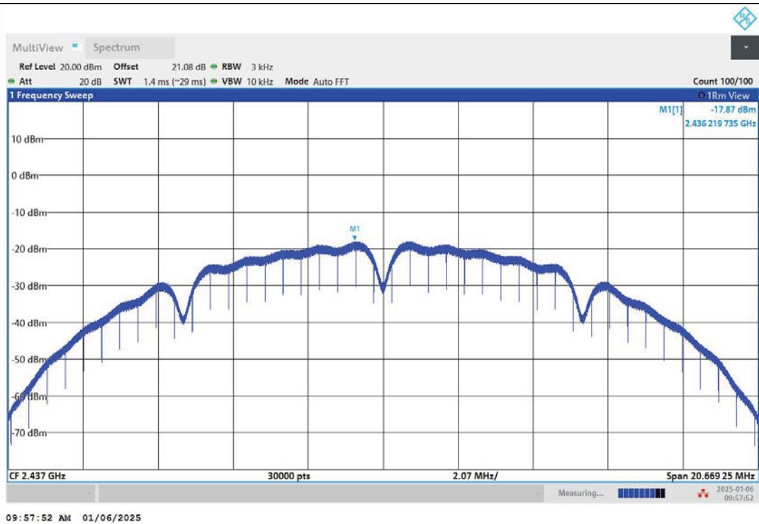
11B-Ant1-2437-PASS
