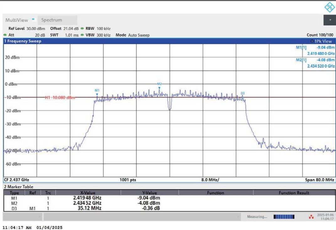
11N40MIMO-Ant2-2437-PASS
