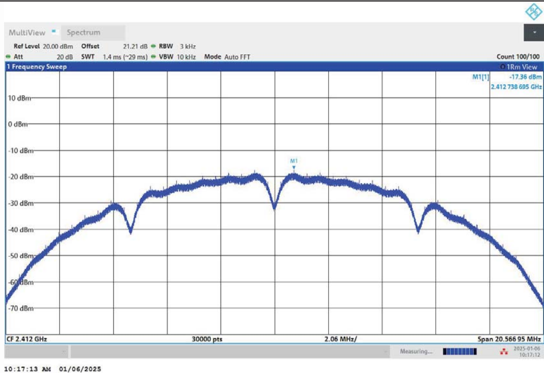
11B-Ant2-2412-PASS
