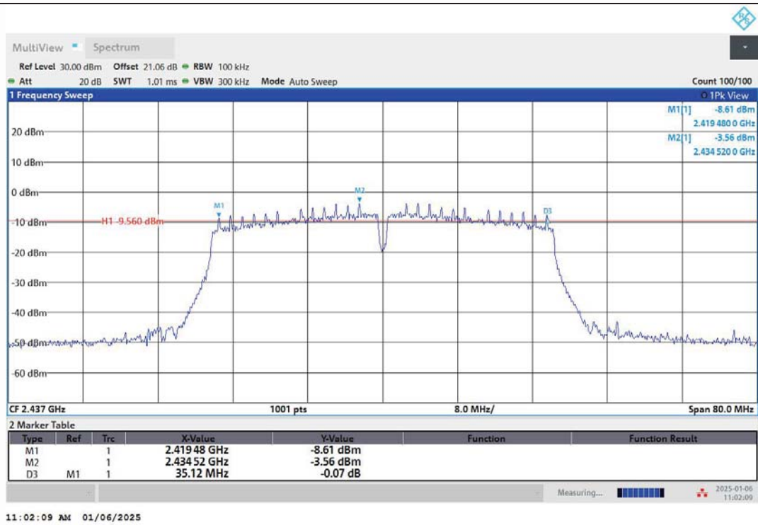
11N40MIMO-Ant1-2437-PASS
