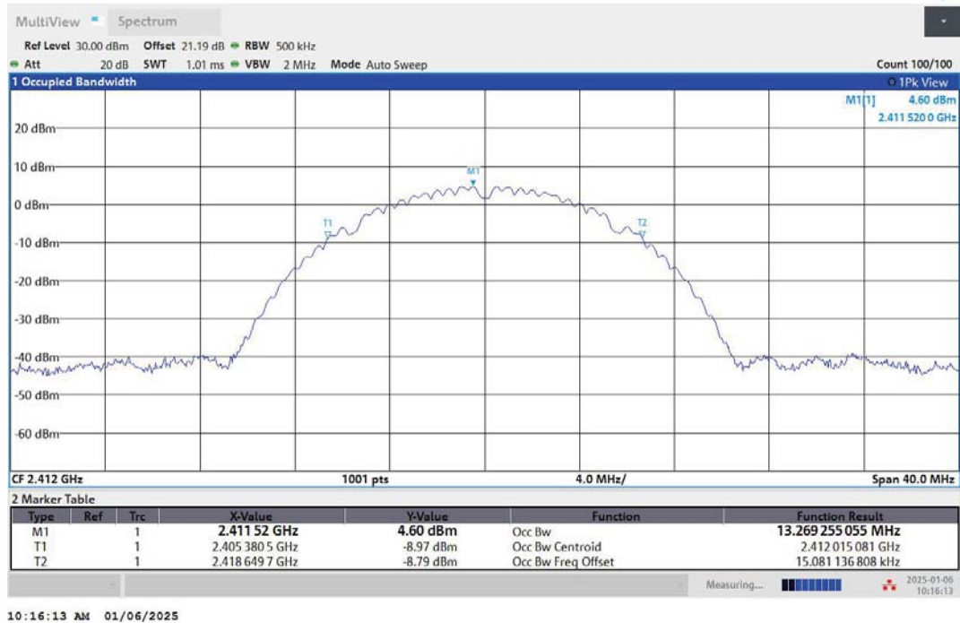
11B-Ant2-2412
