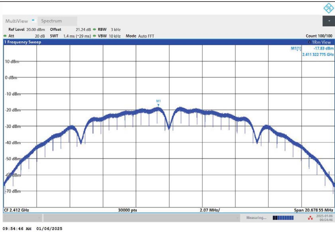
11B-Ant1-2412-PASS
