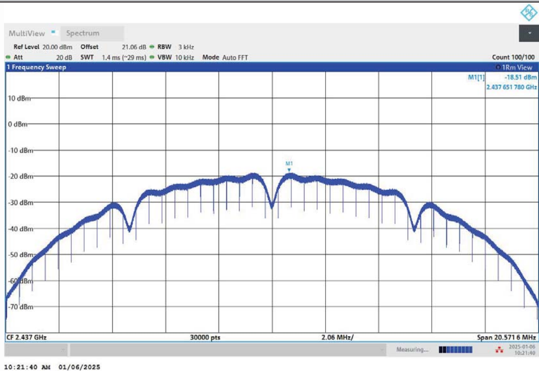
11B-Ant2-2437-PASS
