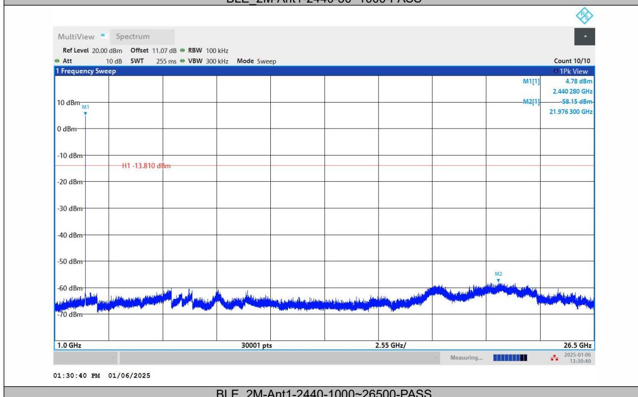
BLE_2M-Ant1-2440-1000~26500-PASS
