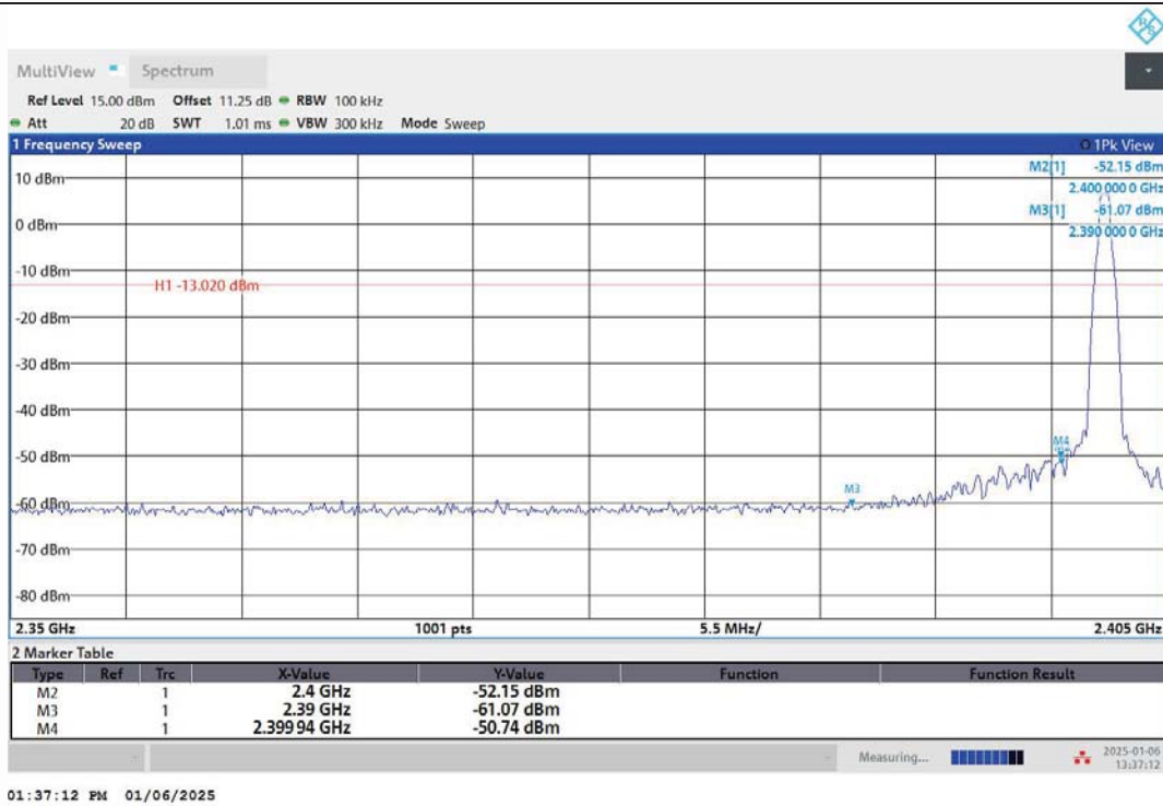
DH5-Ant1-2402-PASS
