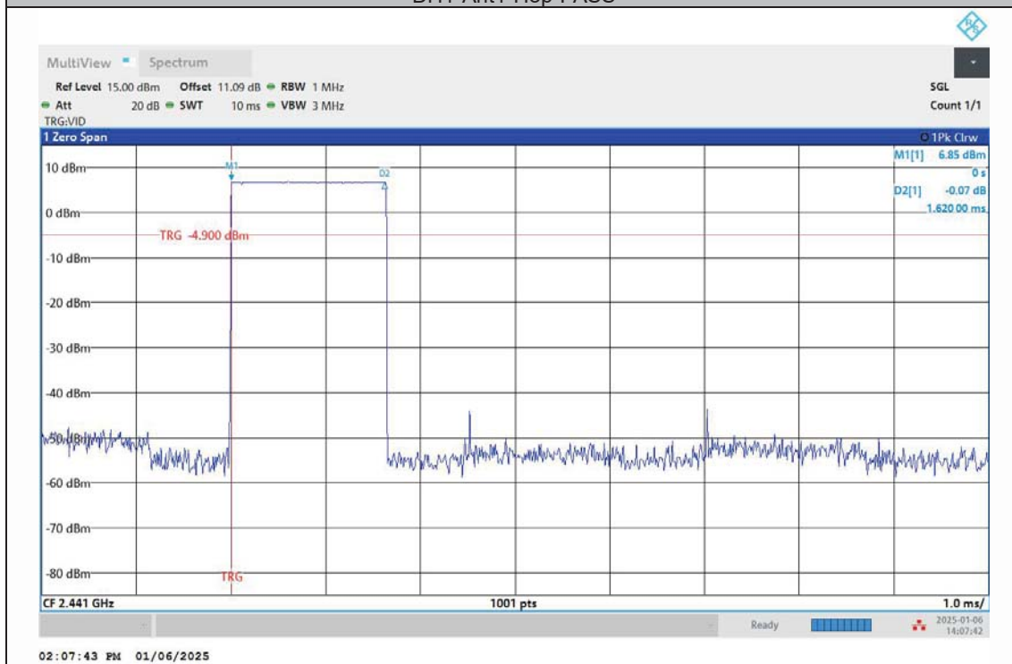
DH3-Ant1-Hop-PASS
