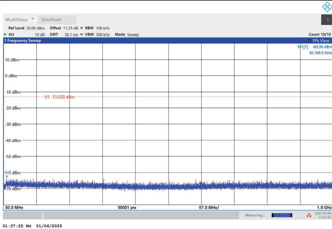
DH5-Ant1-2402-30~1000-PASS
