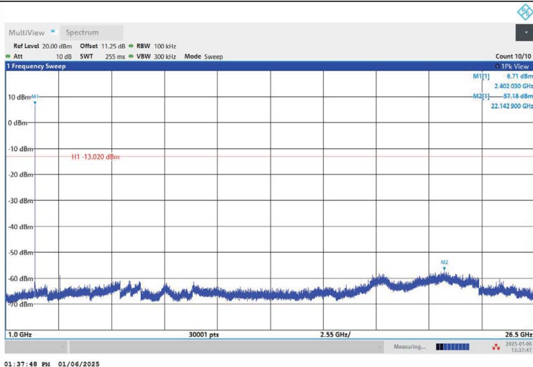
DH5-Ant1-2402-1000~26500-PASS
