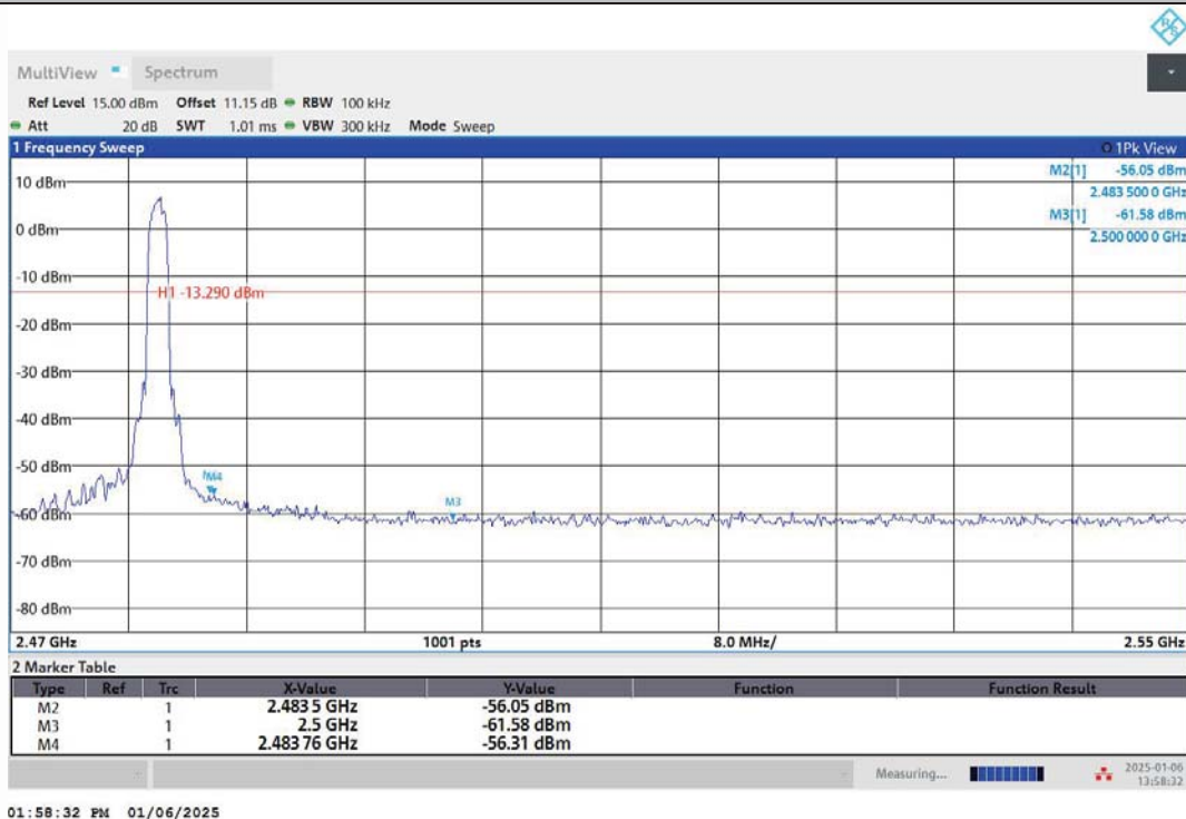
3DH5-Ant1-2480-PASS
