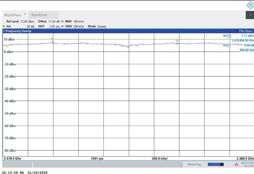
2DH5-Ant1-Hop_2480-PASS
