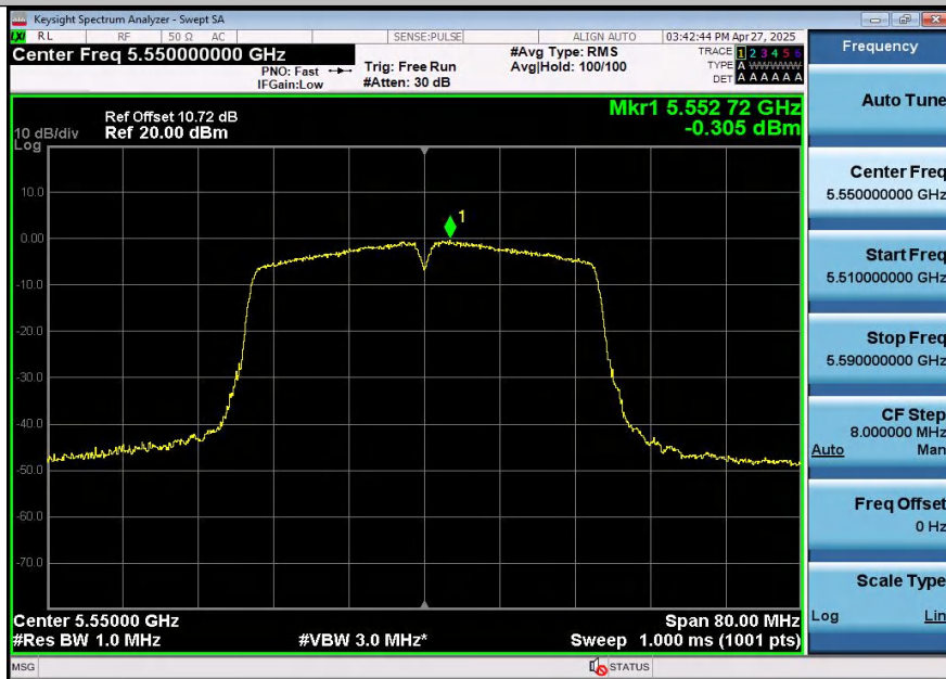
11N40SISO-Ant2-5550-PASS
