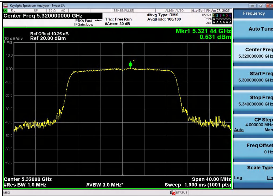
11AX20SISO-Ant1-5320-PASS
