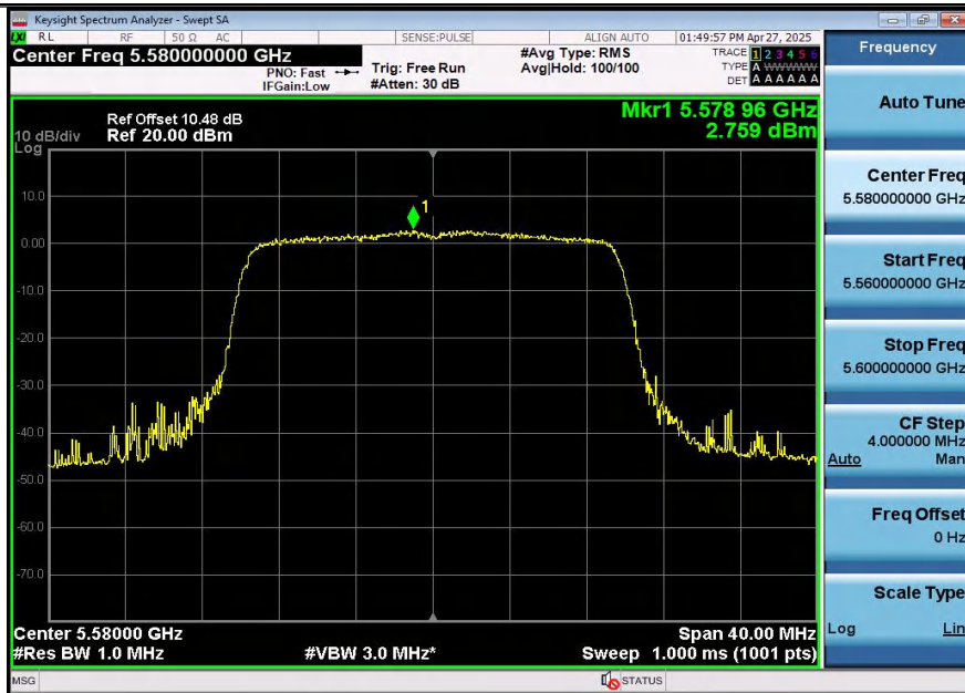
11AX20SISO-Ant1-5580-PASS
