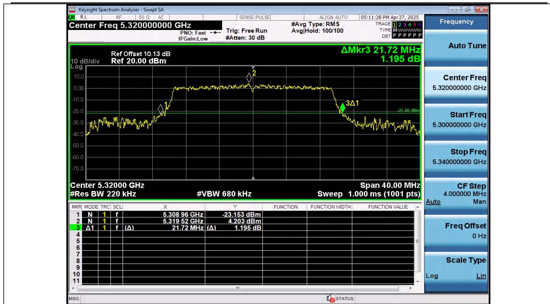
11AX20SISO-Ant2-5320
