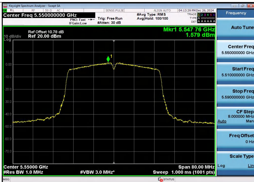
11AC40SISO-Ant2-5550-PASS
