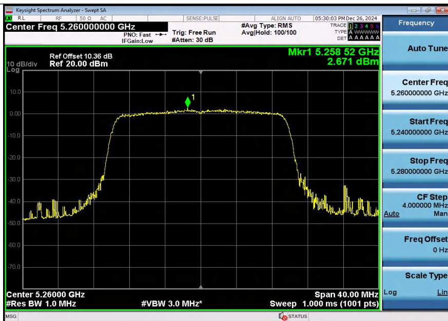
11AX20SISO-Ant2-5260-PASS
