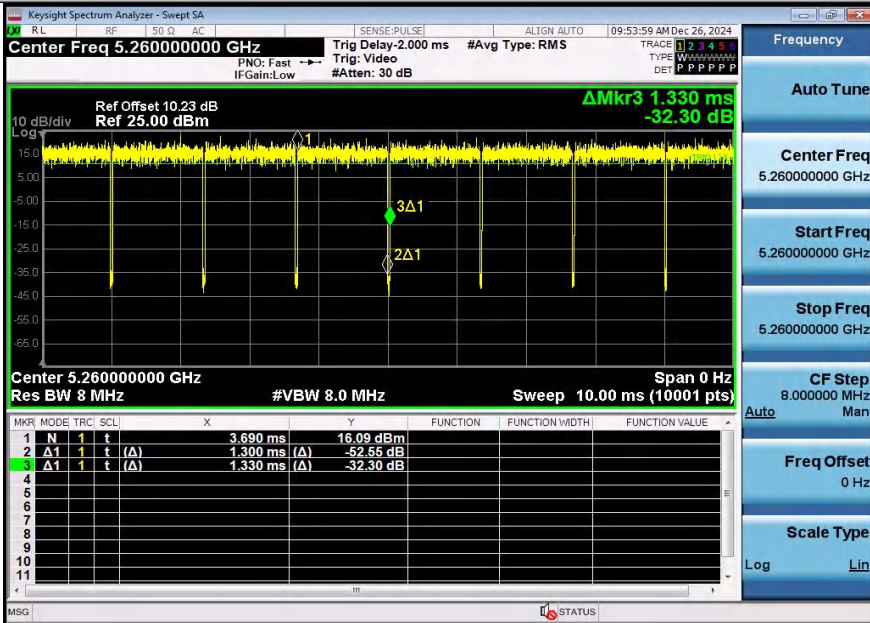
NTNV-11N20SISO-Ant1-5260
