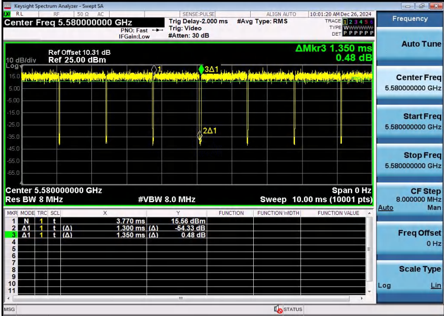
NTNV-11N20SISO-Ant1-5580
