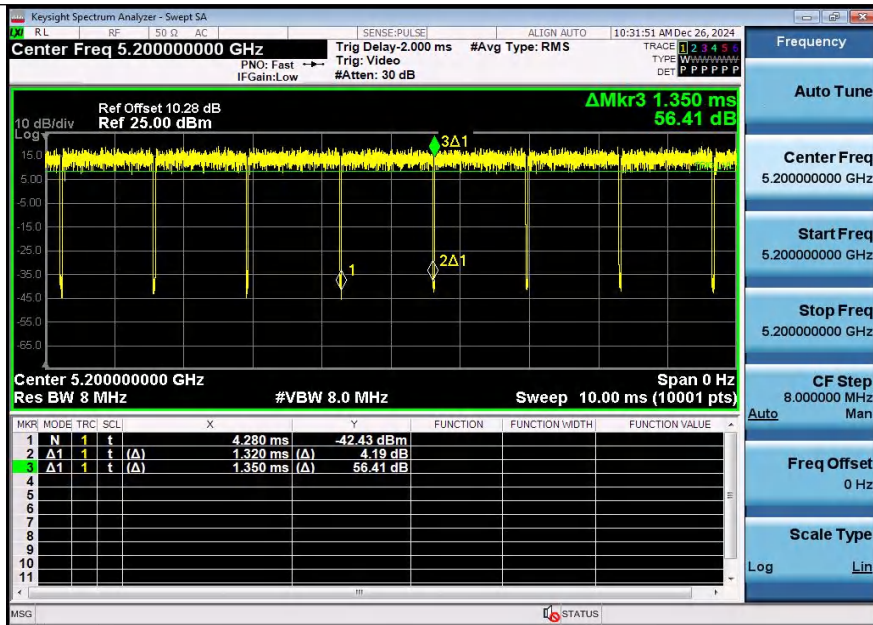
NTNV-11AC20SISO-Ant1-5200
