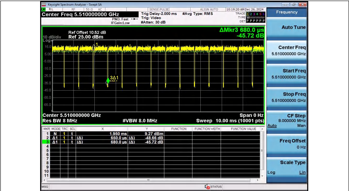
NTNV-11N40SISO-Ant1-5510
