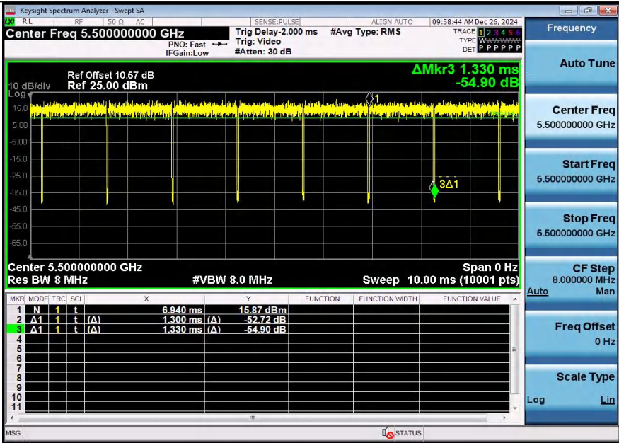
NTNV-11N20SISO-Ant1-5500
