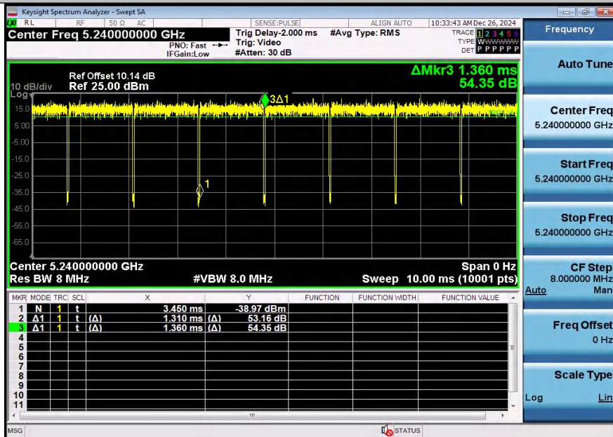
NTNV-11AC20SISO-Ant1-5240
