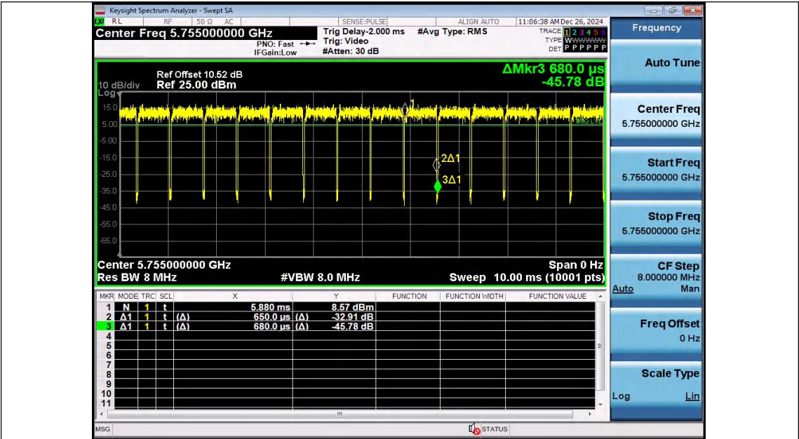
NTNV-11AC40SISO-Ant1-5755
