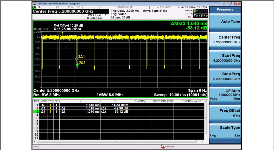
NTNV-11AX20SISO-Ant1-5200
