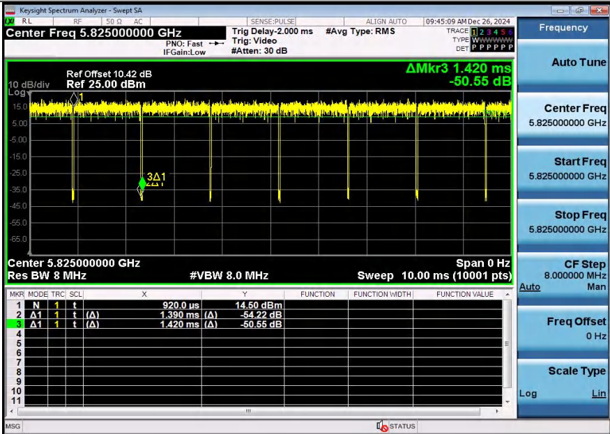
NTNV-11A-Ant1-5825
