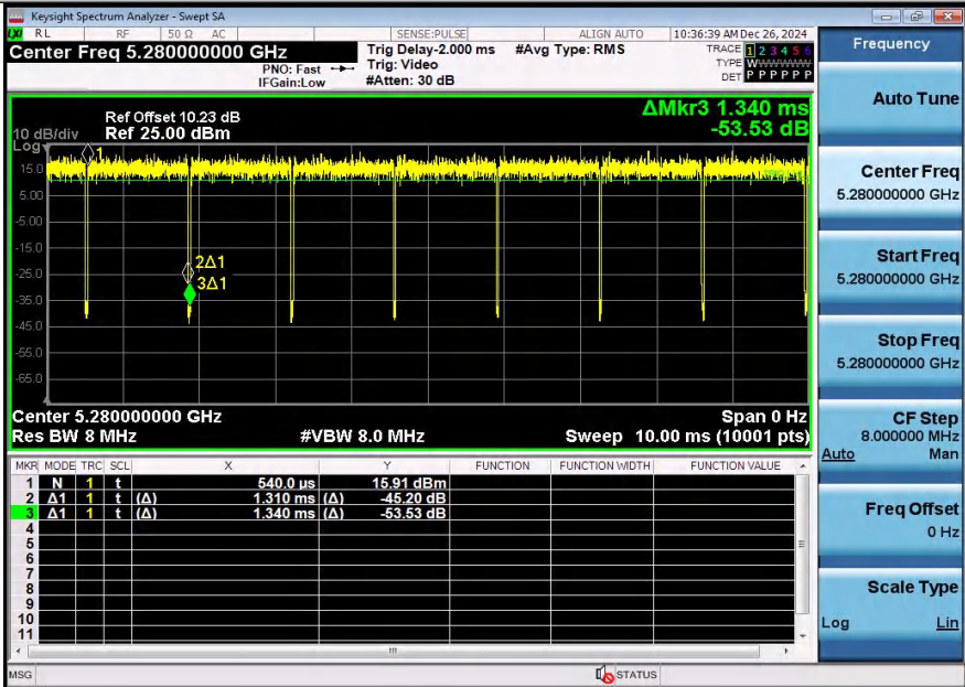
NTNV-11AC20SISO-Ant1-5280
