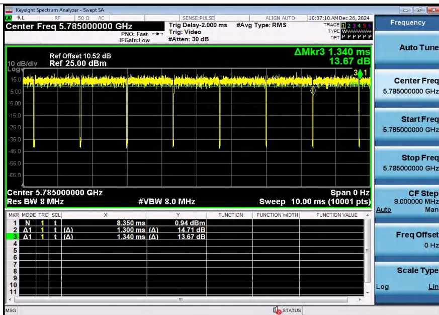
NTNV-11N20SISO-Ant1-5785
