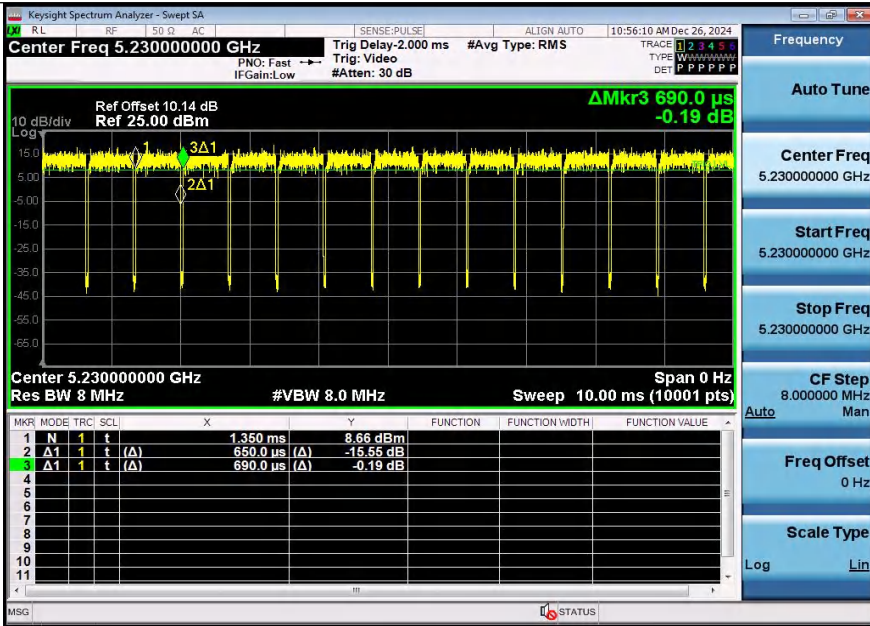
NTNV-11AC40SISO-Ant1-5230
