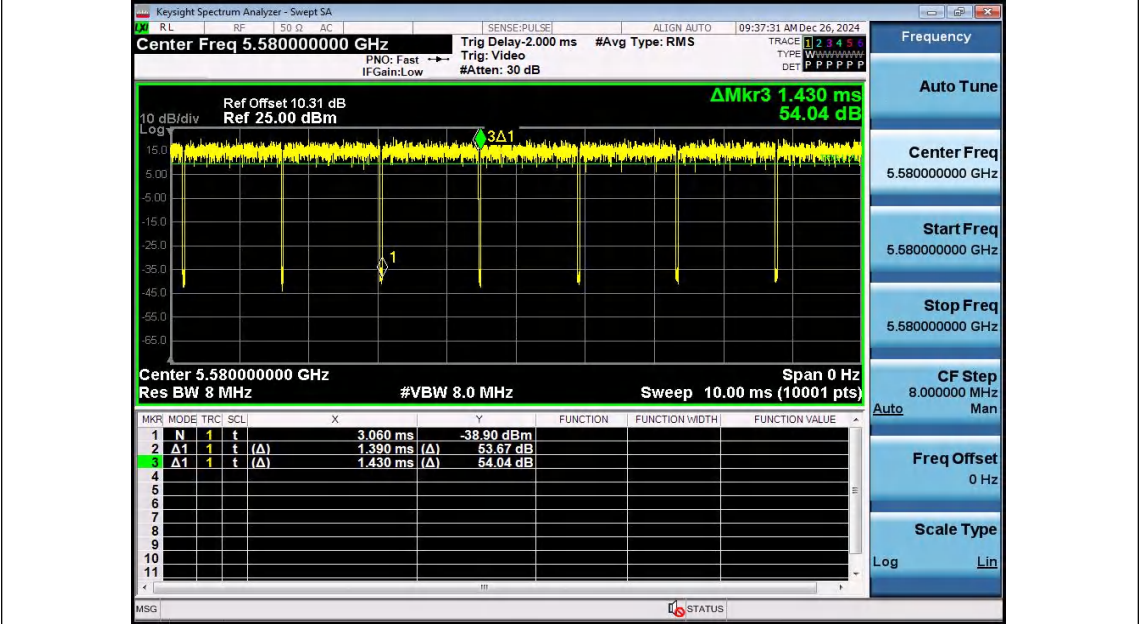
NTNV-11A-Ant1-5580
