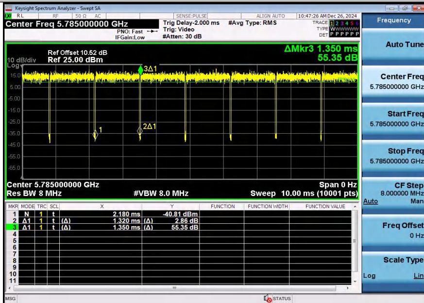
NTNV-11AC20SISO-Ant1-5785
