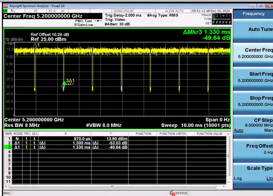
NTNV-11N20SISO-Ant1-5200
