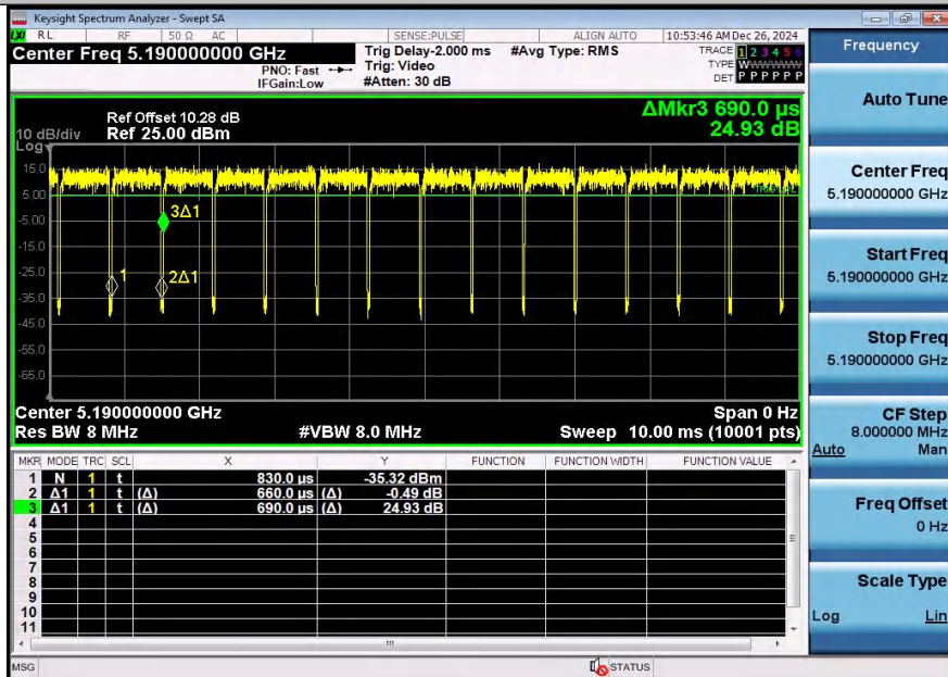
NTNV-11AC40SISO-Ant1-5190
