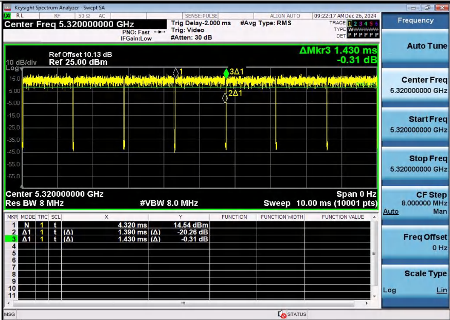
NTNV-11A-Ant1-5320
