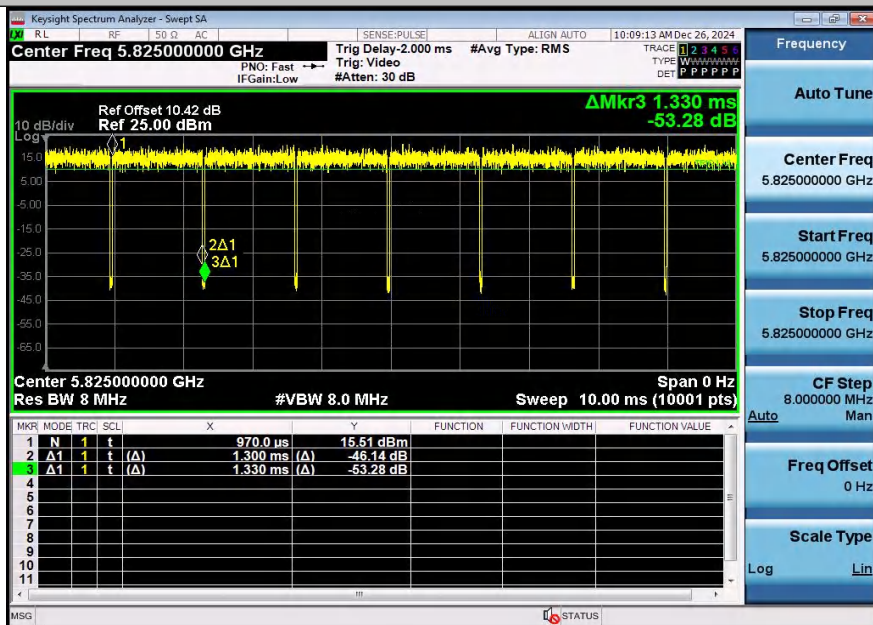
NTNV-11N20SISO-Ant1-5825
