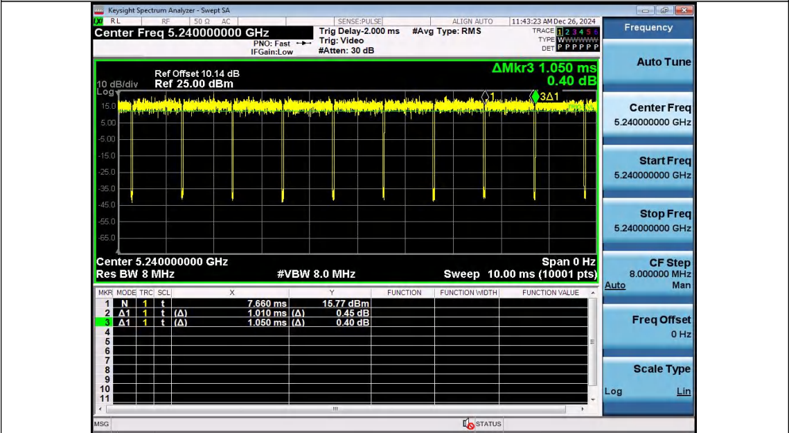
NTNV-11AX20SISO-Ant1-5240
