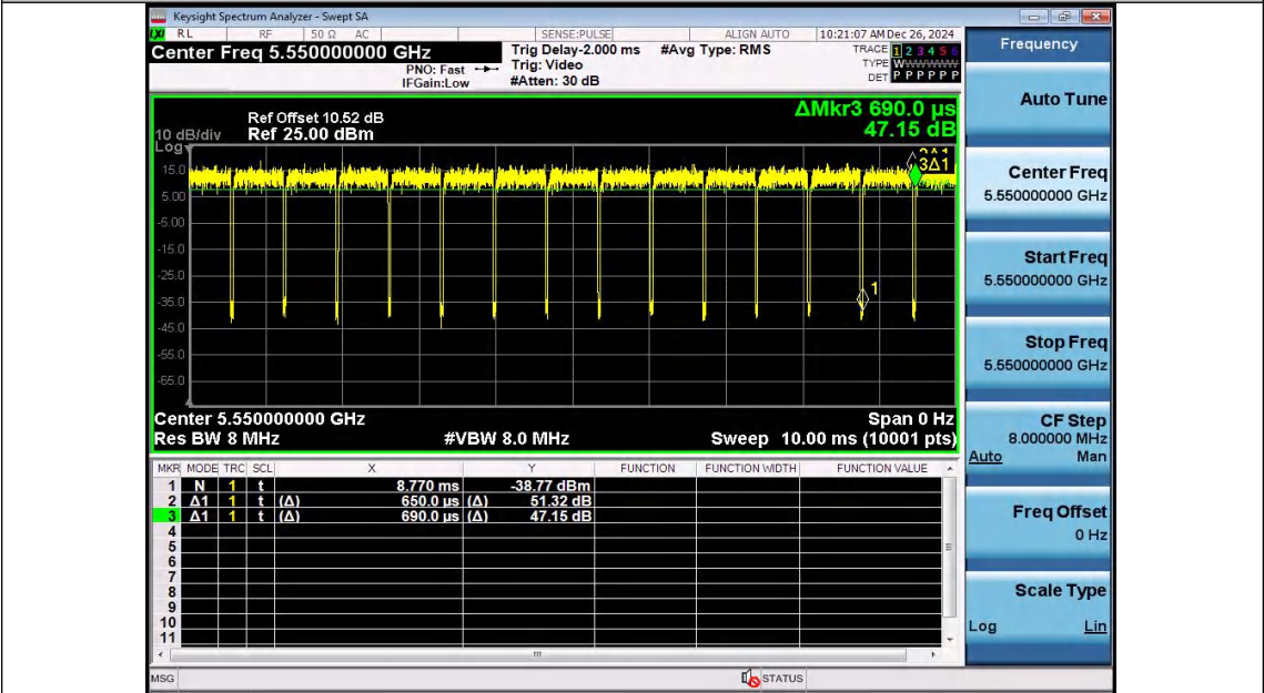
NTNV-11N40SISO-Ant1-5550
