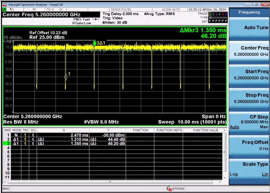
NTNV-11AC20SISO-Ant1-5260
