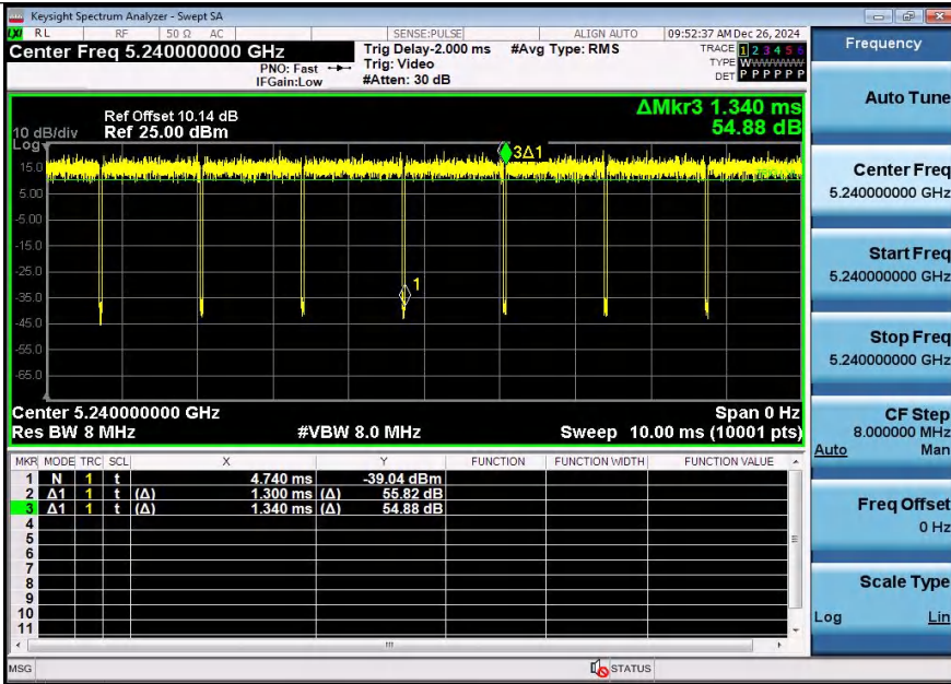
NTNV-11N20SISO-Ant1-5240
