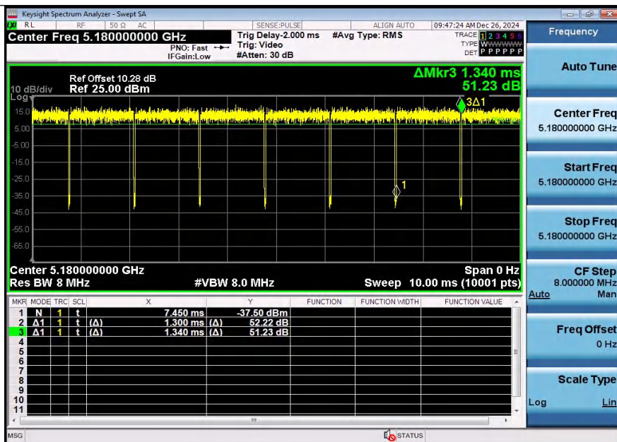
NTNV-11N20SISO-Ant1-5180
