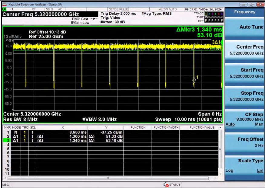
NTNV-11N20SISO-Ant1-5320
