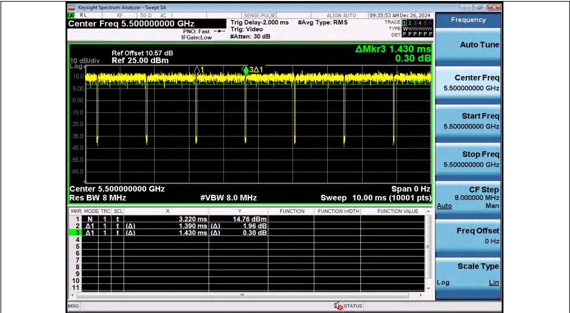
NTNV-11A-Ant1-5500
