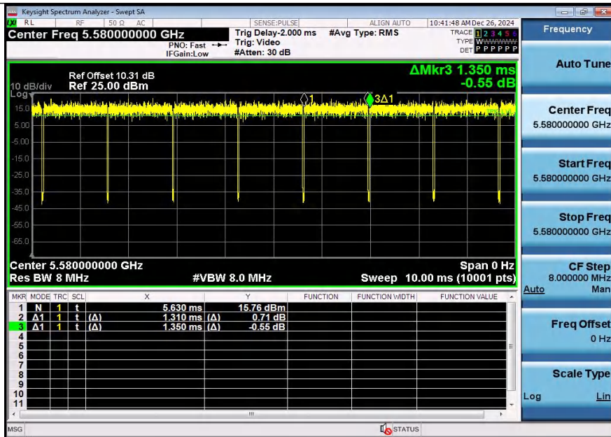
NTNV-11AC20SISO-Ant1-5580
