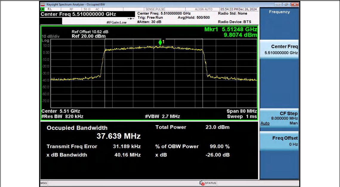
11AX40SISO-Ant2-5510
