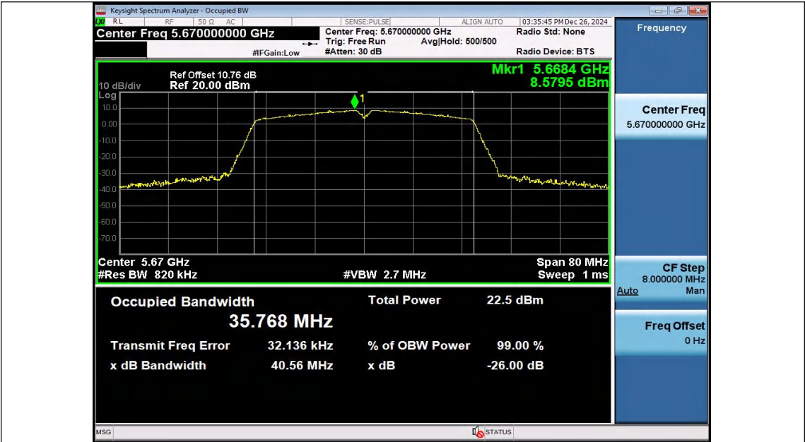
11N40SISO-Ant2-5670
