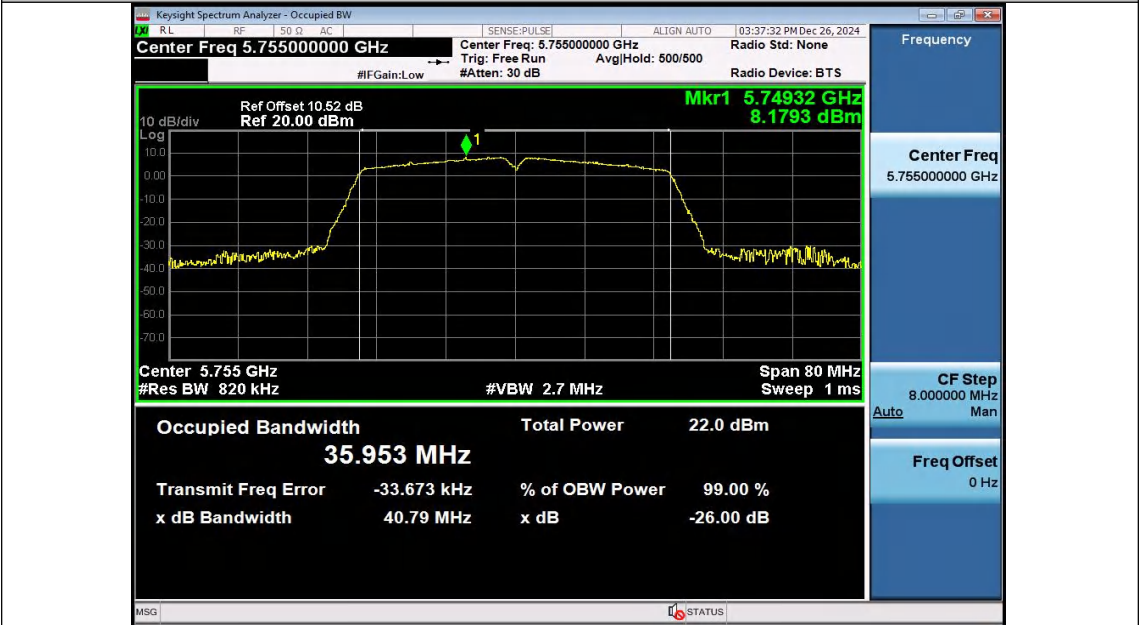
11N40SISO-Ant2-5755
