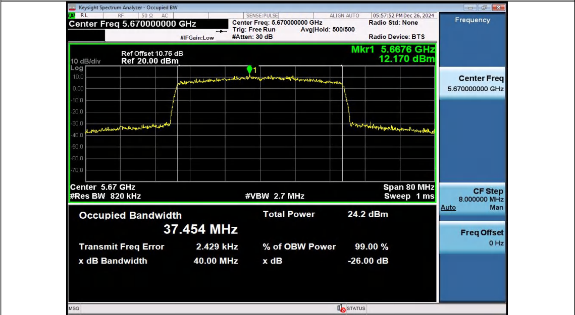
11AX40SISO-Ant2-5670
