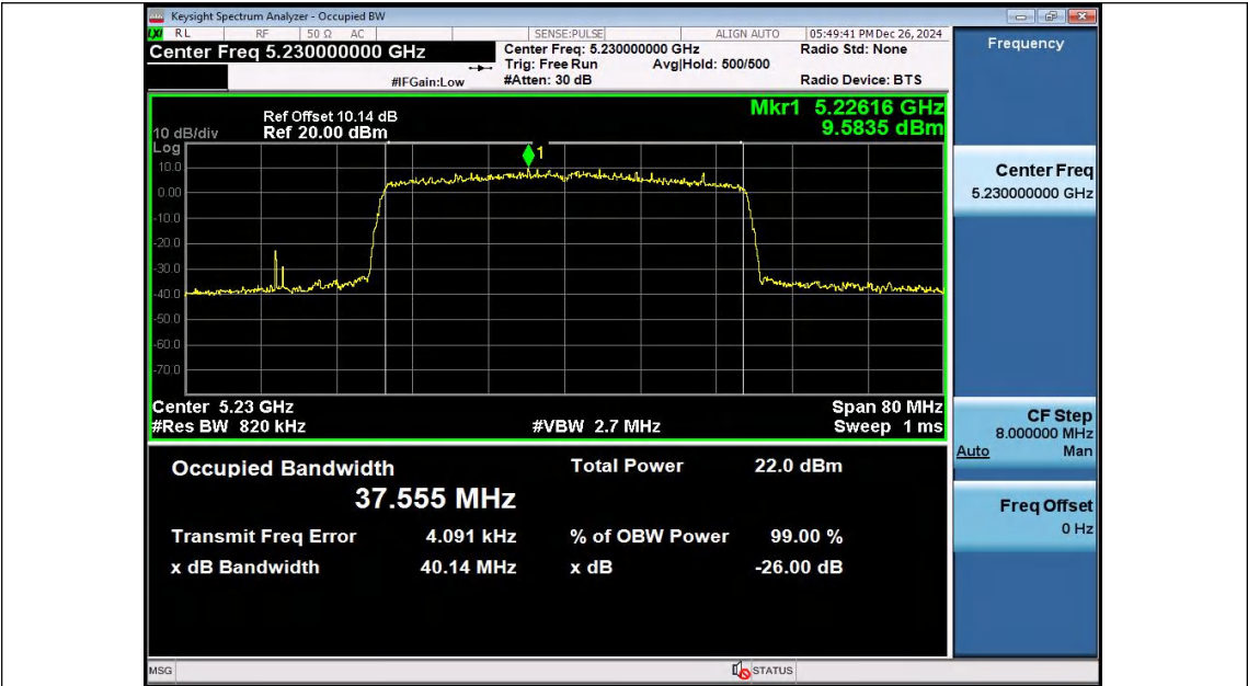
11AX40SISO-Ant2-5230
