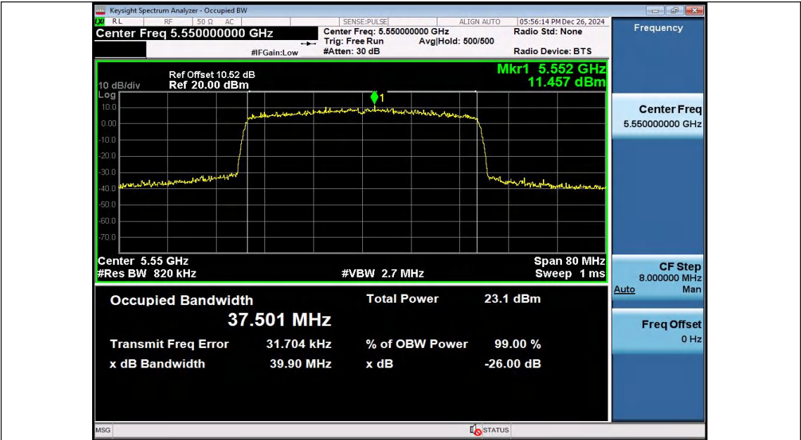
11AX40SISO-Ant2-5550
