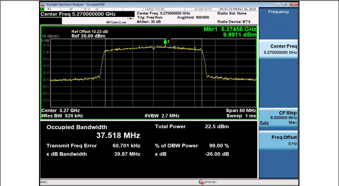
11AX40SISO-Ant2-5270
