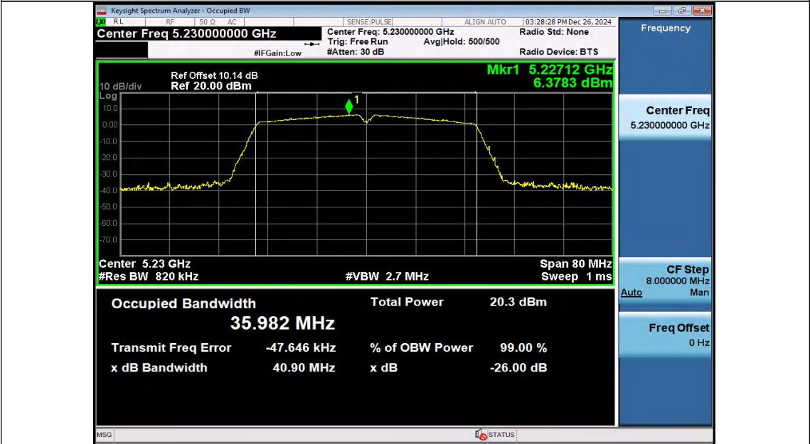
11N40SISO-Ant2-5230
