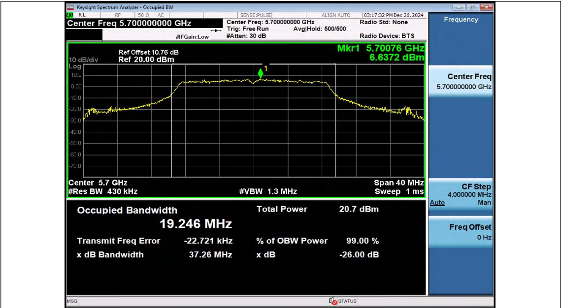
11N20SISO-Ant2-5700
