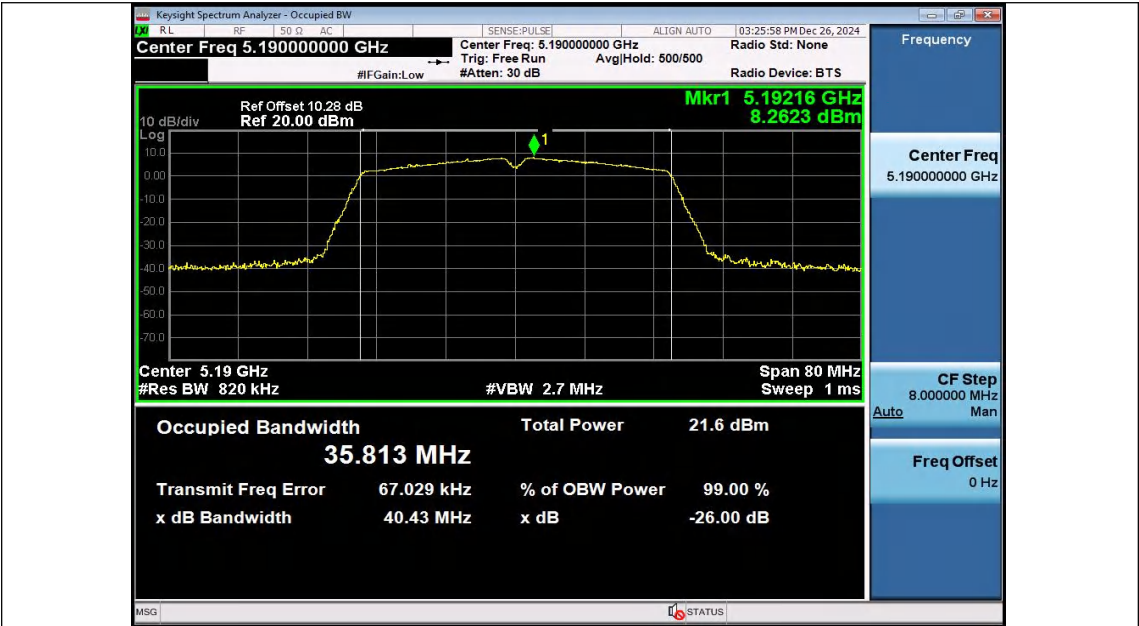
11N40SISO-Ant2-5190
