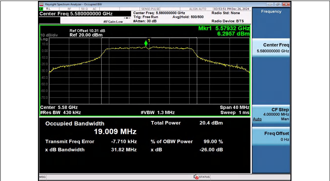
11AC20SISO-Ant2-5580
