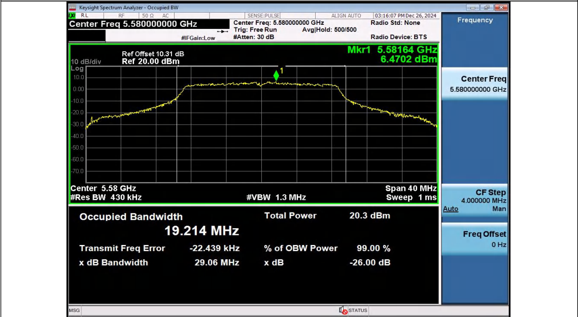
11N20SISO-Ant2-5580
