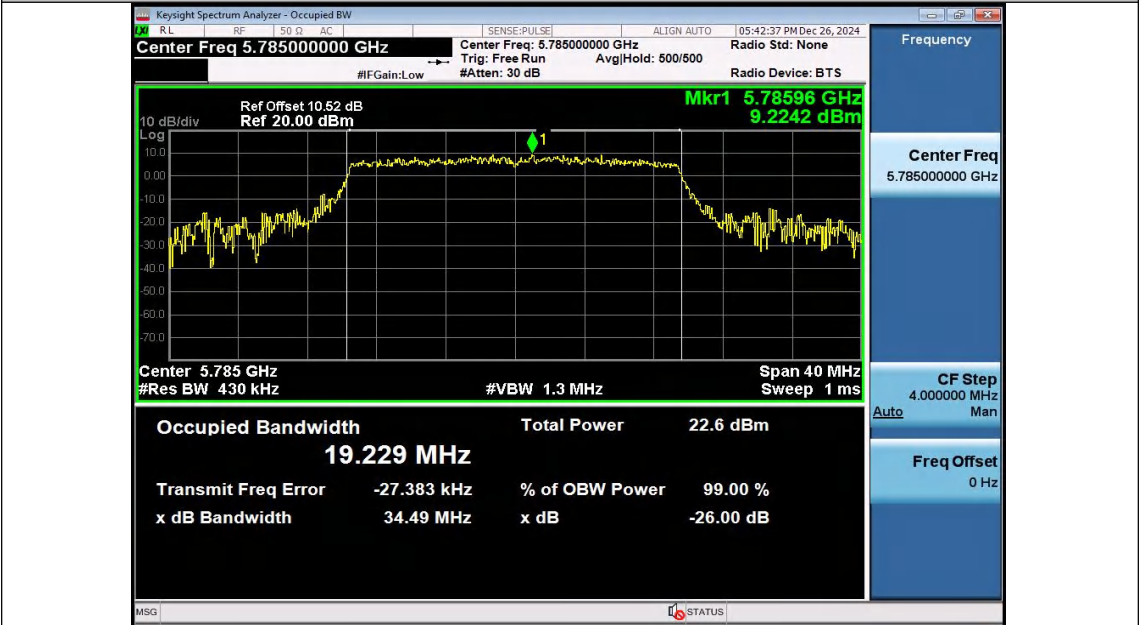
11AX20SISO-Ant2-5785
