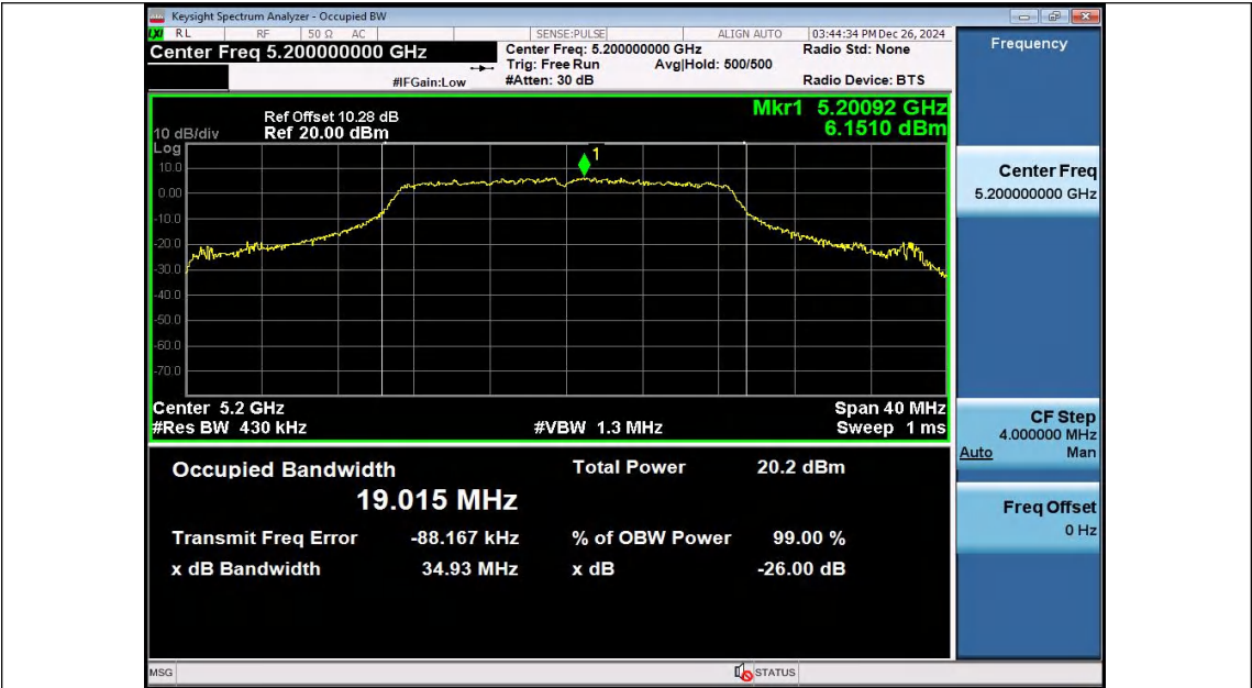
11AC20SISO-Ant2-5200
