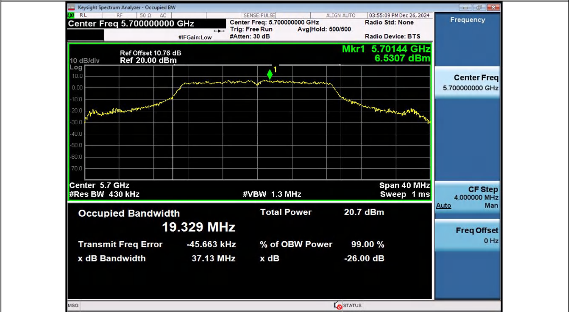
11AC20SISO-Ant2-5700
