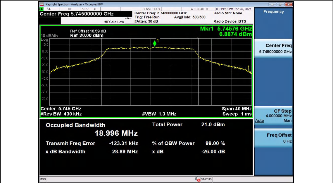
11N20SISO-Ant2-5745
