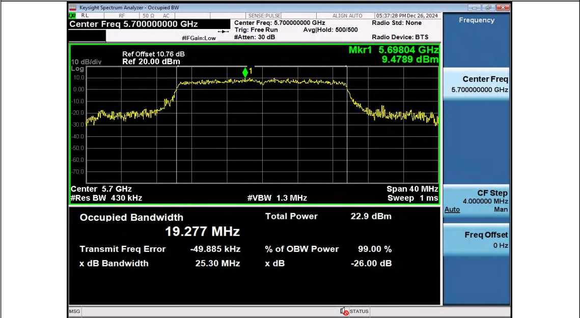
11AX20SISO-Ant2-5700
