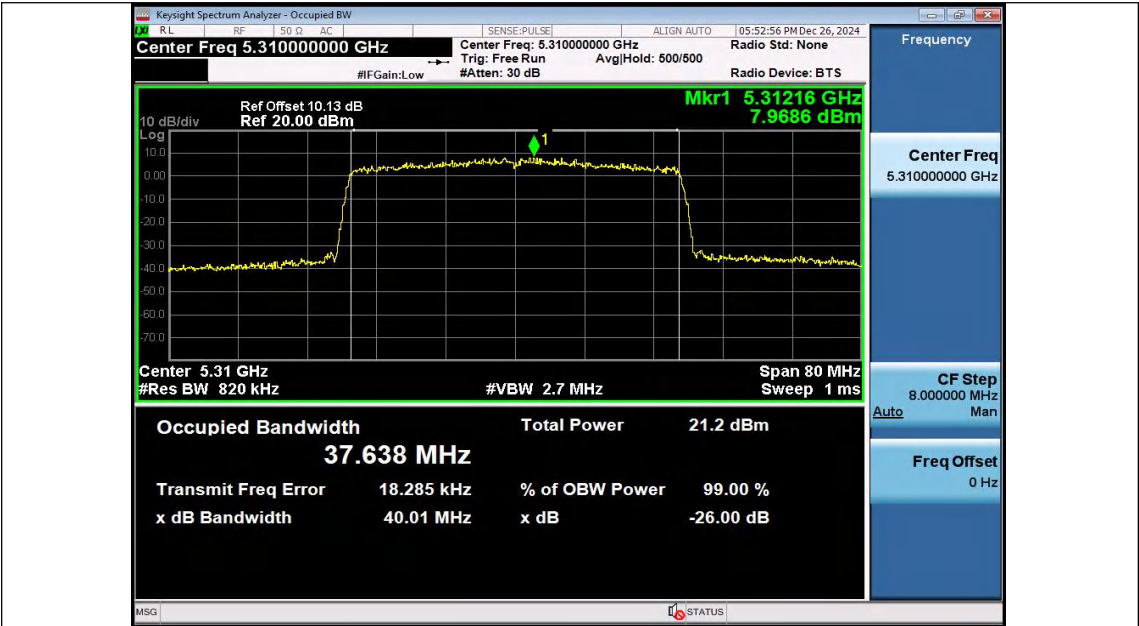
11AX40SISO-Ant2-5310
