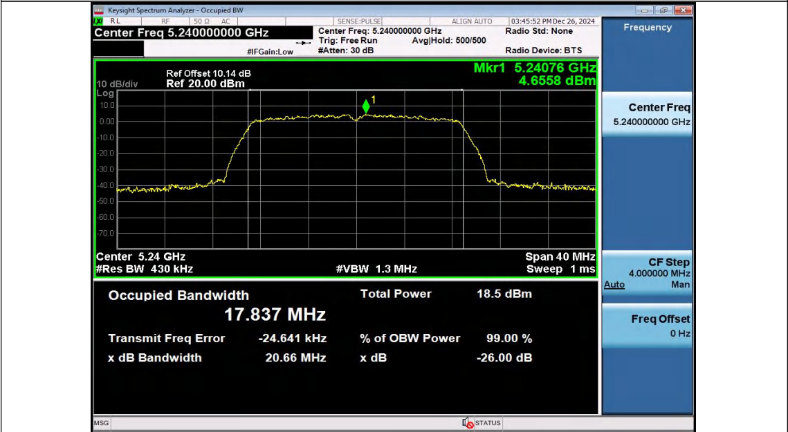
11AC20SISO-Ant2-5240
