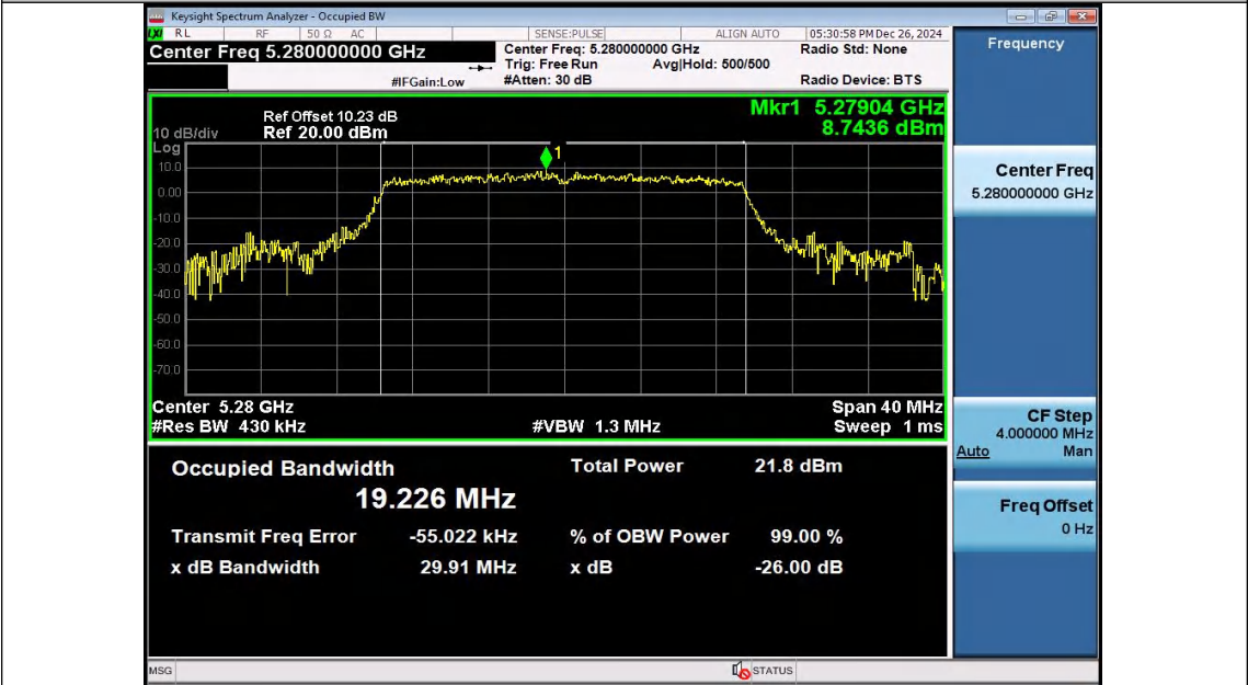
11AX20SISO-Ant2-5280
