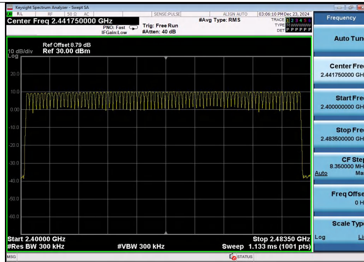
GFSK Modulation
