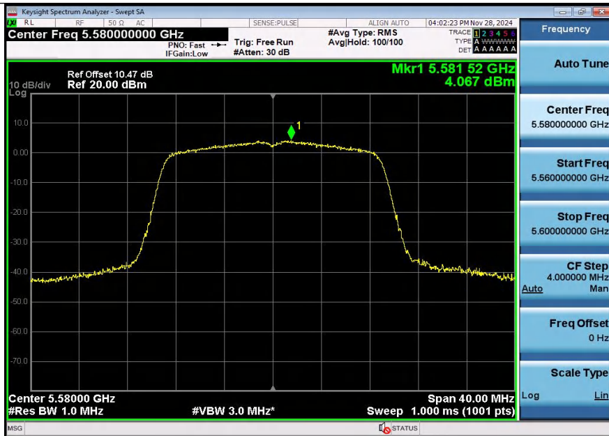
11AC20SISO-Ant2-5580-PASS
