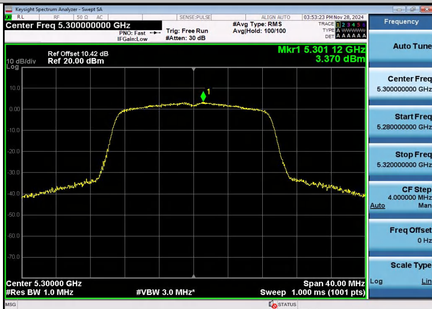
11AC20SISO-Ant2-5300-PASS
