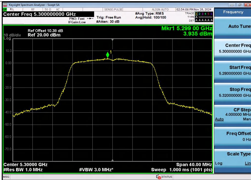
11A-Ant2-5300-PASS
