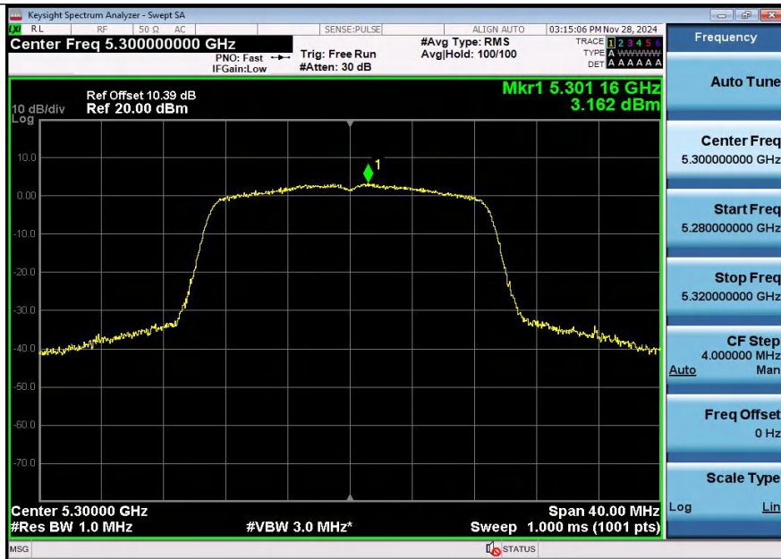
11N20SISO-Ant2-5300-PASS
