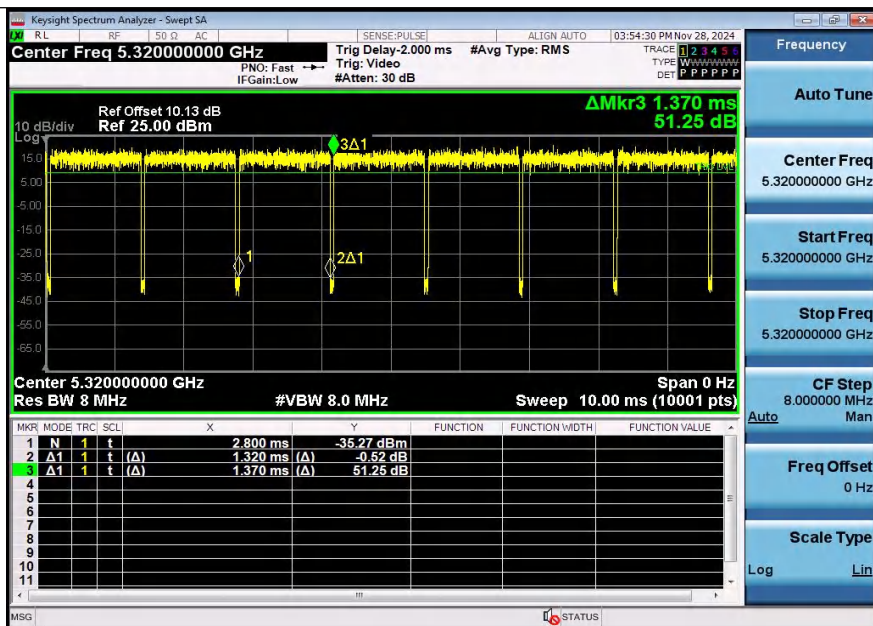
NTNV-11AC20SISO-Ant2-5320
