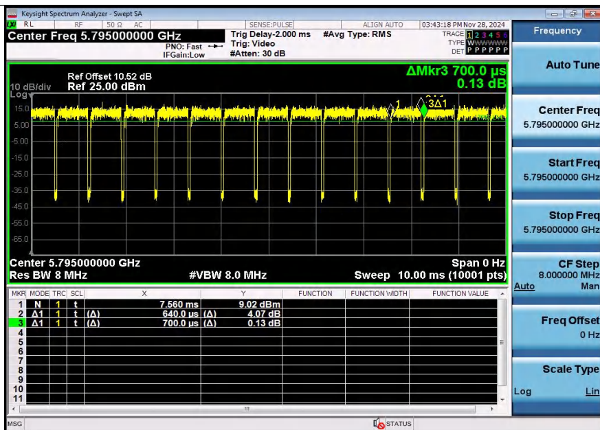
NTNV-11N40SISO-Ant2-5795
