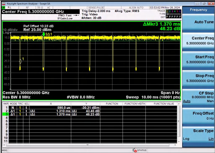
NTNV-11AC20SISO-Ant2-5300
