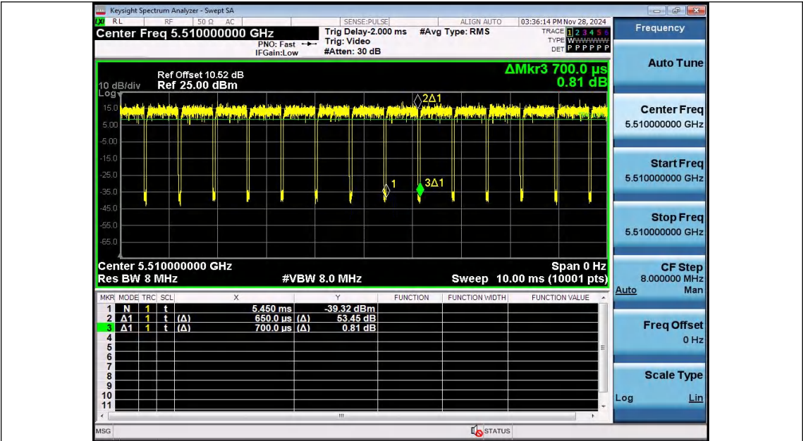
NTNV-11N40SISO-Ant2-5510
