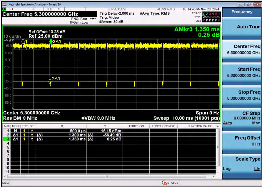
NTNV-11N20SISO-Ant2-5300
