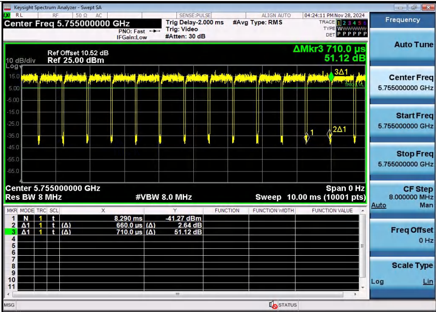
NTNV-11AC40SISO-Ant2-5755
