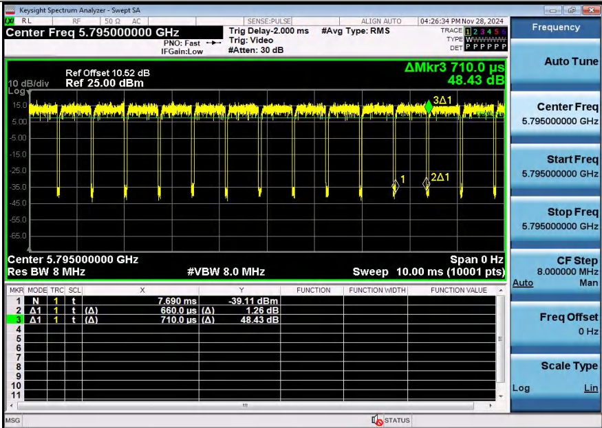
NTNV-11AC40SISO-Ant2-5795
