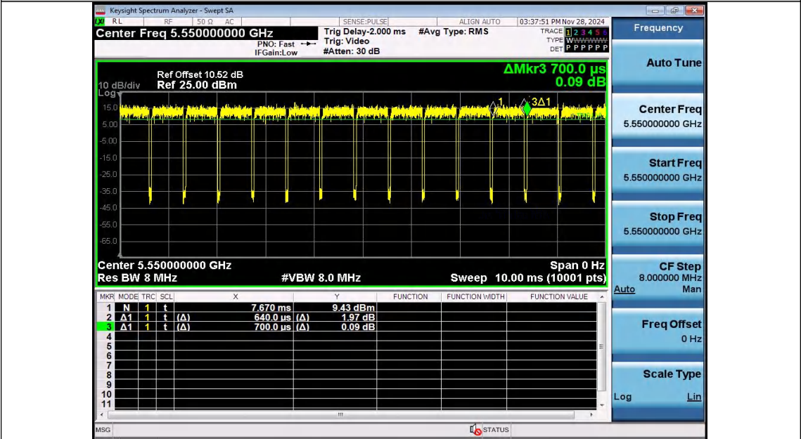
NTNV-11N40SISO-Ant2-5550
