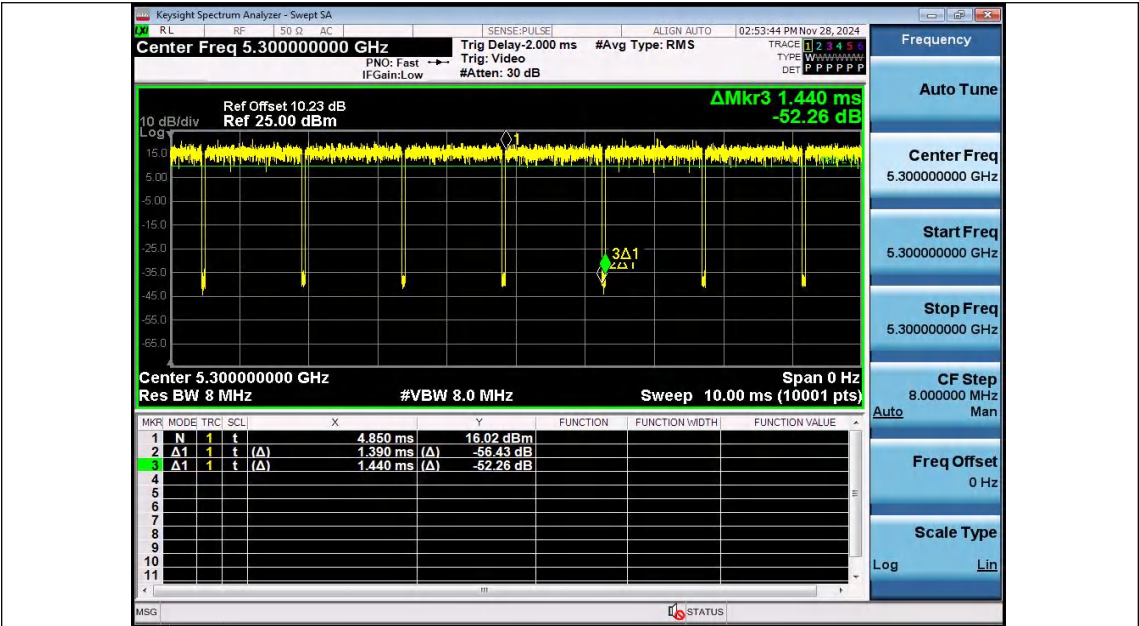
NTNV-11A-Ant2-5300
