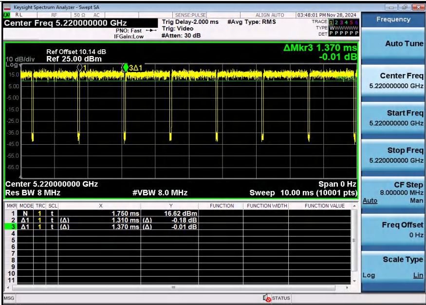
NTNV-11AC20SISO-Ant2-5220
