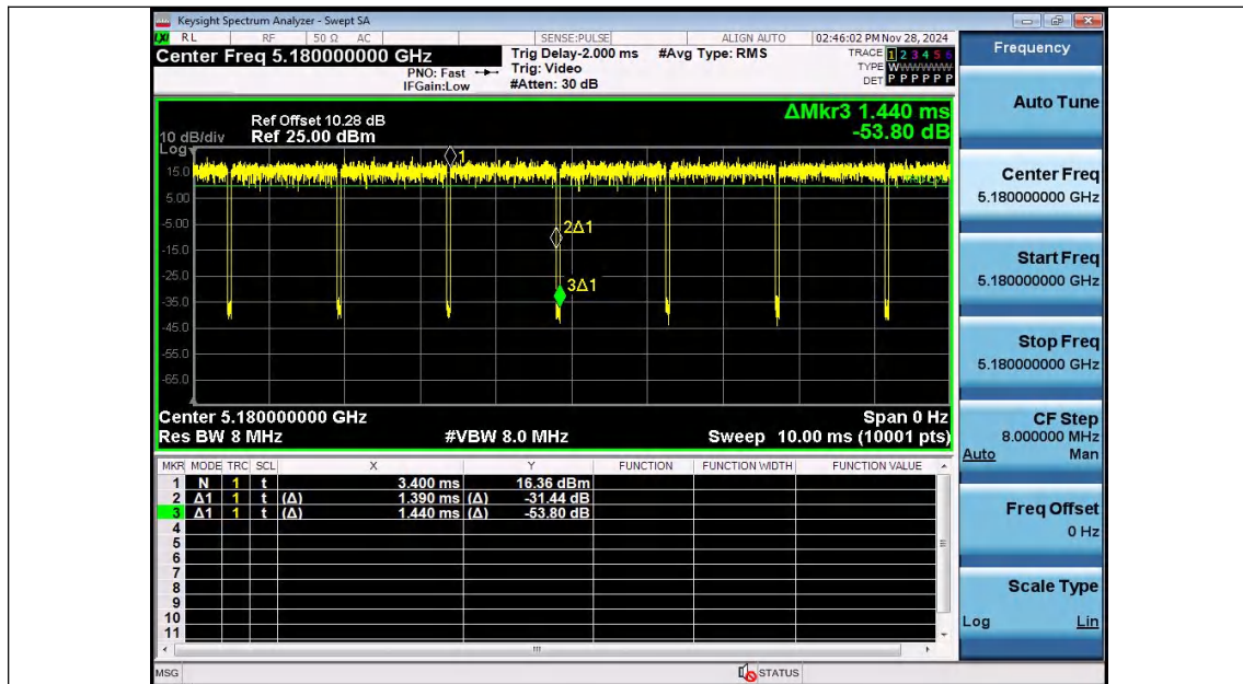
NTNV-11A-Ant2-5180
