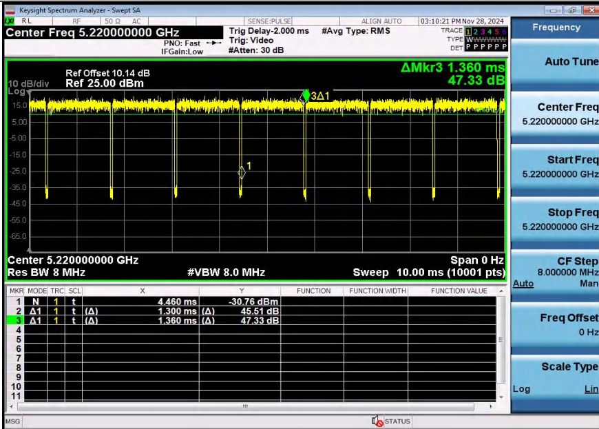
NTNV-11N20SISO-Ant2-5220
