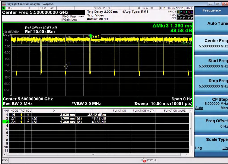
NTNV-11N20SISO-Ant2-5500
