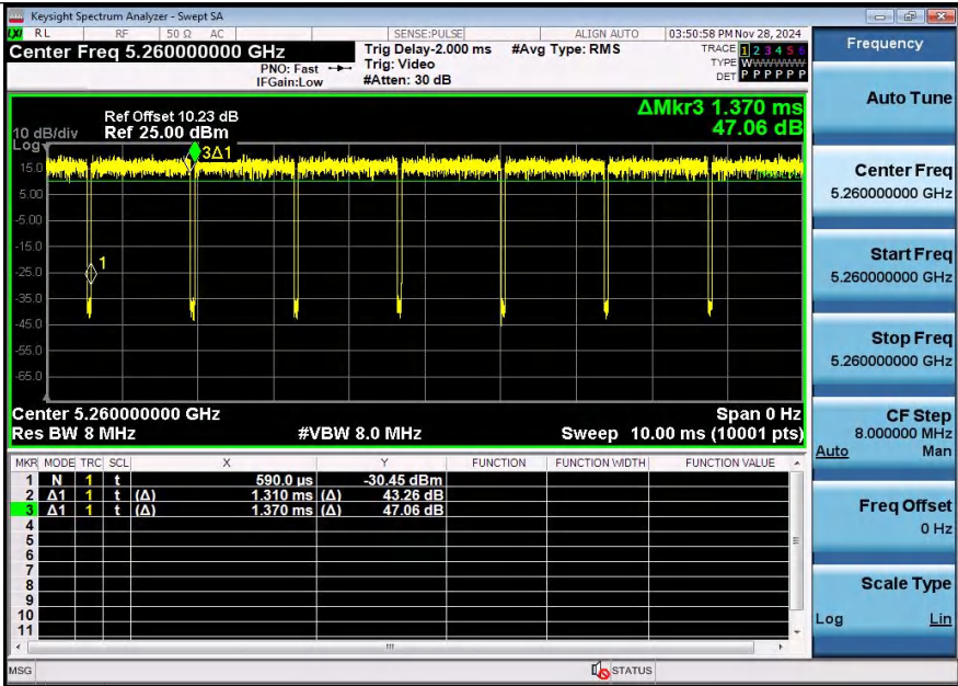
NTNV-11AC20SISO-Ant2-5260
