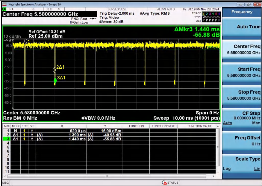
NTNV-11A-Ant2-5580
