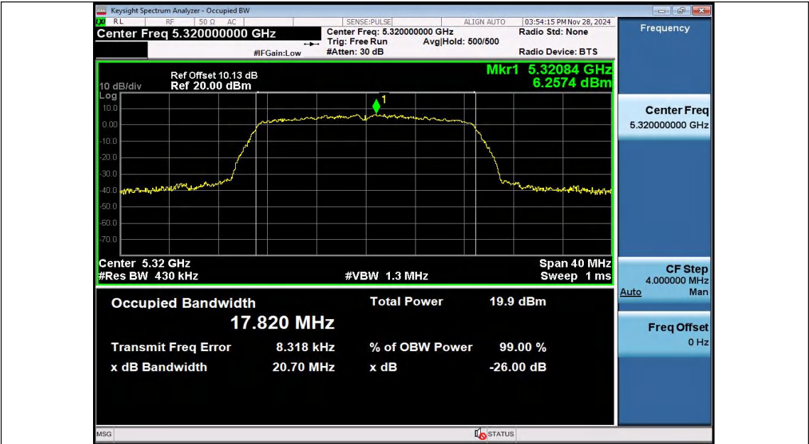
11AC20SISO-Ant2-5320
