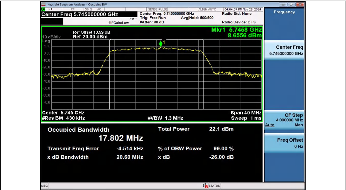
11AC20SISO-Ant2-5745
