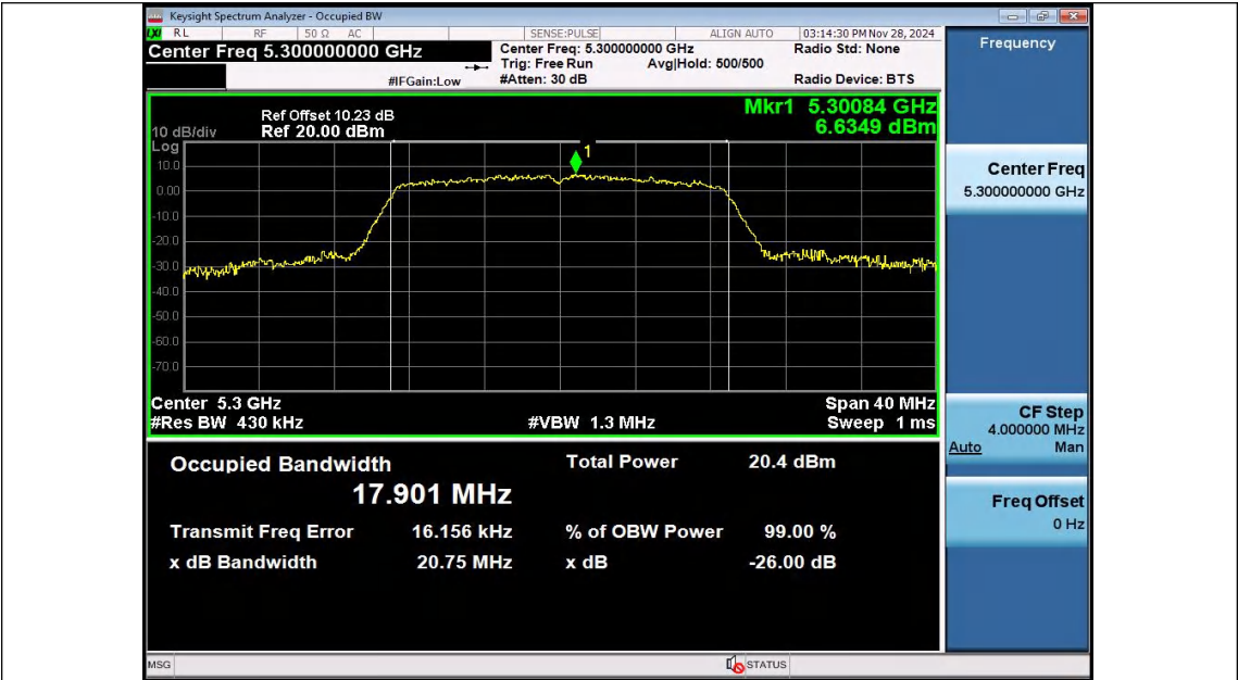
11N20SISO-Ant2-5300
