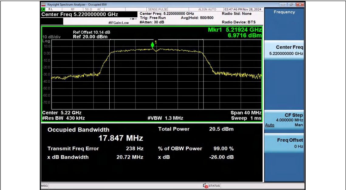
11AC20SISO-Ant2-5220
