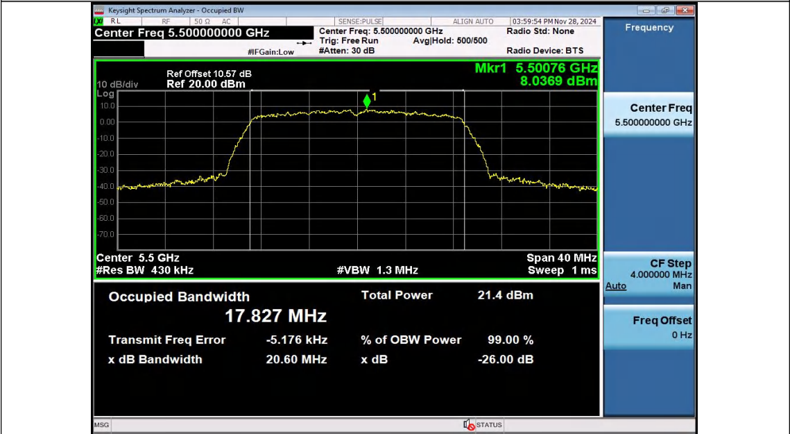
11AC20SISO-Ant2-5500
