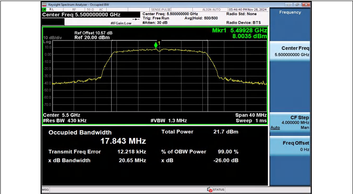
11N20SISO-Ant1-5500
