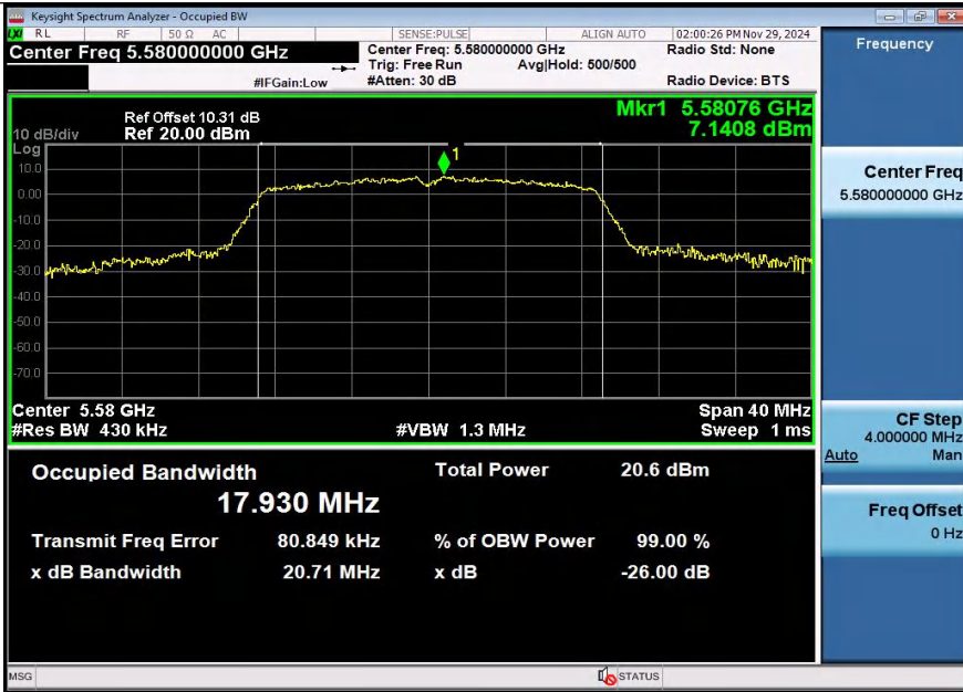
11AC20SISO-Ant1-5580
