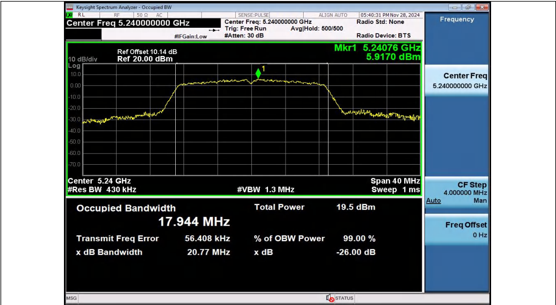
11N20SISO-Ant1-5240
