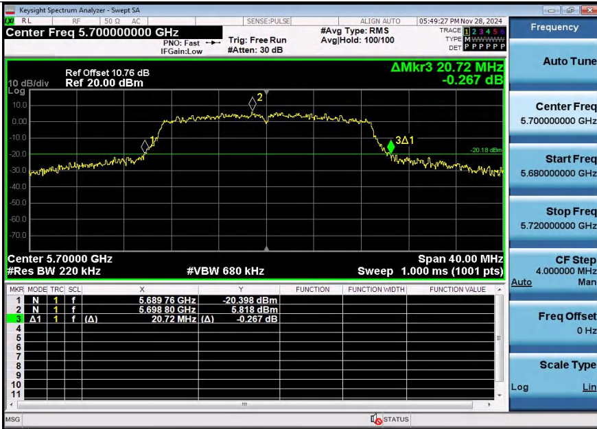
11N20SISO-Ant1-5700
