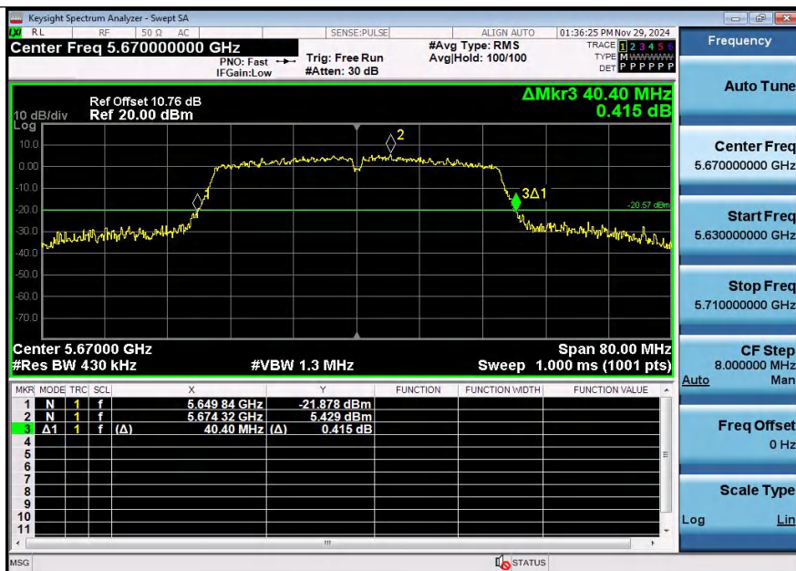
11N40SISO-Ant1-5670
