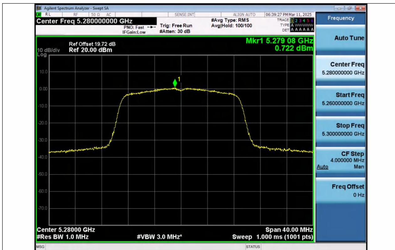
11N20MIMO-Ant1-5280-PASS
