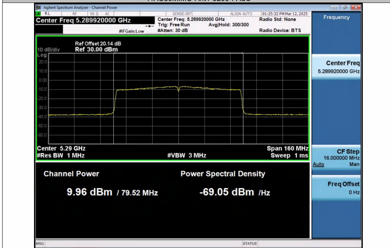
11AC80MIMO-Ant2-5290-PASS
