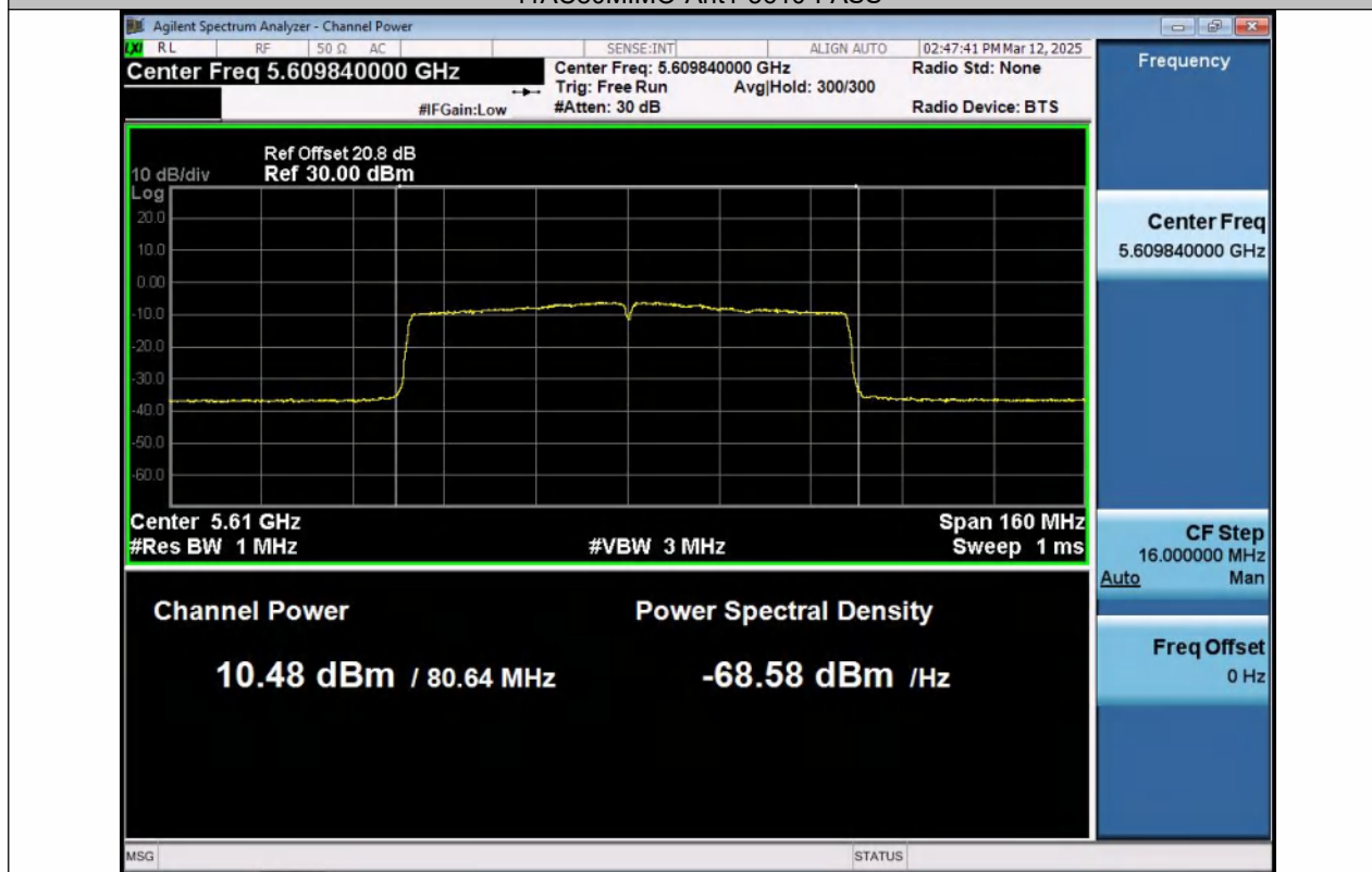
11AC80MIMO-Ant2-5610-PASS
