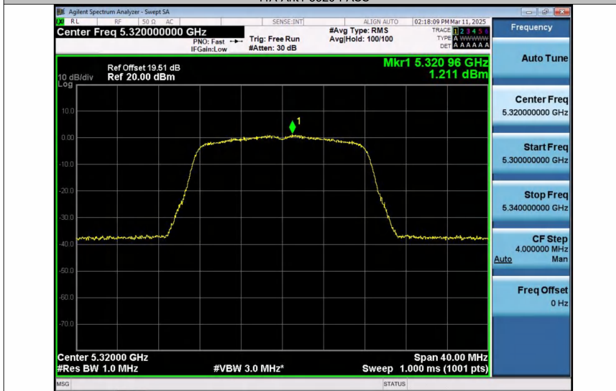
11A-Ant2-5320-PASS
