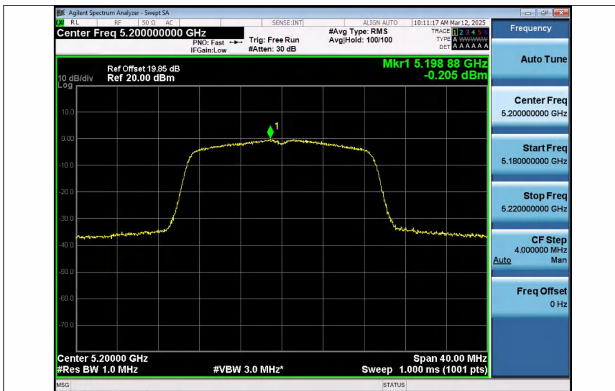
11AC20MIMO-Ant1-5200-PASS
