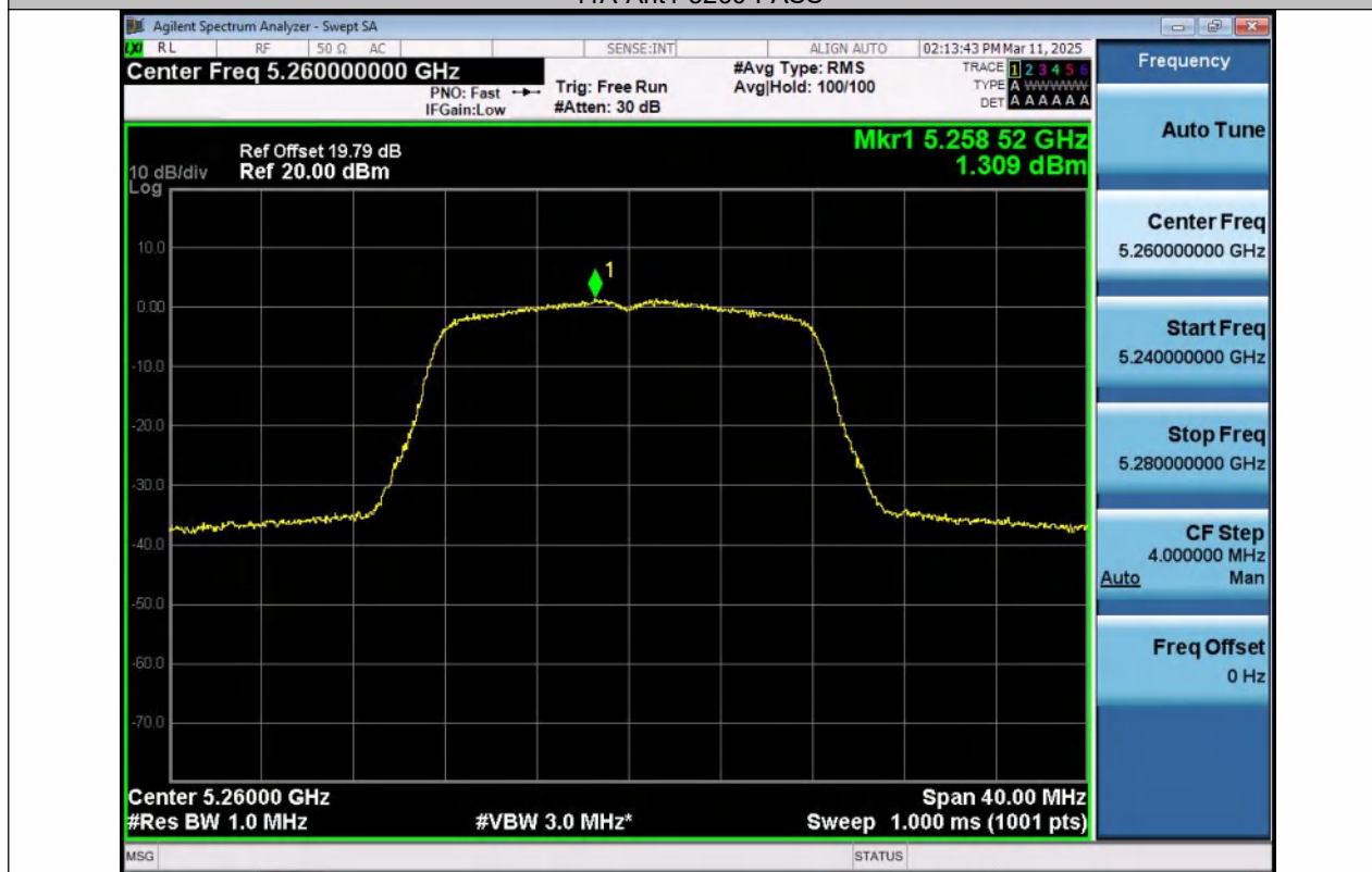
11A-Ant2-5260-PASS
