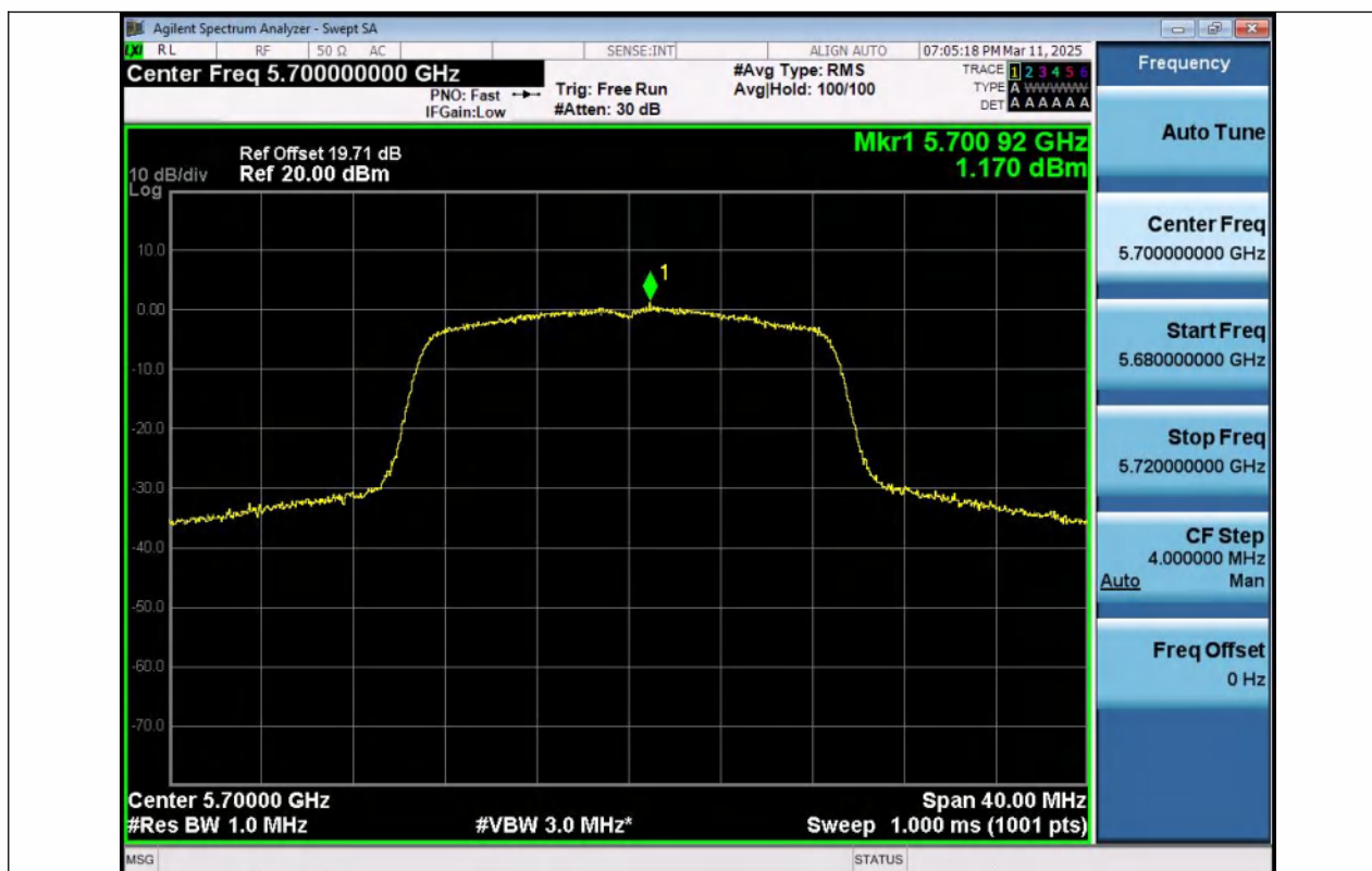
11N20MIMO-Ant1-5700-PASS
