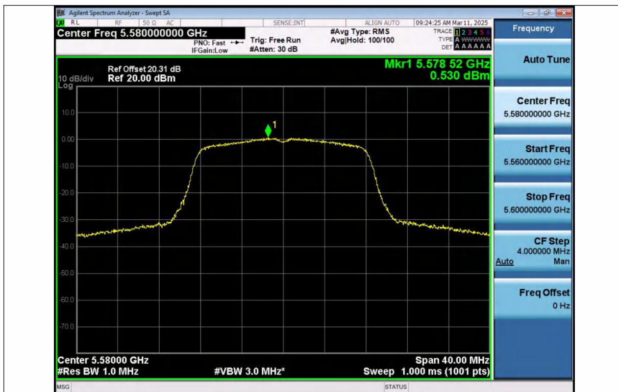
11A-Ant1-5580-PASS
