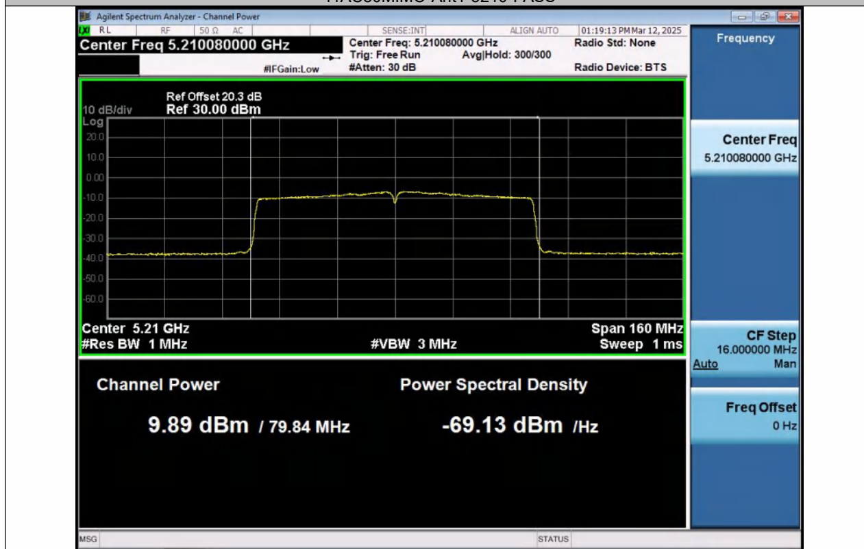
11AC80MIMO-Ant2-5210-PASS
