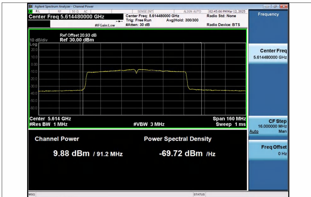
11AC80MIMO-Ant1-5610-PASS
