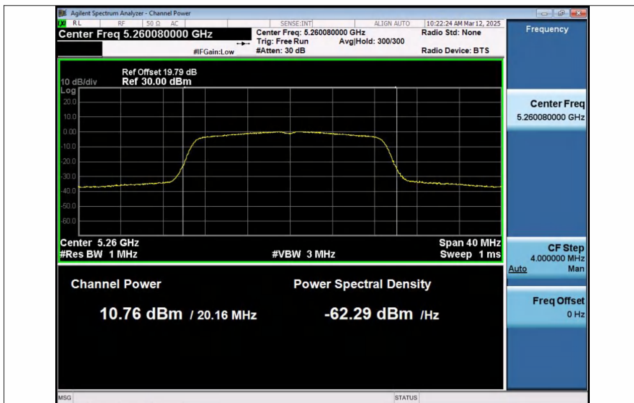
11AC20MIMO-Ant1-5260-PASS
