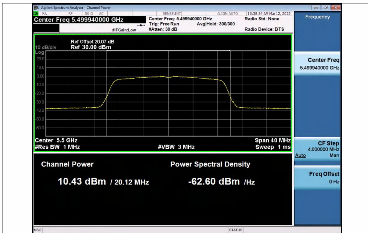
11AC20MIMO-Ant1-5500-PASS
