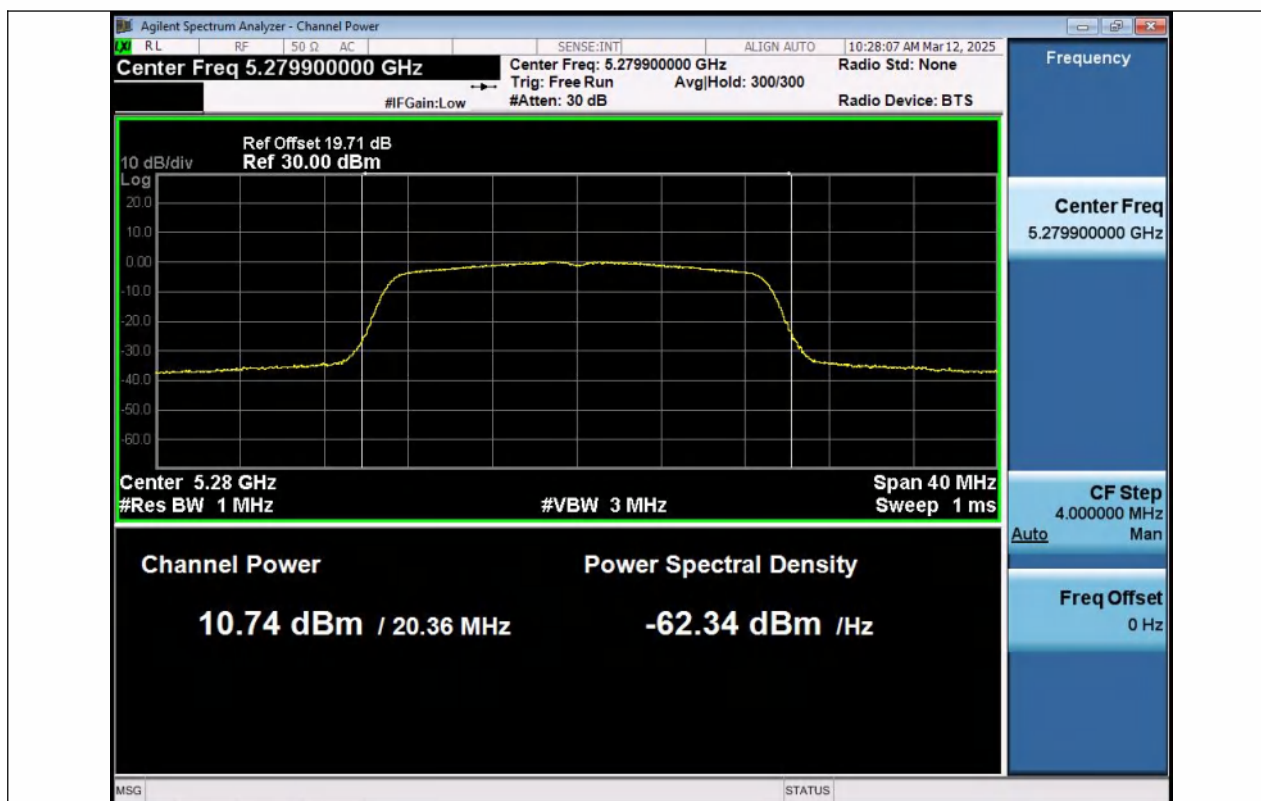
11AC20MIMO-Ant1-5280-PASS
