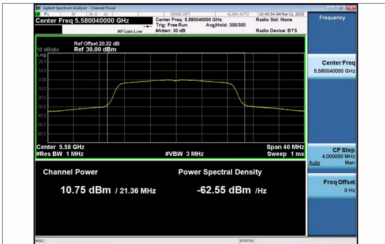
11AC20MIMO-Ant1-5580-PASS
