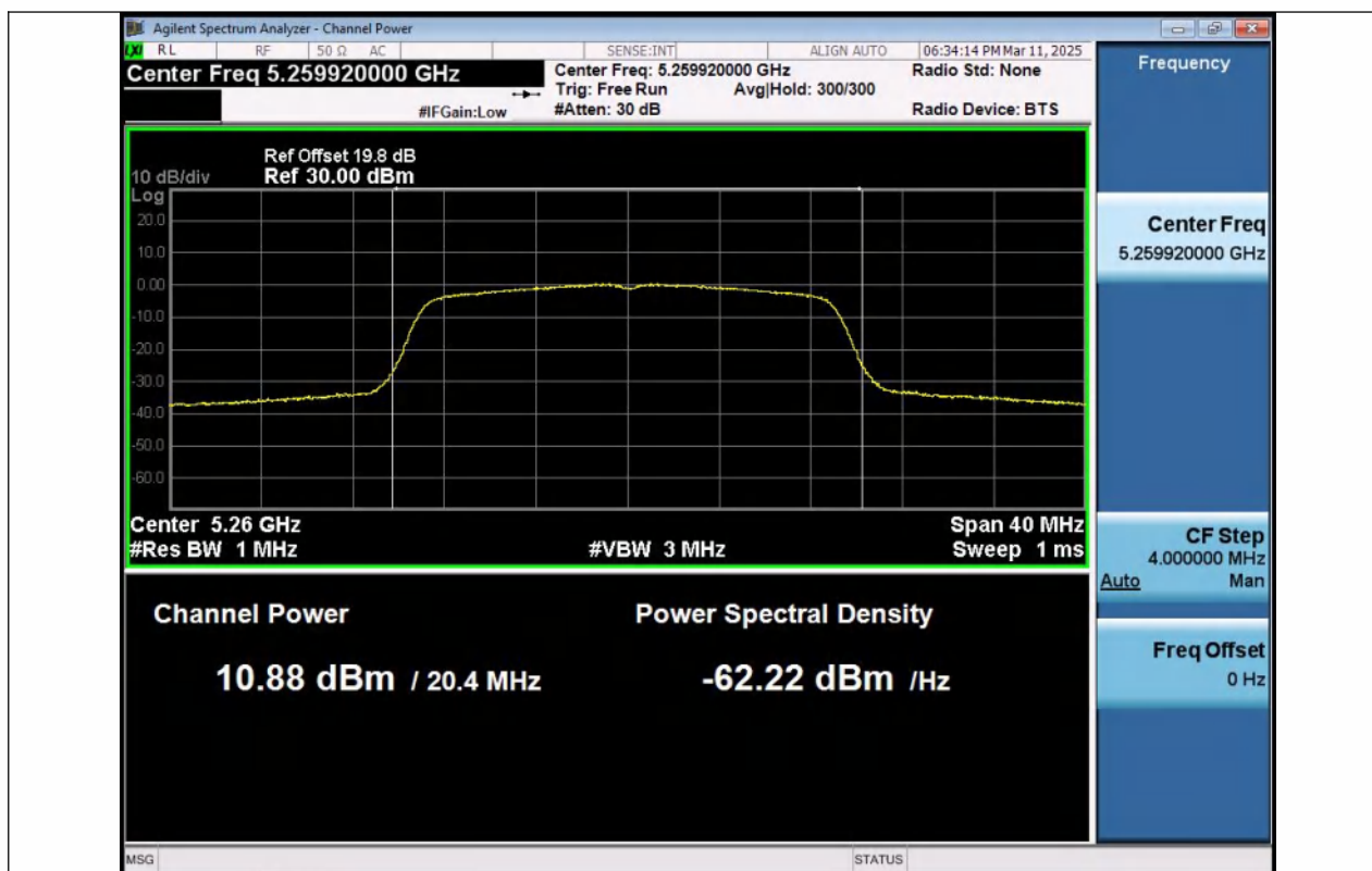
11N20MIMO-Ant1-5260-PASS
