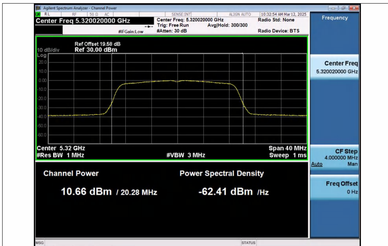
11AC20MIMO-Ant1-5320-PASS
