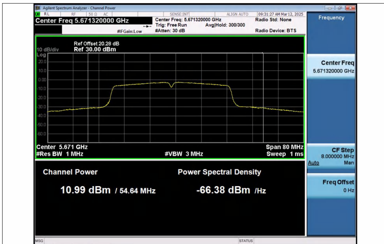
11N40MIMO-Ant1-5670-PASS
