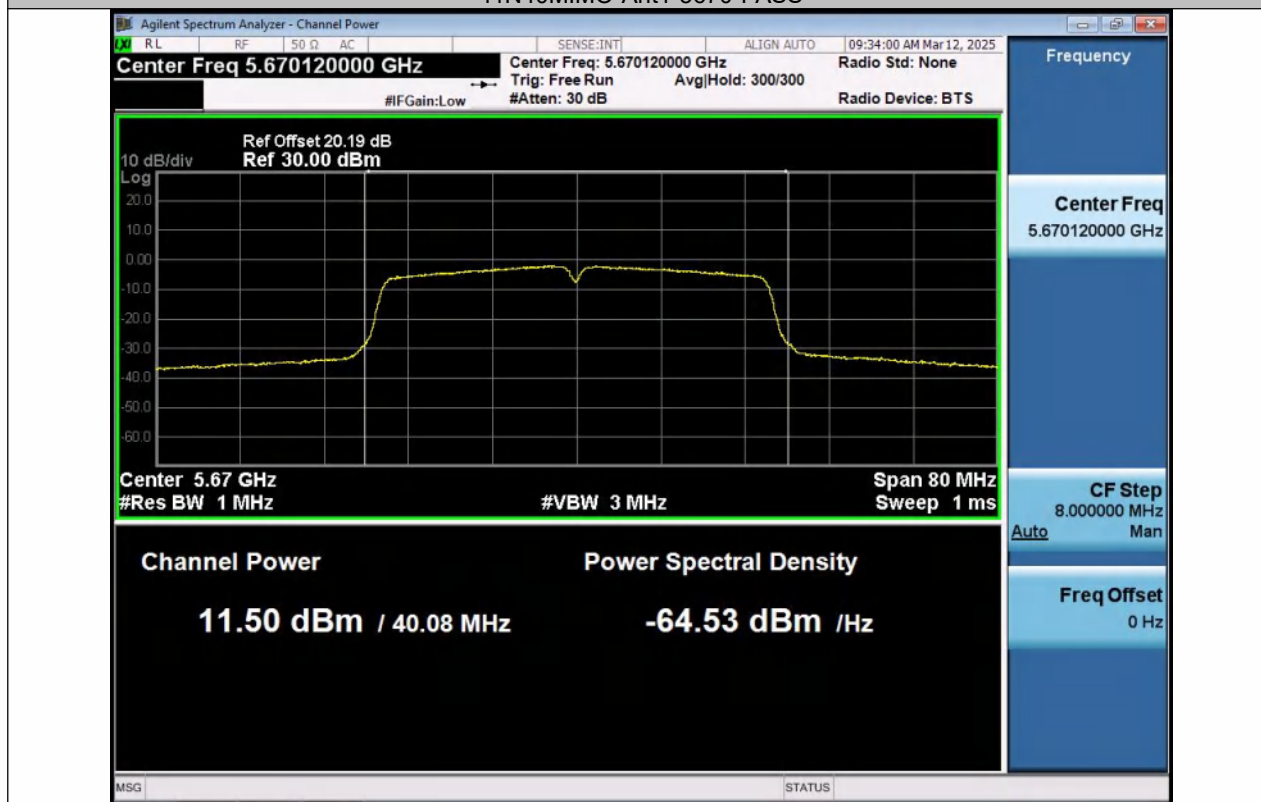
11N40MIMO-Ant2-5670-PASS
