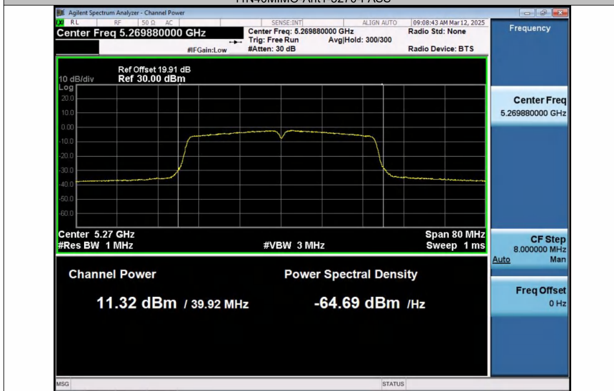
11N40MIMO-Ant2-5270-PASS
