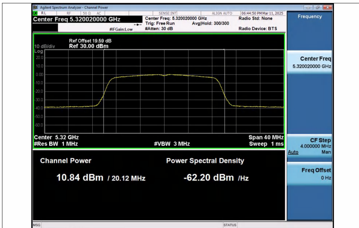
11N20MIMO-Ant1-5320-PASS
