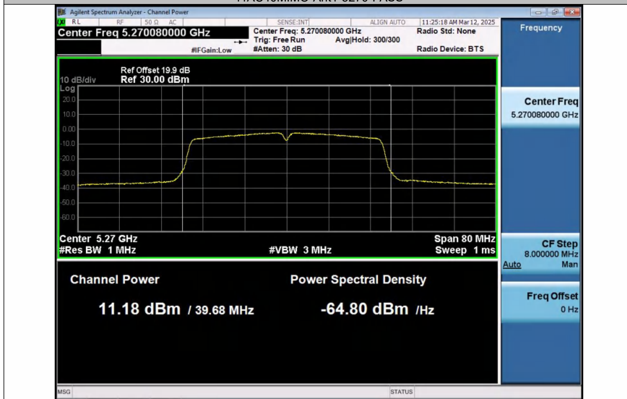
11AC40MIMO-Ant2-5270-PASS
