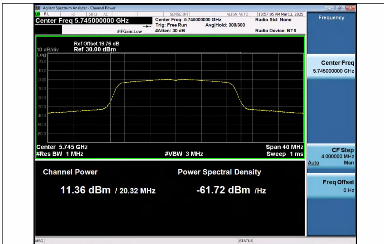
11AC20MIMO-Ant1-5745-PASS
