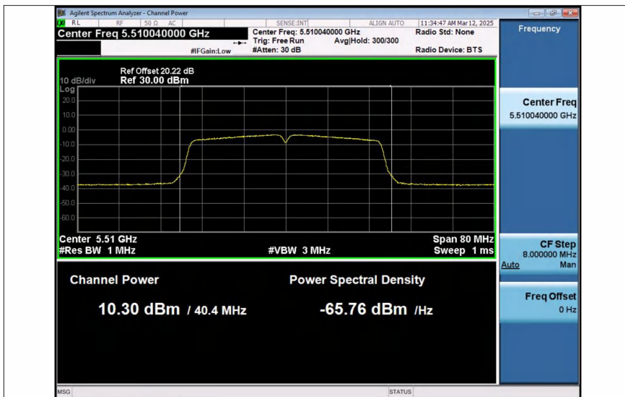
11AC40MIMO-Ant1-5510-PASS
