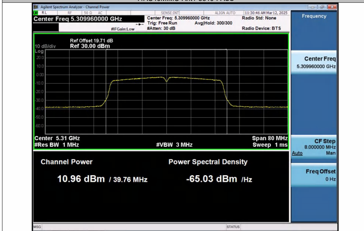
11AC40MIMO-Ant2-5310-PASS
