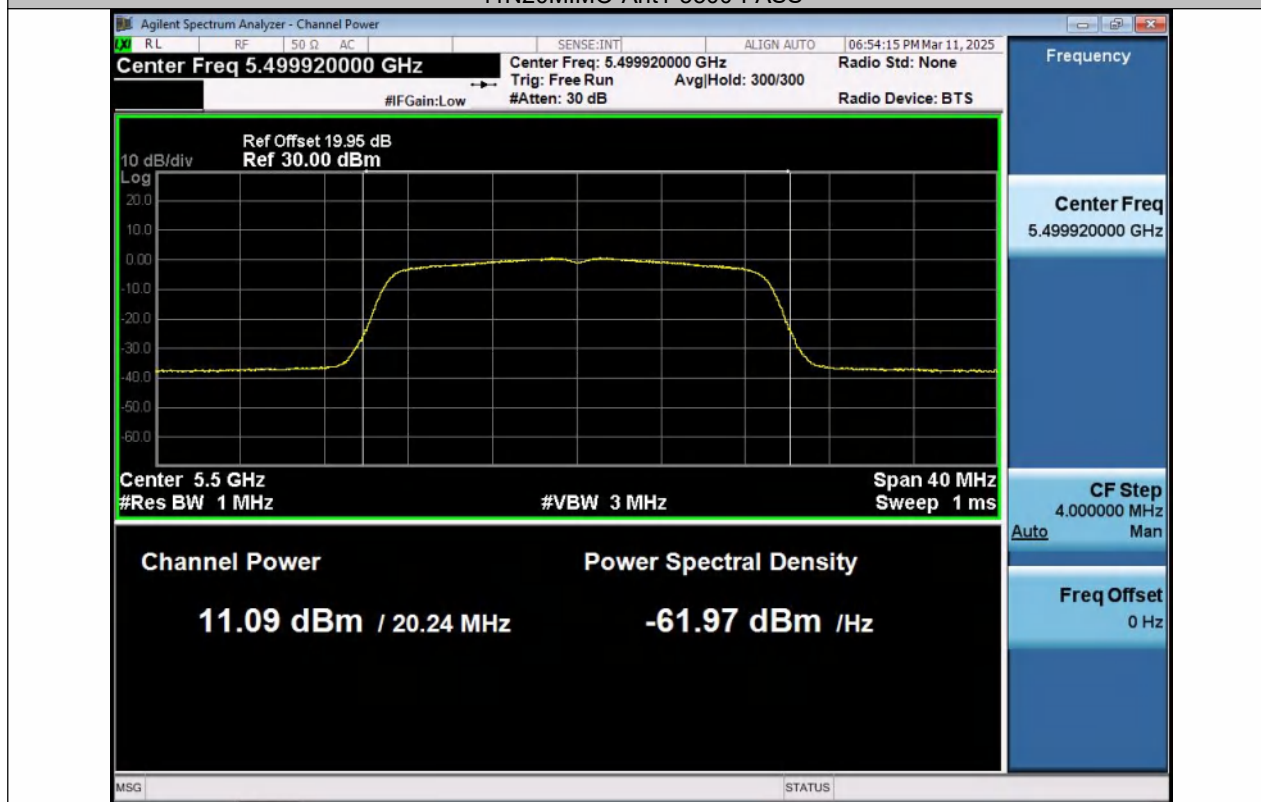
11N20MIMO-Ant2-5500-PASS
