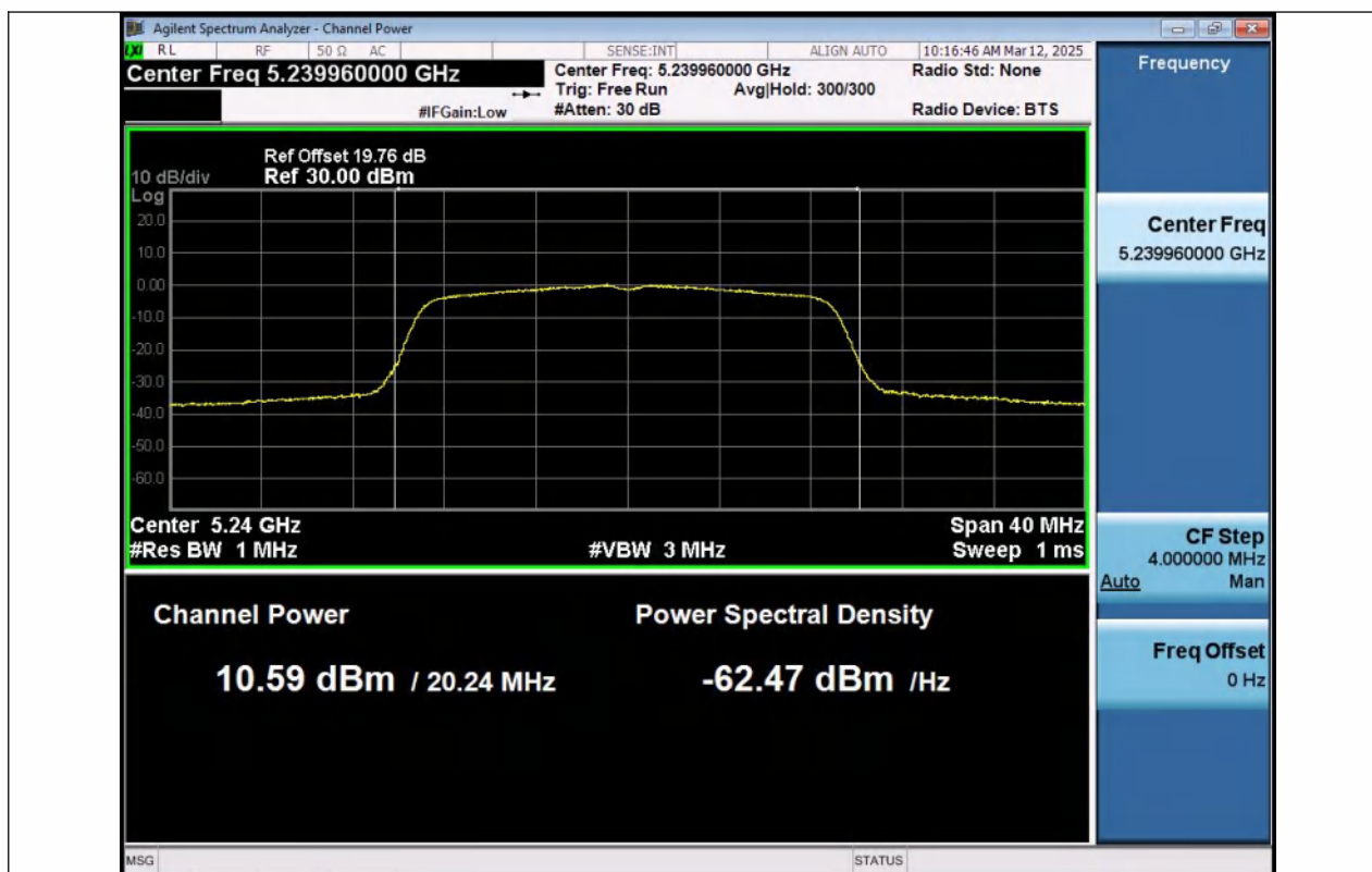
11AC20MIMO-Ant1-5240-PASS
