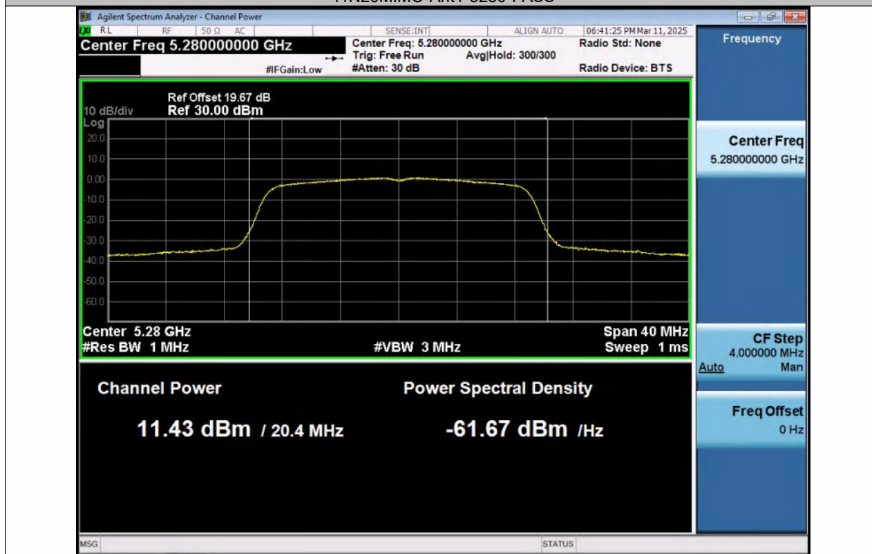
11N20MIMO-Ant2-5280-PASS
