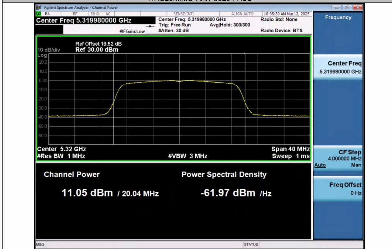
11AC20MIMO-Ant2-5320-PASS
