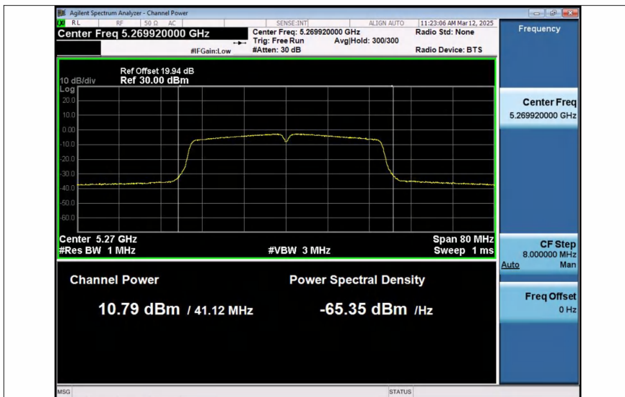
11AC40MIMO-Ant1-5270-PASS
