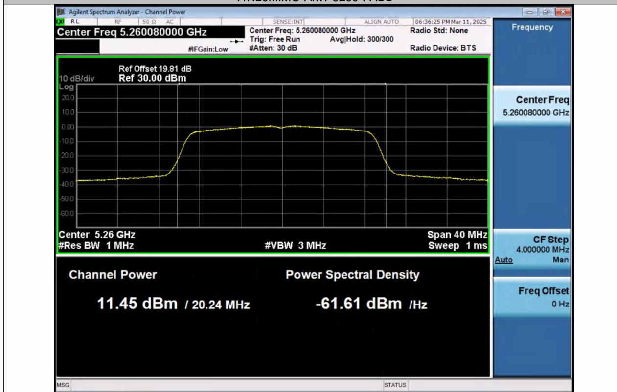
11N20MIMO-Ant2-5260-PASS
