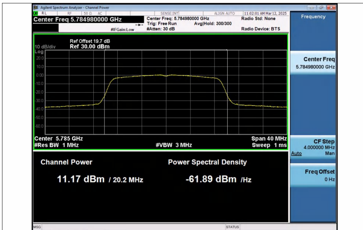
11AC20MIMO-Ant1-5785-PASS
