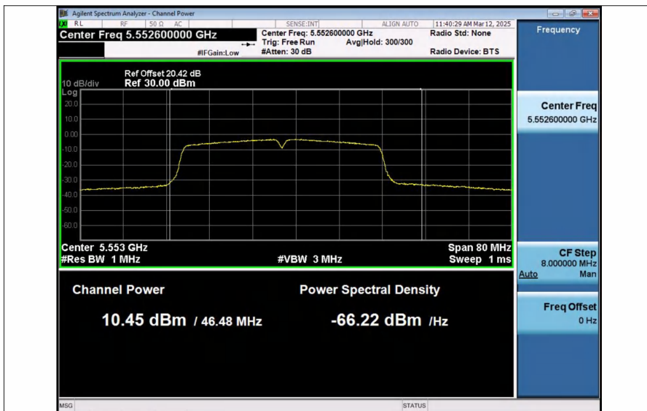
11AC40MIMO-Ant1-5550-PASS
