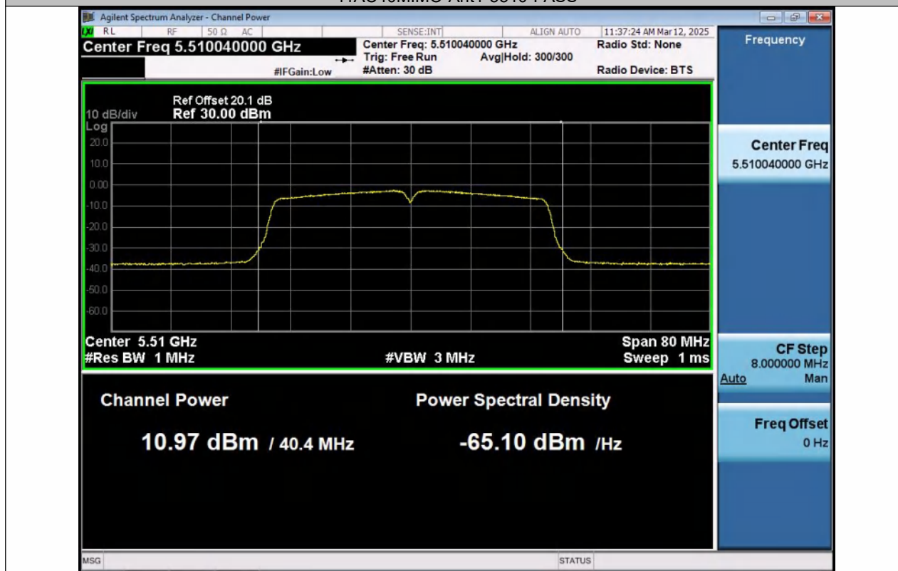
11AC40MIMO-Ant2-5510-PASS
