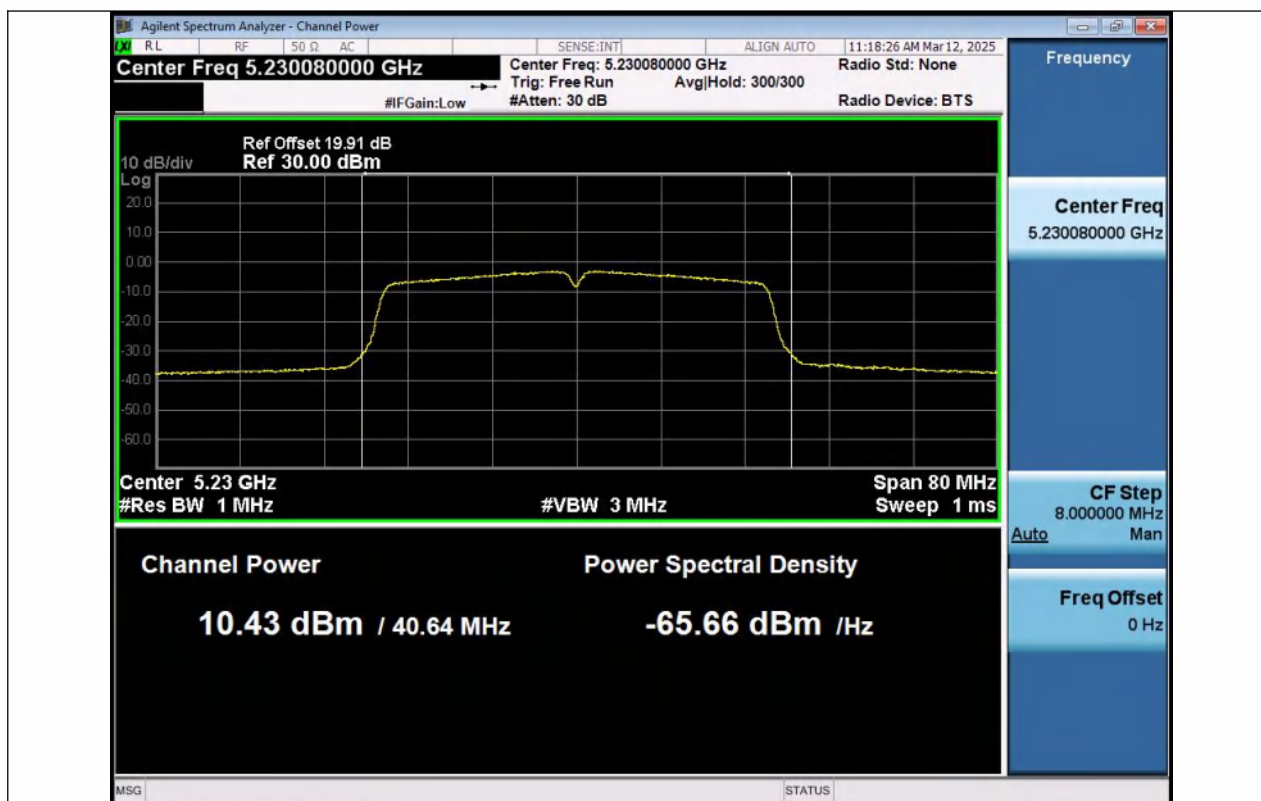
11AC40MIMO-Ant1-5230-PASS
