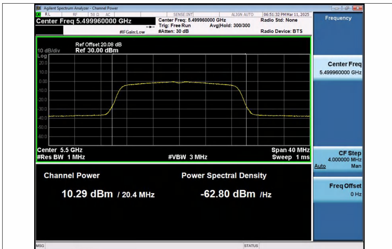
11N20MIMO-Ant1-5500-PASS
