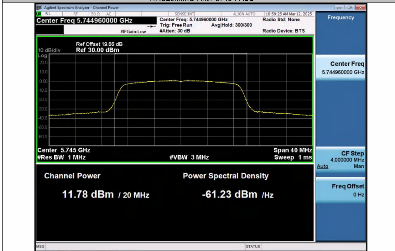
11AC20MIMO-Ant2-5745-PASS
