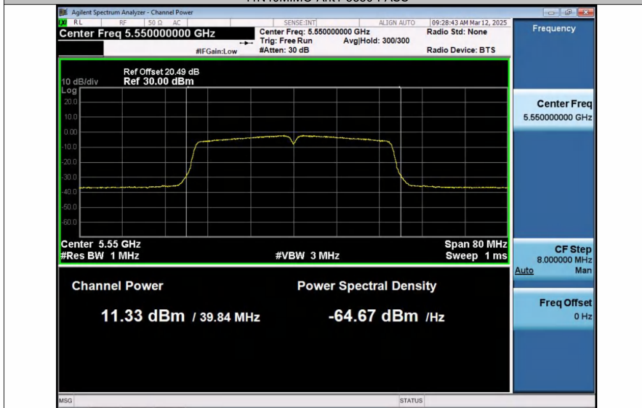
11N40MIMO-Ant2-5550-PASS
