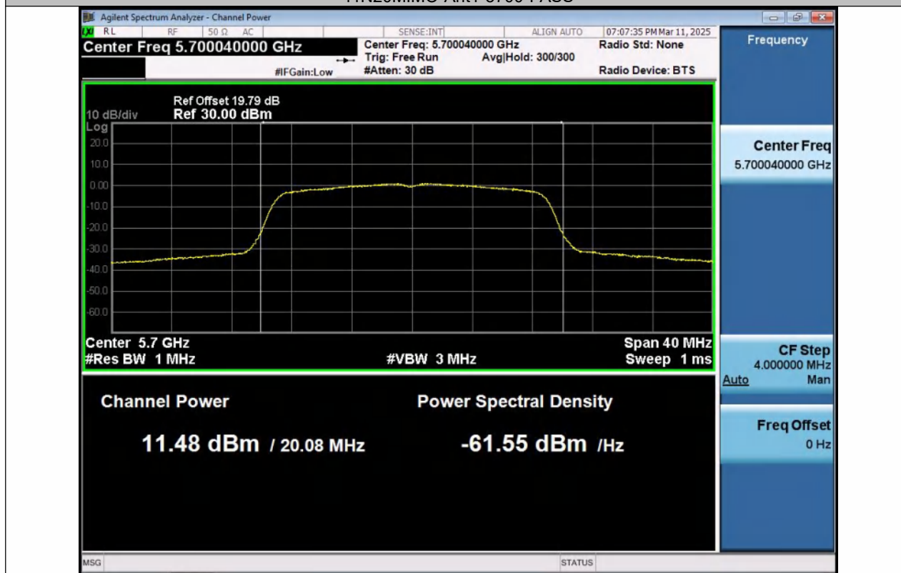
11N20MIMO-Ant2-5700-PASS
