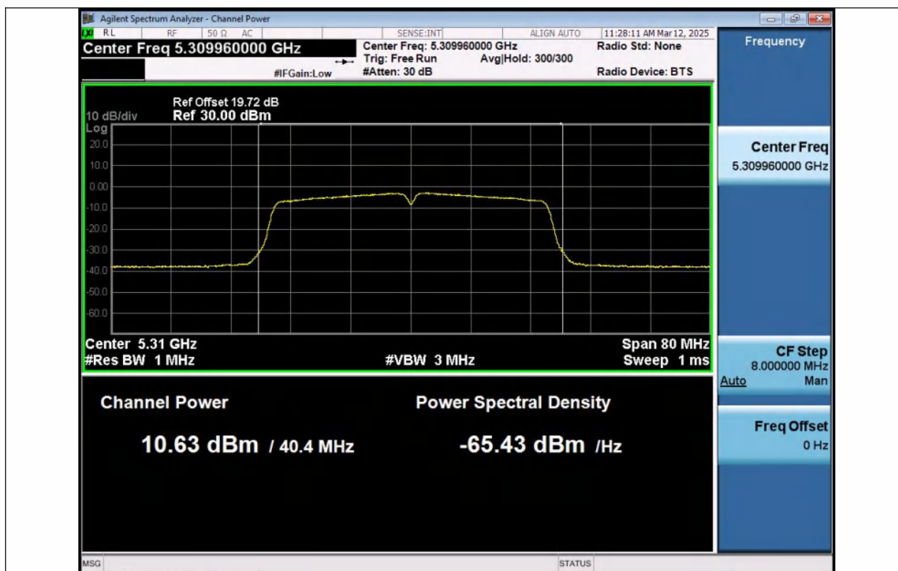
11AC40MIMO-Ant1-5310-PASS
