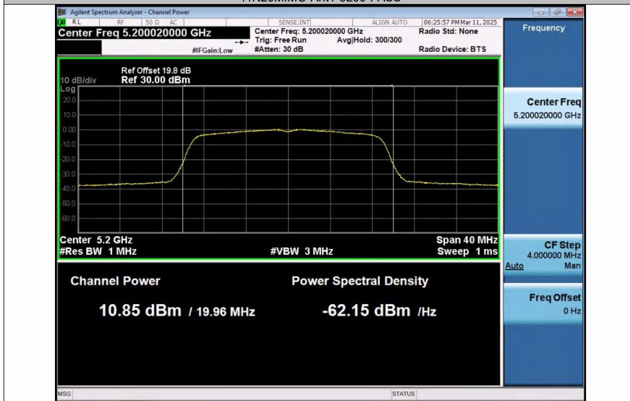
11N20MIMO-Ant2-5200-PASS
