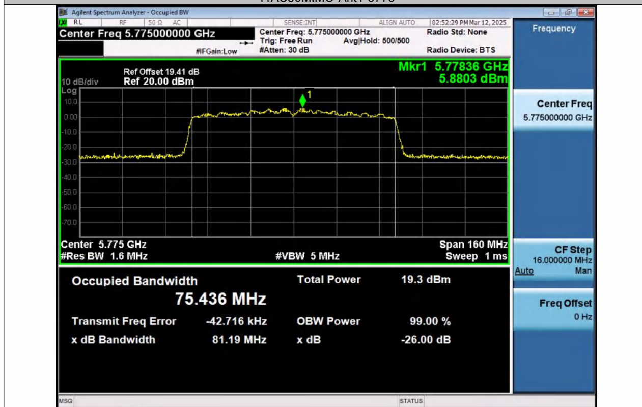
11AC80MIMO-Ant2-5775
