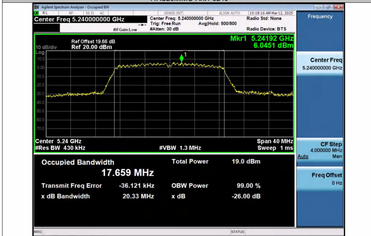
11AC20MIMO-Ant2-5240
