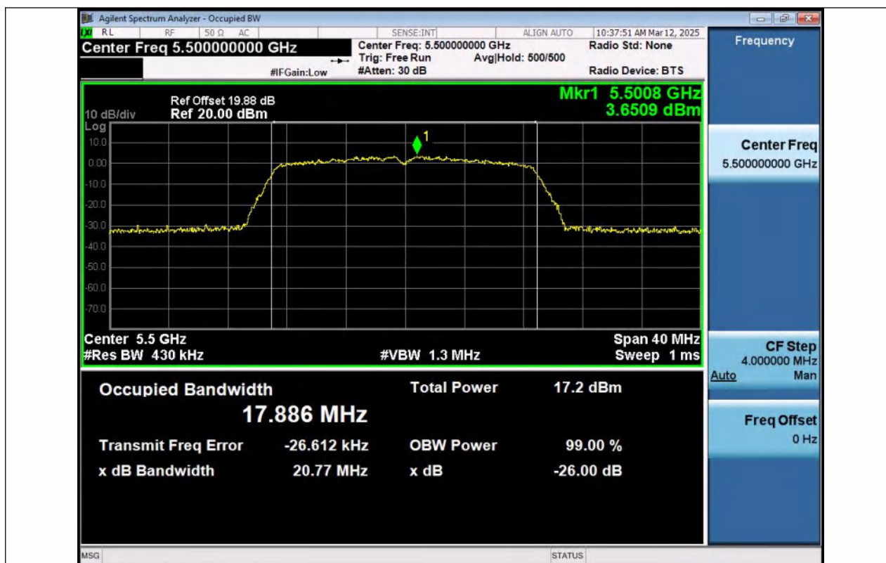
11AC20MIMO-Ant1-5500
