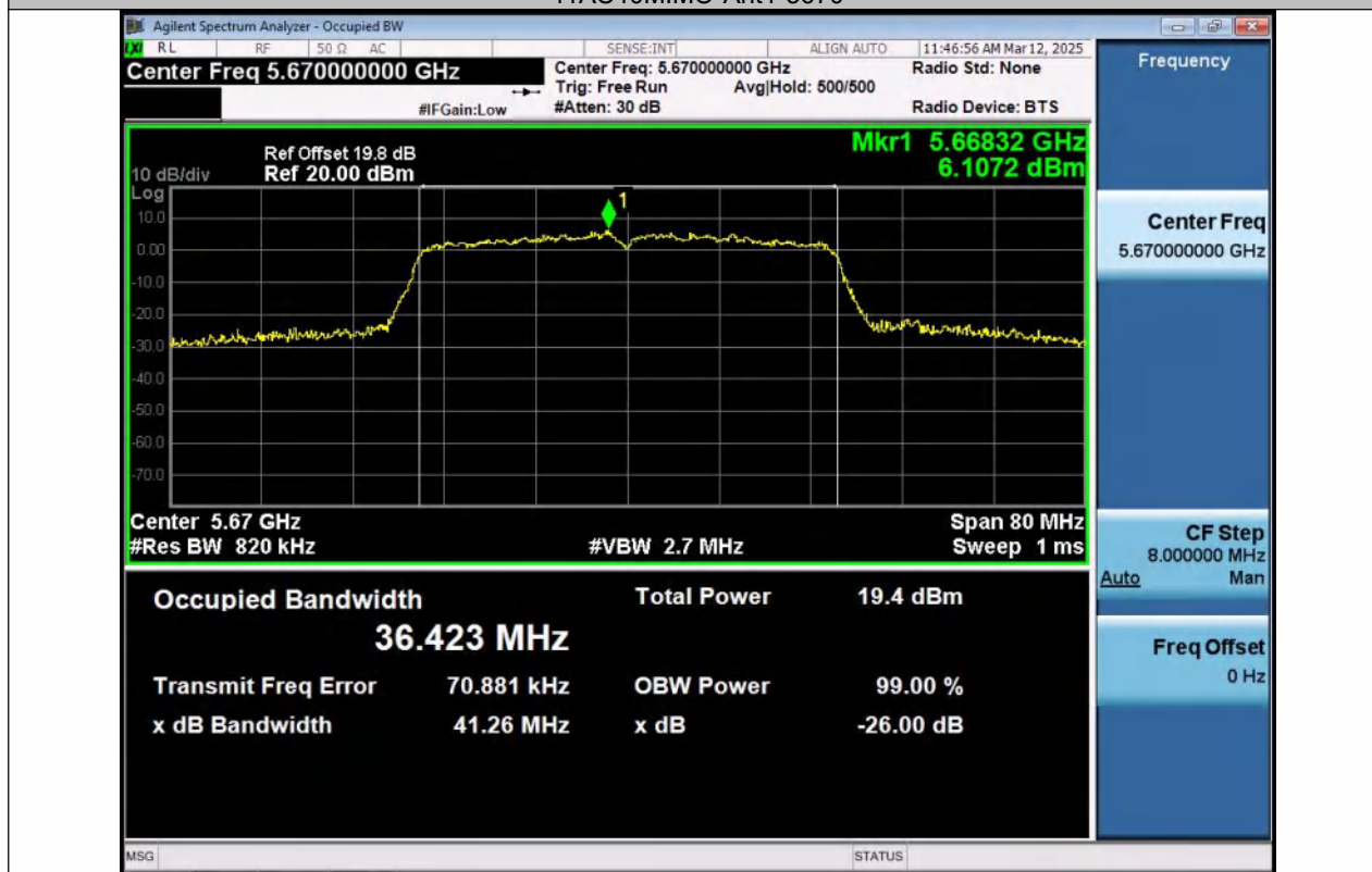
11AC40MIMO-Ant2-5670
