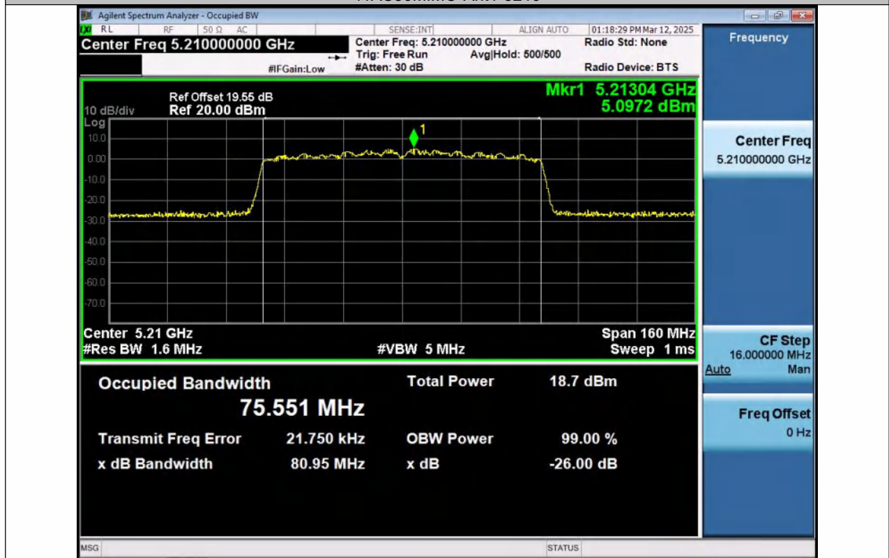
11AC80MIMO-Ant2-5210
