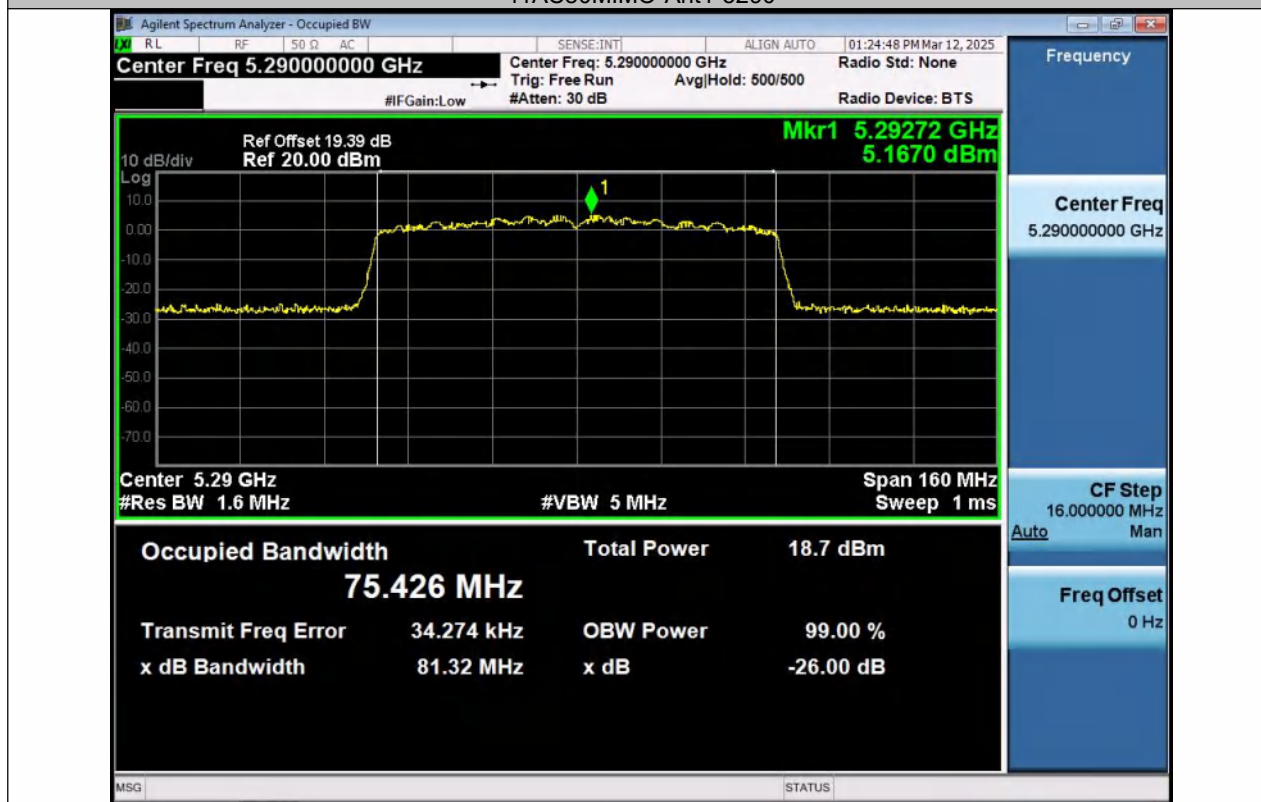
11AC80MIMO-Ant2-5290
