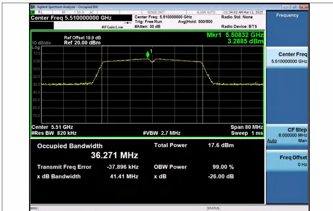
11AC40MIMO-Ant1-5510
