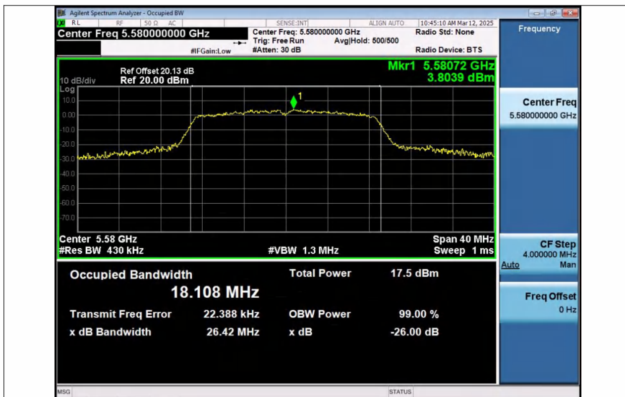
11AC20MIMO-Ant1-5580
