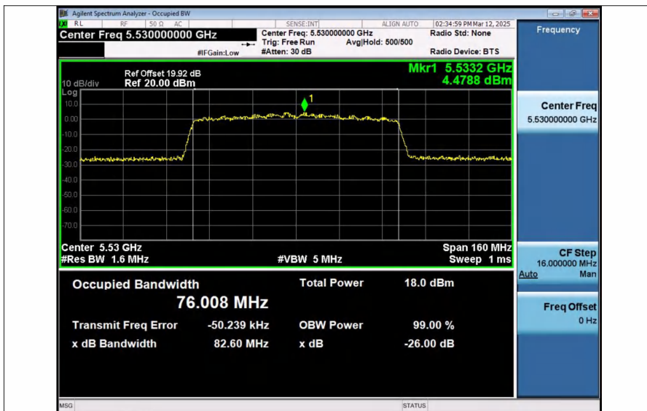
11AC80MIMO-Ant1-5530
