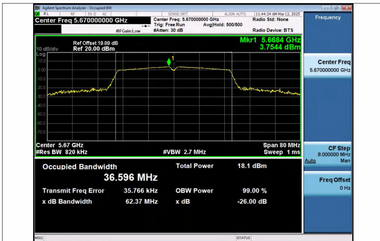
11AC40MIMO-Ant1-5670
