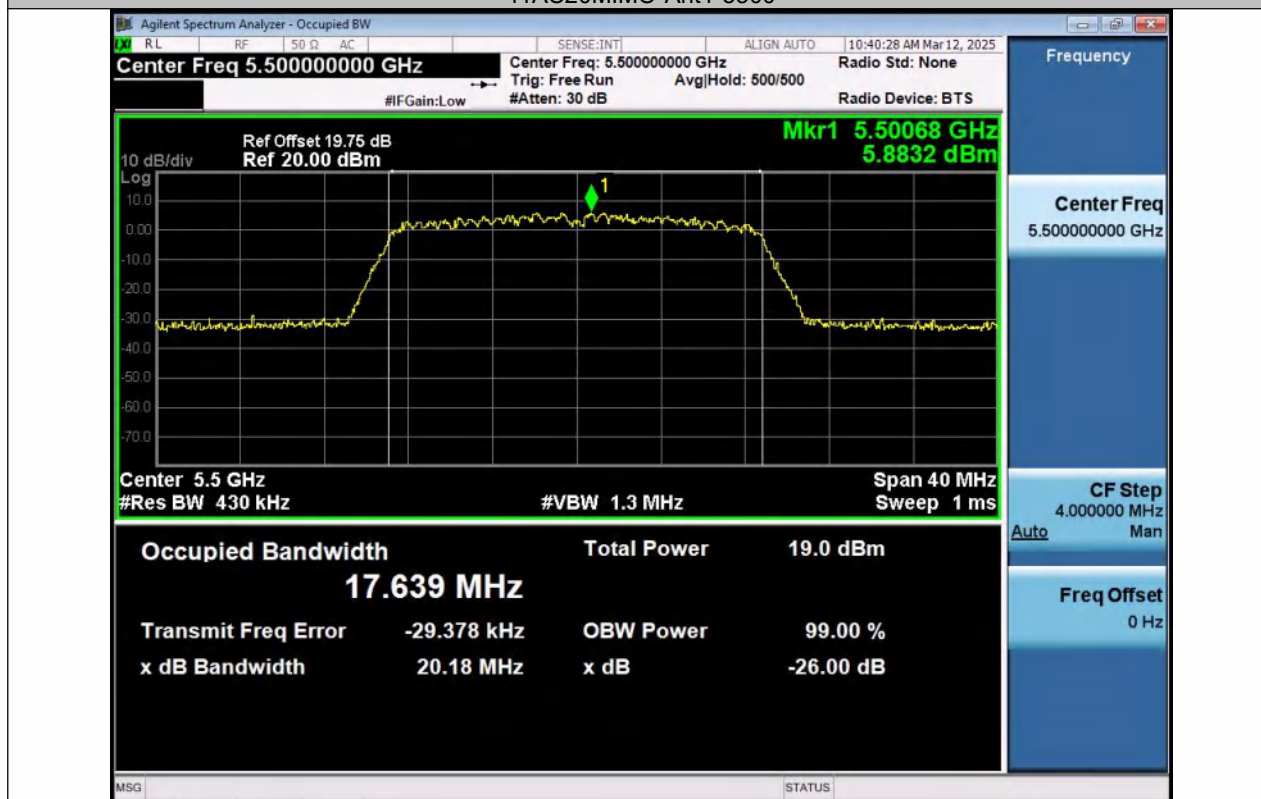
11AC20MIMO-Ant2-5500
