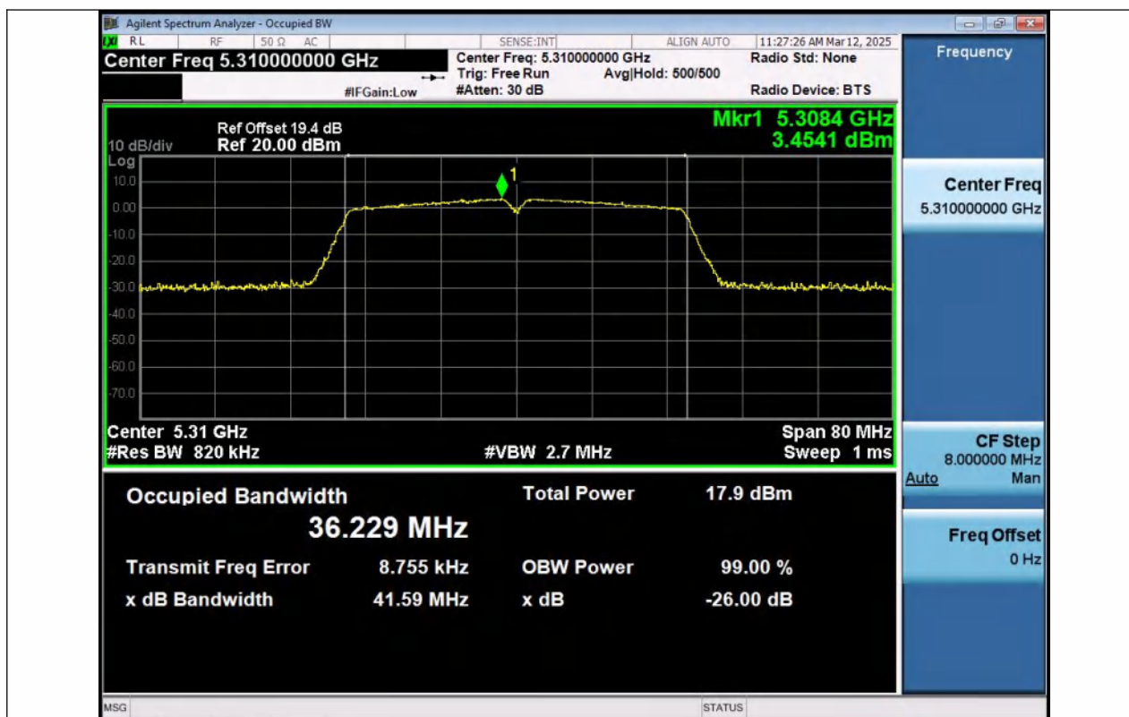
11AC40MIMO-Ant1-5310
