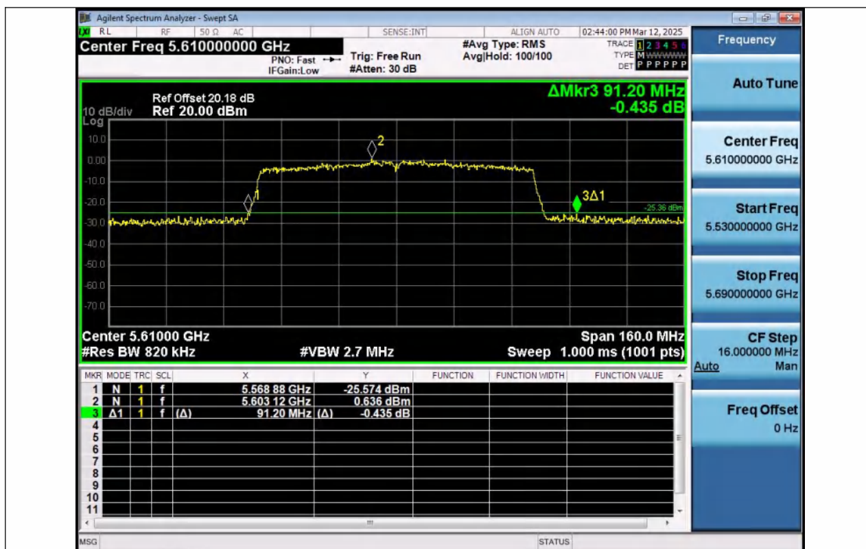
11AC80MIMO-Ant1-5610
