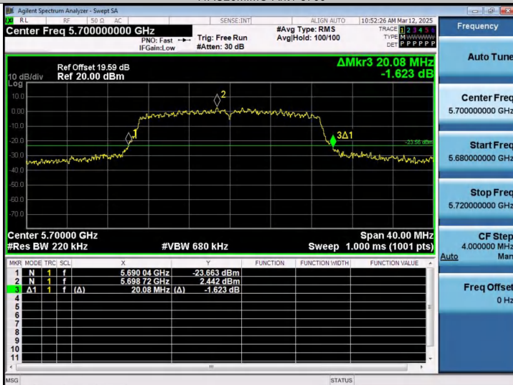
11AC20MIMO-Ant2-5700
