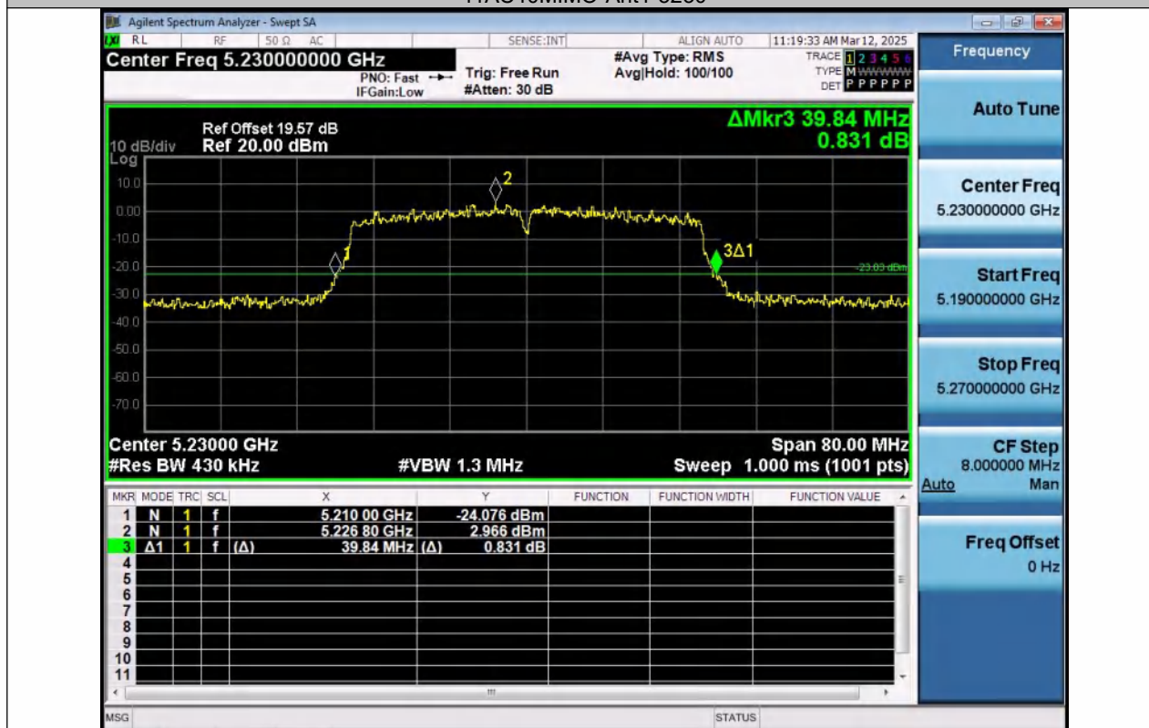
11AC40MIMO-Ant2-5230
