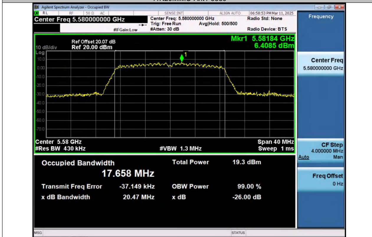
11N20MIMO-Ant2-5580
