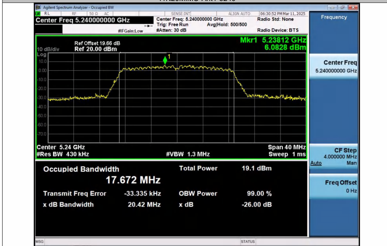
11N20MIMO-Ant2-5240
