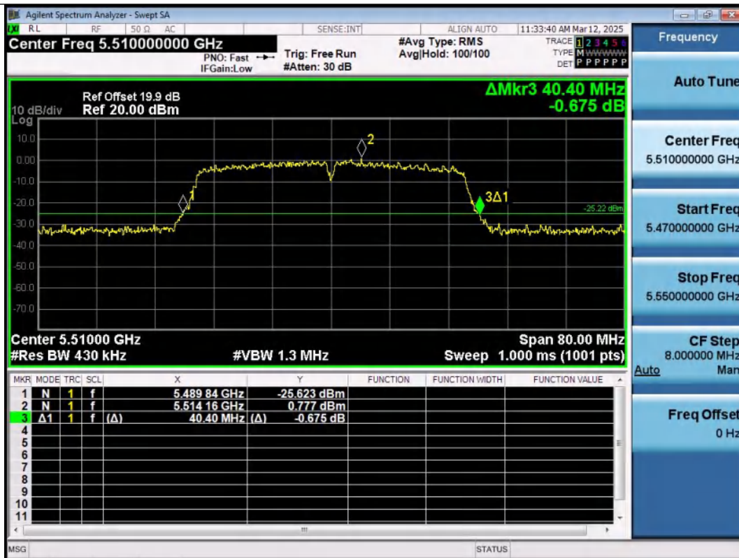
11AC40MIMO-Ant1-5510
