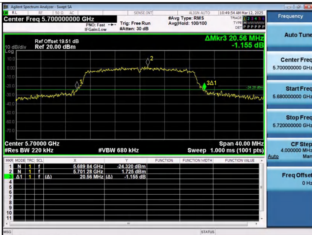
11AC20MIMO-Ant1-5700
