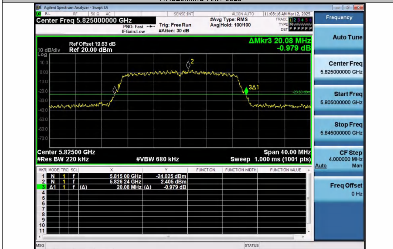
11AC20MIMO-Ant2-5825
