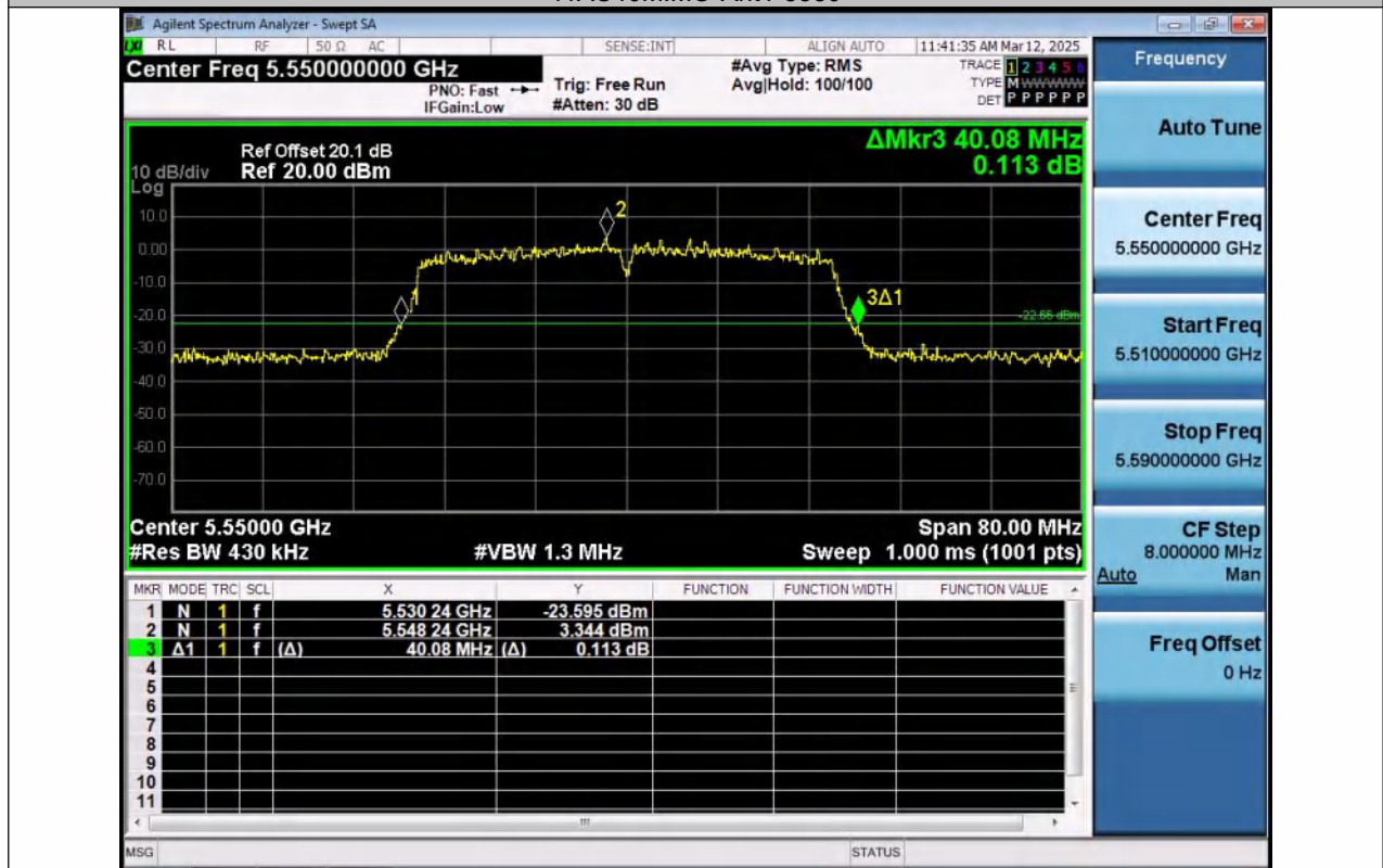
11AC40MIMO-Ant2-5550
