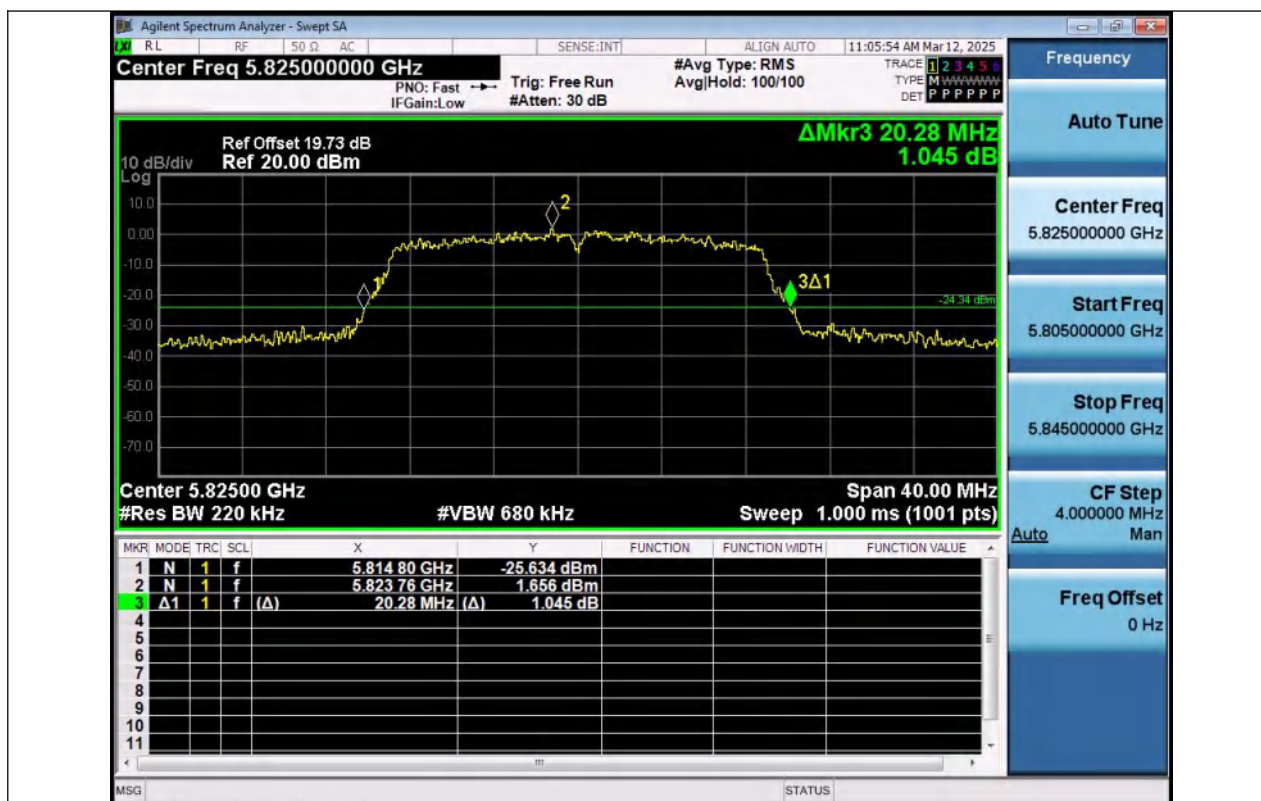
11AC20MIMO-Ant1-5825
