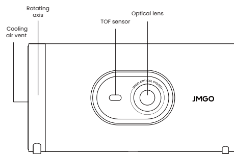
Projector Body
