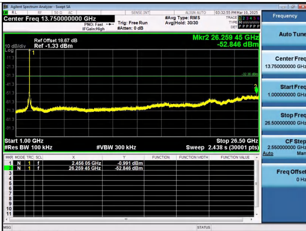
11N40MIMO-Ant1-2452-1000~26500-PASS
