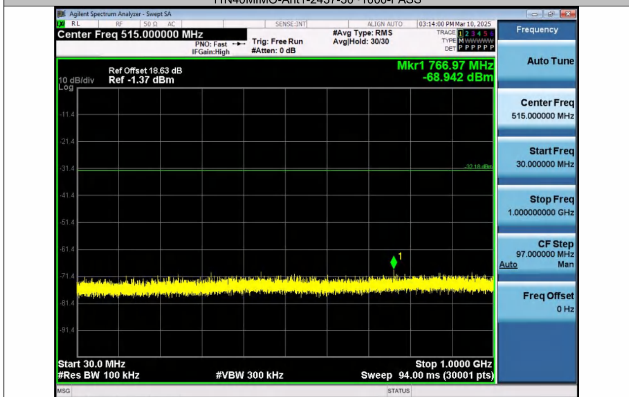
11N40MIMO-Ant2-2437-30~1000-PASS
