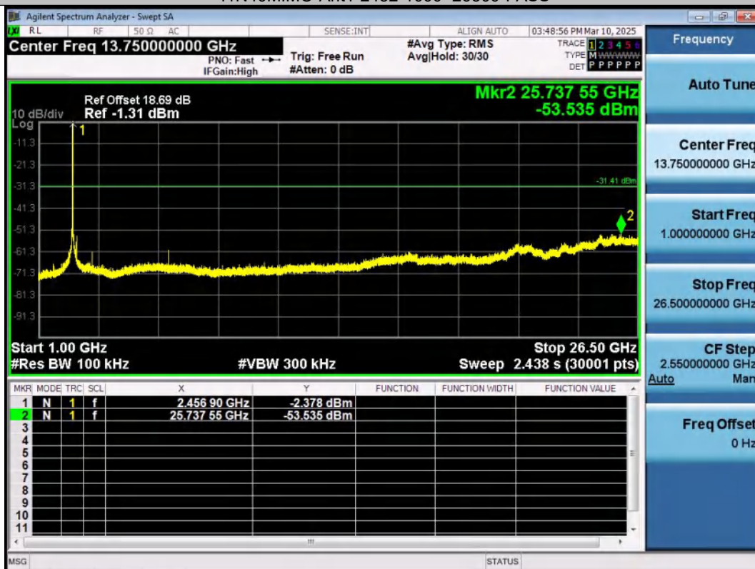
11N40MIMO-Ant2-2452-1000~26500-PASS
