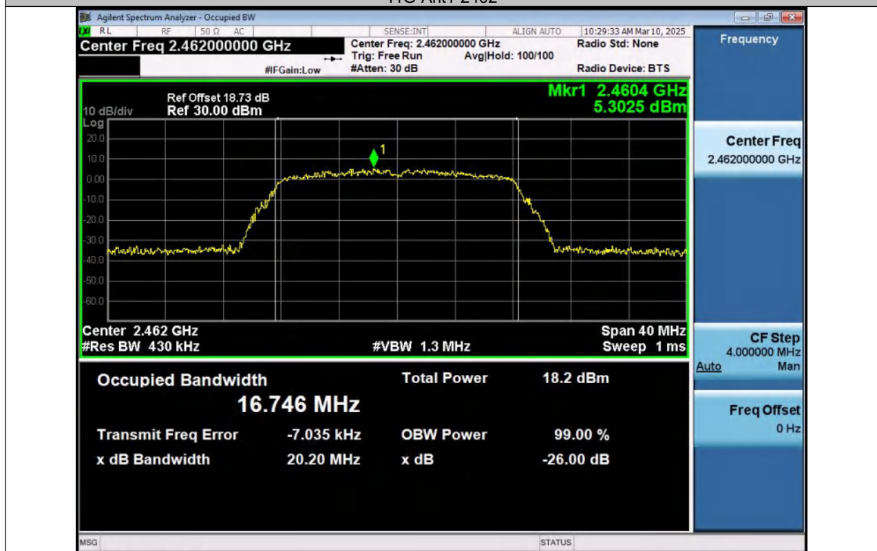
11G-Ant2-2462
