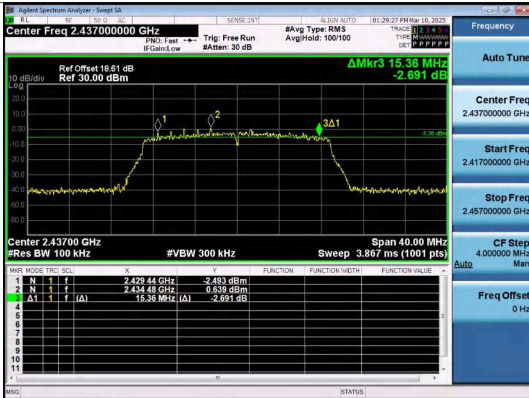
11N20MIMO-Ant1-2437-PASS
