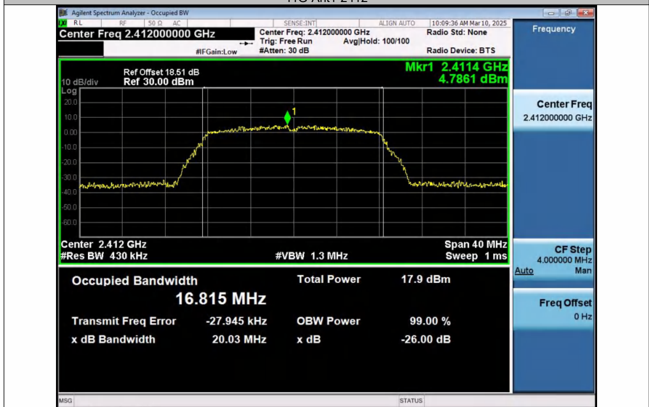
11G-Ant2-2412
