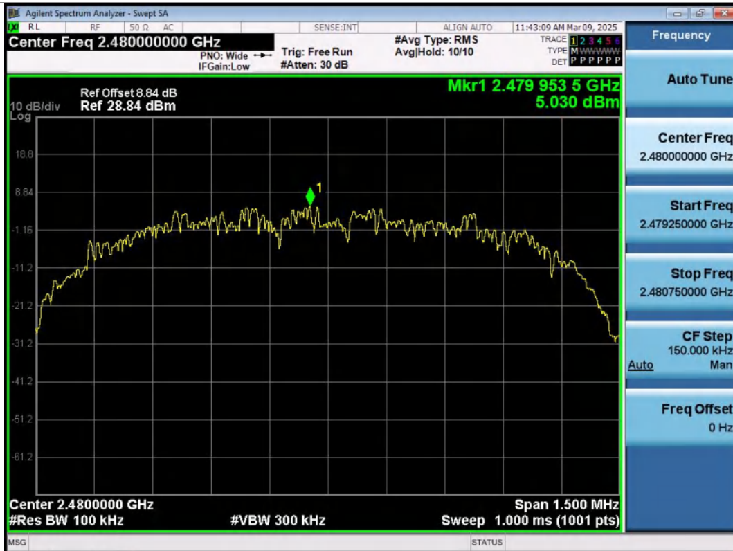
3DH5-Ant1-2480-0~Reference-PASS
