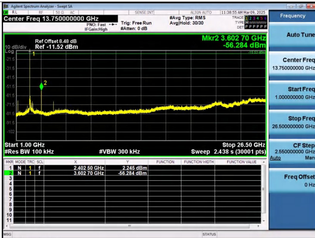
3DH5-Ant1-2402-1000~26500-PASS
