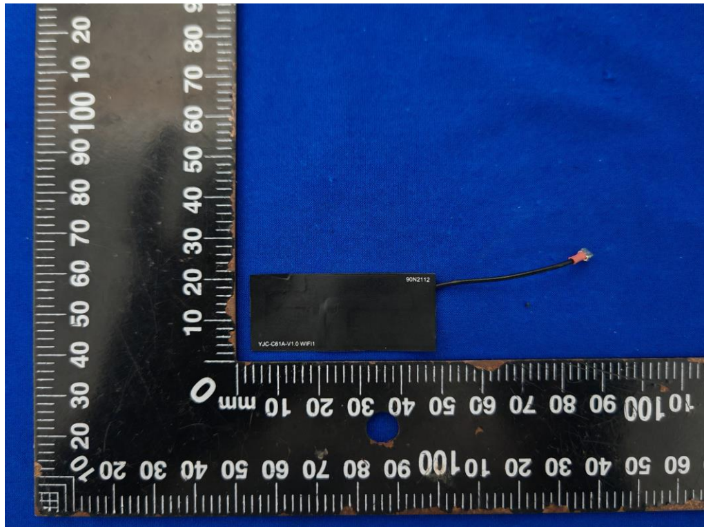
26) EUT Photo (WIFI ANT A)
