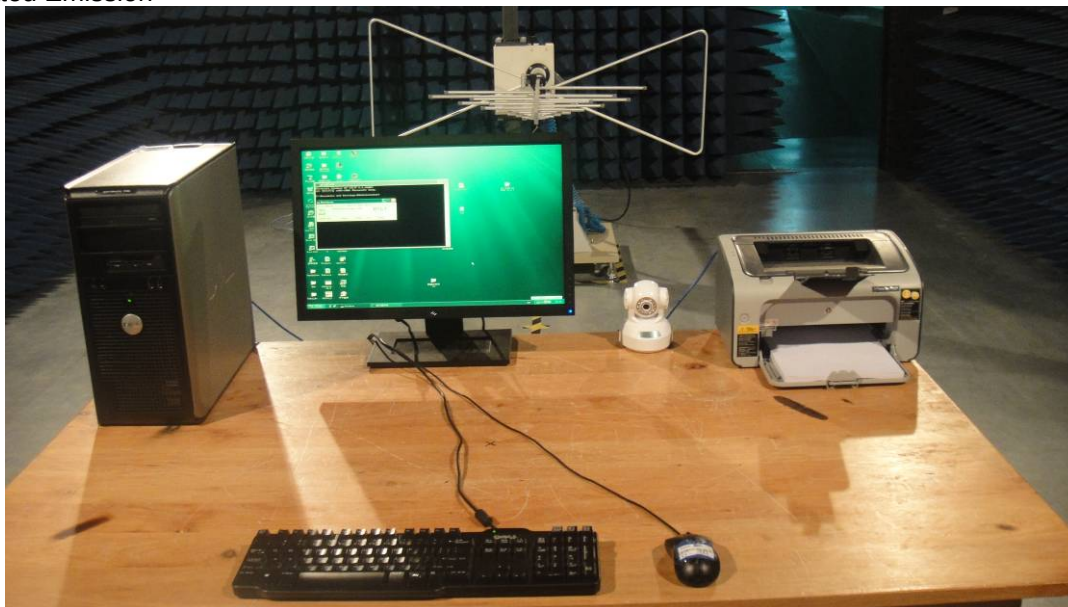
Radiated Emission
