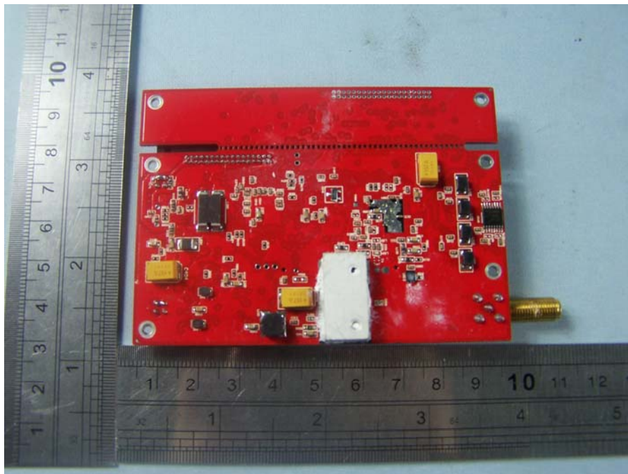
Radio board- bottom view
