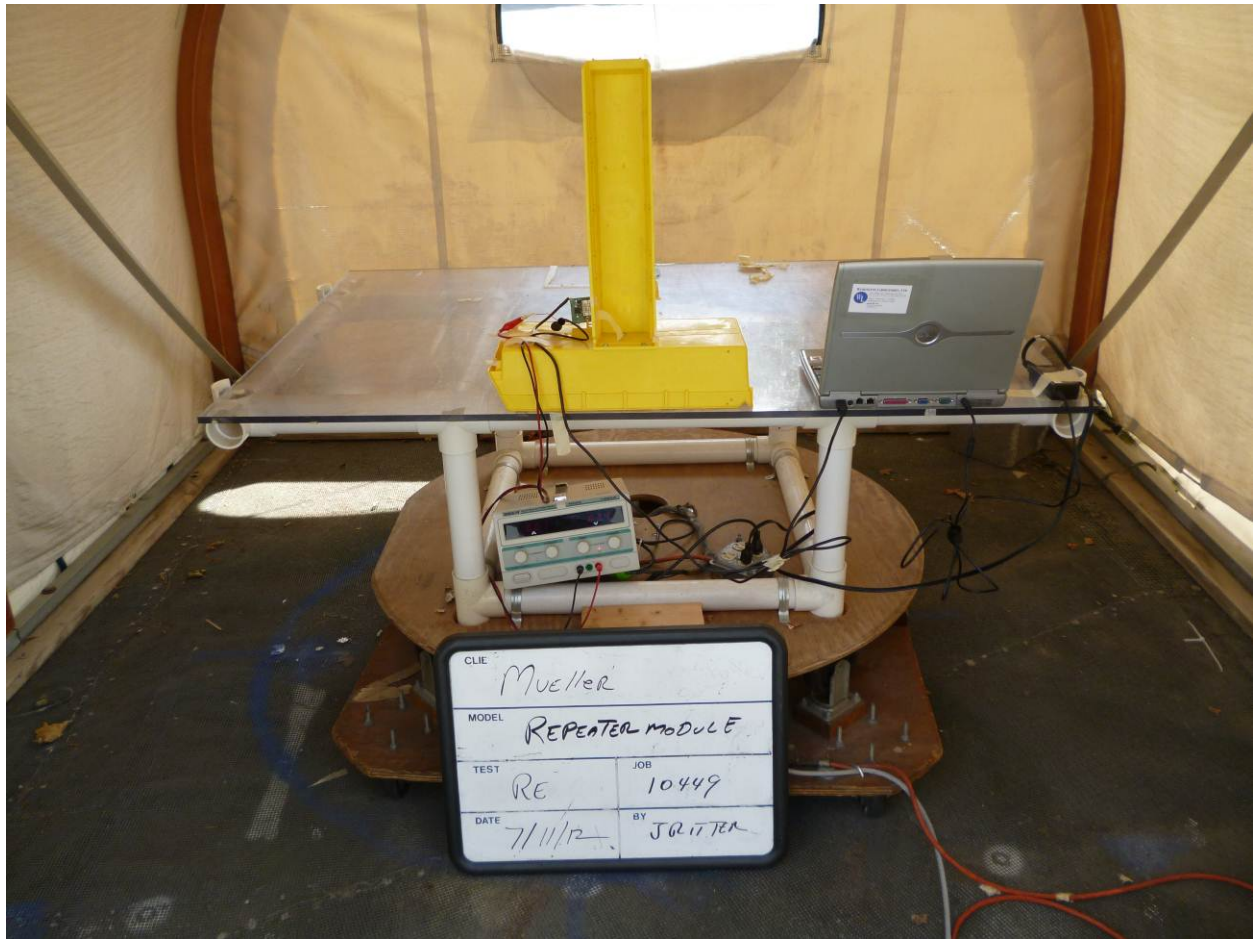
Figure 4- Set up for radiated emissions testing, back view
