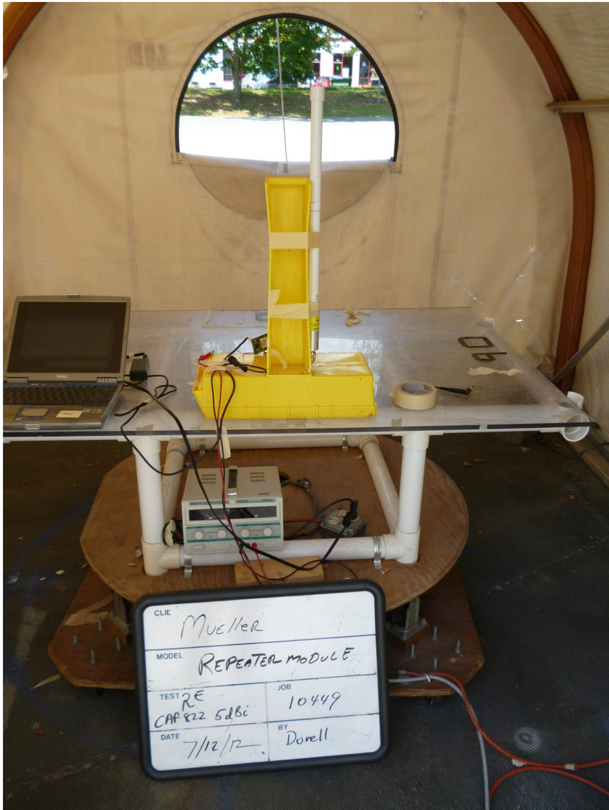
Figure 7- Set up for radiated emissions testing, front view
