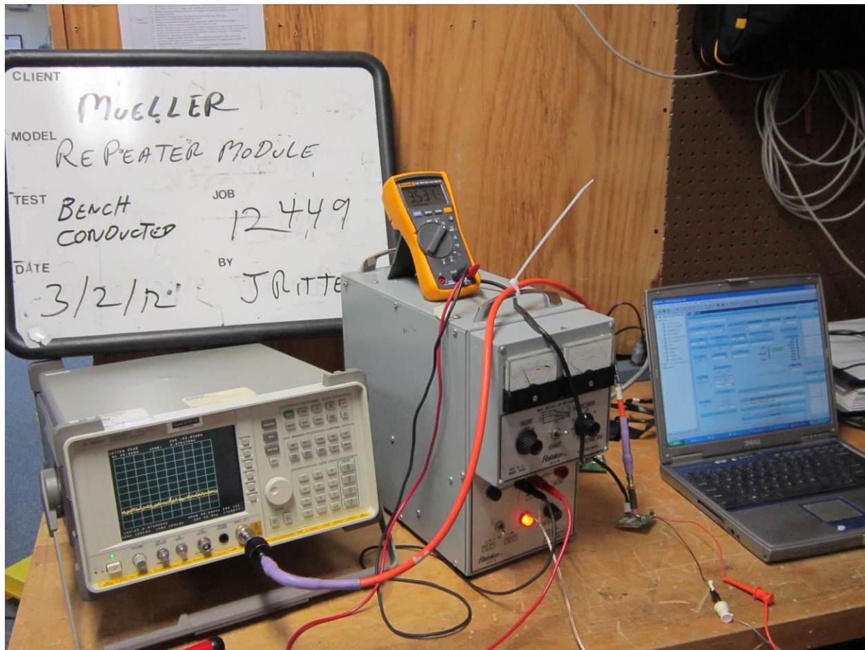
Figure 2 - Set up for conducted testing
