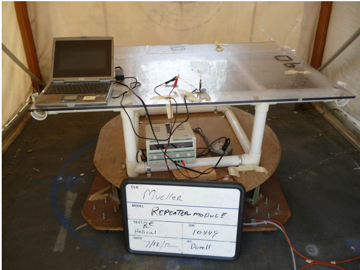
Figure 8- Set up for radiated emissions testing, front view
