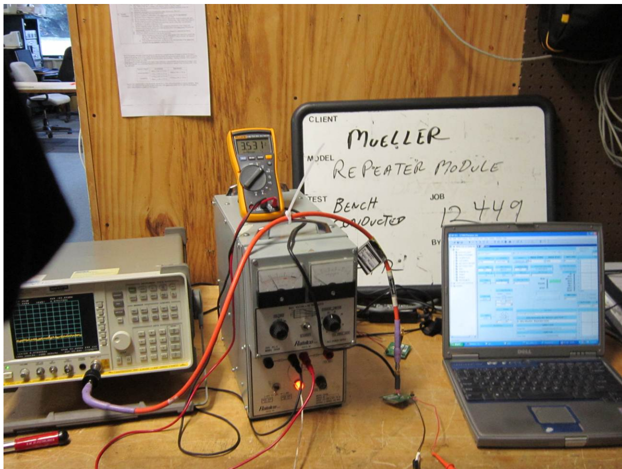
Figure 1- Set up for conducted testing
