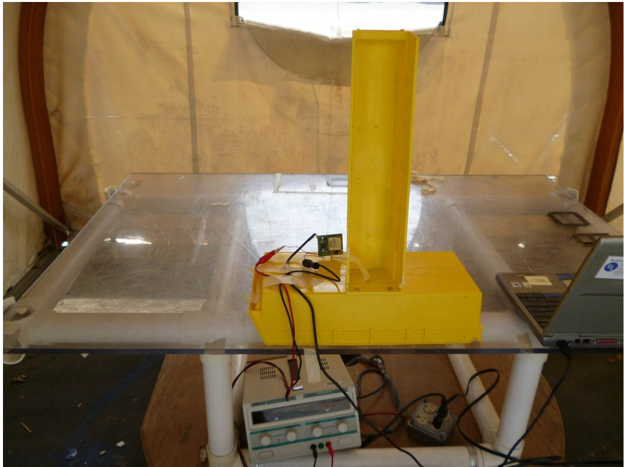
Figure 5- Set up for radiated emissions testing, back view
