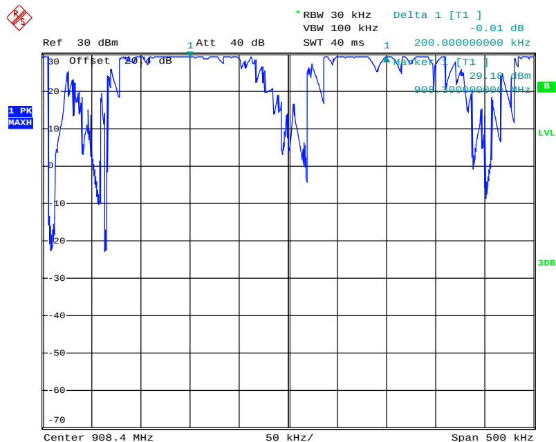
Figure 7.3.1.2-4: Carrier Frequency Separation – LoRaWAN – SF8
