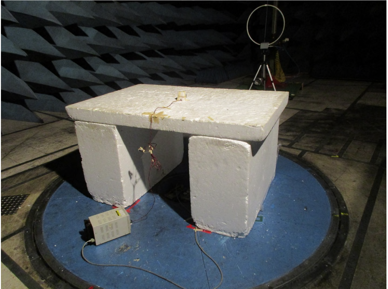
Figure 2: Radiated Emissions – Back View – 9 kHz to 30 MHz
