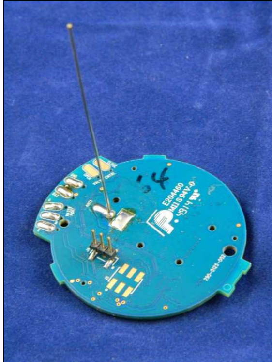
Figure 2: External Photo – Monopole Antenna
