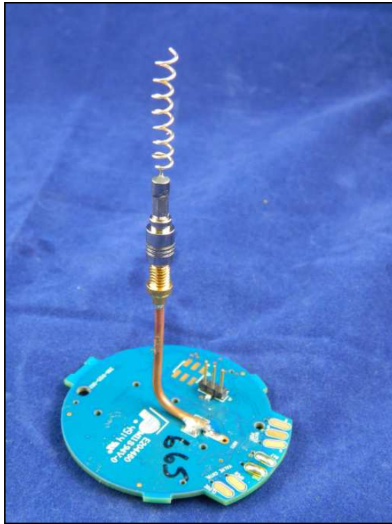
Figure 1: External Photo – Helical Antenna
