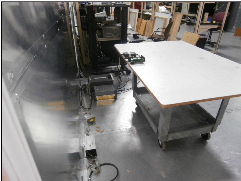
Figure 8: Conducted Emissions – Printed Inverted F Antenna
