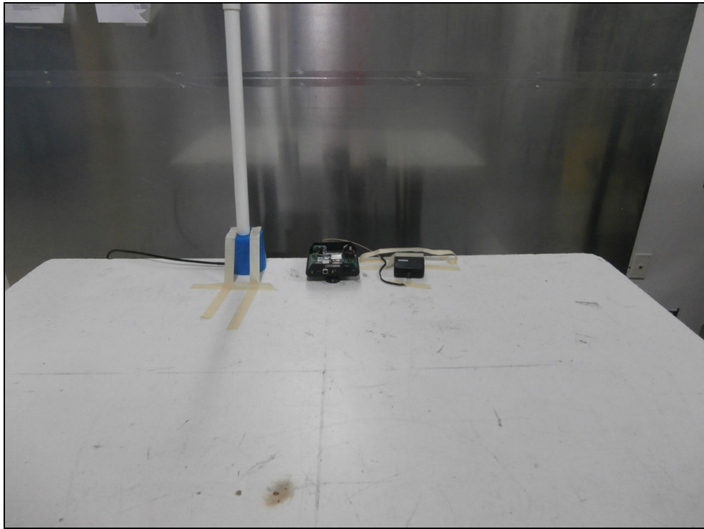
Figure 5: Conducted Emissions – Dipole Antenna
