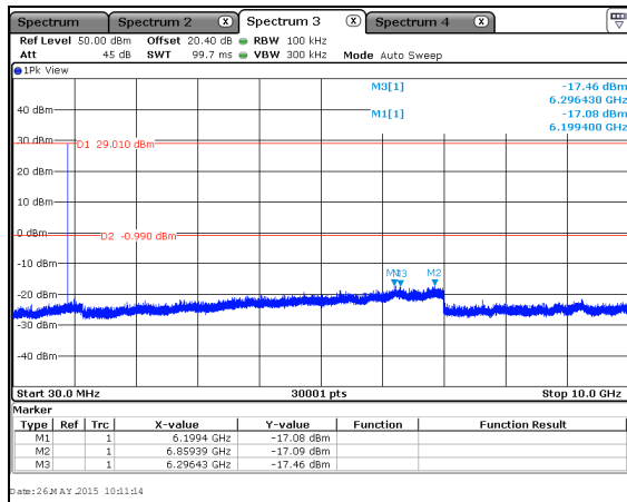
Figure 7.5.1.2-2: 30 MHz – 10 GHz – MCH
