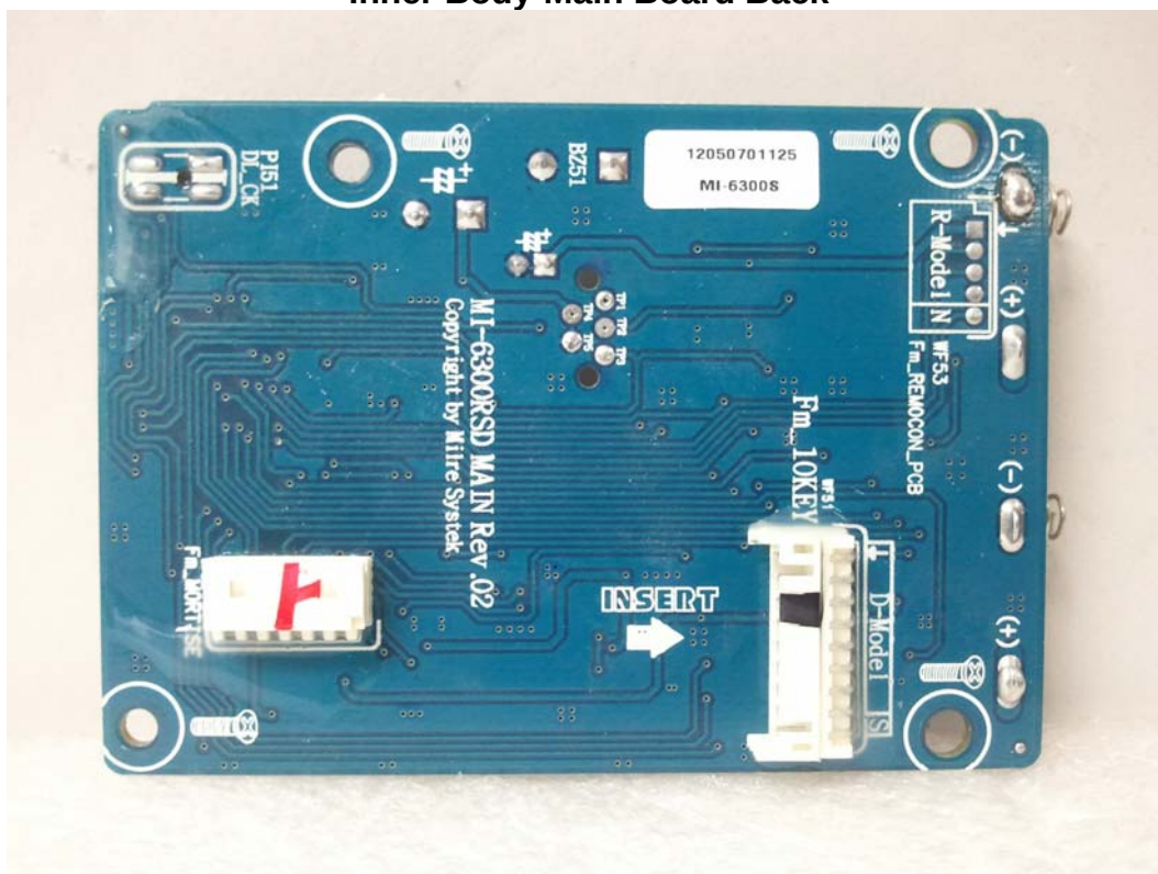
Inner Body-Main Board Back
