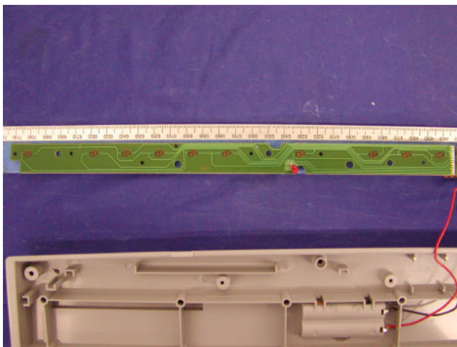
EUT – Board Component View
