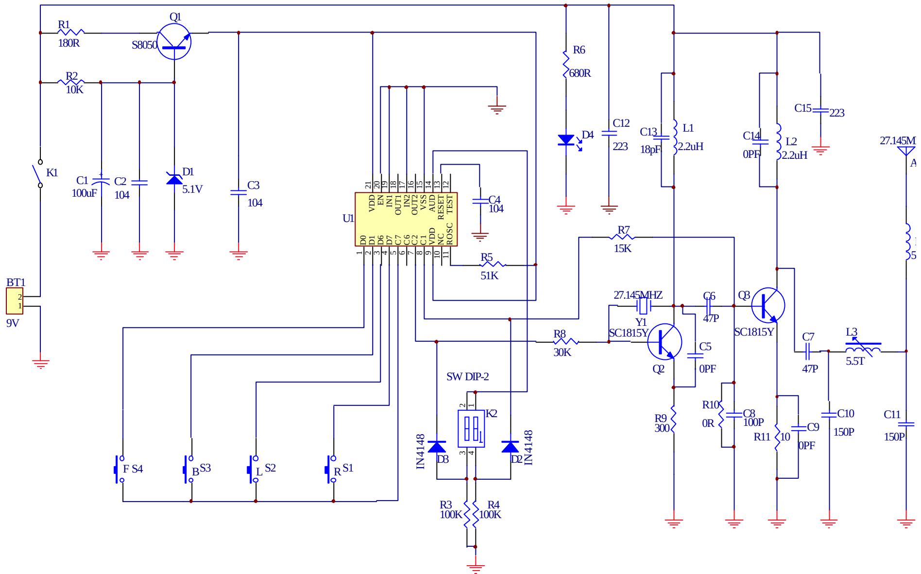
27.145MHZ TX CIRCUIT SCHEMATIC
