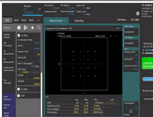
7-7-20MHz-20MHz-16QAM-16QAM -21001-21199-100RB#0-100RB#0
